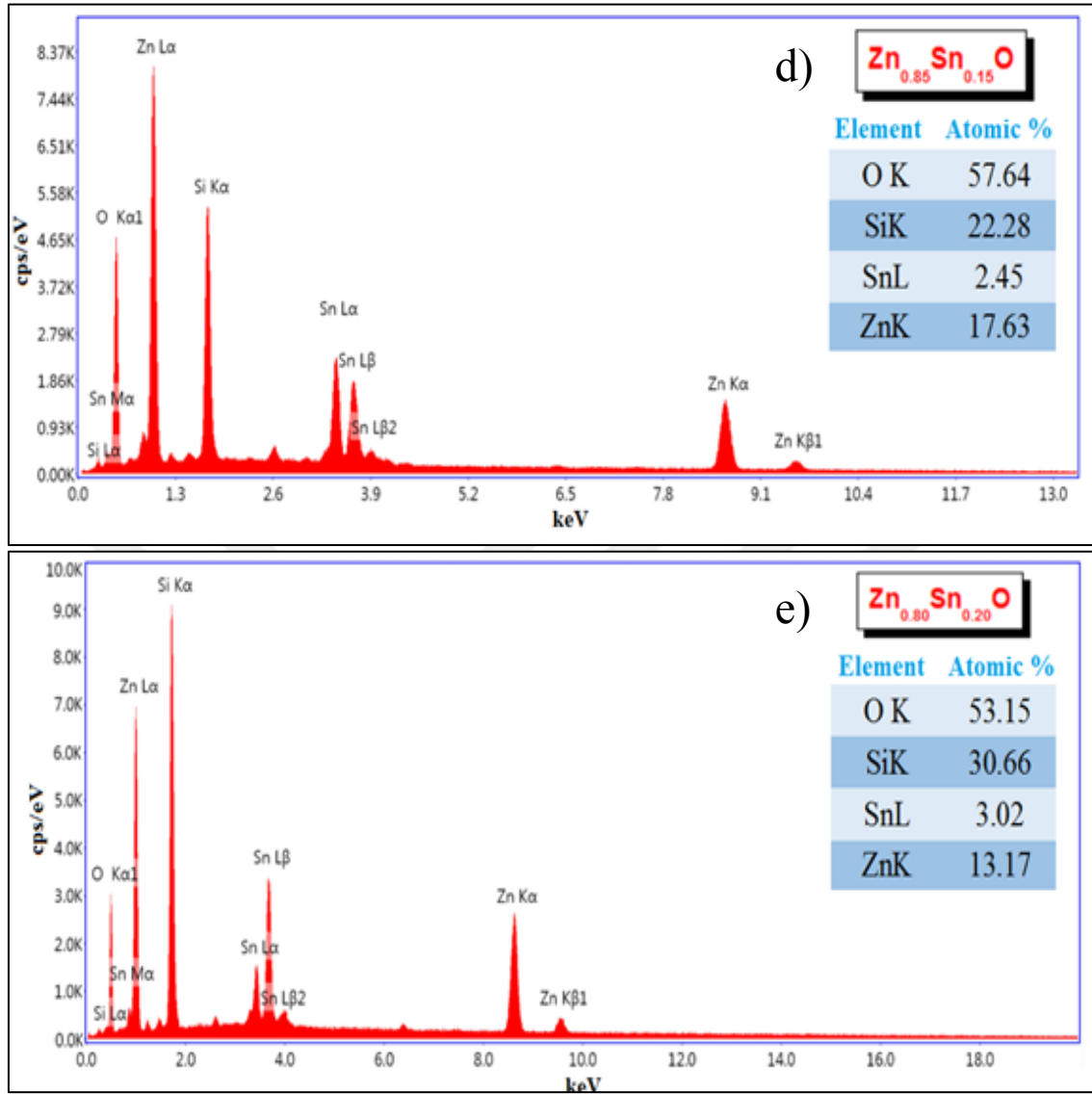
Şekil 6.3. (Devamı) a) ZnO b) \text{Zn}_{0.95}\text{Sn}_{0.05}\text{O} c) \text{Zn}_{0.90}\text{Sn}_{0.10}\text{O} d) \text{Zn}_{0.85}\text{Sn}_{0.15}\text{O} e) \text{Zn}_{0.80}\text{Sn}_{0.20}\text{O} sensörlerinin EDAX görüntüleri
