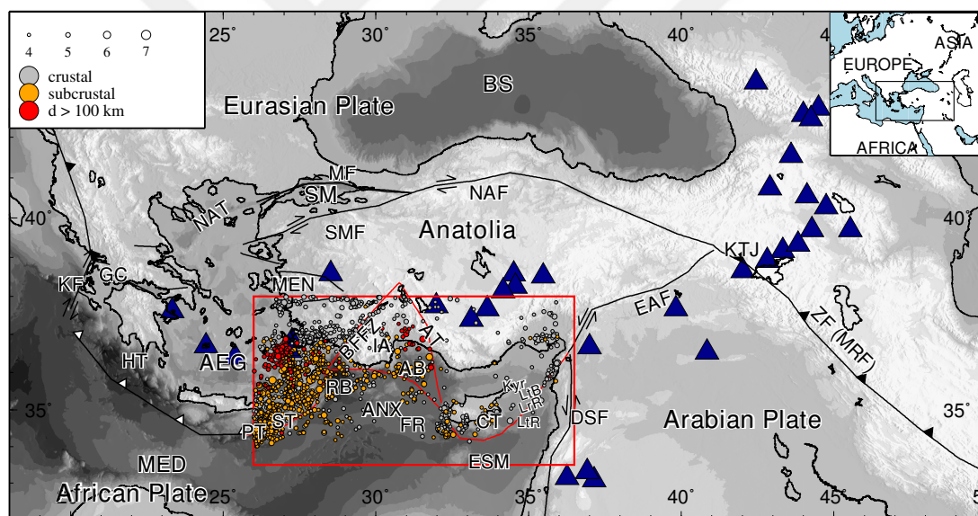
Figure 3.1: Tectonic setting of the Eastern Mediterranean. We mainly focus on the location and nature of (possible) plate boundaries (red line segments) in the boxed region. Triangles on faults with black and white filling indicate collision and subduction zones, respectively. Conjugate arrows indicate the strike-slip character of faults; normal faults have no additional labels. Seismicity in the box is shown for the period of 1973–2009 (NEIC, https://earthquake.usgs.gov/earthquakes/search/ , Last Accessed:02-07-2019). The distinction between crustal and subcrustal earthquakes is based on the Moho depth map of Grad et al. (2009). Loci of subcrustal and deep seismicity are Hellenic and Cyprus trenches. Blue triangles indicate active volcanism. Abbreviations: AB, Antalya Basin; AEG, Aegean Sea; ANX, Anaximander Mountains; AT, Aksu Thrust; BFFZ, Burdur Fethiye Fault Zone; BS, Black Sea; CT, Cyprus Trench; DSF, Dead Sea Fault; EAF, East Anatolian Fault; ESM, Eratosthenes Seamount; FR, Florence Rise; GC, Gulf of Corinth; HT, Hellenic Trench; IA, Isparta Angle; KF, Kephallonia Fault; KTJ, Karhova Triple Junction; Kyr, Kyrenia Ridge; LrT, Larnaka Ridge; LtB, Latakia Basin; LtR, Latakia Ridge; MED, Mediterranean Sea; MEN, Menderes Massif; MF, Marmara Fault; NAF, North Anatolian Fault; NAT, North Aegean Through; PT, Pliny trench; SM, Sea of Marmara; SMF, Southern Marmara Fault; ST, Strabo Trench; ZF, Zagros Fault (Main Recent Fault).
