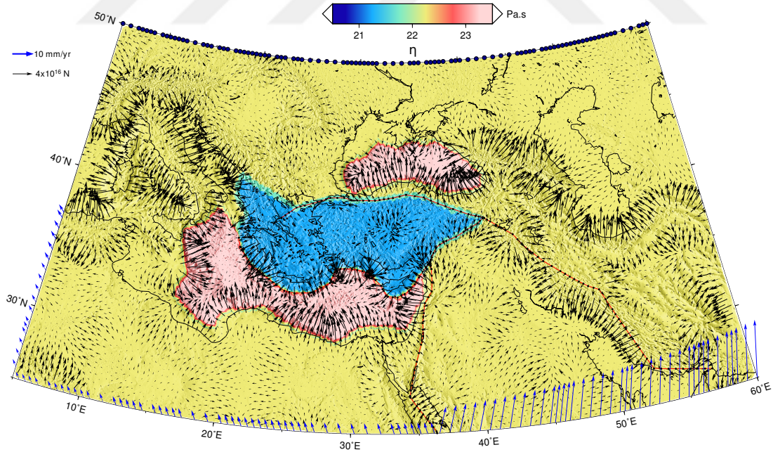
Figure D.1: Model domain and boundary conditions (blue arrows) of GPE-driven models. The specific model shown here is for relatively low Aegean-Anatolian viscosity, and for horizontal forces (black arrows) computed with the assumption that the lithosphere is not isostatically compensated. Logarithmic viscosity contours are draped over shaded relief.
