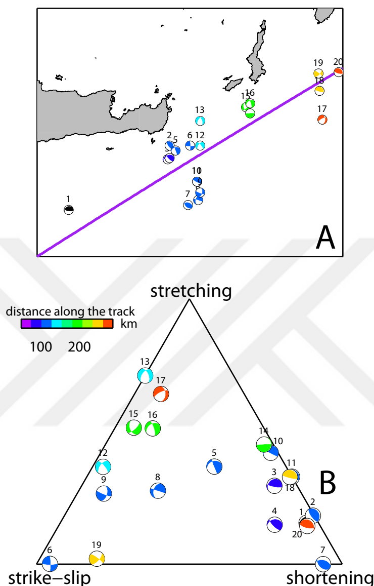
Figure 2.6: (A) Focal mechanisms colored according to their distance along the purple line, which roughly shows the strike of PSSZ. The distance is measured from the tip of the active STEP. (B) Ternary diagram of focal mechanisms with color coded spatial distributions.
