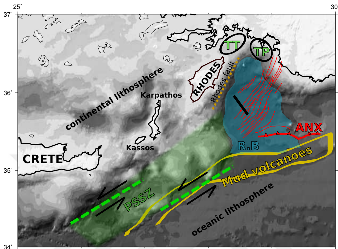
Figure 2.5: Summary figure showing the deformation agents near the PSSZ and Rhodes. The green dashed lines and the green transparent area are the PSSZ; yellow ribbon is the extent of the mud volcanism (Huguen et al. , 2006); transparent blue region is the Rhodes basin (R.B); dotted orange line segment off the SE coast of Rhodes is the Rhodes fault (after Kontogianni et al. (2002)); thick red teethed line indicates the eastern Mediterranean lithosphere underthrusting below Anaximander Mountains (ANX); red thin line segments show Hall et al. 's (2009) fold and thrust belt; thick black line segment is the seismic reflection line in which Woodside et al. (2000) identified a transpressional fault perpendicular to it; TT and TP refers to the transpression and transtensional zones of Oçakoglu (2012), with bounding ellipses indicating their extent.
