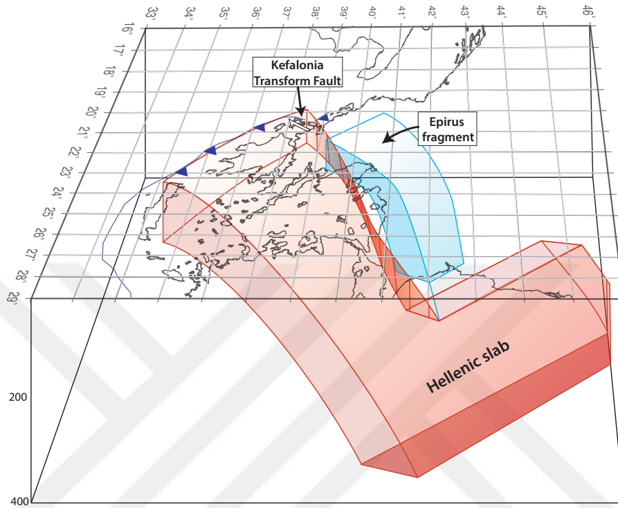
Figure 4.12: Summary block diagram of our interpretation of the structure of the west Hellenic subduction zone and the Epirus fragment (the eastern part is cut off here, and does not correctly display the actual structure)
