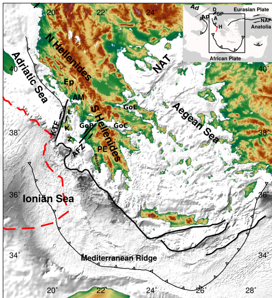
Figure 4.2: Topography/bathymetry of the Hellenic subduction zone. The extent of the Ionian oceanic crust is marked by red dashed lines (Chamot-Rooke et al. , 2005), thick black lines represent the approximate location of plate contacts and major faults, and the trench physiography is shown with thin barbed black lines. Abbreviations refer to: AM: Amvrakikos Gulf; AFZ: Achaia Fault Zone; Ep: Epirus; GoC: Gulf of Corinth; GoE: Gulf of Evia; GoP: Gulf of Patras; K: Kefalonia; L: Levkas; PE: Peloponnesus; Z: Zakynthos; KTF: Kefalonia Transform Fault; NAT: North Aegean Trough; Inset map shows central and eastern Mediterranean subduction/collision zones. A: Albanides, Ad: Adria, Ap: Apulia, D: Dinarides, H: Hellenides, NAF: North Anatolian Fault, SP: Scutari-Pec.
