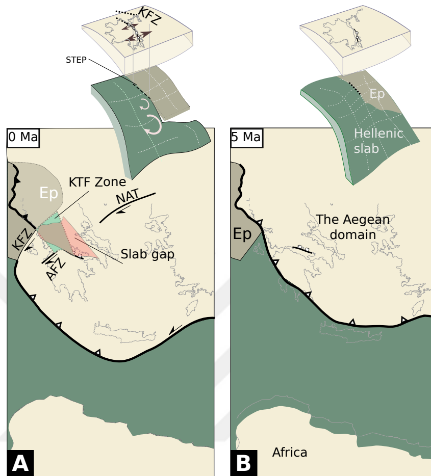
Figure 4.13: Tectonic evolution of the Hellenic slab and the overriding plate deformation. Circular arc with arrows indicate sagging/rotation of the subducted slab. Gray lines on 0 Ma show the plate boundary geometry of the 5 Ma setting.
