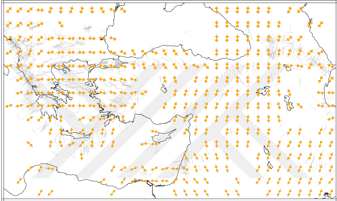
Figure A.1: World stress map data, smoothed stress field, and stress variances.
