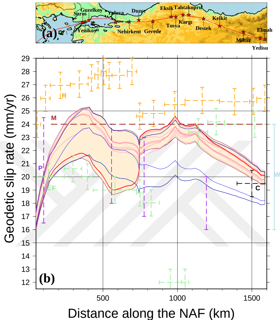
Figure 3.8: Comparison of present-day slip-rates on the North Anatolian Fault (NAF) zone with fault slip-rates from our models. a) Shaded relief map of the NAF region locations of geological slip-rate studies (red stars). b) Model slip-rates of SOUTH (orange shaded band) and NORTH (blue hatched band), with individual model slip-rate results shown by red and blue lines, respectively. Thick red line represents our best model (SOUTH-6). Model slip-rates are calculated for the northern branch of the NAF, whose geometry is given nearly parallel to the plot axis shown in panel (a). Brown colored line with label ‘M’ indicates the rate determined from the Eurasia-Anatolia Euler pole (McClusky et al. , 2000). Discrete orange boxes with label ‘R’ represent the slip-rates from Reilinger et al. (2006) block model, where computation error is defined by the height of each box. Light green discrete lines with label ‘F’ represent Flerit et al. (2004) model slip-rates. Purple error bars with label ‘P’ indicate slip-rates determined from Provoost et al. (2003). The seismic slip-rate estimates (Table 3.3, light blue bar at the right end of plot area) span a range of 16-24 mm/year for the NAF and represent the slip-rate value for the whole fault zone.
