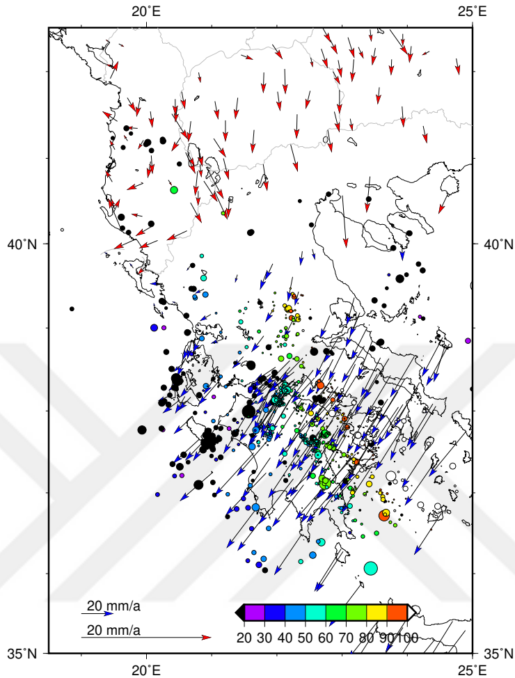
Figure 4.3: GNSS-derived horizontal velocity field and seismicity. The velocities are relative to stable Europe, and are compiled from Jouanne et al. (2012), Nocquet (2012), and Metois et al. (2015). Please note that velocity vectors are 4 times larger for sites north of 40°N to allow better evaluation. Relocated earthquakes for the upper-crust (top 20 km) marked with black circles –symbol size is scaled with the magnitude (Halpaap et al. , 2018), while earthquakes deeper than 20 km are colored according to their depth.
