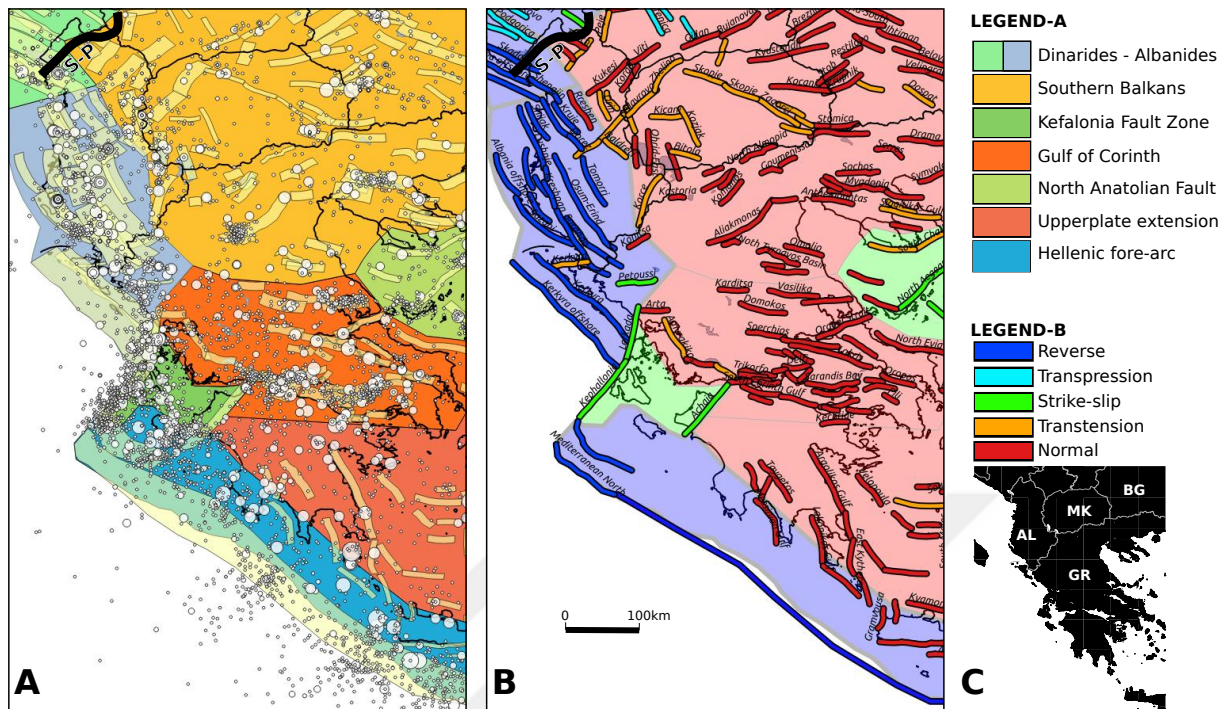
Figure 4.10: Map of seismic zones and active seismogenic faults modified from SHARE; The European database of Seismogenic Faults (Basili et al. , 2013). A. Seismogenic zones are shown in different colors. M4+ crustal seismicity is indicated with white circles, whose magnitudes are proportional to their radius. Faults are plotted with their surface projections in order to better illustrate limits of dipping interfaces. Thick black line label S-P indicates the Scutari-Pec line, which separates the Dinarides from the Albanides-Hellenides. B. Seismic zones of extension, transpression and compression are shown in red, green and blue shading. Fault names are taken verbatim from SHARE database. C. National borders of Balkan countries and Greece are mentioned in the text (GR:Greece, AL:Albania, MK: North Macedonia; BG: Bulgaria).
