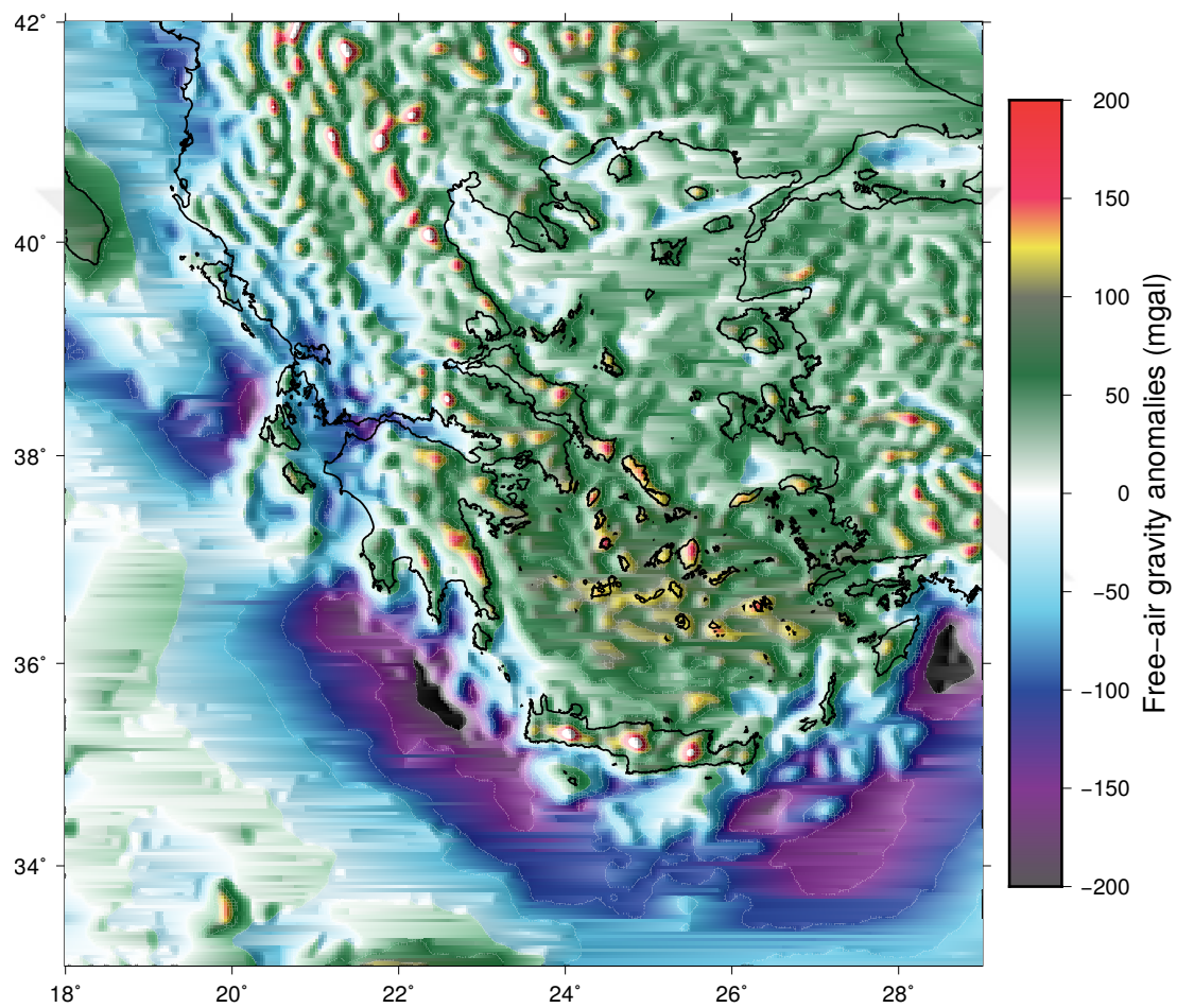
Figure A.4: Free-air gravity anomalies in our study area from the World Gravity Map (Bonvalot et al., 2012). The location of the SW-NE oriented 50 mgal anomaly to the SW of the KTF in the Ionian basin aligns with the velocity contrast within the Ionian lithospheric mantle (Figure 4.5B and C).
