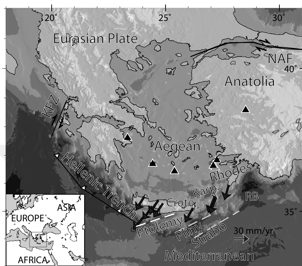
Figure 2.1: Bathymetry and the elements of eastern Mediterranean geodynamics. Arrows show the Aegean velocity field with respect to Africa. Dashed-lines indicate Ptolemy, Pliny and Strabo “trenches”; Triangles are volcanoes. NAF: North Anatolian fault; Karp.: Island of Karpathos; KFZ: Kephallonia fault zone; RB: Rhodes basin.
