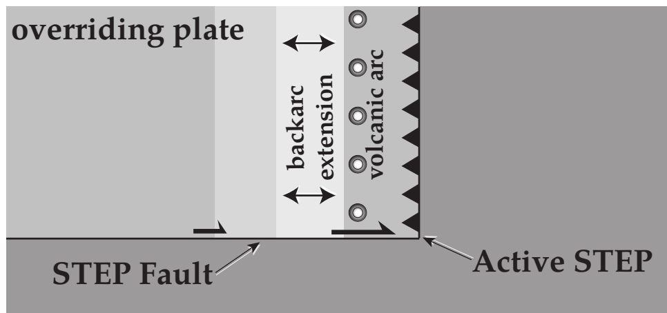
Figure 1.1: Schematic illustration of STEP fault.
