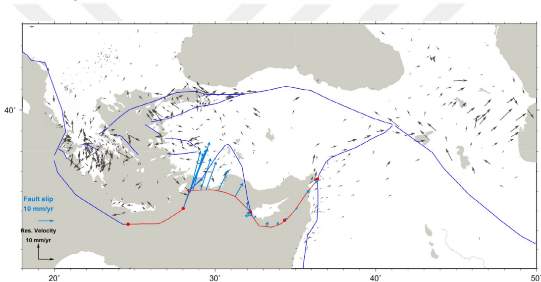
Figure 3.6: Velocity misfits (observed minus calculated) for model SOUTH-9, i.e. independent Isparta Block. The symbol explanations are the same as in Figure 3.5 .
