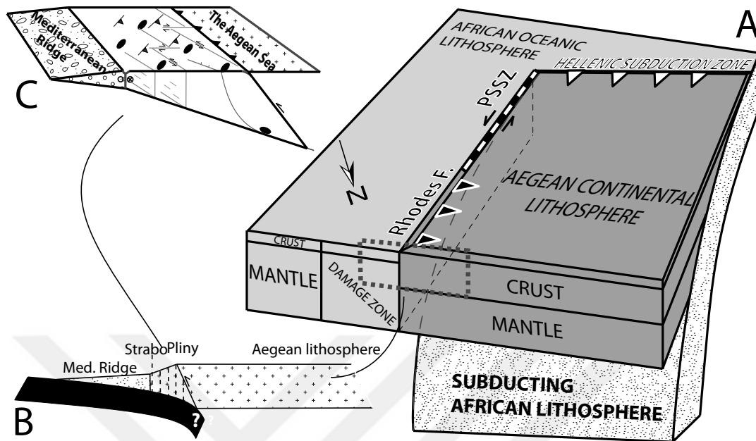
Figure 2.4: (A) Block diagram schematically indicating the structure of the eastern part of the Hellenic subduction zone (modified from Baes et al. (2011)). The structure indicated in (A) can be seen as a schematic indication of the starting situation upon which the effect of compression should be superimposed. Triangles with white and black fill indicate subduction and thrusting, respectively. The dents next to the Rhodes fold and thrust belt (Rhodes F.) indicate extent of the shear zone. (B) More detailed (albeit still schematic) representation of the geometry of the plate boundary region of the eastern part of the Hellenic arc within the (approximately) rectangular box indicated in (A). (C) Predicted styles of deformation along the Pliny–Strabo Shear Zone.
