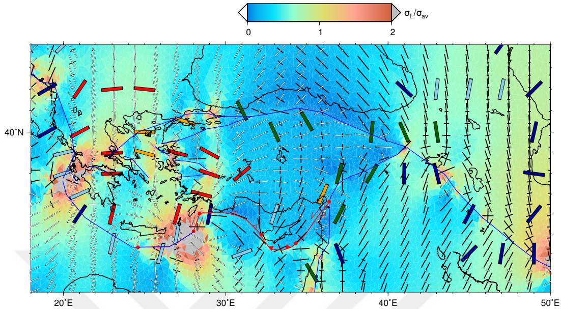
Figure 3.7: Stress field for model SOUTH-6. Black and white arrows indicate principal axis directions of horizontal compression and tension, respectively. Color contours indicate effective shear stresses (normalized by the average effective shear stress). Wide bars represent average WSM directions of maximum horizontal compression, with their color indicating the stress regime: dark blue for thrusting, light blue for oblique thrusting, green for strike-slip, orange for oblique tension, and red for tension (Figure 3.2).
