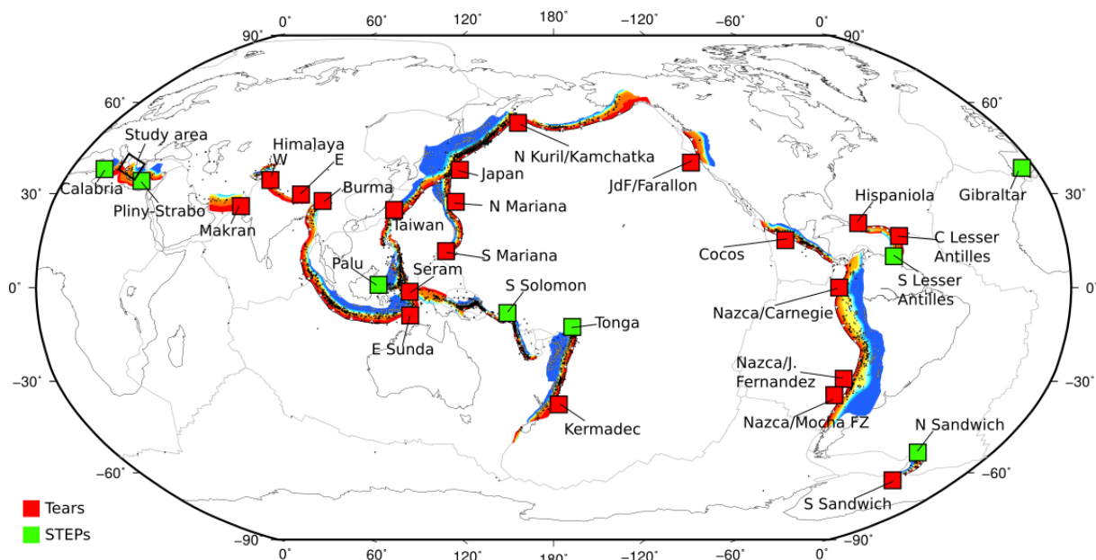
Figure 4.1: Global overview of slabs with a vertical tear or a lateral edge that are associated with a STEP fault in the overriding plate (“STEPs”), or not (“Tears”). Slab depth contours (Hayes et al. , 2018) are shown in colors, along with plate boundaries from (Bird, 2003) and the intermediate – deep focus earthquake epicenters from the ISC Catalogue (2019) (Weston et al. , 2018; Lentas et al. , 2019)
