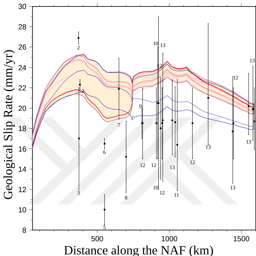
Figure 3.9: Comparison of geological slip-rates on the North Anatolian Fault (NAF) zone with fault slip-rates from our models. For location see shaded relief map in Figure 3.8a. Model slip-rates of SOUTH (orange shaded band) and NORTH (blue hatched band), with individual model slip-rate results shown by red and blue lines, respectively. Thick red line represents our best model (SOUTH-6). Model slip-rates are calculated for the northern branch of the NAF, whose geometry is given nearly parallel to the plot axis shown in Figure 3.8a. Observed slip-rates with error bars are labeled by numbers (Table 3.1)
