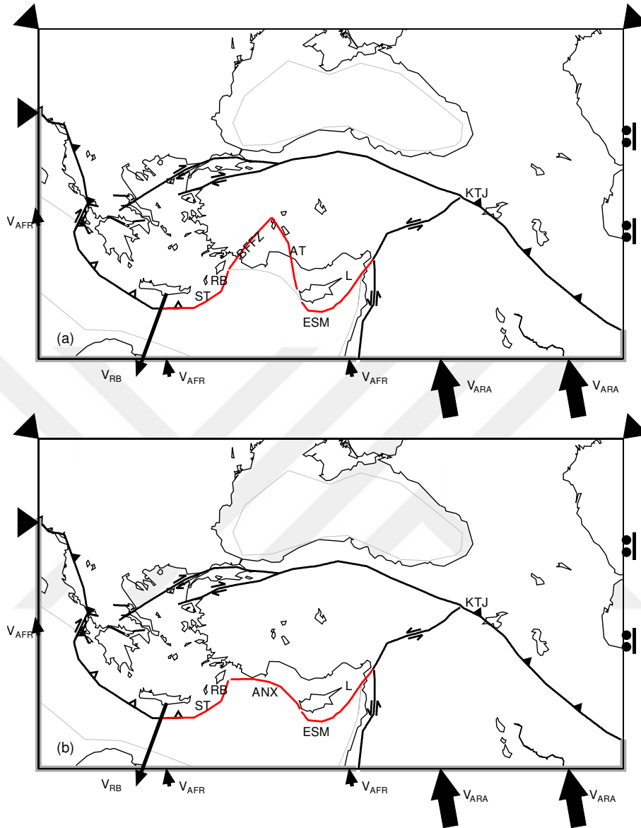
Figure 3.3: Model domain, boundary conditions, and known and unknown faults for (a) NORTH and (b) SOUTH model. Known faults are colored black with their sense of slip. Unknown faults are shown in red. The shaded region indicates oceanic lithosphere. GPS-derived velocities are imposed along the African and Arabian margins of the model (thick gray line along the plot frame): v_{AFR} and v_{ARA} . v_{RB} is the imposed differential velocity on the plate contact of the Hellenic subduction zone. Rollers on the east boundary correspond to the observation that GPS velocities are oriented approximately north-south here. Solid triangles along the north and NW boundary of the model indicate that here the model is fixed. Abbreviations are the same as in Figure 3.1.
