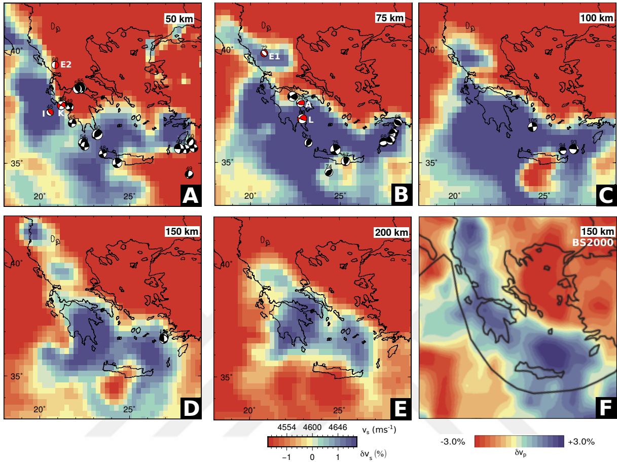
Figure 4.5: (A-E) Horizontal section at 50, 75, 100, 150 and 200 km through the isotropic S-wave velocity ( v_s ) volume. The color scale indicates perturbations from 4600 \text{ m s}^{-1} in percent (below). Above the color scale there are the corresponding absolute S-wave velocities (F) Relative P-wave velocities v_p from Bijwaard and Spakman (2000) for the same region. Please refer to Figure 4.A.1 for the same cross sections with an unsaturated color scale.
