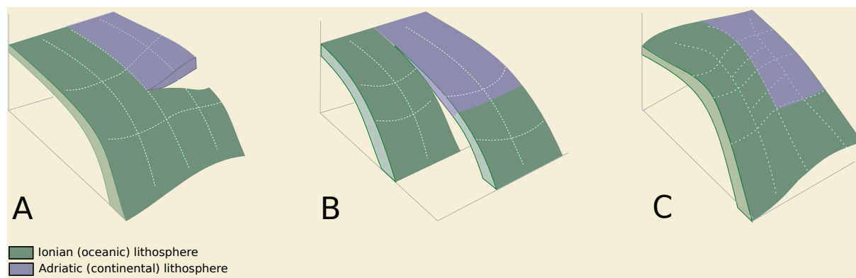
Figure 4.4: Previous interpretations of the geometry of the western Hellenic subduction zone. A. Slab detachment (horizontal tear) model (Wortel and Spakman, 2000); B. STEP (vertical slab tear) model (Govers and Wortel, 2005); C. Smooth ramp model (Pearce et al. , 2012).
