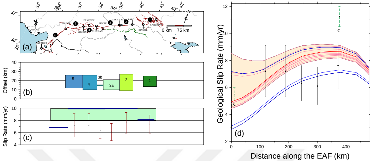
Figure 3.10: a) East Anatolian Fault from Karlıova to Antakya (Herece, 2008). Line segments in red show the EAF and green shows Bitlis suture zone. Major rivers in the region are shown in gray. Numbers indicate fault segments: 1. Karlıova - Bingöl, 2. Palu - Lake Hazar, 3. Sincik - Çelikhan, 4. Çelikhan - Gölbaşı, 5. Gölbaşı - Türkoğlu, 6. Türkoğlu - Antakya. b) Measured offsets on the fault, which are tabulated in Table 3.2. Boxes indicate the minimum and maximum estimates. c) Black points with error bars refer to slip-rates obtained from paleoseismology studies listed in Table 3.2. C: (Çetin et al. , 2003); S: Seyrek et al. (2007) and Karabacak et al. (2010). Red points with error bars are the long-term slip-rates of the EAF, calculated from Table 3.2. Light green box indicates the rate determined from the Eurasia-Anatolia Euler pole (McClusky et al. , 2000). Discrete line segments are fault parallel slip-rates determined by mechanical models. Dark blue denotes Flerit et al. (2004), whereas Reilinger et al. (2006) slightly overlies the central segment of Flerit et al. (2004) for the whole EAF. Continuous red line with blue circles shows our slip-rate model results. d) Comparison of geological slip-rates on the East Anatolian Fault (EAF) zone with fault slip-rates from our models. For location see Figure 3.10(a). Model slip rates of SOUTH (orange shaded band) and NORTH (blue hachured band), with individual model slip rate results shown in red and blue lines, respectively. Thick red line represents our best model (SOUTH-6).
