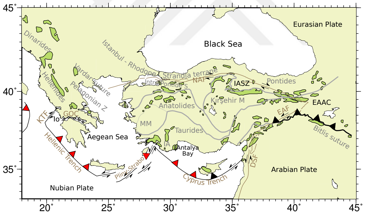
Figure 1.2: Tectonic setting of the eastern Mediterranean region. Abbreviations, DSF: Dead Sea Fault, EAAC: East Anatolian Accretionary Complex, EAF: East Anatolian Fault, GOC: Gulf of Corinth, IA: Isparta Angle, IASZ: Izmir Ankara Suture Zone, MM: Menderes Massif, NAF: North Anatolian Fault; KTF: Kefalonia Transform Fault; Io: Ionian Islands.
