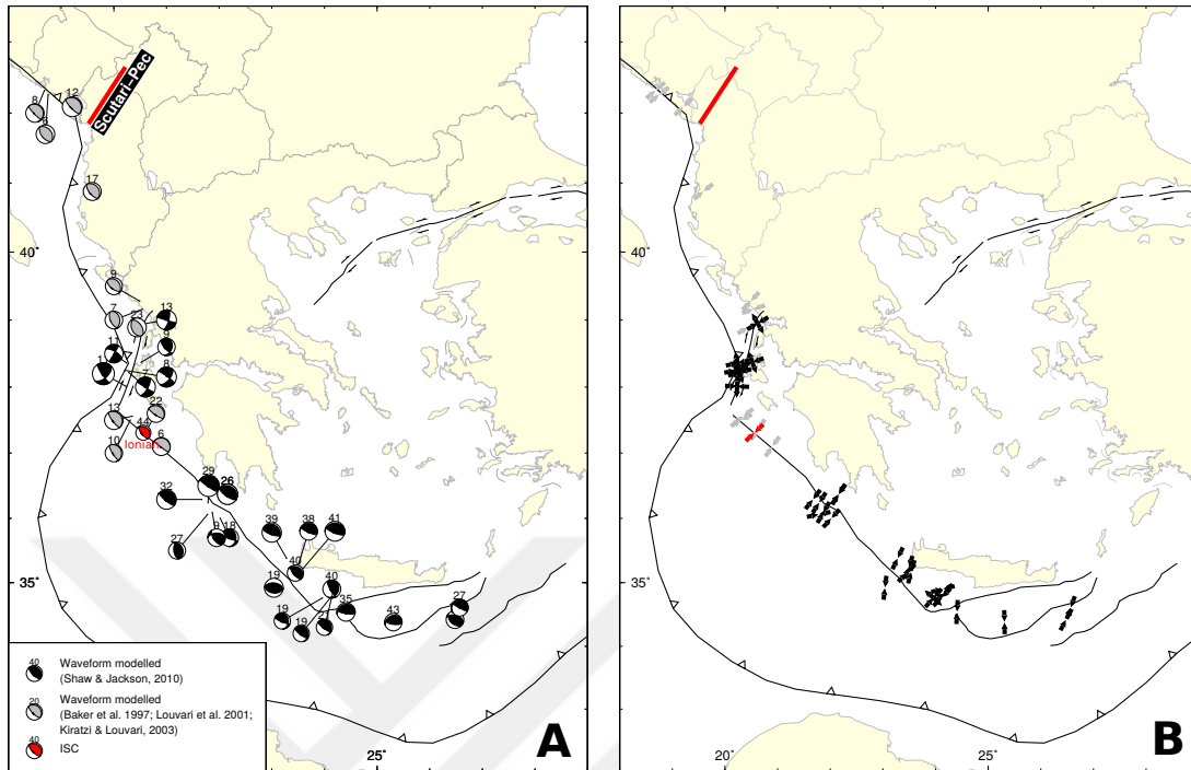
Figure 4.9: A synthesis of plate contact (interface) earthquakes in the larger Hellenic subduction zone. A. focal mechanisms, B. their P- and T-axes of focal mechanisms. Number above beach-balls indicates centroid depths.
