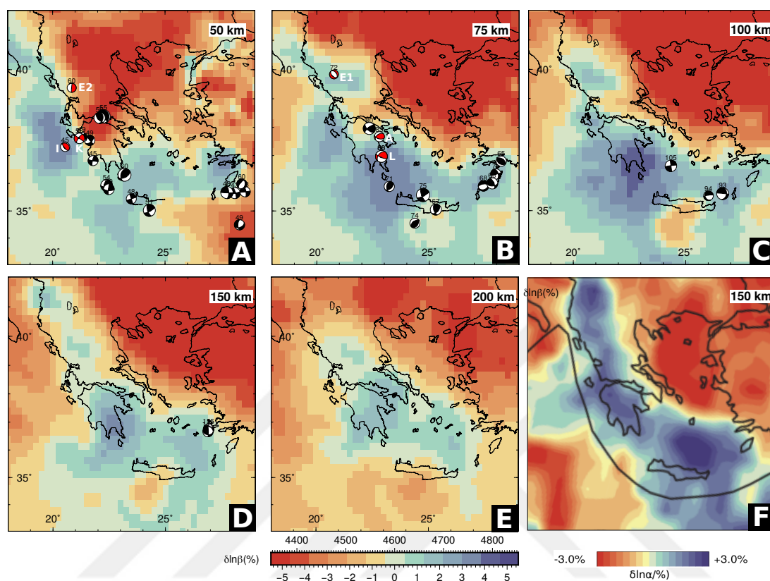
Figure A.1: Figure 4.S1. Figure equivalent to Fig. 4.5, i.e., horizontal cross sections through the tomographic volume, now with an unsaturated color scale.
