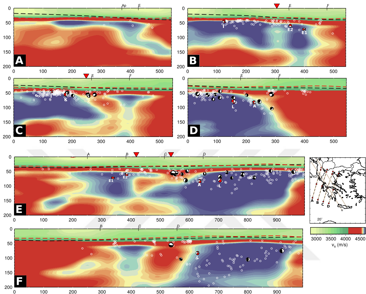
Figure 4.7: Vertical cross sections along the present-day rollback direction of the trench (Sections A-D), and in a direction that is approximately parallel to the Western Hellenic Subduction Zone (Sections E-F). The map panel shows where the cross sections are taken, and red and white circles on the cross section lines indicate 250 km intervals. On cross sections (A-F), red inverted triangles are used to indicate surface locations of the KTF and the Gulf of Corinth. Letters on top of the vertical cross sections refer to the labels of intersecting profiles. White open circles represent M > 4 events, taken from the ISC, that have hypocenter errors (both vertical and horizontal) \leq 10 km. Hypocenters within a swath of 50 km are projected onto the profiles. Red and black dashed lines show the crustal thickness variations from CRUST1.0 (Laske et al. , 2013) and (Karabulut et al. , 2019) respectively. Please refer to Figure 4.A.3 for the same cross sections with an unsaturated color scale.
