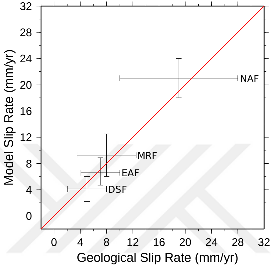
Figure 3.11: Spatially averaged geological slip rates vs. slip rates of best model SOUTH-6 for the Dead Sea Fault (DSF), East Anatolian Fault (EAF), Zagros Main Recent Fault (MRF), and North Anatolian Fault (NAF).
