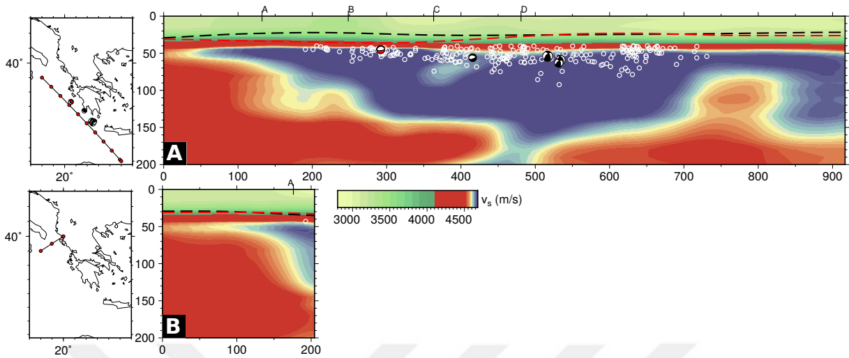
Figure 4.6: Vertical cross-sections through our S-velocity volume A . Ionian lithosphere and asthenosphere, NW left, SE right. B . Apulian escarpment, SW left, NE right. Letters on top of the panels indicate intersecting profiles from Figure 4.7. Red and black dashed lines show the crustal thickness variations from CRUST1.0 (Laske et al. , 2013) and Karabulut et al. (2019) respectively. Open circles and focal mechanisms represent epicenters of earthquakes within a horizontal perpendicular distance of 25 km of the cross section. Please refer to Figure 4.A.2 for the same cross sections with an unsaturated color scale.
