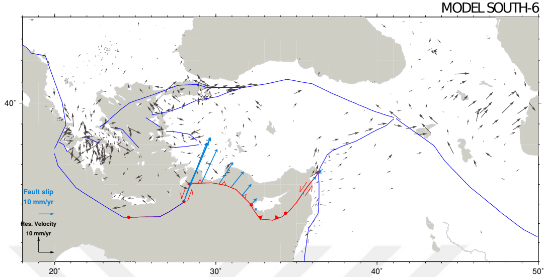
Figure 3.5: Velocity misfits (observed minus calculated) for model SOUTH-6. Symbols show the assumed nature of the faults; filled triangles indicate that only fault-perpendicular motion is allowed, strike-slip symbols indicate that only fault parallel motion is allowed. Open triangles indicate that both strike-slip and fault normal motions are allowed in the model. Blue arrows indicate the resulting fault slip-rate and direction.
