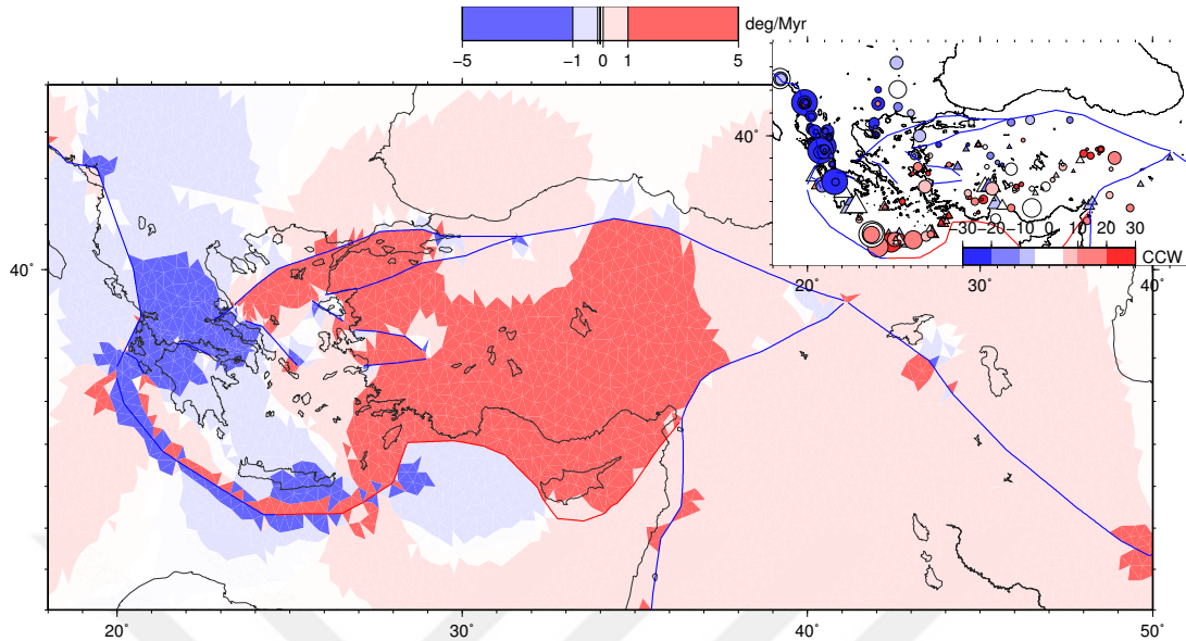
Figure 3.12: Vertical axis rotations predicted by model SOUTH-6. The color scale shows the vertical axis rotations in degrees per Myr. Blue and red colors indicate clockwise and counter-clockwise motions, respectively. Inset: Paleomagnetic rotation data (see the main text for references). Circles show pre-Pliocene sampling sites and triangles represent Oligocene and Miocene sample sites. Diameter of symbols are scaled with \alpha_{95} value (larger symbol indicates a more reliable measurement).
