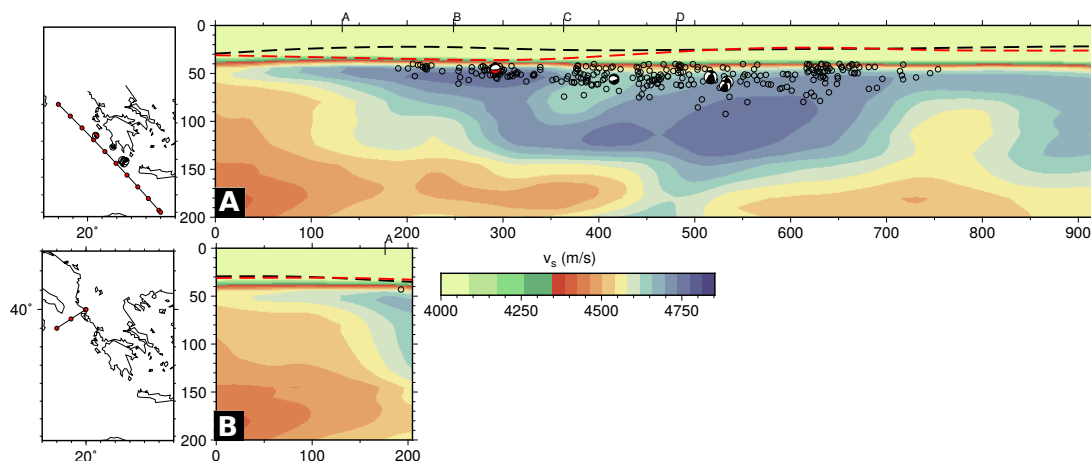
Figure A.2: Figure equivalent to Fig. 4.6, i.e., vertical cross sections through the tomographic volume, now with an unsaturated color scale.
