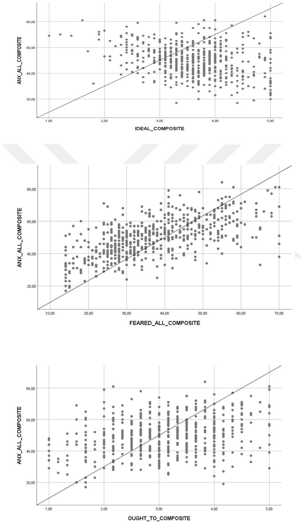
Scatterplots for Linear Relationships of FLPA, ILPS, FLPS, and OLPS
