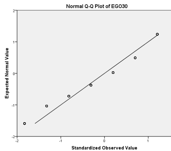
Normal Q-Q Plot for Self-worth concerns
