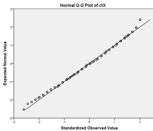
Normal Q-Q Plot for Test Anxiety
