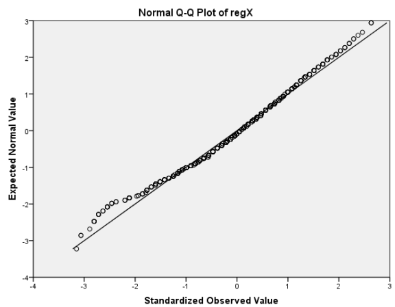
Normal Q-Q Plot for Meta-cognitive Self-regulation
