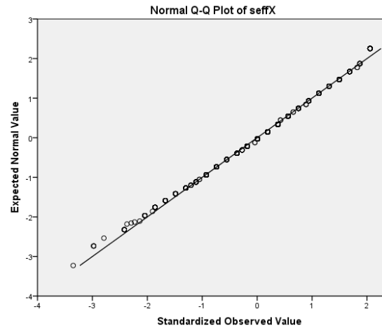
Normal Q-Q Plot for Self-efficacy
