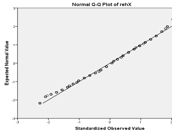
Normal Q-Q Plot for Meta-cognitive Self-regulation
