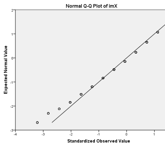
Normal Q-Q Plot for Intrinsic Motivation
