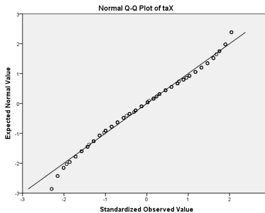
Normal Q-Q Plot for Test Anxiety
