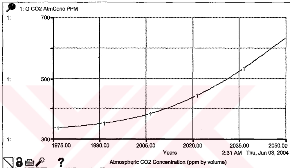
Figure 9.9. Atmospheric CO 2 concentration in “optimistic non-renewable energy reserves” scenario
