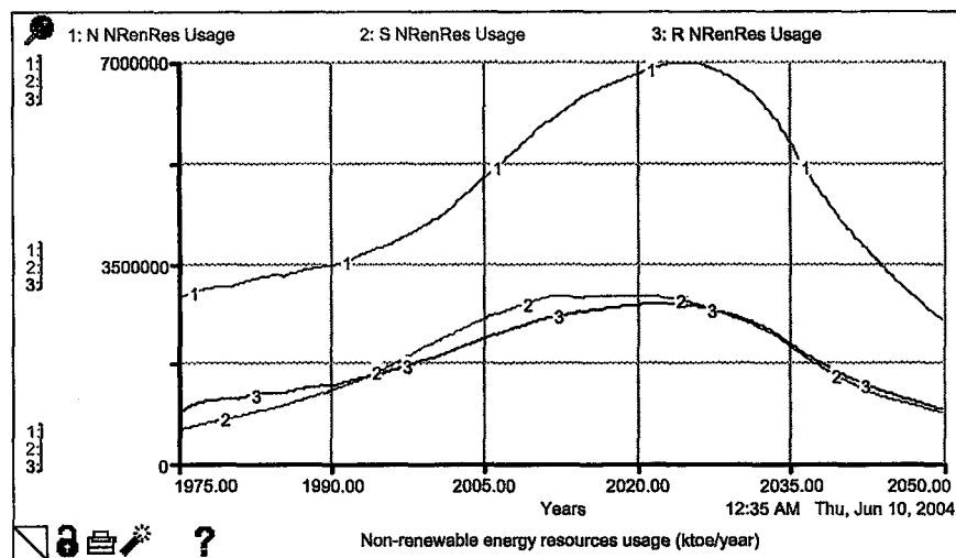
Figure 10.11. Non-renewable resource usage with “North supported energy transition in South” policy
