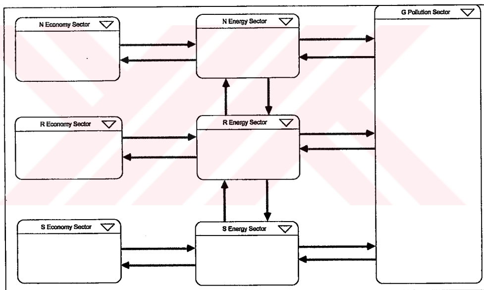
Figure 6.25. Interrelationships between energy-related sectors
