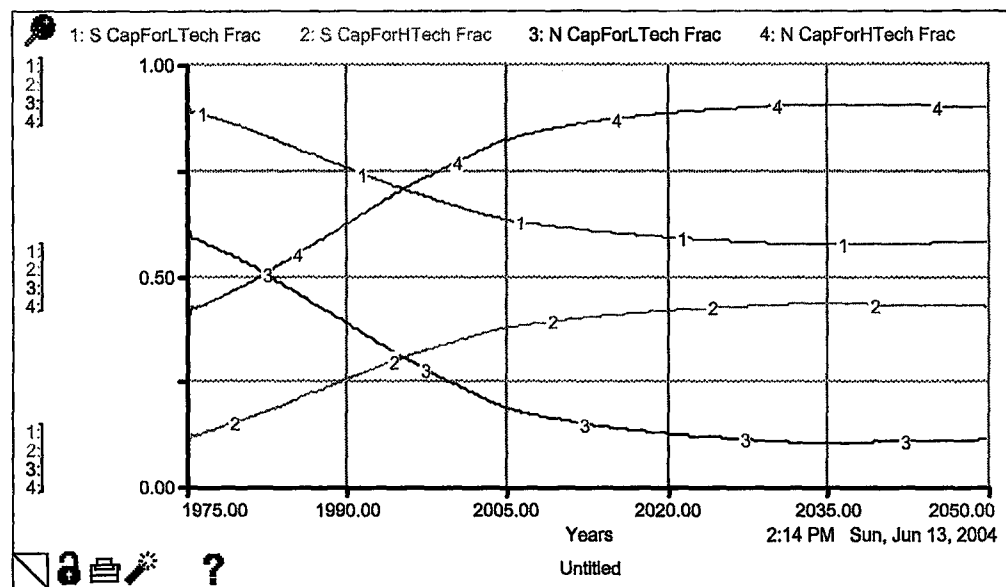
Figure 6.64. Fraction of capital allocated to the two sectors in isolated sector run
