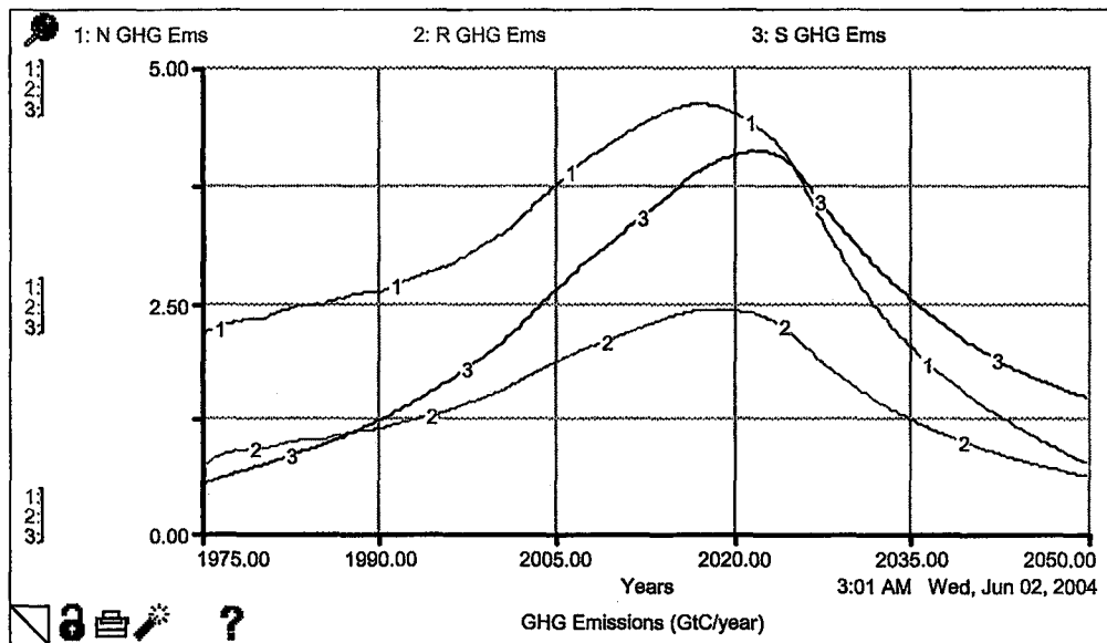
Figure 8.15. CO 2 emission rates for all three blocks
