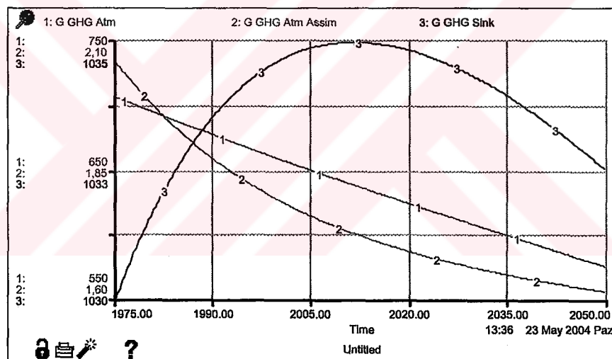
Figure 7.22. Behavior of CO 2 accumulation in atmospheric and oceanic sinks with constant global emission rate of 0 GtC/year
