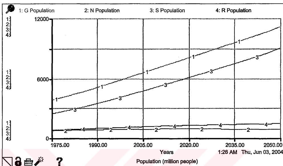
Figure 9.1. Behavior of global population with ineffective fertility control at South
