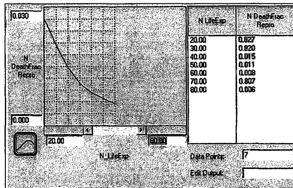
Figure 6.7. Death fraction of reproductive population as a function of life expectancy (North)
