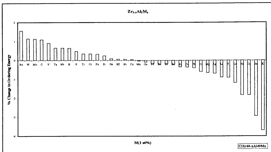
Figure B.37. % Change in ordering energy of Zr_{60}Al_{40} binary system for the addition of 1 at % impurity elements (M) when 1 at % is taken from Zr ( Zr_{0.59}Al_{0.40}M_{0.01} system).
