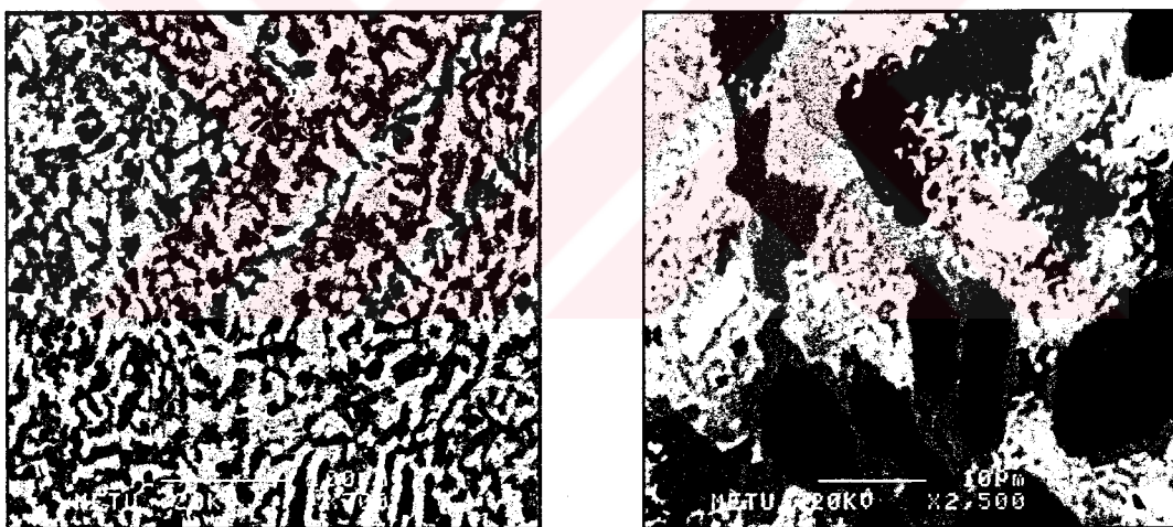
Figure 4.70. SEM images of near-equilibrium \text{Zr}_{50}\text{Ni}_{20}\text{Al}_{15}\text{Mo}_{10}\text{W}_5 alloy:
