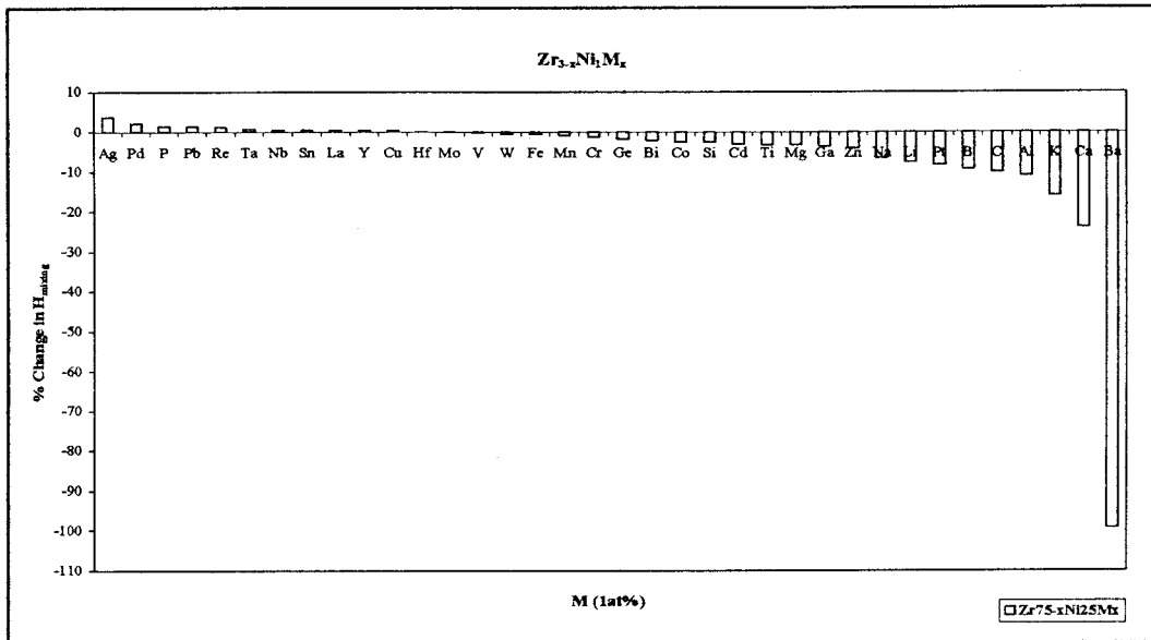
Figure B.21. % Change in \Delta H_{mixing} of Zr_{75}Ni_{25} intermetallic for the addition of 1 at % impurity elements (M) when 1 at % is taken from Zr ( Zr_{0.74}Ni_{0.25}M_{0.01} system).
