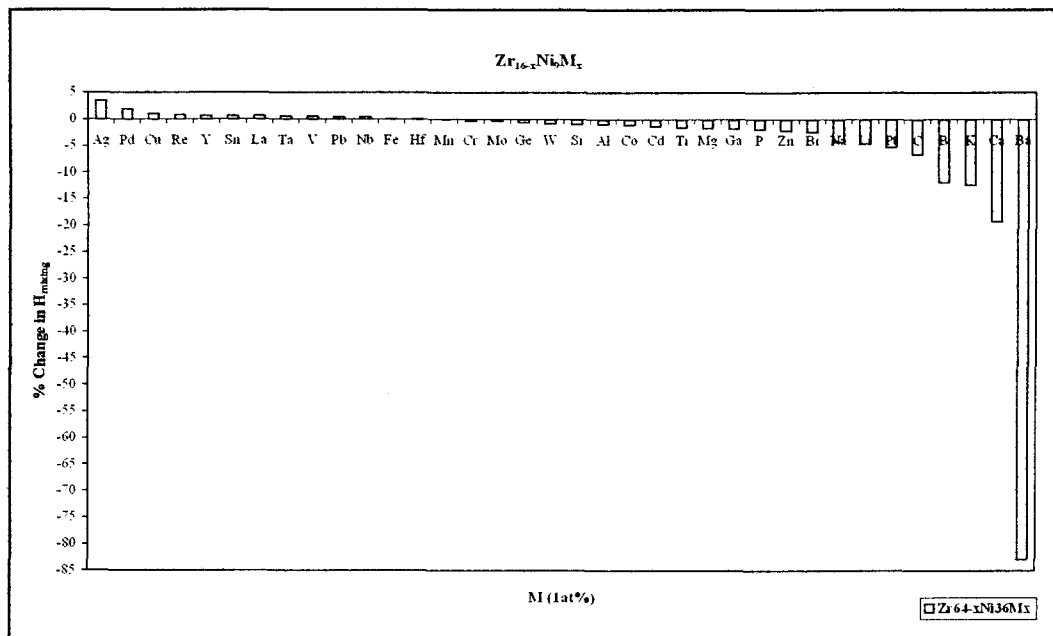
Figure B.9. % Change in \Delta H_{mixing} of Zr_{64}Ni_{36} binary system for the addition of 1 at % impurity elements (M) when 1 at % is taken from Zr ( Zr_{0.63}Ni_{0.36}Mo_{0.01} system).
