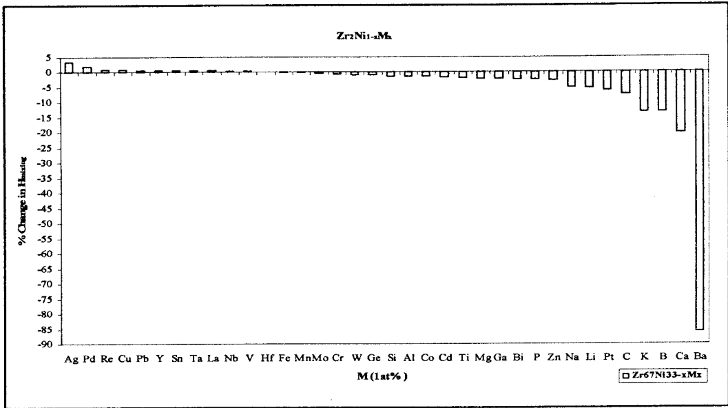
Figure 4.6. % Change in \Delta H_{\text{mixing}} of Zr 67 Ni 33 intermetallic for the addition of 1 at % impurity elements (M) when 1 at % is taken from Ni (Zr 0,67 Ni 0,32 M 0,01 system).
