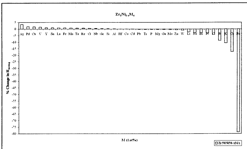
Figure B.5. % Change in \Delta H_{mixing} of Zr_{50}Ni_{50} binary system for the addition of 1 at % impurity elements (M) when 1 at % is taken from Ni ( Zr_{0.50}Ni_{0.49}M_{0.01} system).
