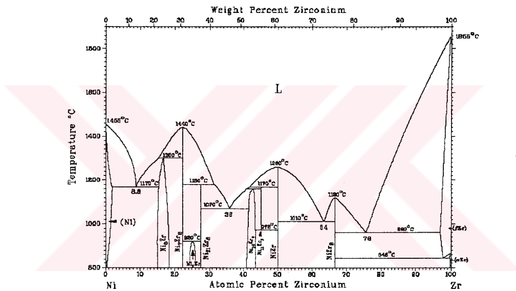
Figure A.1. The equilibrium phase diagram for Zr-Ni binary alloys
