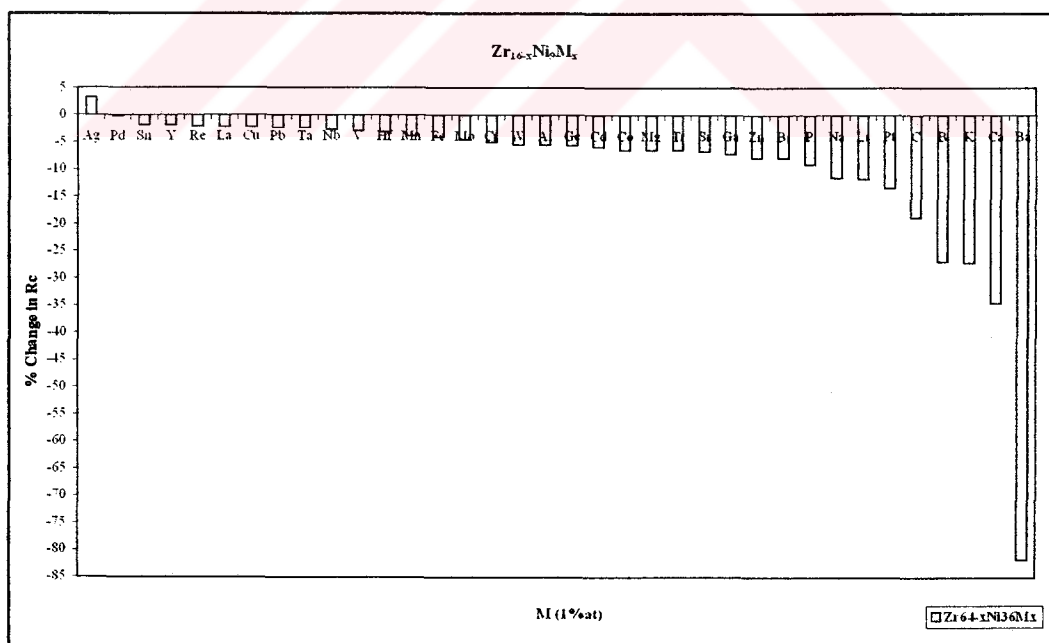
Figure B.10. % Change in R_c of Zr_{64}Ni_{36} binary system for the addition of 1 at % impurity elements (M) when 1 at % is taken from Zr ( Zr_{0.63}Ni_{0.36}Mo_{0.01} system).
