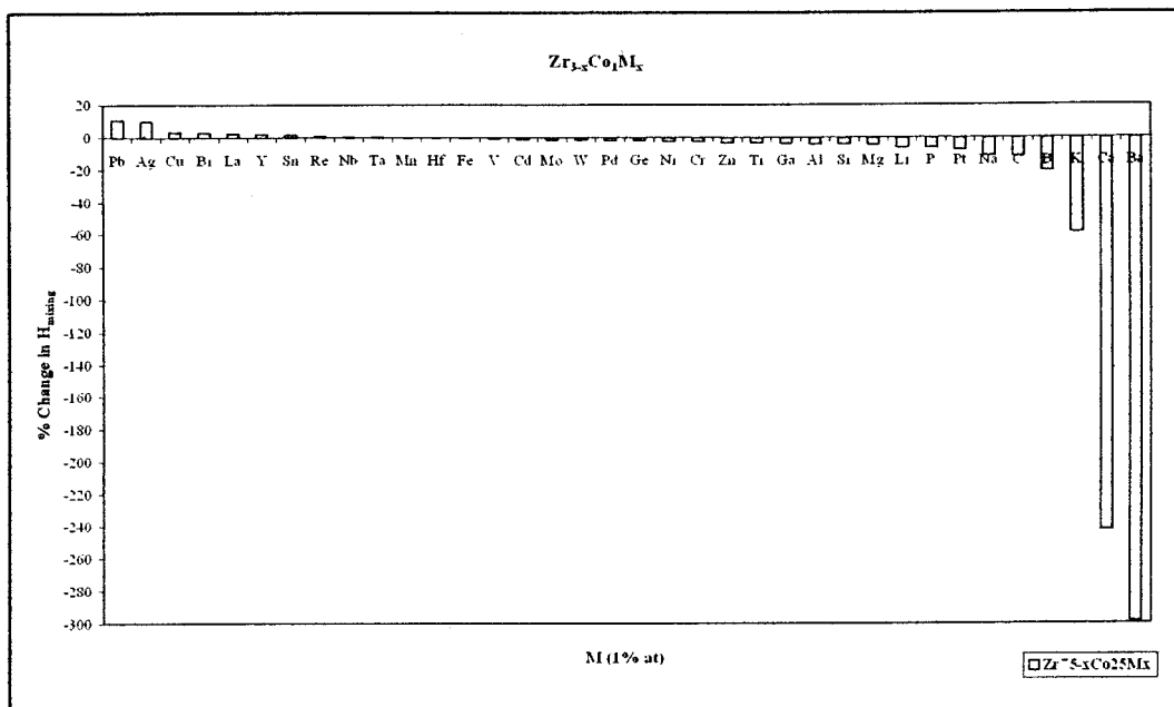
Figure B.33. % Change in \Delta H_{mixing} of Zr_{75}Co_{25} binary system for the addition of 1 at % impurity elements (M) when 1 at % is taken from Zr ( Zr_{0.74}Co_{0.25}M_{0.01} system).
