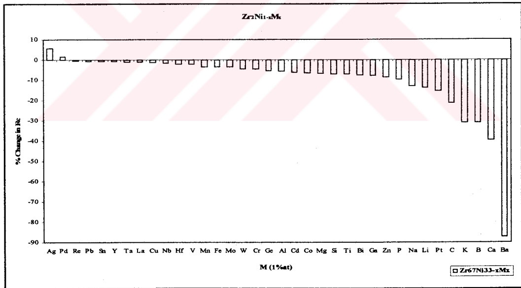
Figure 4.7. % Change in R_c of Zr 67 Ni 33 intermetallic for the addition of 1 at % impurity elements (M) when 1 at % is taken from Ni (Zr 0,67 Ni 0,32 M 0,01 system).
