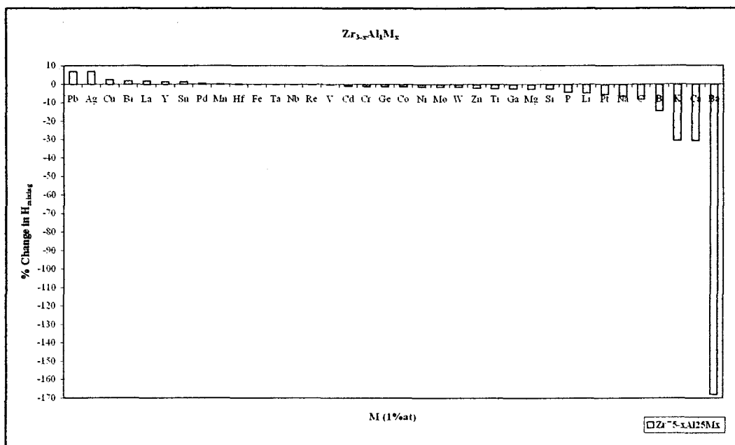
Figure B.45. % Change in \Delta H_{mixing} of Zr_{75}Al_{25} binary system for the addition of 1 at % impurity elements (M) when 1 at % is taken from Zr ( Zr_{0.74}Al_{0.25}M_{0.01} system).
