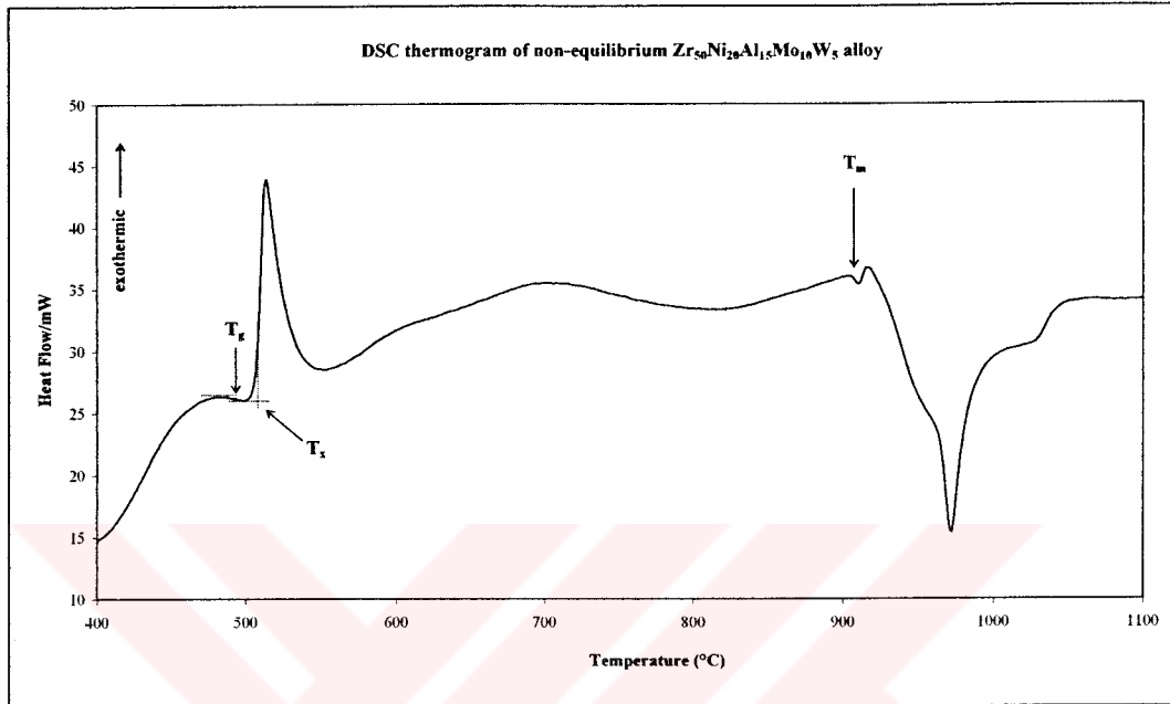
Figure 4.72. Isochronal DSC thermogram of the non-equilibrium \text{Zr}_{50}\text{Ni}_{20}\text{Al}_{15}\text{Mo}_{10}\text{W}_5 alloy.
