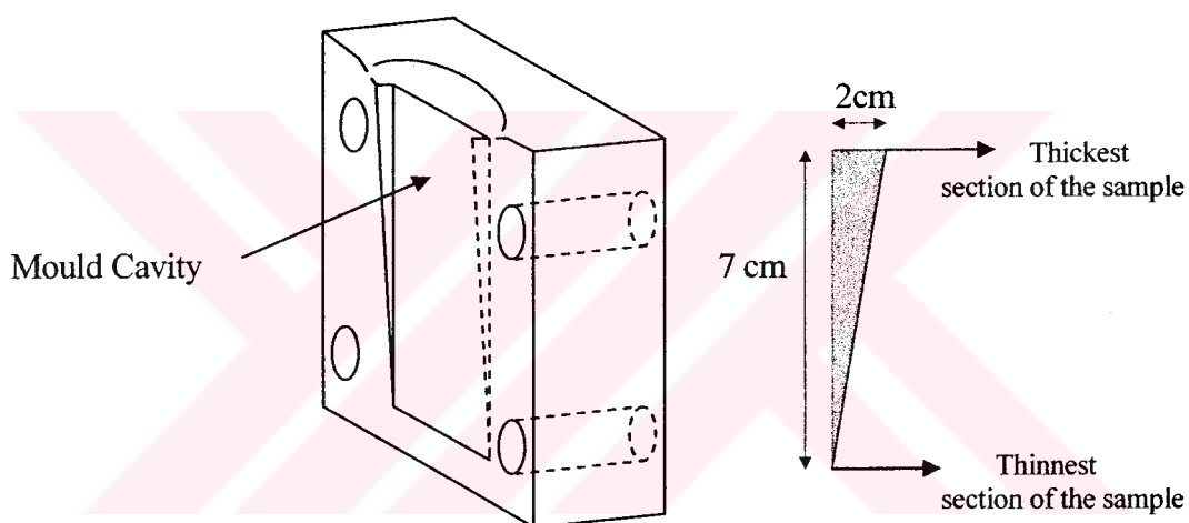
Figure 3.4. Schematic view of the half of the wedge-shaped copper mould and the dimensions of the cast sample.
