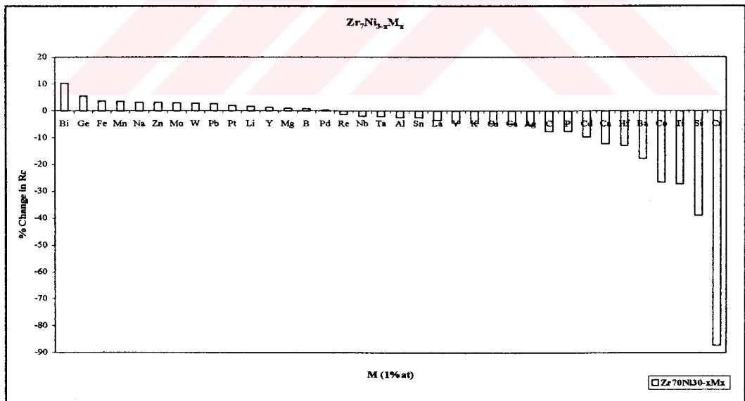
Figure B.18. % Change in R_c of Zr_{70}Ni_{30} intermetallic for the addition of 1 at % impurity elements (M) when 1 at % is taken from Ni ( Zr_{0,70}Ni_{0,29}M_{0,01} system).
