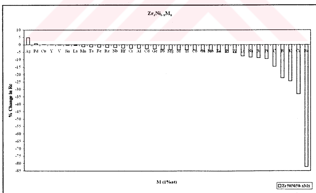
Figure B.6. % Change in R_c of Zr_{50}Ni_{50} binary system for the addition of 1 at % impurity elements (M) when 1 at % is taken from Ni ( Zr_{0.50}Ni_{0.49}M_{0.01} system).
