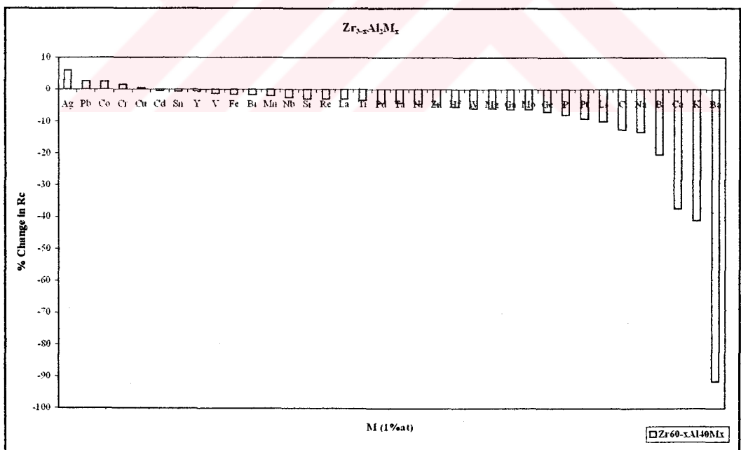
Figure B.40. % Change in R_c of Zr_{60}Al_{40} binary system for the addition of 1 at % impurity elements (M) when 1 at % is taken from Zr ( Zr_{0.59}Al_{0.40}M_{0.01} system).
