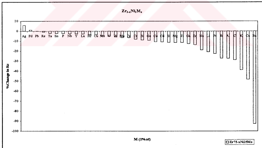
Figure B.22. % Change in R_c of Zr_{75}Ni_{25} intermetallic for the addition of 1 at % impurity elements (M) when 1 at % is taken from Zr ( Zr_{0.74}Ni_{0.25}M_{0.01} system).
