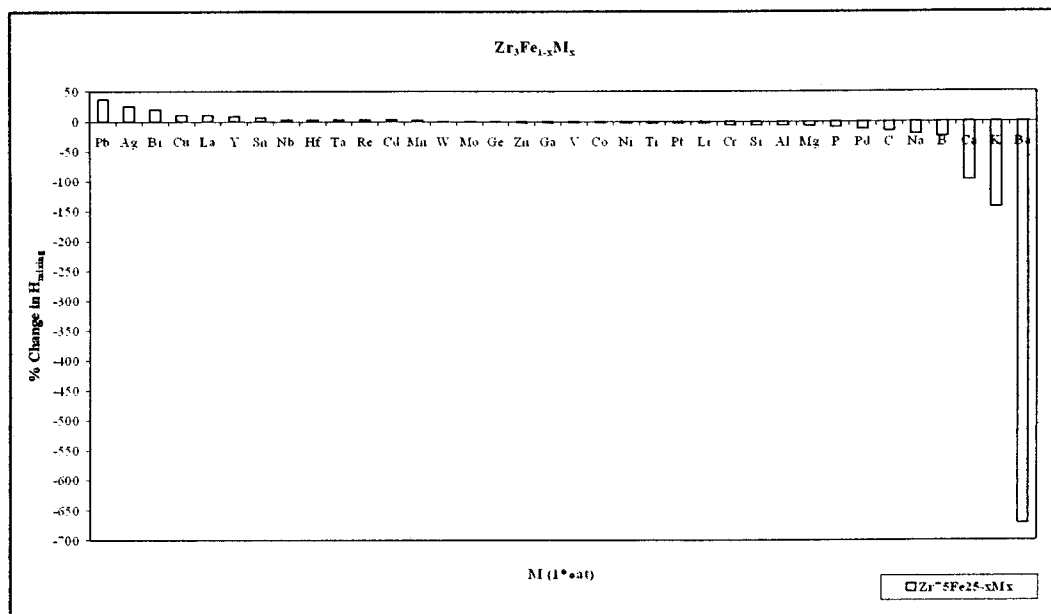
Figure B.29. % Change in \Delta H_{mixing} of Zr_{75}Fe_{25} binary system for the addition of 1 at % impurity elements (M) when 1 at % is taken from Fe ( Zr_{0.75}Fe_{0.24}M_{0.01} system).
