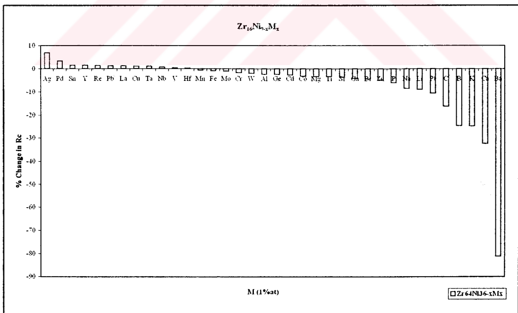
Figure B.12. % Change in R_c of Zr_{64}Ni_{36} binary system for the addition of 1 at % impurity elements (M) when 1 at % is taken from Ni ( Zr_{0.64}Ni_{0.35}M_{0.01} system).
