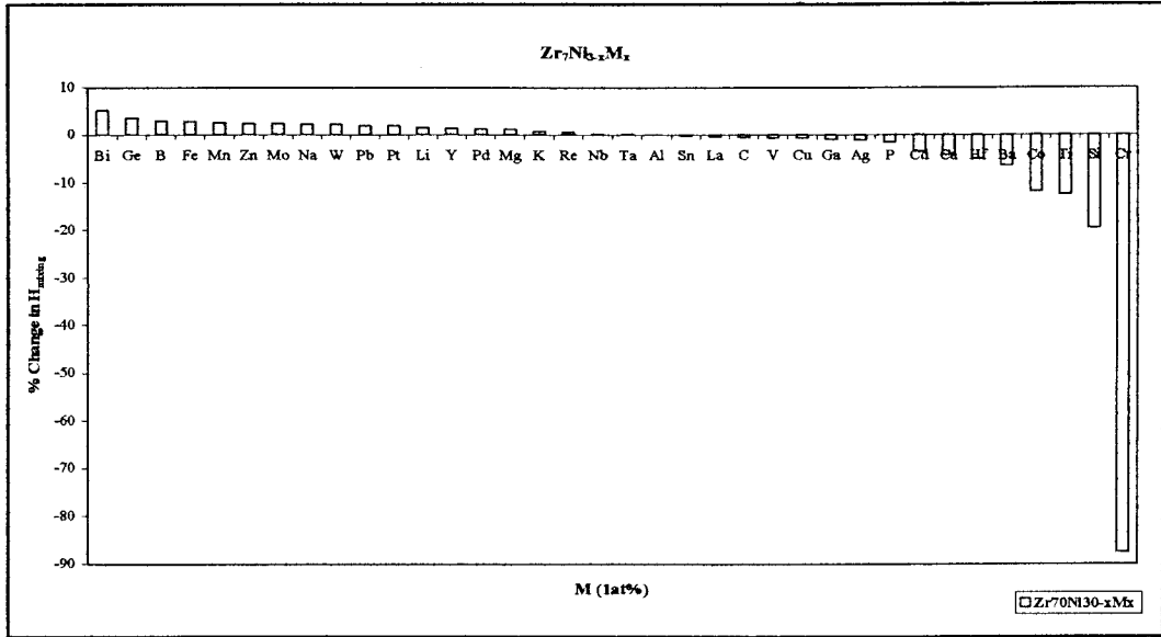
Figure B.17. % Change in \Delta H_{mixing} of Zr_{70}Ni_{30} intermetallic for the addition of 1 at % impurity elements (M) when 1 at % is taken from Ni ( Zr_{0,70}Ni_{0,29}M_{0,01} system).
