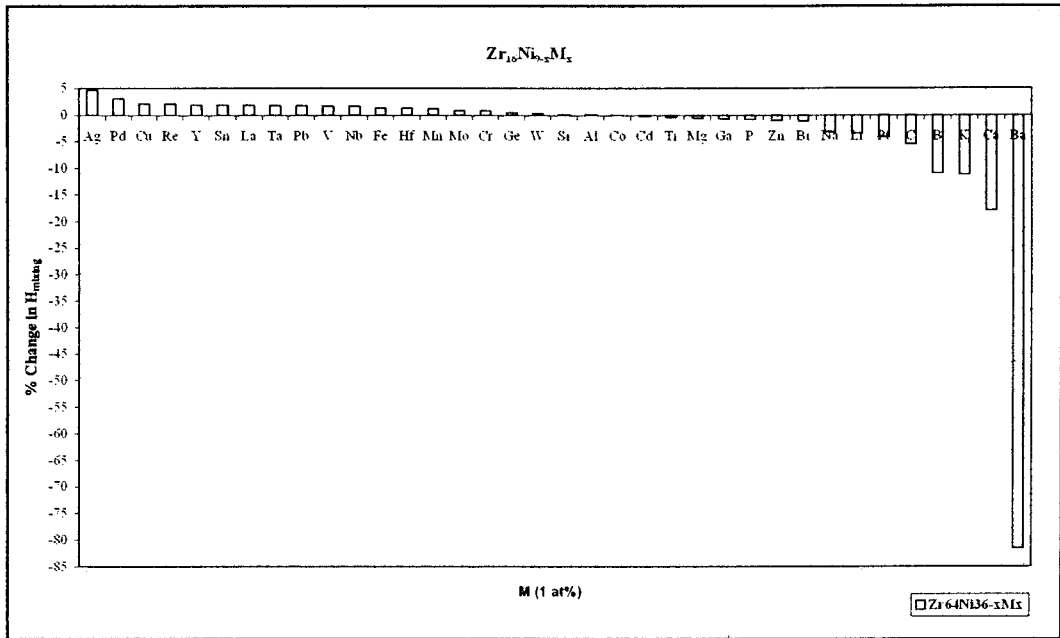
Figure B.11. % Change in \Delta H_{mixing} of Zr_{64}Ni_{36} binary system for the addition of 1 at % impurity elements (M) when 1 at % is taken from Ni ( Zr_{0.64}Ni_{0.35}M_{0.01} system).
