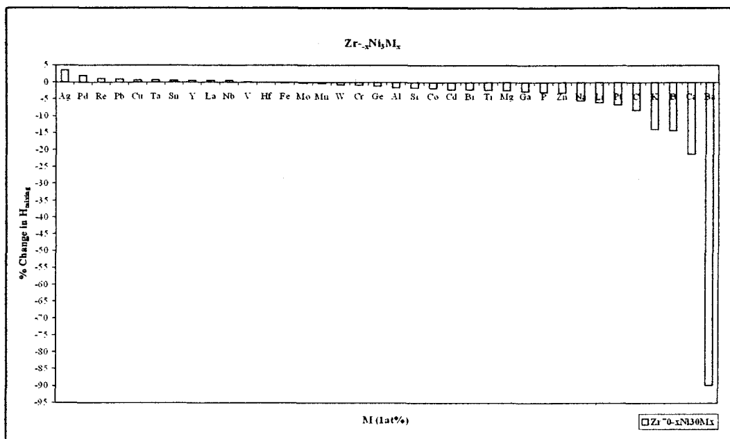
Figure B.15. % Change in \Delta H_{mixing} of Zr_{70}Ni_{30} intermetallic for the addition of 1 at % impurity elements (M) when 1 at % is taken from Zr ( Zr_{0.69}Ni_{0.30}M_{0.01} system).
