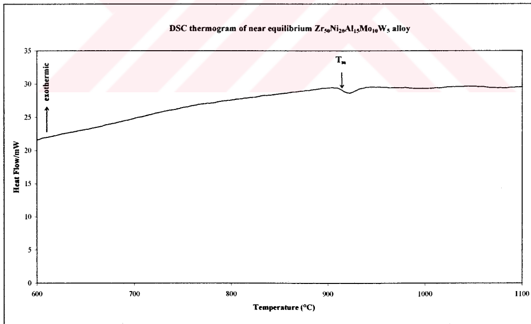
Figure 4.69. Isochronal DSC thermogram of the near-equilibrium \text{Zr}_{50}\text{Ni}_{20}\text{Al}_{15}\text{Mo}_{10}\text{W}_5 alloy.
