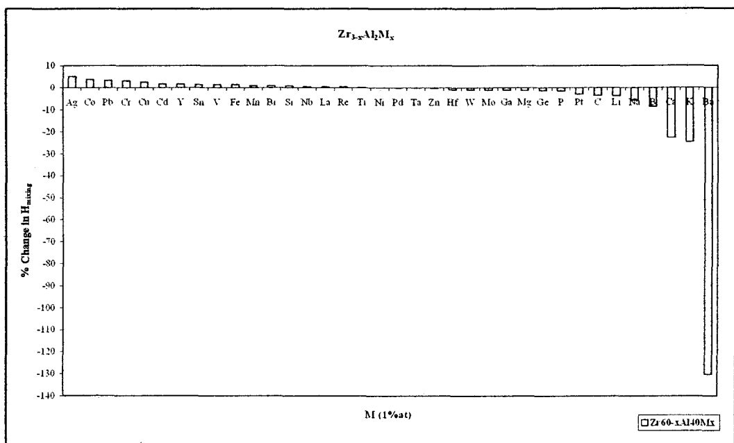
Figure B.39. % Change in \Delta H_{\text{mixing}} of Zr_{60}Al_{40} binary system for the addition of 1 at % impurity elements (M) when 1 at % is taken from Zr ( Zr_{0.59}Al_{0.40}M_{0.01} system).
