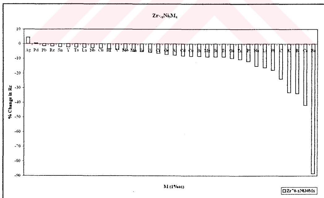
Figure B.16. % Change in R_c of Zr_{70}Ni_{30} intermetallic for the addition of 1 at % impurity elements (M) when 1 at % is taken from Zr ( Zr_{0.69}Ni_{0.30}M_{0.01} system).
