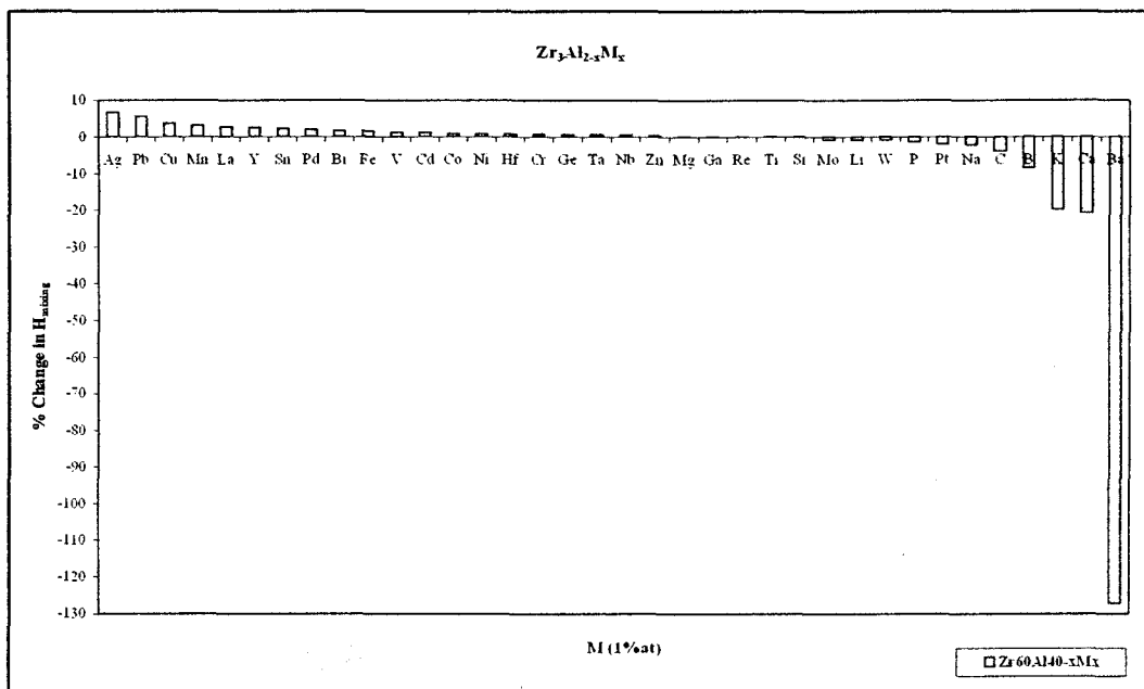
Figure B.41. % Change in \Delta H_{\text{mixing}} of Zr_{60}Al_{40} binary system for the addition of 1 at % impurity elements (M) when 1 at % is taken from Al ( Zr_{0.60}Al_{0.39}M_{0.01} system).
