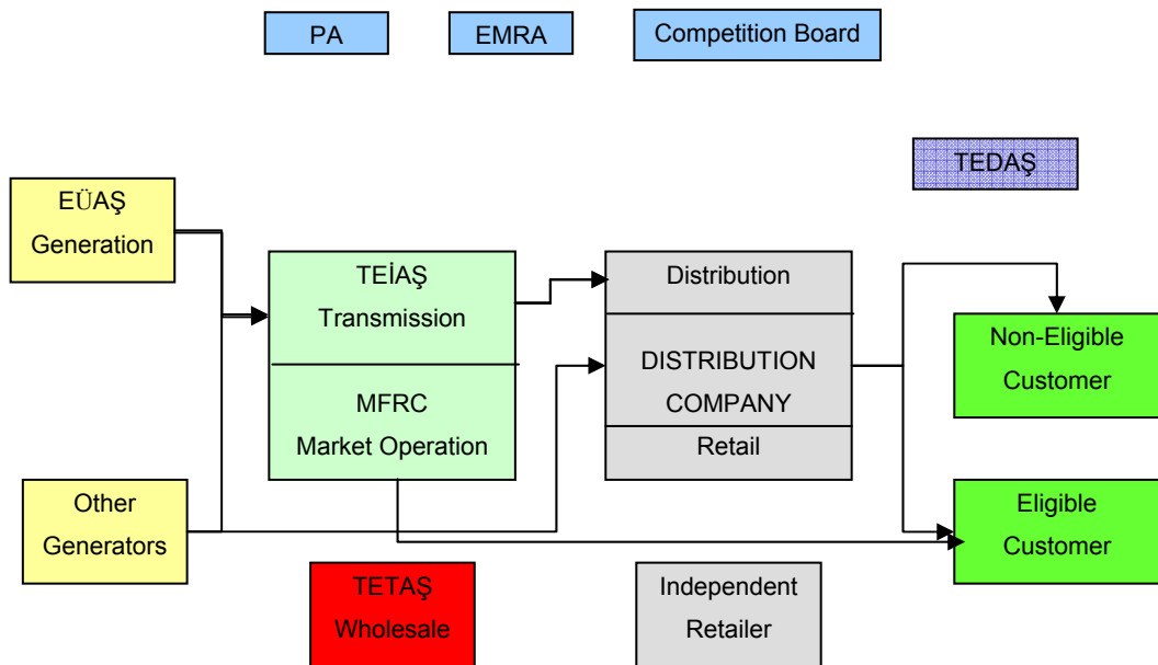
Figure 7. Industry Power Flows and Connections
