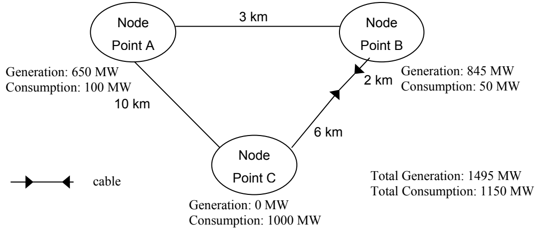
Figure 22. Network with Three Node Points
