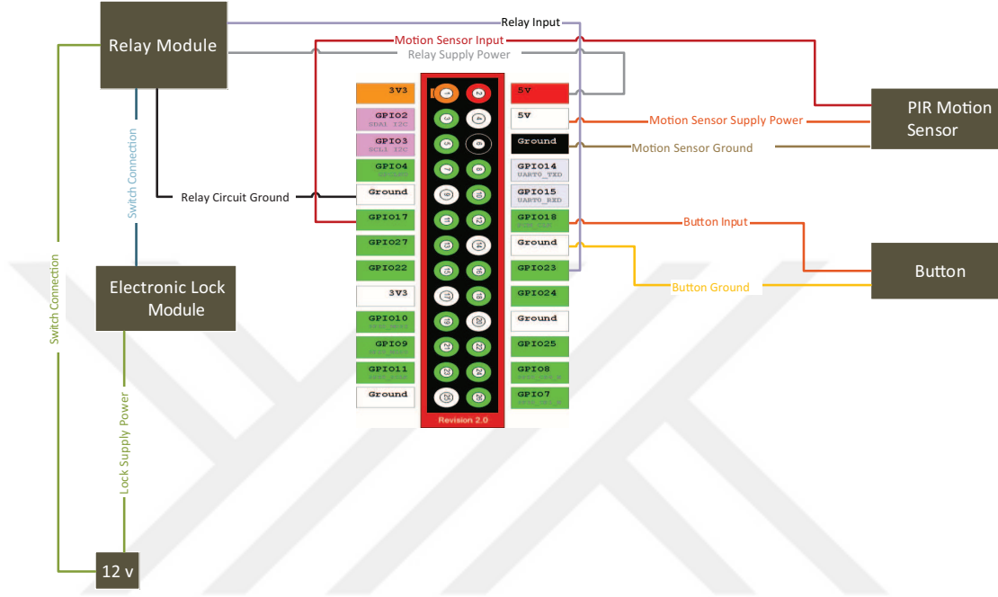
Figure 3.9 : Circuit design of FPFERS.
