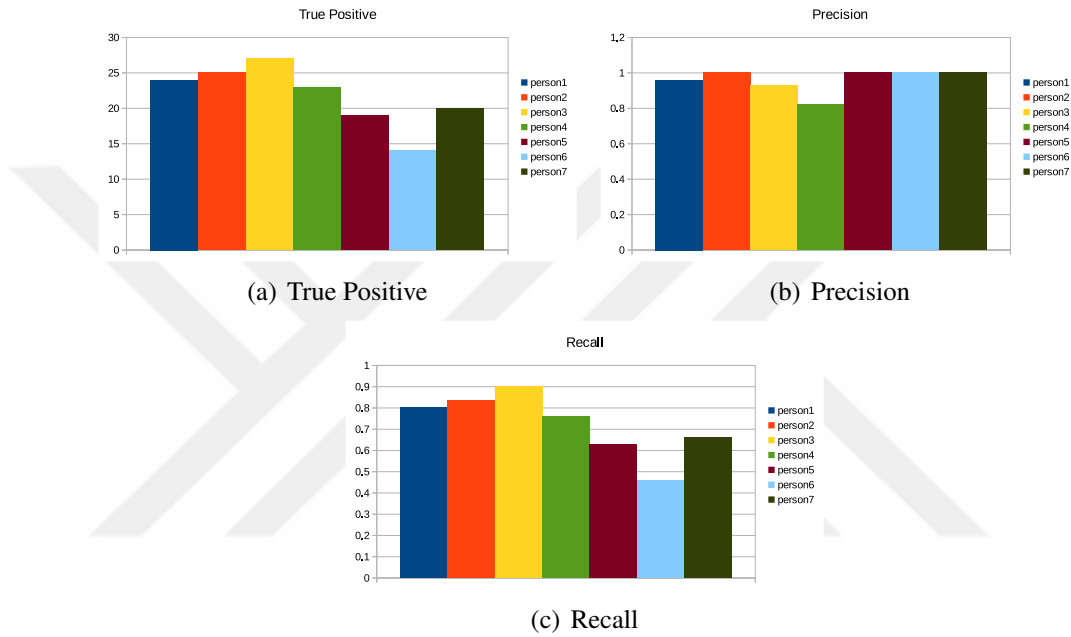
Figure 4.5 : Recognition scores using the mobile robot.
