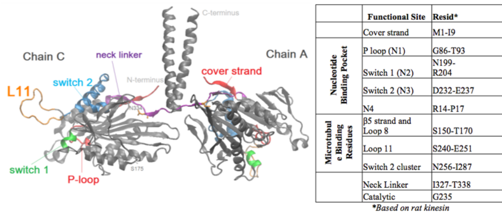
Figure 9.1. Kinesin functional sites are shown on structures.
