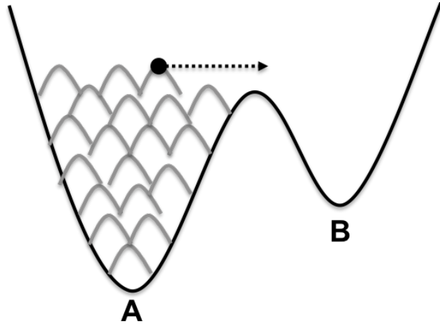
Figure 6.2. Schematic representation of Gaussian functions deposition of the potential energy of the system.
