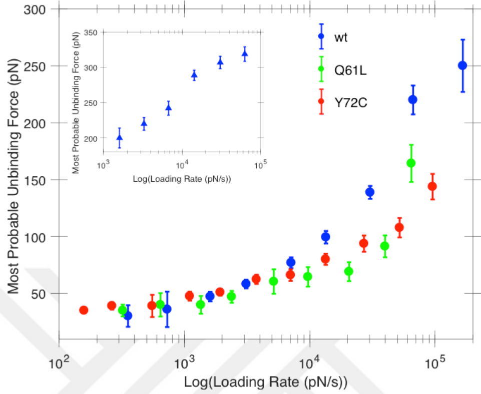
Figure 10.8. Observed Most Probable Rupture Forces Along the Measured Loading Rates.
