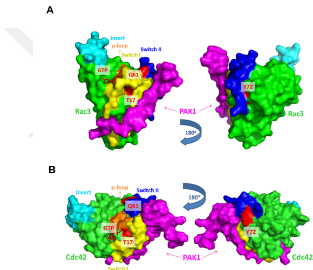
Figure 10.1. Available Structures of Rac1-Like Proteins Bound to PAK1. (A) Rac3 - PAK1 (CRIB Domain) Complex Structure (PDB ID: 2qme). (B) Cdc42 - PAK1 (GTPase Binding Domain) Complex Structure (PDB ID: 1e0a).
