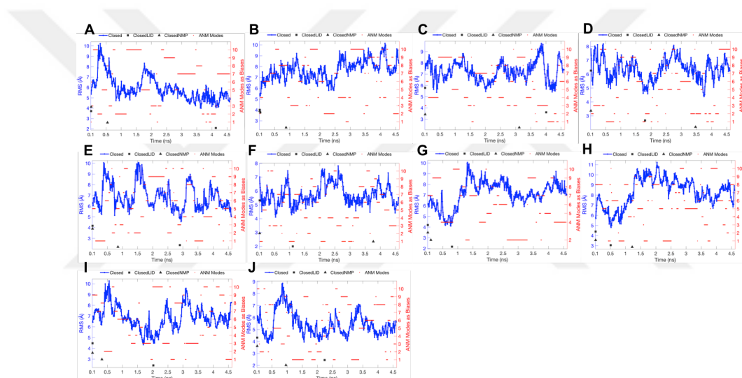
Figure 7.11. RMSD and the biased CV versus simulation time of each replica for apo AdK with non-targeted simulation. Replicas 1 to 10 are given in A to J, respectively.
