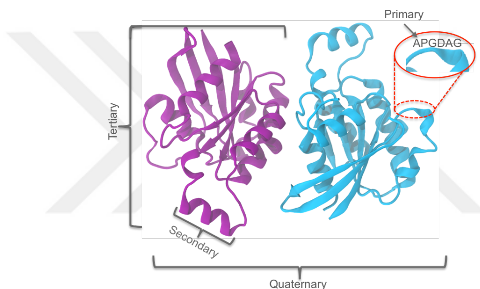
Figure 2.1. The four hierarchical levels of protein structure. The levels are illustrated on the structure of Rac1 dimer protein.
