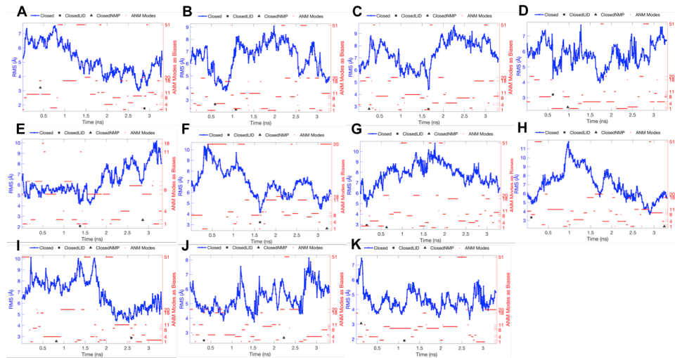
Figure 7.6. RMSD and the biased CV versus simulation time of each replica for wild type-2. Replicas 1 to 11 are given in A to K, respectively.
