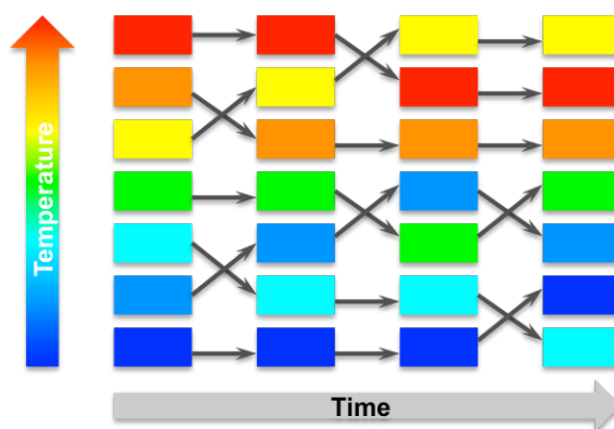
Figure 3.2. Schematic representation of the REMD method. Adapted from [3].
