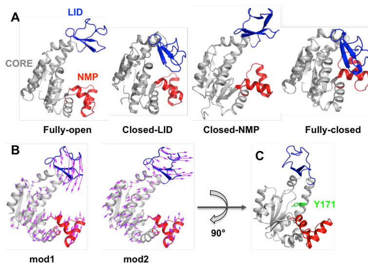
Figure 7.1. Structures and Slowest ANM Modes of AdK. A) Fully-Open (PDB ID: 4AKE), Fully-Closed (PDB ID: 1AKE), Closed-LID (PDB ID: 1DVR) and Closed NMP (PDB ID: 2AK3) Structures of AdK. C) Position of Y171 is Labeled on the Fully-Open Conformation.
