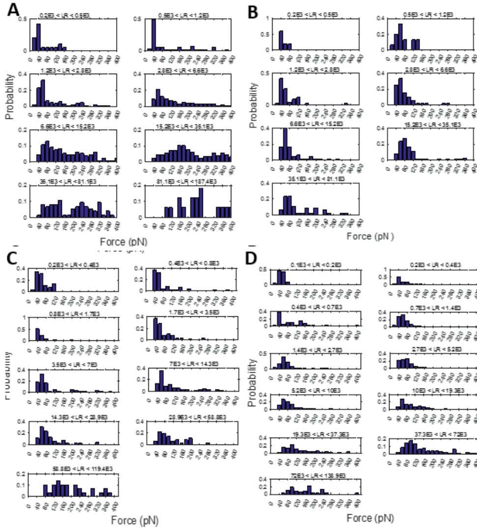
Figure 10.7. Adhesion Force Histograms at Different Loading Rates GTP Loaded Wild-Type T17N, Q61L and Y72C Rac1-PAK1 Complex are Given in A-D, Respectively.
