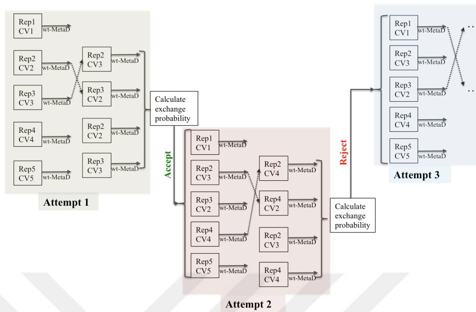
Figure 6.3. Flow Diagram of Bias-Exchange Well-Tempered Metadynamics (wt-MetaD) Scheme. Here, a wt-MetaD Simulations with the Replicas (Rep1, ... Rep5) Each Biased with a CV (CV1, ... CV5) are Illustrated Schematically.
