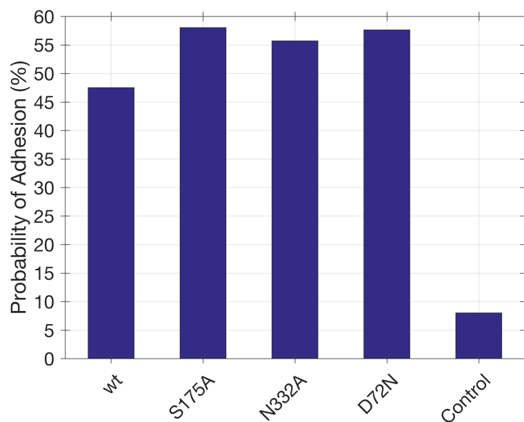
Figure 9.3. Comparison of the Probability of Adhesion of Regular Experiments with the Control Experiment (Functionalized AFM Cantilevers Were Saturated with Excess Tubulin Molecules before the Pulling).
