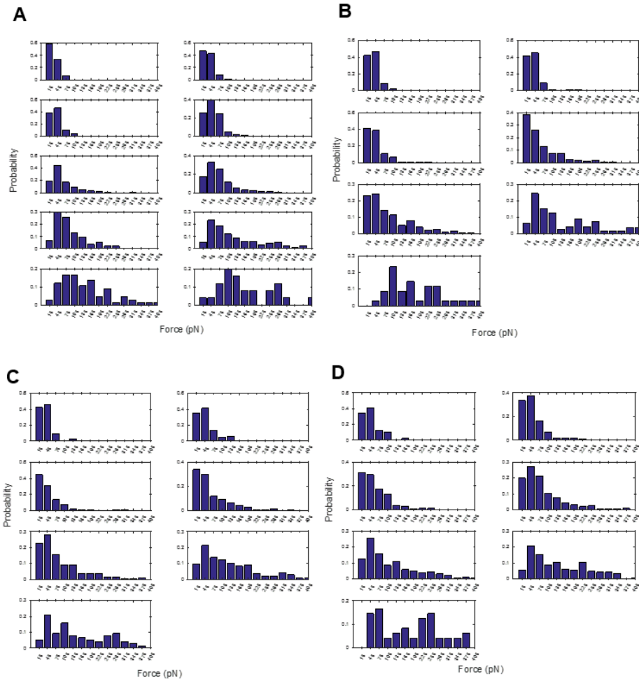
Figure 9.4. Adhesion Force Histograms Obtained at Different Loading Rates. A) Wild Type Kinesin B) S175A Kinesin C) cN332A Kinesin D) cD72N Kinesin. There is Unimodal Distribution at Low Loading Rates and Bimodal Distribution at High Loading Rates in All Cases.
