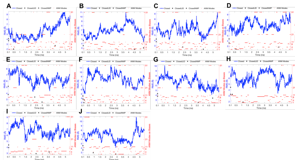
Figure 7.4. RMSD and the biased CV versus simulation time of each replica for wild type-1. Replicas 1 to 10 are given in A to J, respectively.
