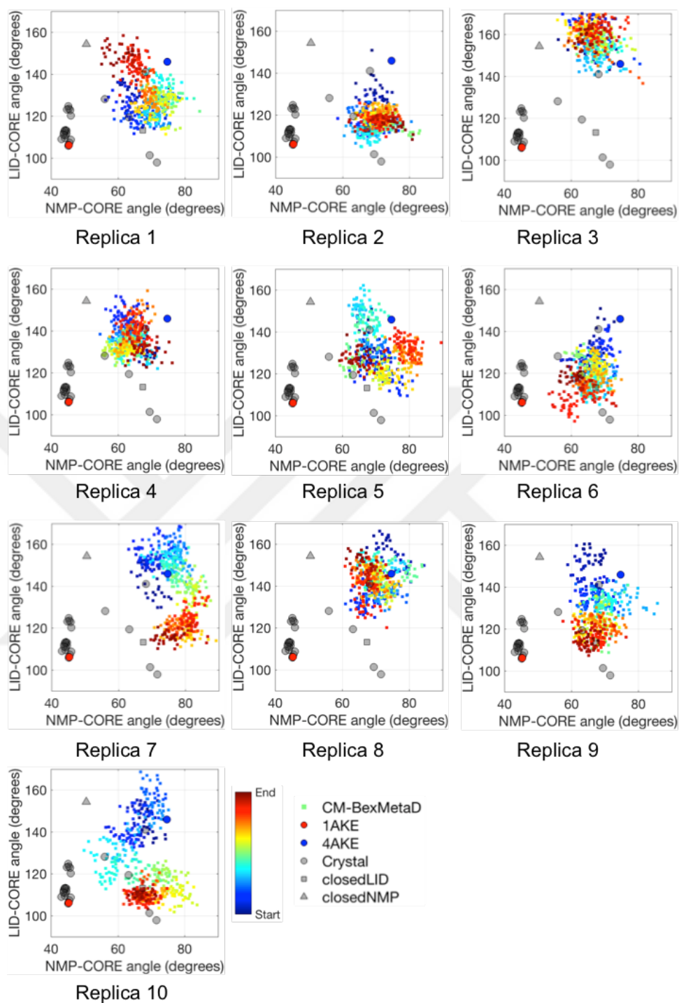
Figure 7.8. Conformational sampling of AdK in terms of LID-CORE and NMP-CORE angles for Y171W simulation via CM-BexMetaD-2 protocol together with experimentally determined structures. The angles are color-coded according to the simulation time.
