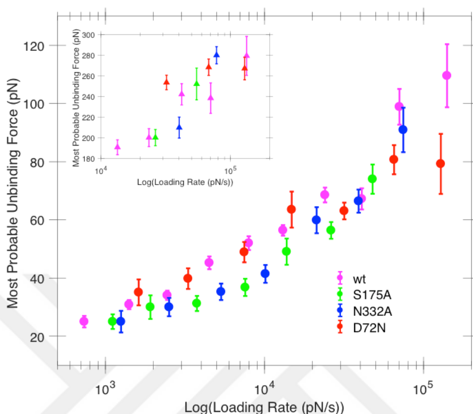
Figure 9.5. The dynamic adhesion force spectra of kinesin-tubulin complex depending on the loading rates. The most probable rupture force vs logarithm of the loading rates determined as low-strength state is given as main plot, whereas the high-strength state is given as inset.
