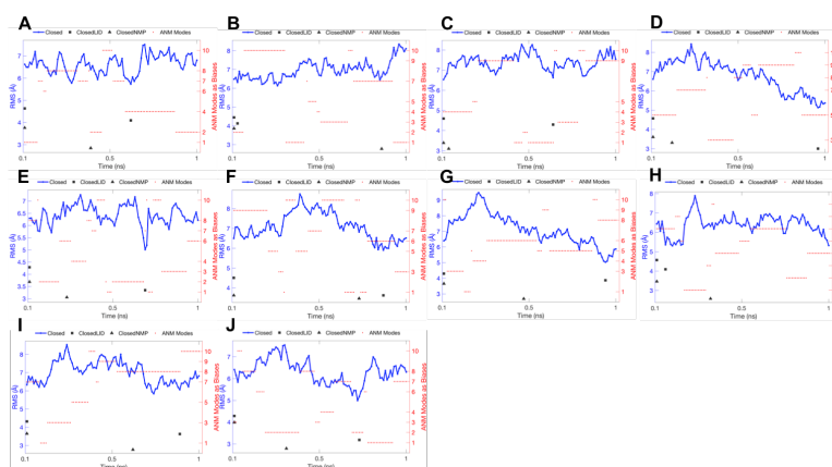
Figure 7.2. RMSD and the biased CV versus simulation time of each replica at cycle 1 by CM-BexMetaD-1. Replicas 1 to 10 are given in A to J, respectively.
