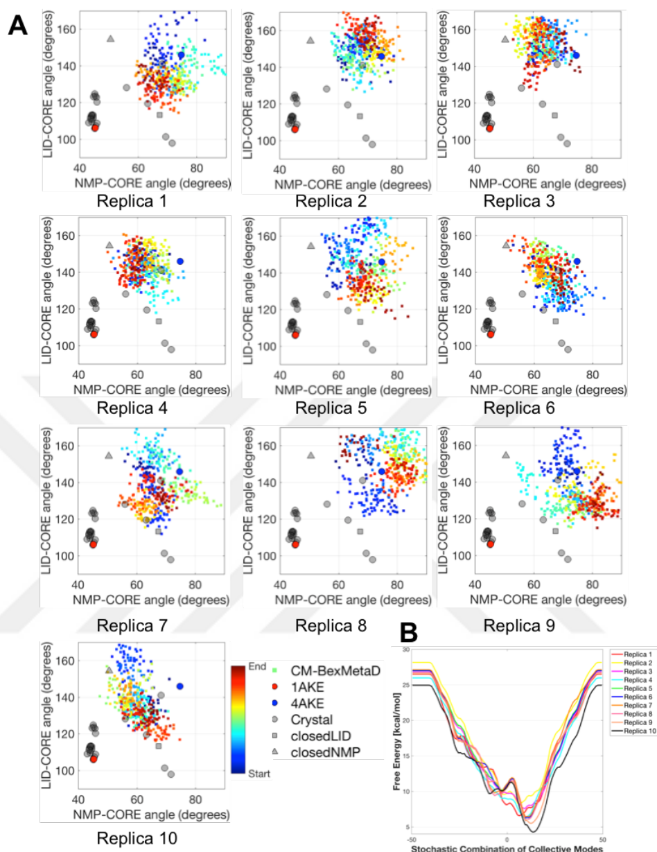
Figure 7.12. A) Conformational Sampling of AdK in terms of LID-CORE and NMP-CORE Angles for Non-Targeted Simulation of apo AdK The Angles are Color-Coded According to the Simulation Time. B) FEL Underlying the Conformational Transition of the Enzyme.
