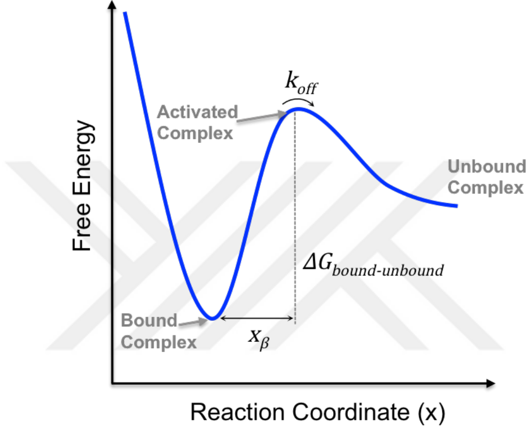
Figure 5.4. Free energy landscape of the dissociation of a biomolecular complex, together with the associated Bell model parameters.
