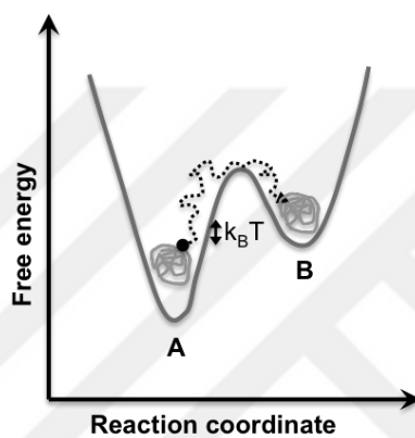
Figure 3.1. Schematic representation of two stable states A and B on the FEL of a molecular system.
