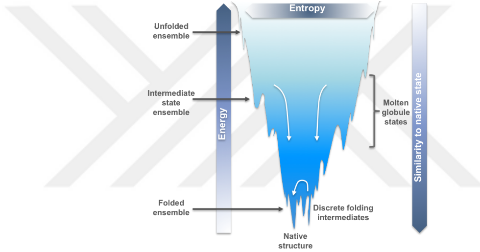
Figure 2.3. Schematic Representation of the Folding Funnel of a Protein. The Funnel Shape Reflects the Simultaneous Decrease in the Energy and Entropy as well as the Increase in Similarity to Native State of the Protein during its Folding. Adapted from [32].
