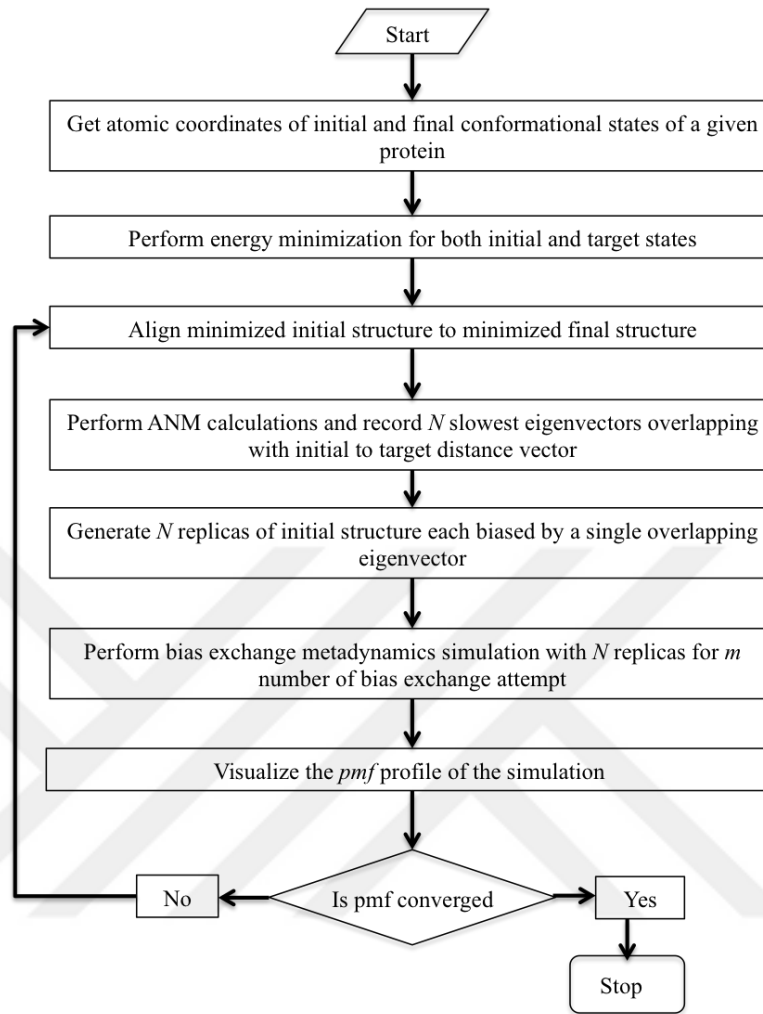
Figure 6.5. Flowchart of targeted CM-BexMetaD-2 approach.
