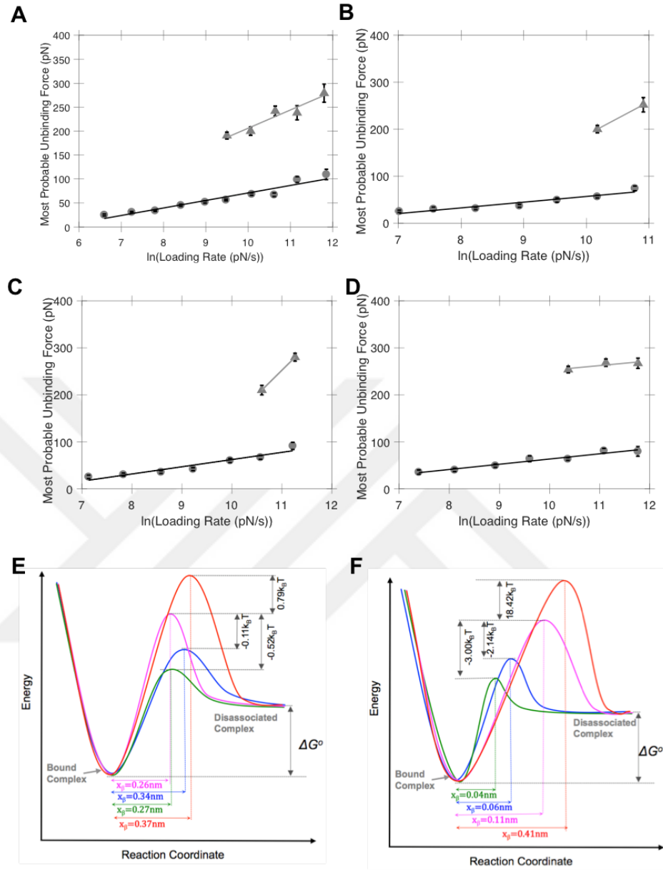
Figure 9.6. DFS Results of Kinesin-Tubulin Complex. A) Wild Type Kinesin B) S175A Kinesin C) N332A Kinesin D) D72N Kinesin. A Smooth Diagram of the Binding Energy Landscape of the Low-Strength State of Kinesin-Tubulin Complex (E) and the High-Strength State (F).
