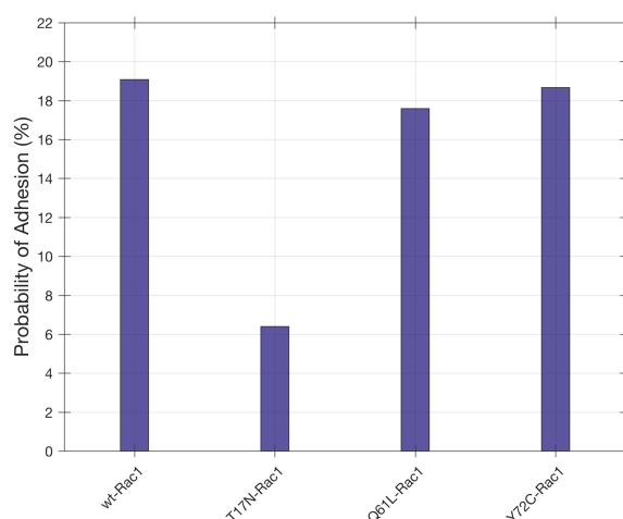
Figure 10.6. The probability of adhesion of wild-type, T17N, Q61L and Y72C Rac1-PAK1 observed in the experiments.
