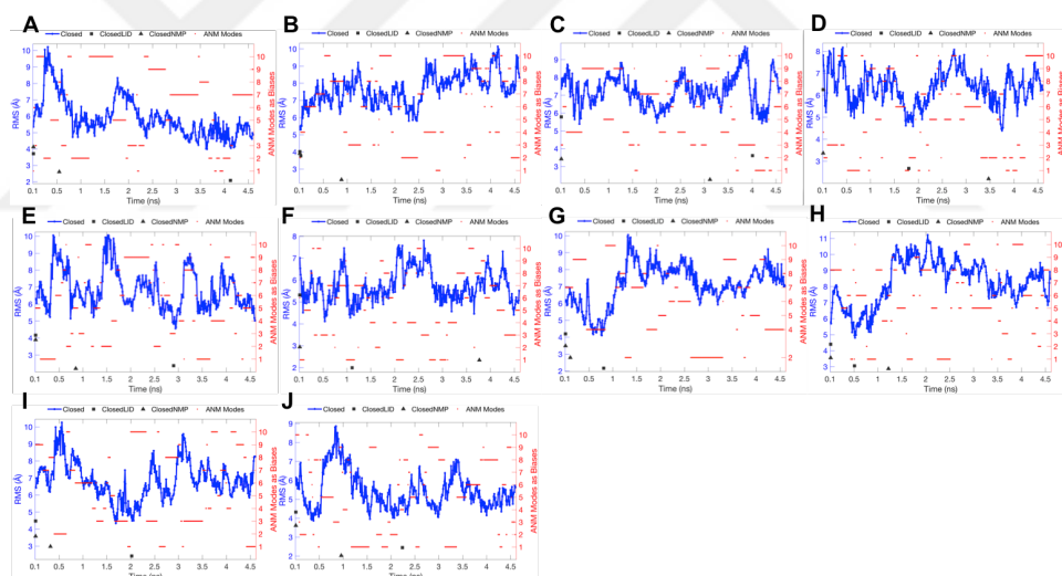
Figure 7.5. RMSD and the biased CV versus simulation time of each replica for Y171W. Replicas 1 to 10 are given in A to J, respectively.
