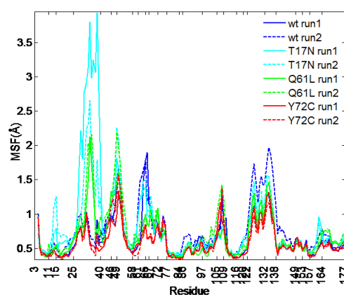
Figure 10.4. MSF profiles during parallel MD simulations for the wild-type and mutant Rac1 structures. Functional regions on Rac1: p-loop (res. 10-17, GTP-binding), Switch I (res. 26-45, downstream effector), Switch II (res. 59-74, activation loop) and Insert (res. 124-135).
