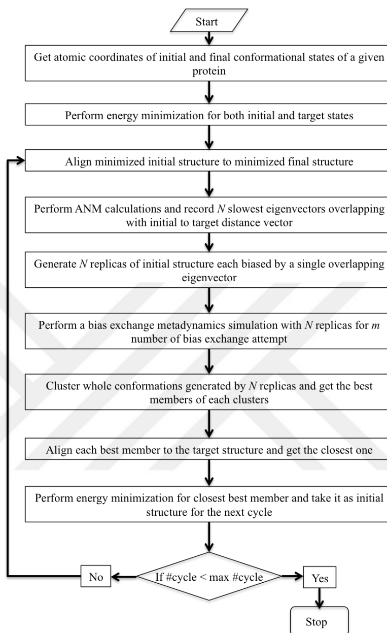
Figure 6.4. Flowchart of targeted CM-BexMetaD-1 approach.
