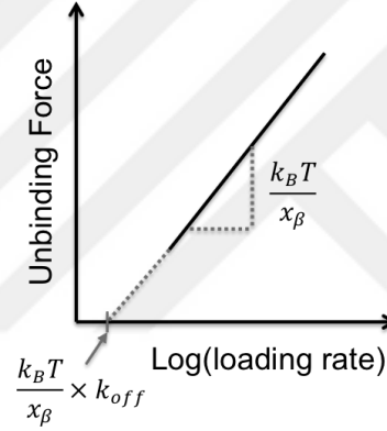
Figure 5.5. The linear relation between the unbinding force and the logarithm of the loading rate. Bell parameters can be extracted from the slope and the intercept of the linear relation [177].
