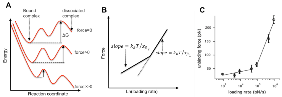
Figure 5.6. Energy Landscape of a Molecular Complex Having two Transition States and the Corresponding DFS Results. a) Two-Barrier Model in Energy Landscape b) Corresponding Two Linear Regimes. c) Dynamic Force Spectra of Biotin-Streptavidin Complex [156].
