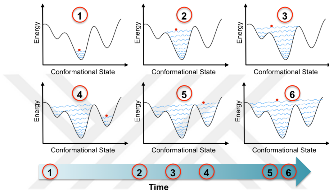
Figure 3.3. A Schematic Representation of Metadynamics Method. The Simulation Searches Energy Well Avoiding Oversampling Using its Memory. When the Bias Potential Fills the First Minima, the System Goes to a Lower Energy Configuration.
