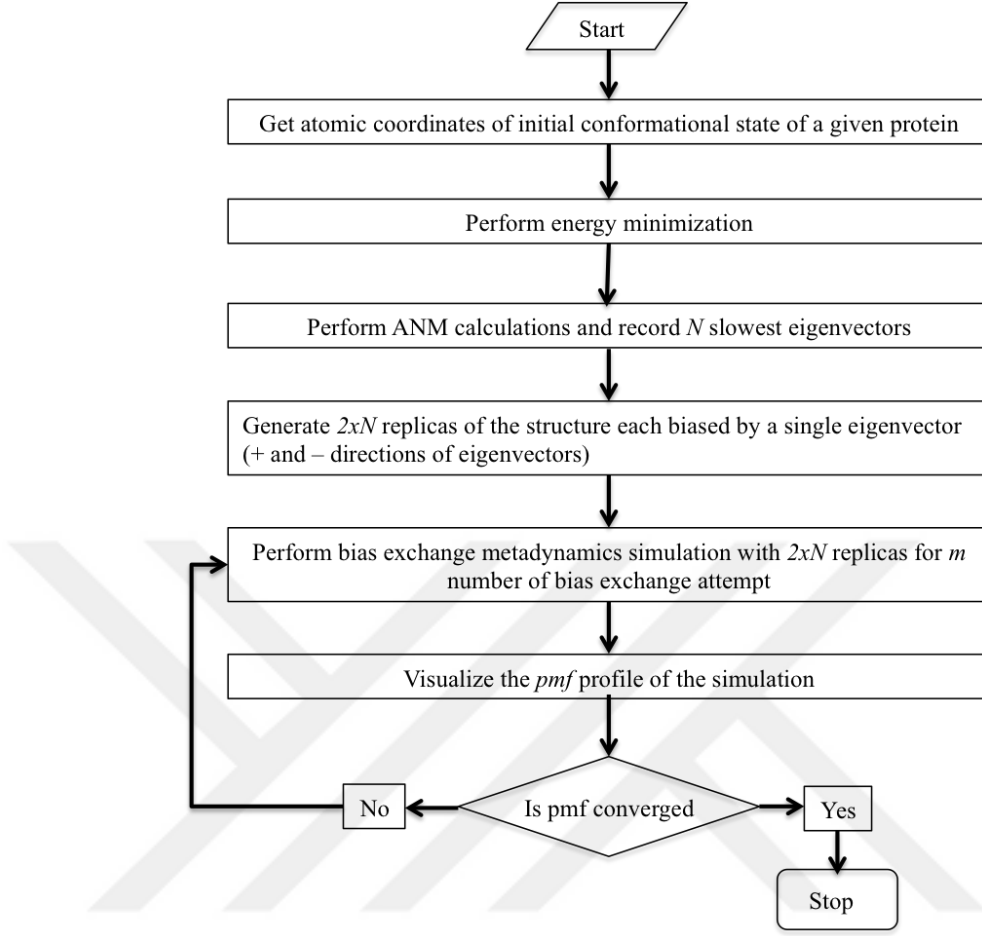
Figure 6.6. Flowchart of non-targeted CM-BexMetaD approach.
