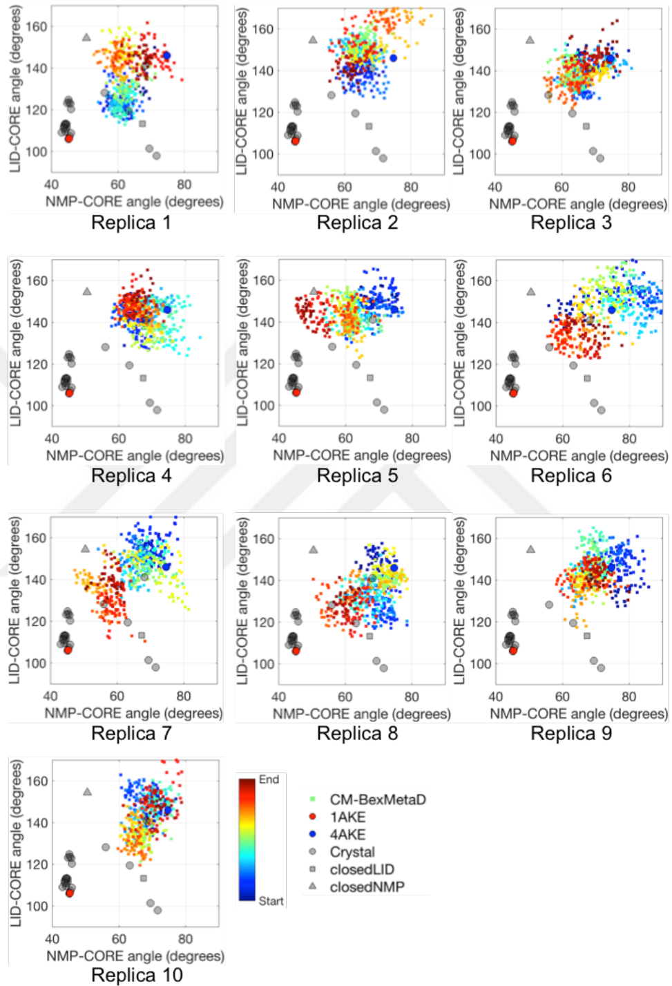
Figure 7.7. Conformational Sampling of AdK in Terms of LID - CORE and NMP - CORE Angles for the wild - type - 1 Simulation Via CM - BexMetaD - 2 Protocol Together with experimentally determined Structures. The Angles are Color - Coded According to the Simulation Time.
