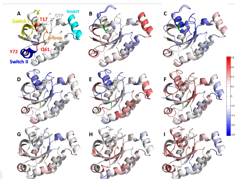
Figure 10.5. A) Functional Regions and Mutations on Wild-Type Rac1. Average PCA Cross Correlations at P-Loop and Switch I for T17N (B-C). P-Loop, Switch I, and Switch II (D-F) for Q61L and (G-I) for GTP-Bound Y72C Mutant Rac1 (in silico).
