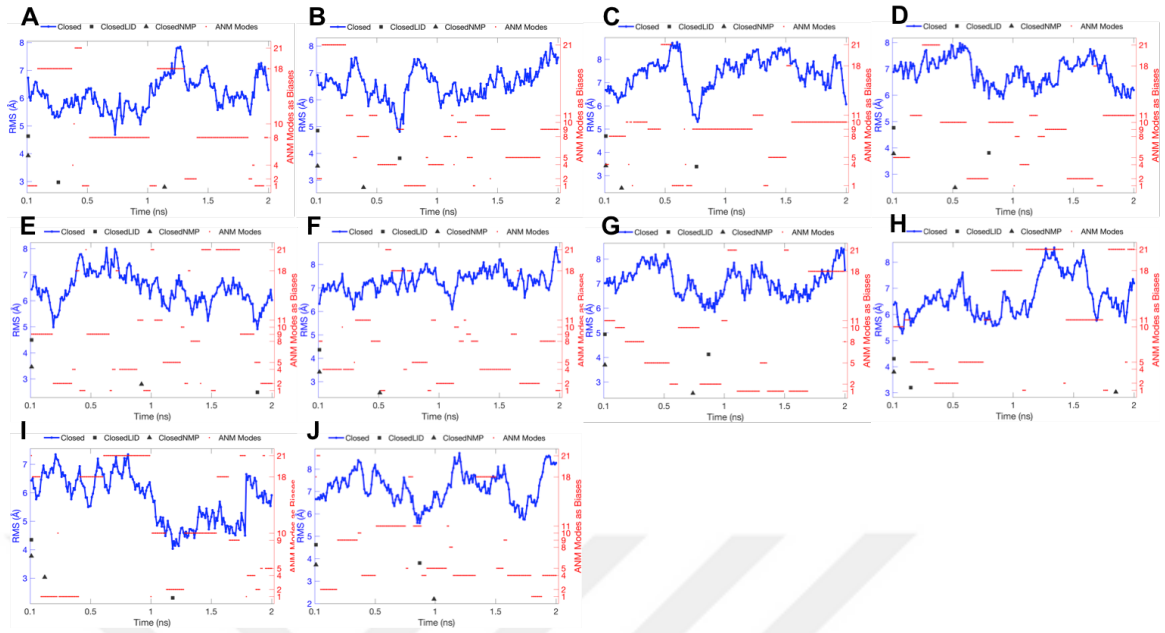
Figure 7.3. RMSD and the biased CV versus simulation time of each replica at cycle 1. Replicas 1 to 10 are given in A to J, respectively.
