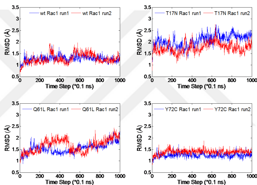
Figure 10.3. RMSD profiles during parallel MD simulations for the wild-type and mutant Rac1 structures.
