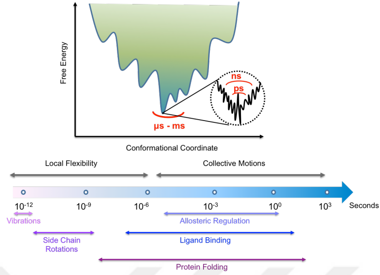
Figure 2.2. Some examples of the protein conformational dynamical movements.
