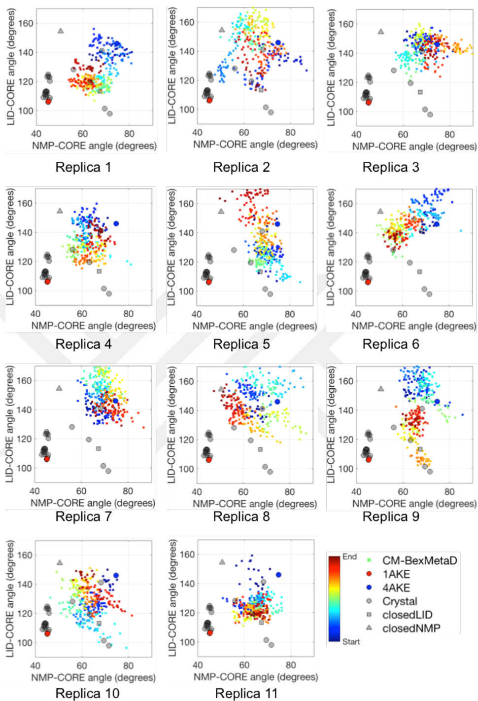
Figure 7.9. Conformational sampling of AdK in terms of LID-CORE and NMP-CORE angles for the wild-type-2 simulation via CM-BexMetaD-2 protocol together with experimentally determined structures. The angles are color-coded according to the simulation time.
