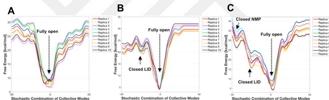
Figure 7.10. FEL along the conformational transition of wild type and mutant apo AdK. A) The wild type-1, B) Y171W, C) the wild type-2.
