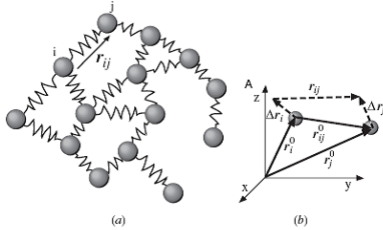
Figure 6.1. Description of the Gaussian network model (GNM).
