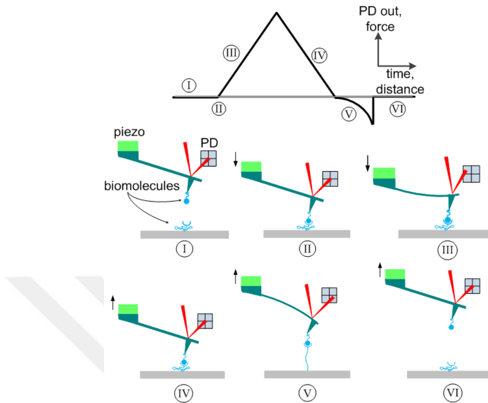
Figure 5.3. A typical photodetector signal recorded during a biomolecular force spectroscopy experiment together with the corresponding situation of cantilever and surface.
