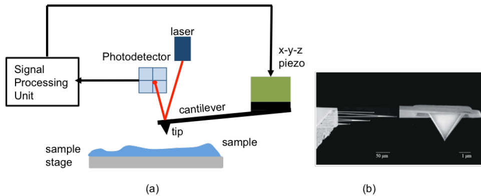
Figure 5.1. Schematic Illustration of the Fundamental Components of an AFM Device with Working Principles (a) and a Sample Cantilever (b).
