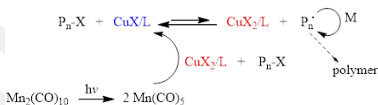
Figure 2.6: Mechanism of using \text{Mn}_2(\text{CO})_{10} in light initiated ATRP.
