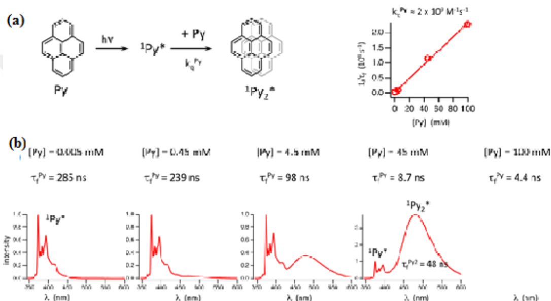
Figure 4.6: a) Determination of the bimolecular quenching rate constants k_q^{\text{Py}} of pyrene singlet excited states by ground state pyrene. b) Fluorescence spectra of pyrene at different concentrations in DMF.
