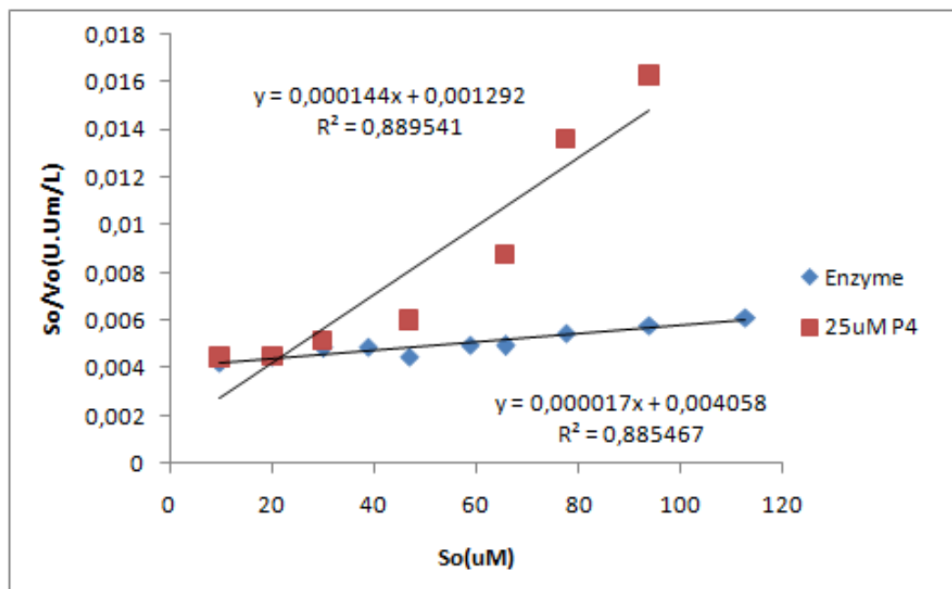
Figure 5.40. Hanes-Woolf plot for enzyme 2 with and without 25 \mu\text{M} P4
