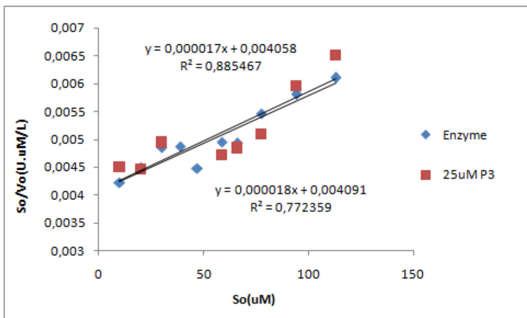
Figure 5.32. Hanes-Woolf plot for enzyme 2 with and without 25 \mu\text{M} P3
