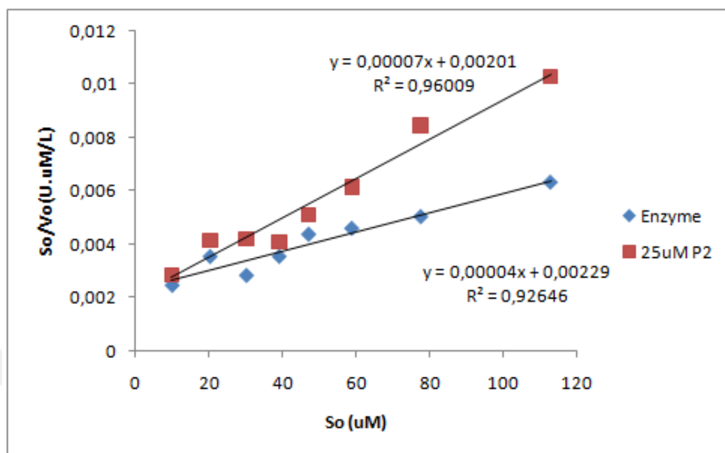
Figure 5.20. Hanes-Woolf plot for enzyme 1 with and without 25 \mu M P2
