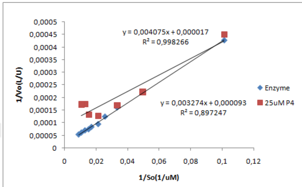
Figure 5.39. Lineweaver-Burk plot for enzyme 2 with and without 25 \mu\text{M} P4
