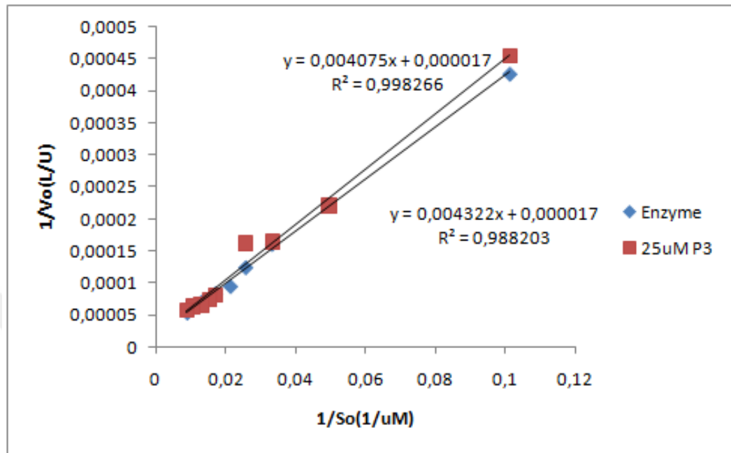
Figure 5.31. Lineweaver-Burk plot for enzyme 2 with and without 25 \mu\text{M} P3
