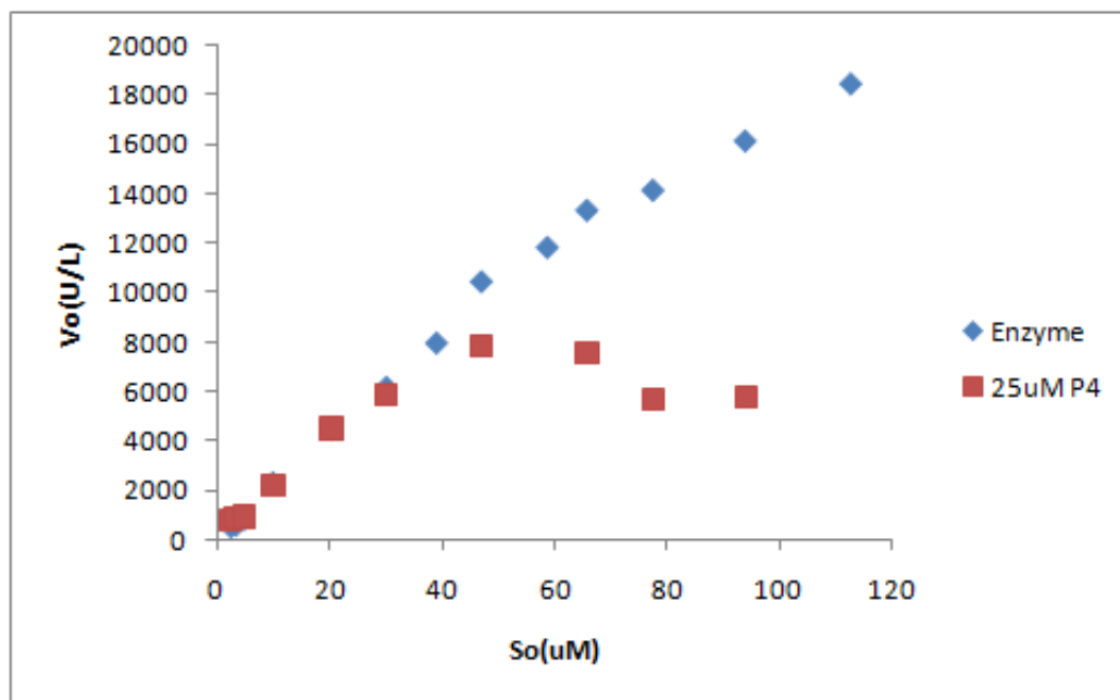
Figure 5.38. Activity Values of Enzyme 2 ( V_o ) with and without 25\mu\text{M} P4 for selected CENTA concentrations
