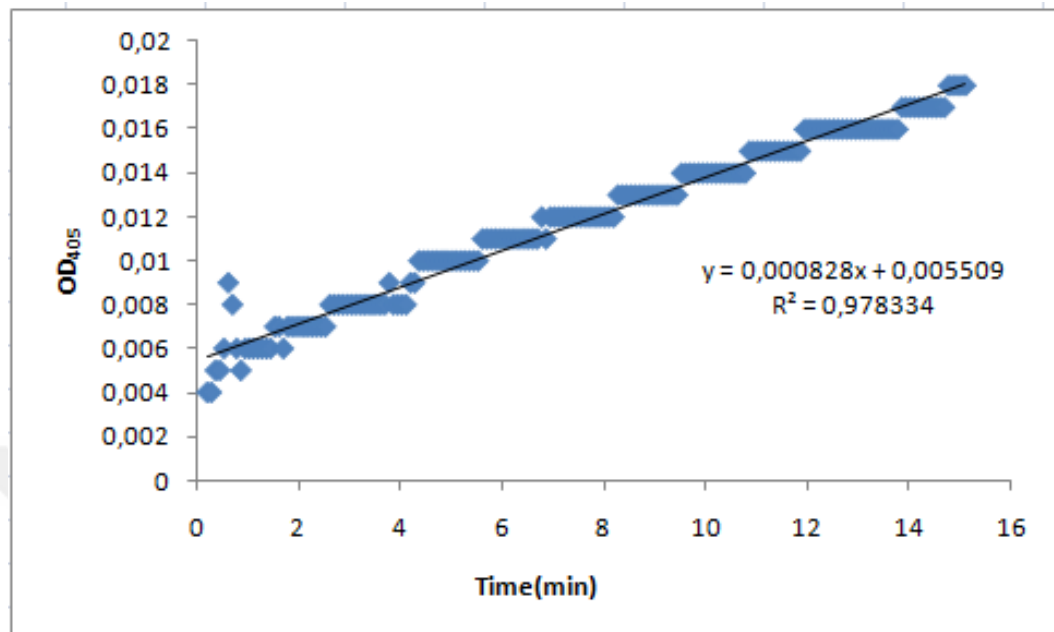
Figure 5.2. Beta lactamase mediated hydrolysis of 47 \mu M CENTA in the presence of 100 \mu M clavulanic acid
