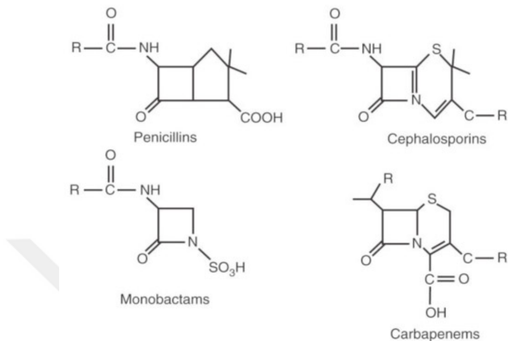
Figure 2.1. Chemical structures of penicillin, cephalosporin, monobactam and carbapenem [8]
