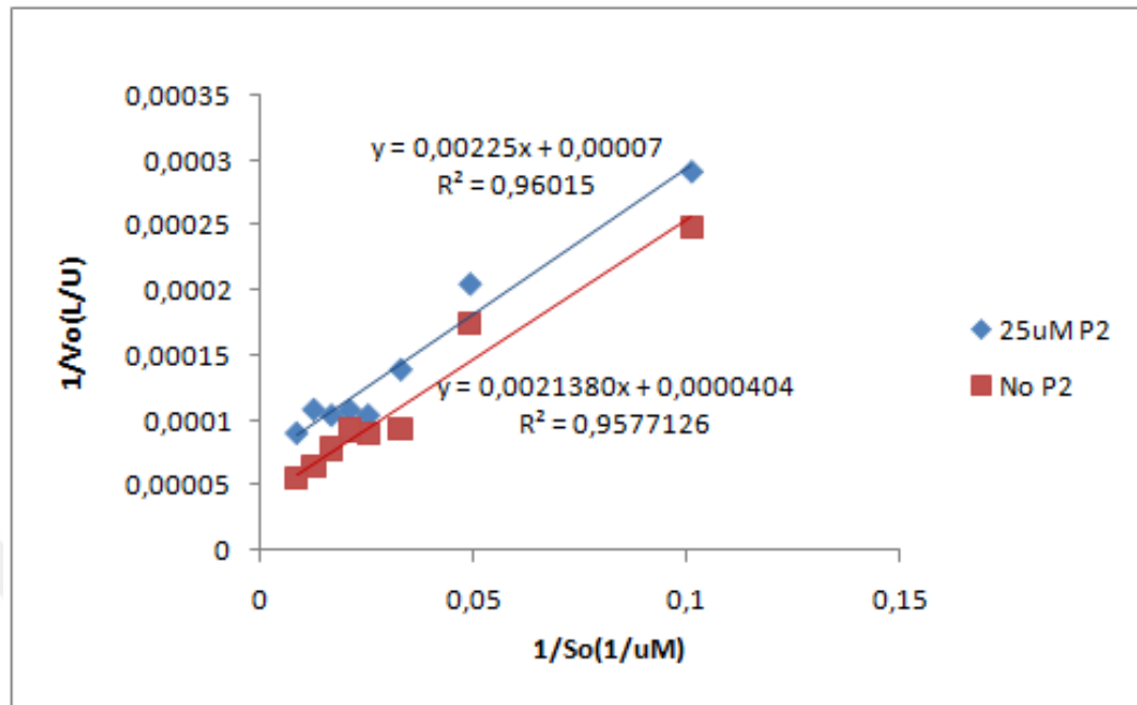
Figure 5.19. Lineweaver-Burk plot for enzyme 1 with and without 25 \mu M P2
