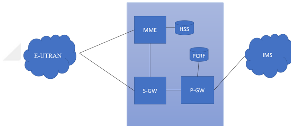
Figure 2.3 EPC Connection with RAN EPC architecture
