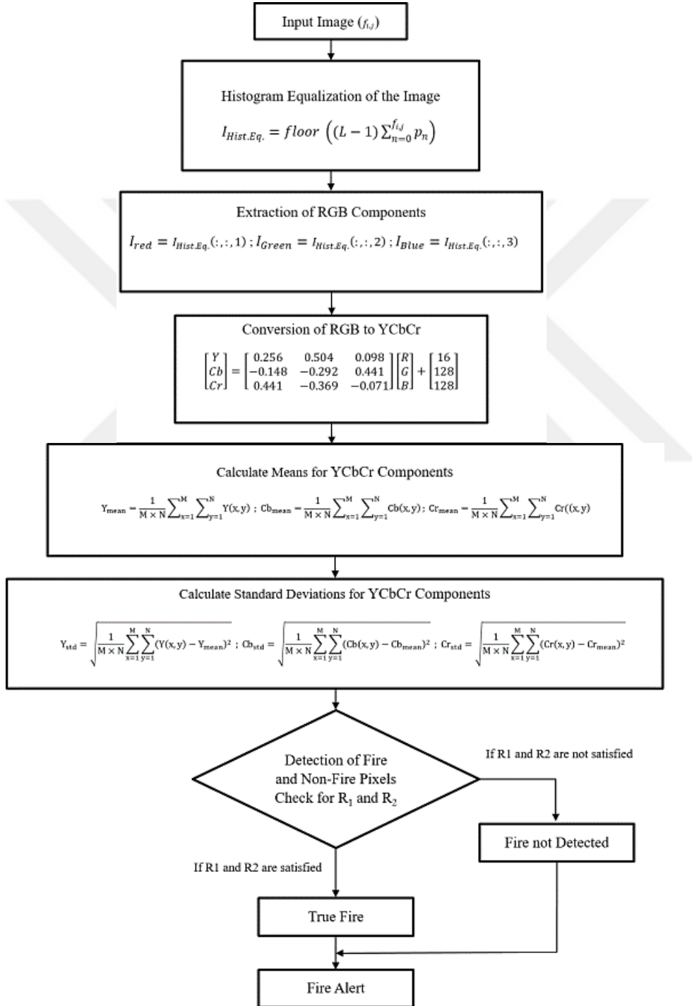
Figure 3.6: Flow diagram of proposed fire verification algorithm
