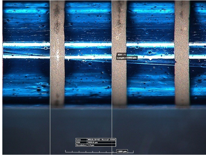
Figure 5.5 Distance between two lines after 1mm test.
