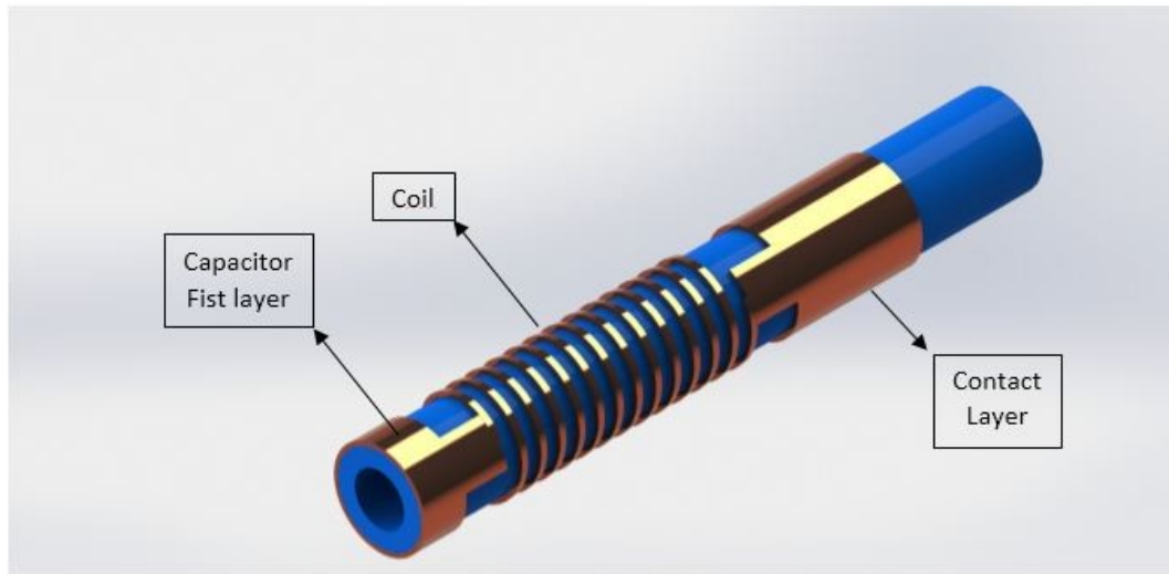
Figure 4.28 First layer of marker device design.
