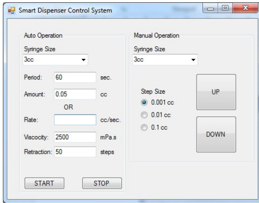
Figure 4.23 Custom Dispenser Unit Control Software Interface.
