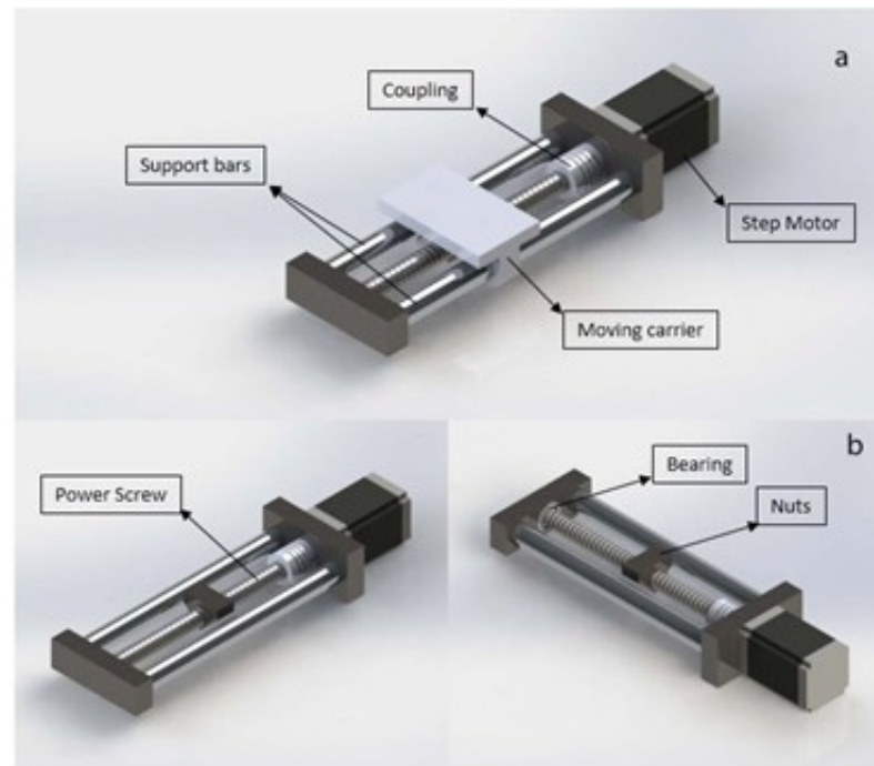
Figure 4.4 (a) Linear motion mechanism with moving carrier is mounted. (b) Components of mechanism from different perspectives.
