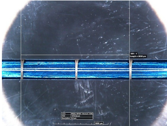
Figure 5.9 Backlash measurement, before calibration.
