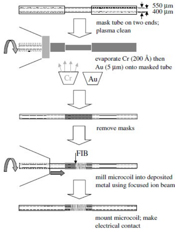
Figure 2.6 The sequence of steps used in the fabrication of the microcoil [64].
