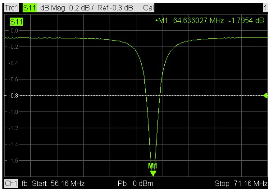
Figure 5.27 Resonance frequency of marker, in the air.
