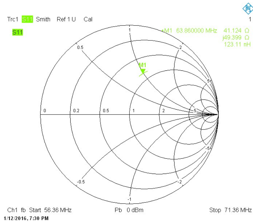
Figure 5.19 Smith chart diagram of coil measurement.
