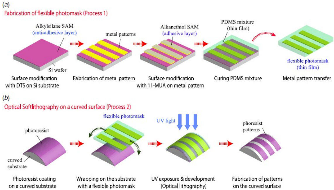
Figure 2.5 The schematic of optical soft-lithography. (a) Pattern transfer process for fabricating micro-metal patterns on the PDMS film surface. (b) Optical lithography on a curved surface using a flexible film type of a photomask [70].
