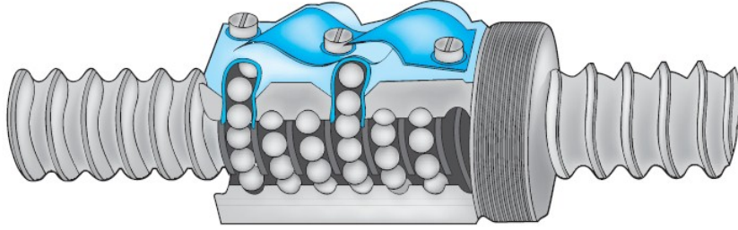
Figure 4.1 Ball-bearing screw assembly with a portion of the nut cut away to show construction [80].
