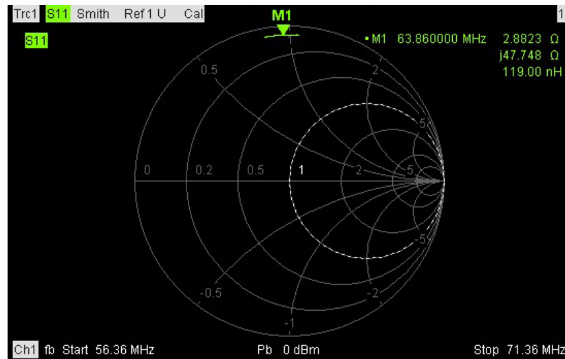
Figure 5.24 Inductance measurement after parylene coating.
