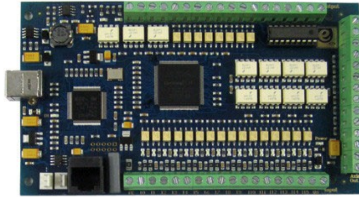
Figure 4.22 USB MACH3 Interface card with 16 bit digital I/O.
