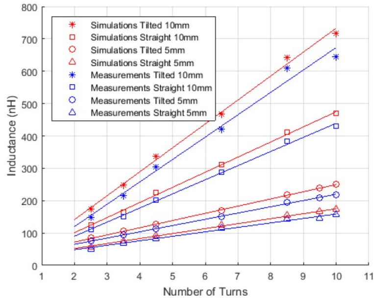
Figure 4.27 Inductance results of simulations and measurements.
