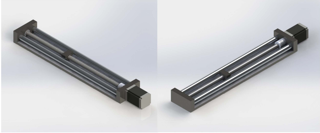
Figure 4.6 Final X axis design, without moving carrier is mounted.
