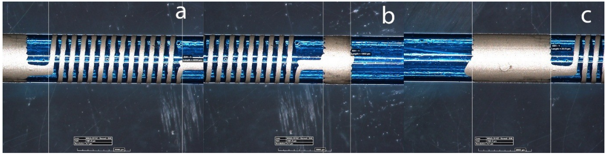
Figure 5.17 (a) Coil length measurement, (b) capacitor first layer length measurement, (c) contact layer length measurement.
