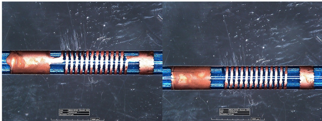
Figure 5.20 First layer of resonant circuit after copper electroplating.
