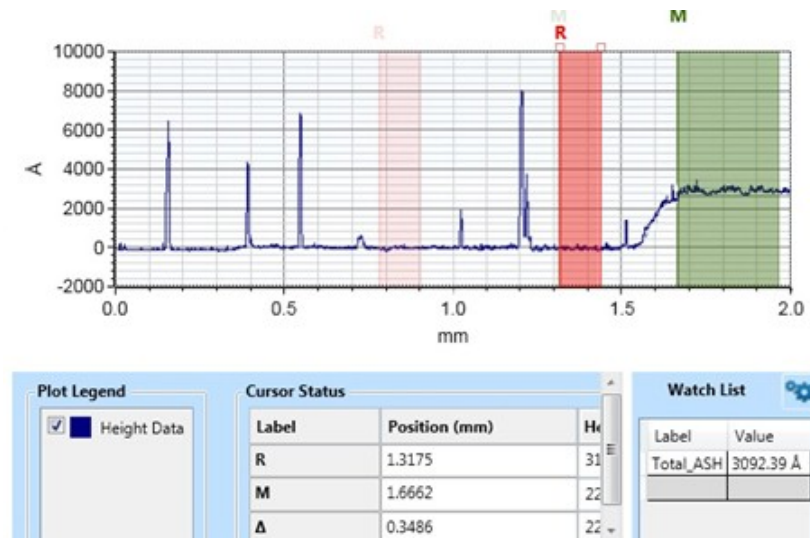
Figure 5.23 Parylene thickness measurement.
