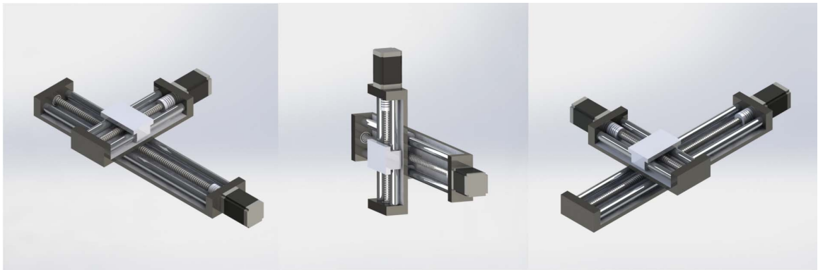
Figure 4.7 Z axis is assembled onto X axis' moving carrier.
