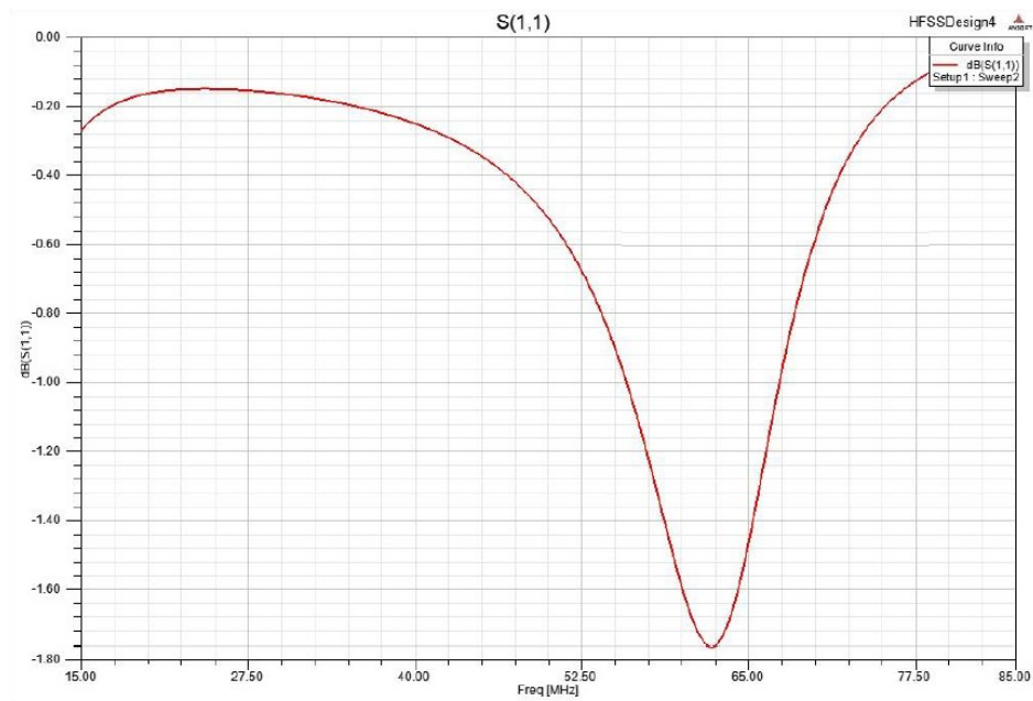
Figure 4.30 S11 plot of resonant circuit.
