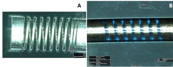
Figure 2.7 . (a) Mask used for coil geometry. (b) Cr/Au Coil geometry formed on 6Fr catheter wall by thermal evaporation.
