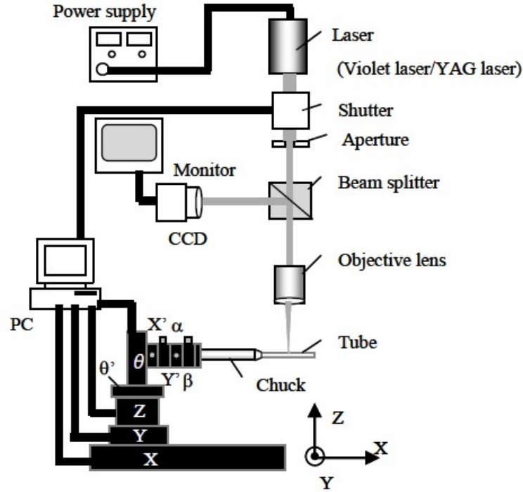
Figure 2.4 Computer controlled 3D laser pointer system. [69].
