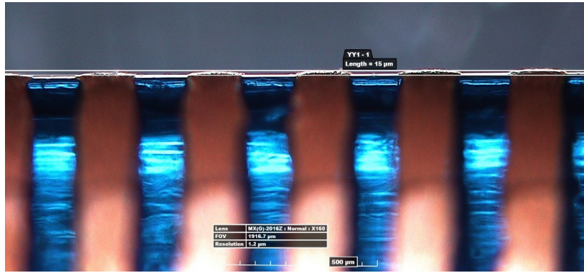
Figure 5.21 First layer thickness measurement after copper electroplating.
