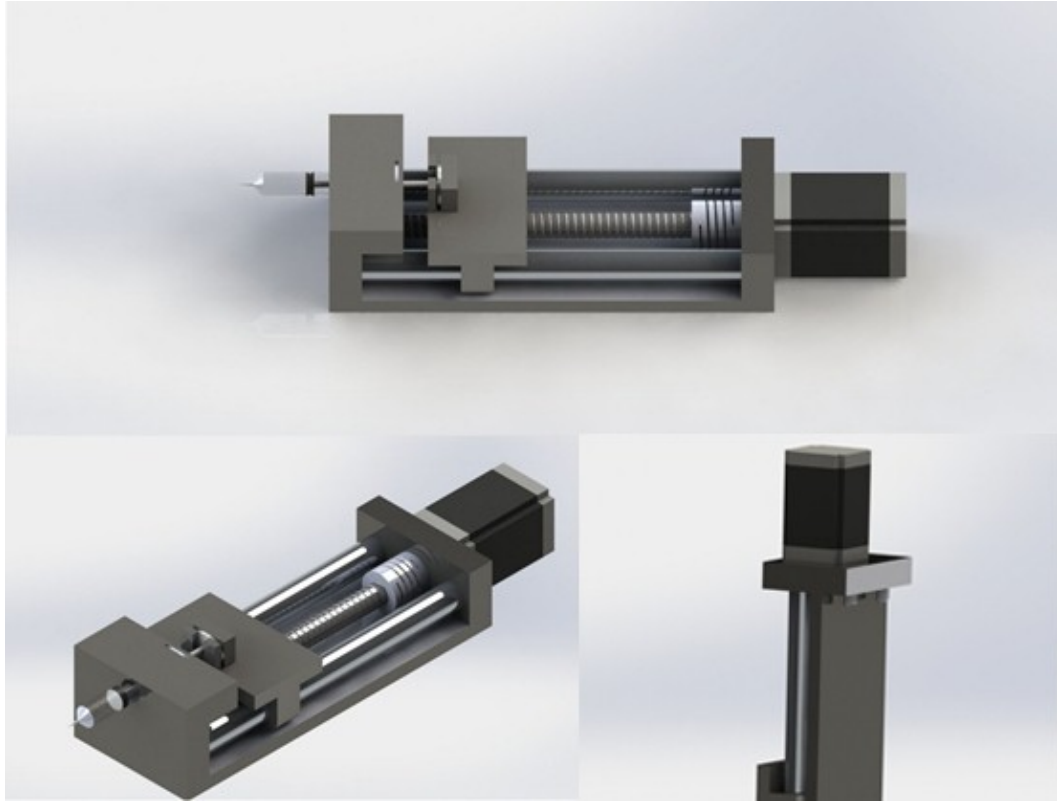
Figure 4.12 Air-free, mechanical dispensing unit mechanism, with 3cc syringe barrel.
