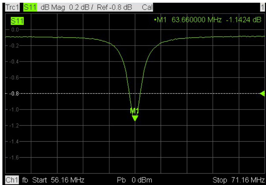
Figure 5.28 Resonance frequency of marker, in liquid phantom.
