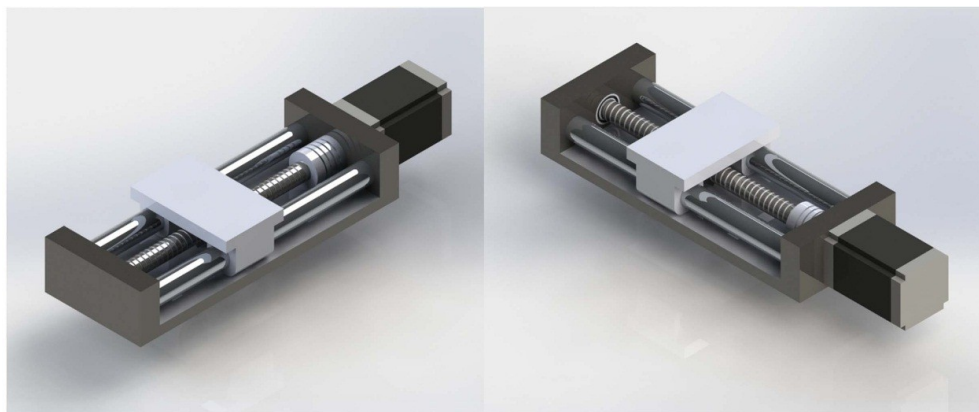
Figure 4.5 Final Z axis design with moving carrier is mounted.
