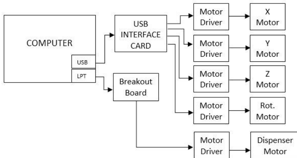
Figure 4.24 Schematic diagram of control and electronic system.
