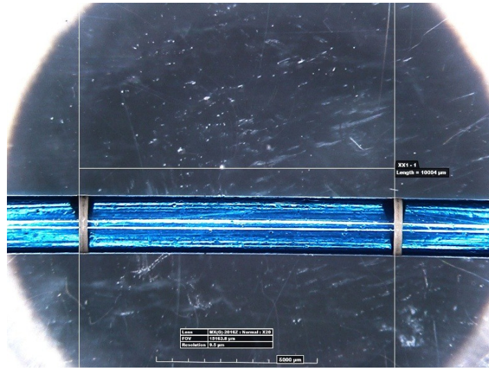
Figure 5.8 Distance between two lines after 10mm test.
