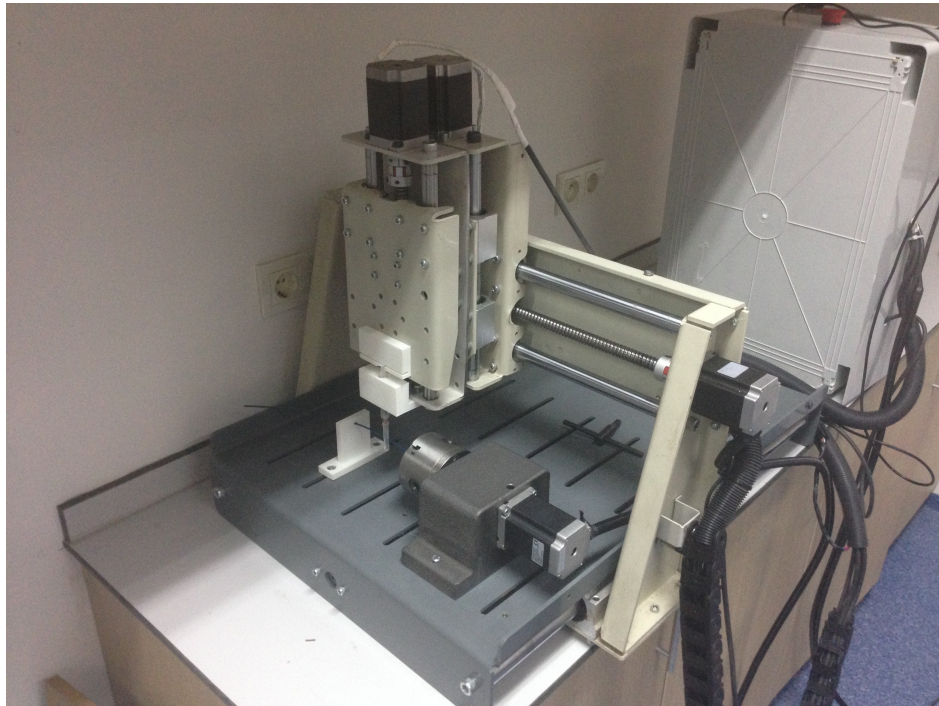
Figure 4.15 Final motion control system with mounted dispenser unit.
