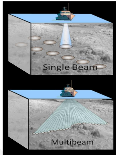
Figure 1.5. Coverage efficiency of multibeam echosounder compared to singlebeam echosounder [29]
