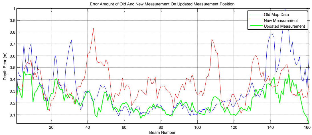
Figure 4.20. Error amount of old and new measurement and error of updated measurement position
