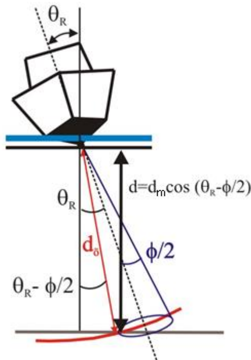
Figure 3.11. Effect of roll of a survey ship [43]
