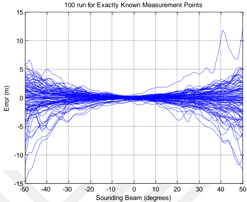
Figure 3.14. Errors caused by measurement line difference – ship motion not corrected (beam number vs error graph with 100 trials)
