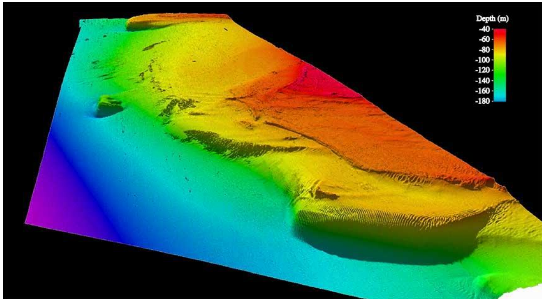
Figure 1.6. An image obtained with a multibeam echosounder [32]
