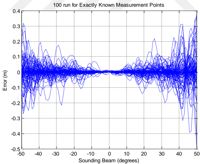
Figure 4.8. Error rates for a measurement with exactly known measurement data points for given ping cycle where ship movement/position effects are not included
