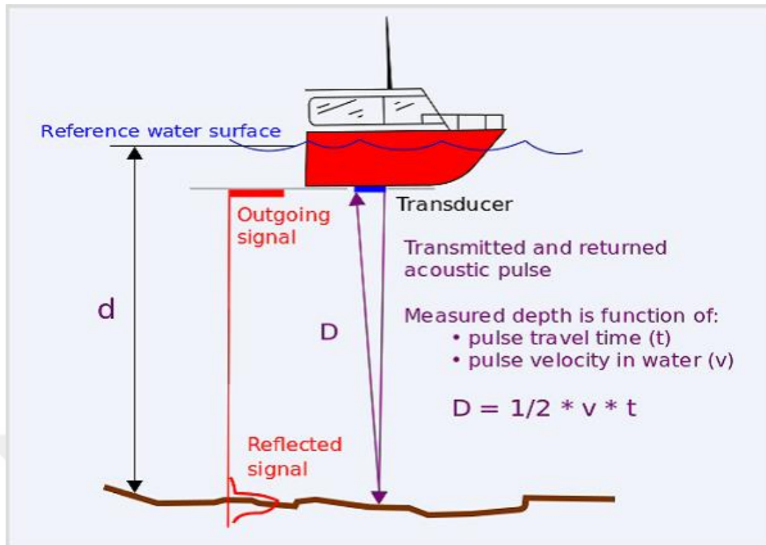
Figure 1.4. Single beam echosounder operation [27]
