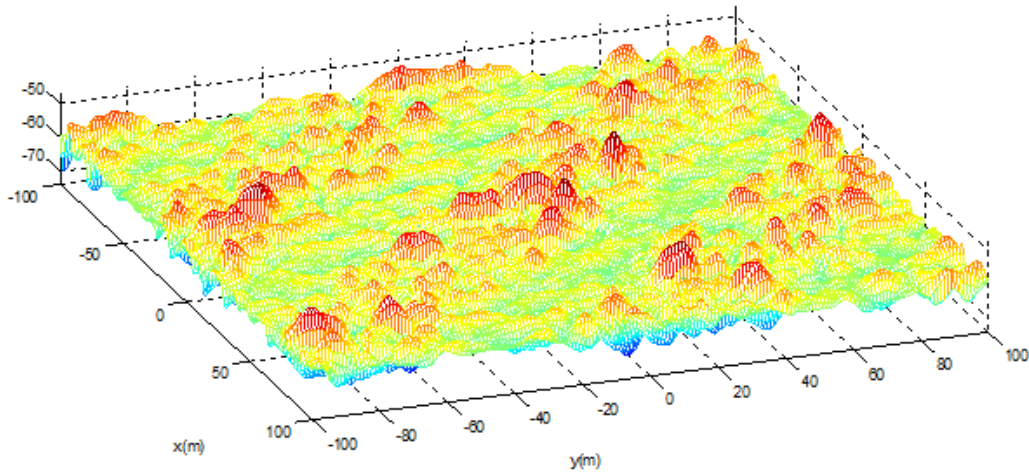
Figure 4.1. Simulated bottom map showing the 100 m vicinity of operation point
