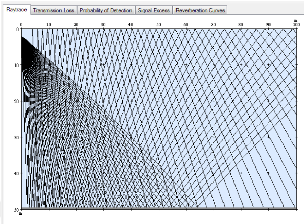
Figure 3.7. Typical summer sound velocity profile causing beams to deflect towards deeper water
