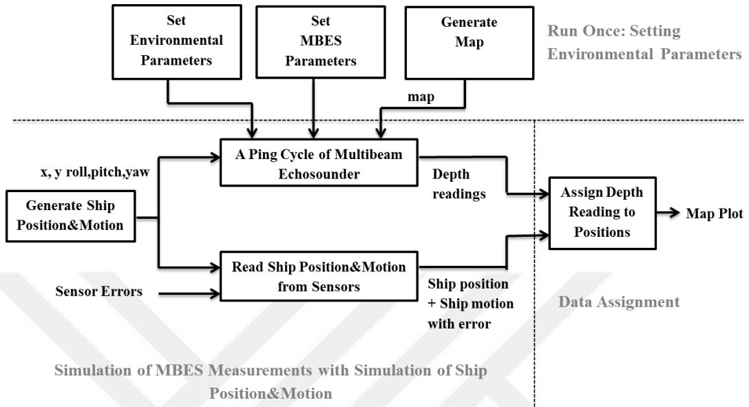
Figure 2.6. First block diagram of multibeam sonar simulation
