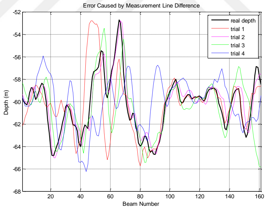
Figure 4.12. Error caused by measurement line difference [\sigma_x, \sigma_y, \sigma_{roll}, \sigma_{pitch}, \sigma_{yaw}] = [1, 1, 1, 1, 1]
