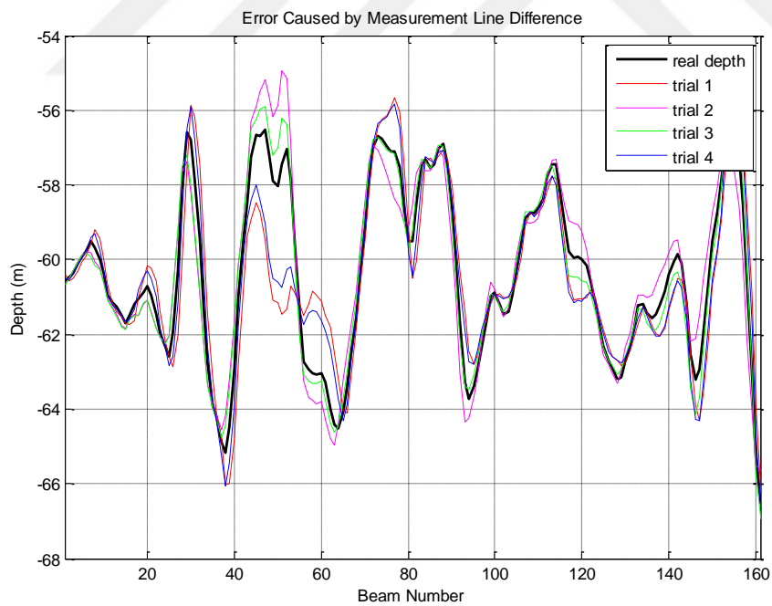
Figure 4.14. Error caused by measurement line difference [\sigma_x, \sigma_y, \sigma_{roll}, \sigma_{pitch}, \sigma_{yaw}] = [0.5, 0.5, 0.2, 0.2, 0.2]
