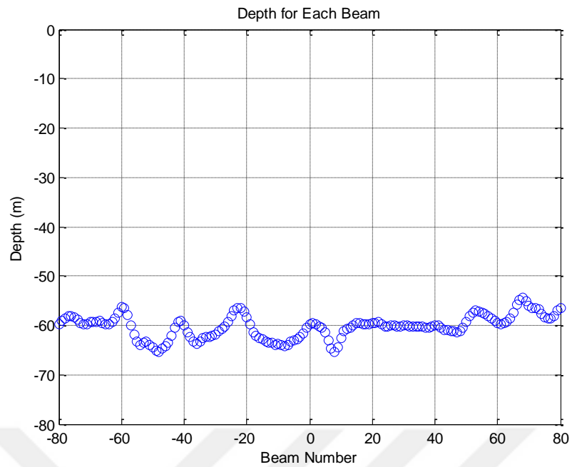
Figure 4.6. Depth vs beam angle for given ping cycle
