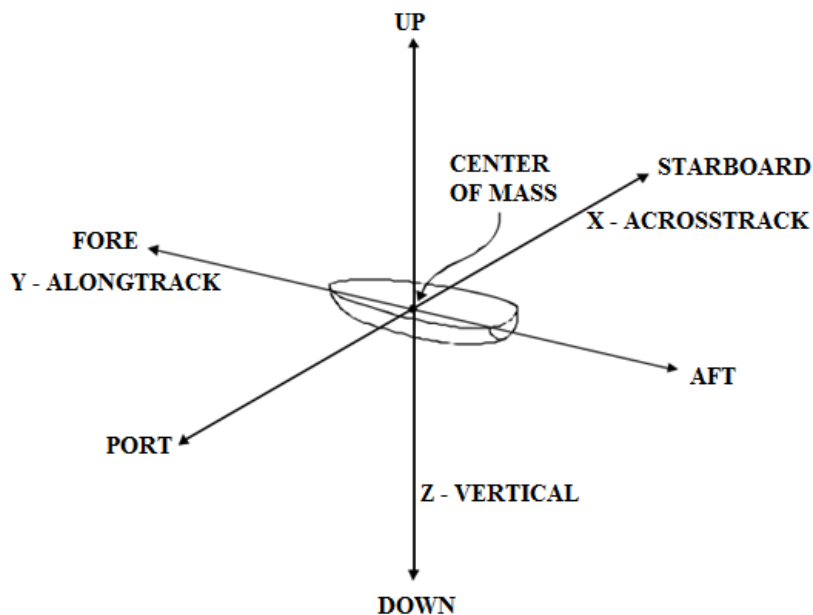
Figure 3.17. Coordinate system with an origin on ship's center of mass [64]
