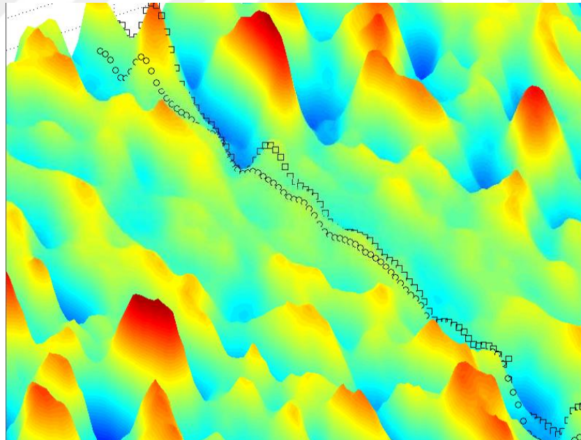
Figure 4.9. Measurement line at 0^\circ pitch 0^\circ roll motion and 0.5^\circ pitch 3^\circ roll motion on 3D Map (actual depth positions are denoted with circle and depth reading positions are denoted with square)
