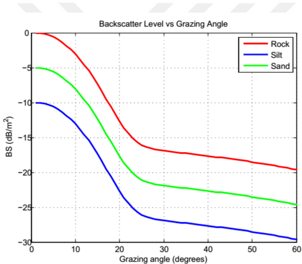
Figure 3.3. Backscattering levels versus grazing angle for different bottom types
