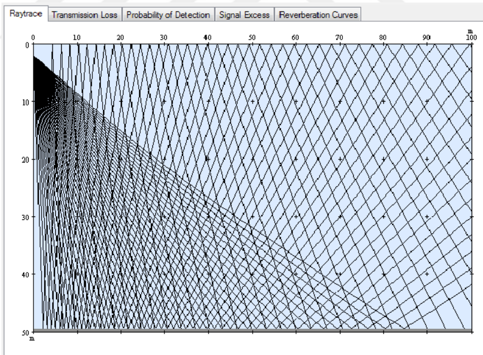
Figure 3.8. Typical winter sound velocity profile causing beams to deflect towards shallow water
