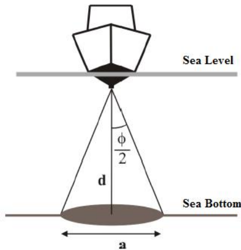
Figure 3.1. Sea bottom coverage in single beam echosounder [44]
