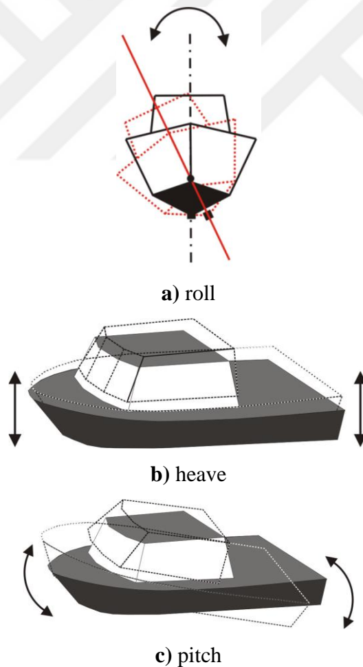
Figure 3.10. Rotational motions of a survey ship [43]
