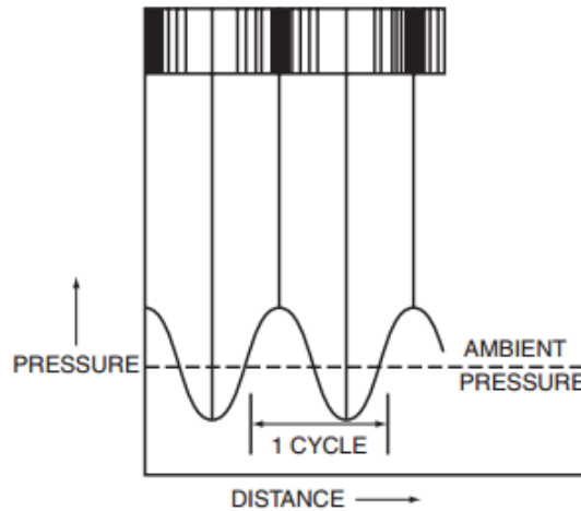
Figure 2.1. Acoustic wave [59]
