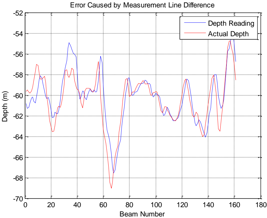
Figure 3.13. Errors caused by measurement line difference – ship motion not corrected (line of readings)
