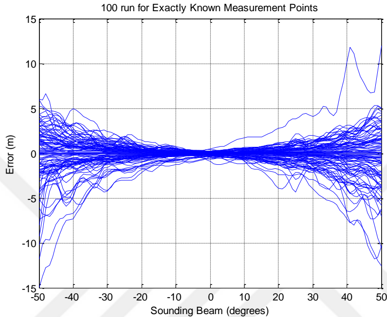
Figure 4.10. Errors caused by measurement line difference – ship motion not corrected (beam number vs error graph with 100 trials)
