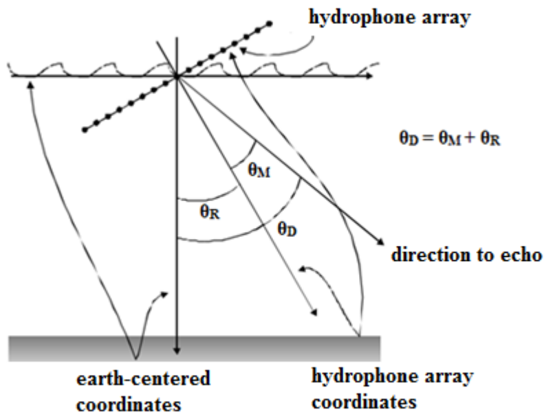
Figure 3.19. Difference of earth-centered coordinates and hydrophone array coordinates caused by roll angle [62]
