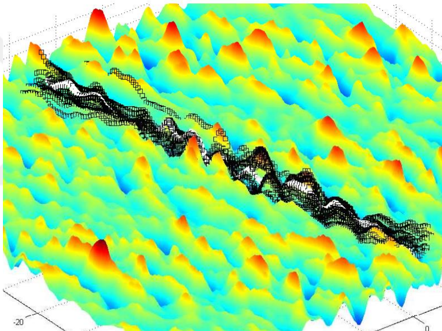
Figure 4.16. On the same location and same roll, pitch, and yaw – the position of depth readings varies with changing motion sensor errors (white denotes the assigned positions for error-free motion sensor)
