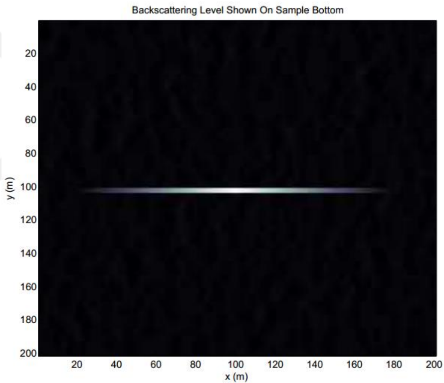
Figure 3.4. Effect of grazing angle on echo shape and level
