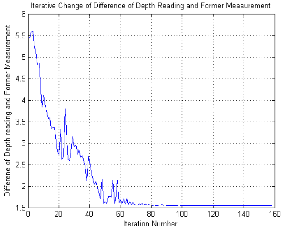
Figure 4.18. Optimization run about error on both depth measurement and ship motion&position sensors (a, b, c, d, e, f are former measurement and depth reading, g is iterative change of difference of depth reading and former measurement)
