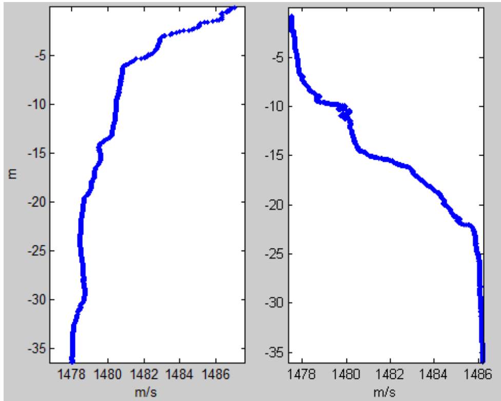
Figure 3.5. Typical summer (left) and winter (right) sound speed profiles [67]
