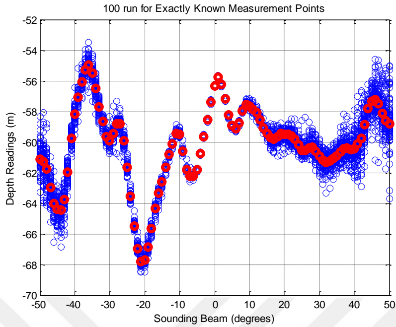
Figure 4.7. Measurement on exactly known positions conducted 100 times where ship movement/position effects are not included (red dots are absolute truth, blue dots are depth measurements)
