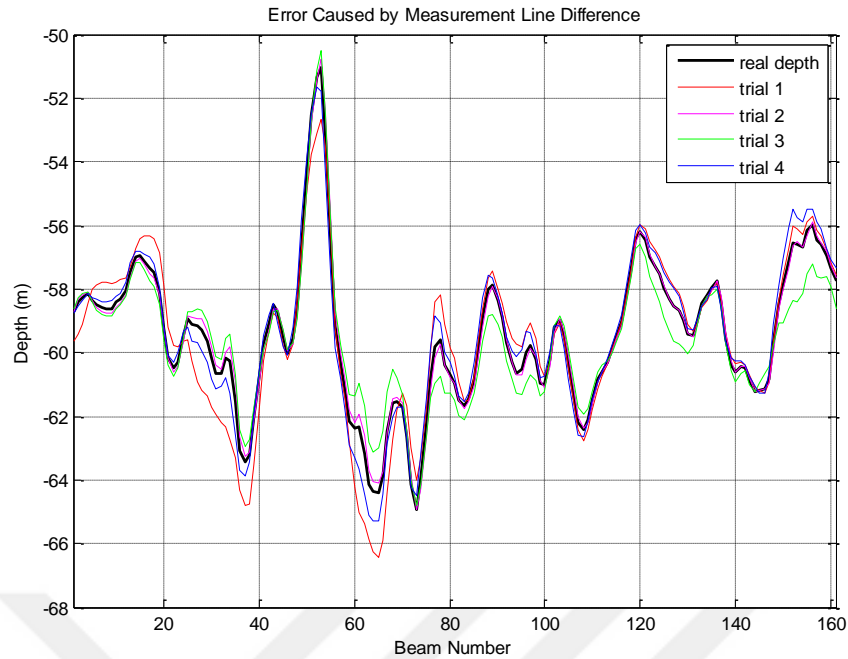
Figure 4.15. Error caused by measurement line difference [\sigma_x, \sigma_y, \sigma_{roll}, \sigma_{pitch}, \sigma_{yaw}] = [0.25, 0.25, 0.1, 0.1, 0.1]
