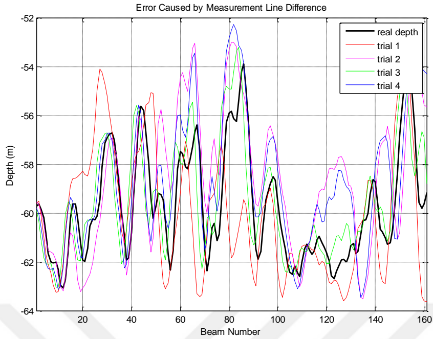
Figure 4.13. Error caused by measurement line difference [\sigma_x, \sigma_y, \sigma_{roll}, \sigma_{pitch}, \sigma_{yaw}] = [1, 1, 0.5, 0.5, 0.5]
