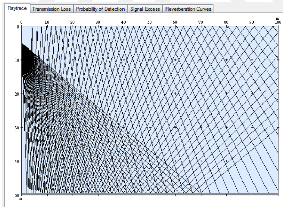
Figure 3.6. Straight rays in isovelocity water
