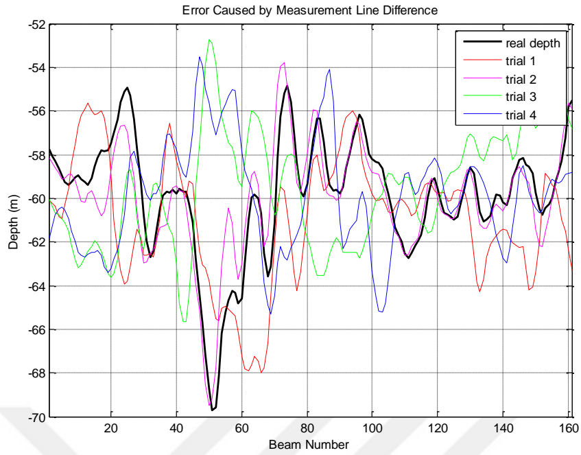
Figure 4.11. Error caused by measurement line difference [\sigma_x, \sigma_y, \sigma_{roll}, \sigma_{pitch}, \sigma_{yaw}] = [5, 5, 1, 1, 1]
