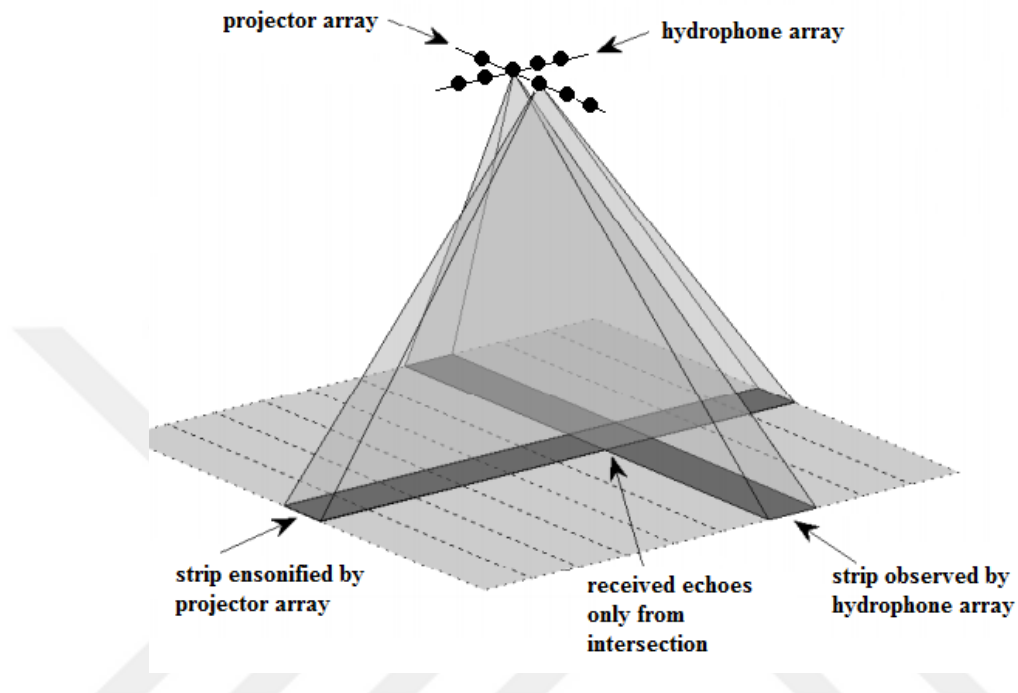
Figure 2.4. Mills cross arrangement of the projector and hydrophone arrays [63]
