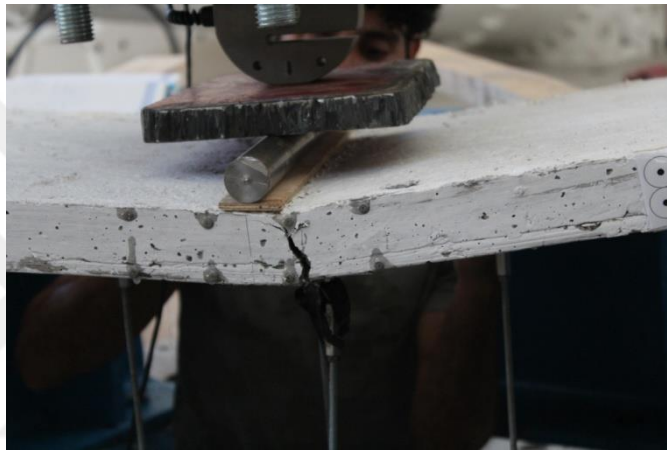
Figure 48: Final view of SA3+PVA after testing
