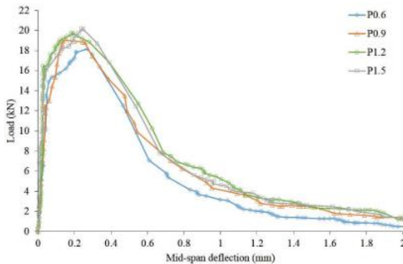
Figure 17: Load vs. mid-span deflection for composites with different PVA contents (Zhang et al. 2019).
