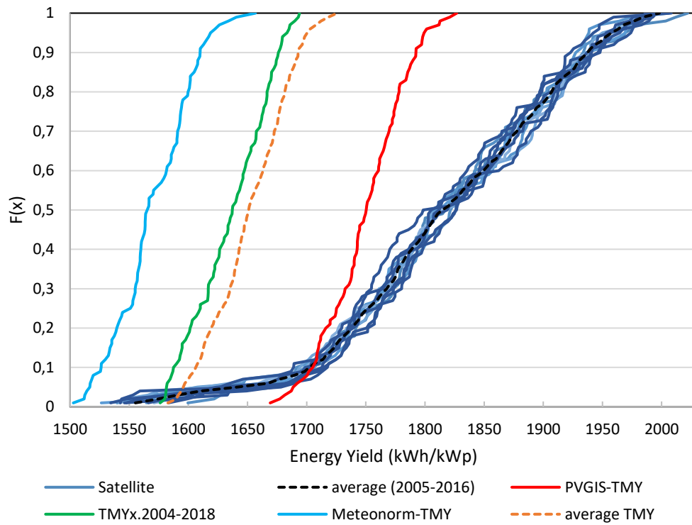
Figure 4.31. CDF of energy yields generated by stochastic simulation, using all uncertainty distributions given in Table 3.7.
