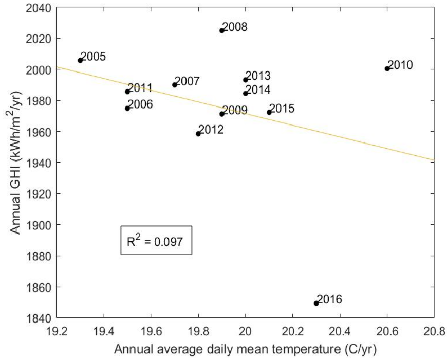
Figure 4.37. Correlation between annual GHI and annual average daily mean temperature between 2005-2016.
