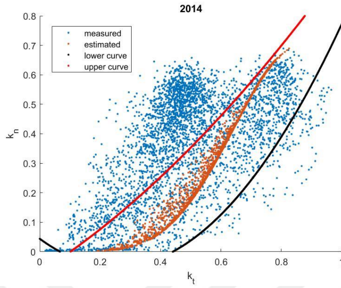
Figure 4.2. k_n - k_t quality envelopes for measured and estimated data with upper and lower boundary layers in 2014.
