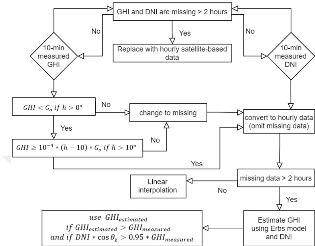
Figure 3.6. A flowchart of detecting erroneous GHI, filling missing data, and estimating GHI when it is needed.
