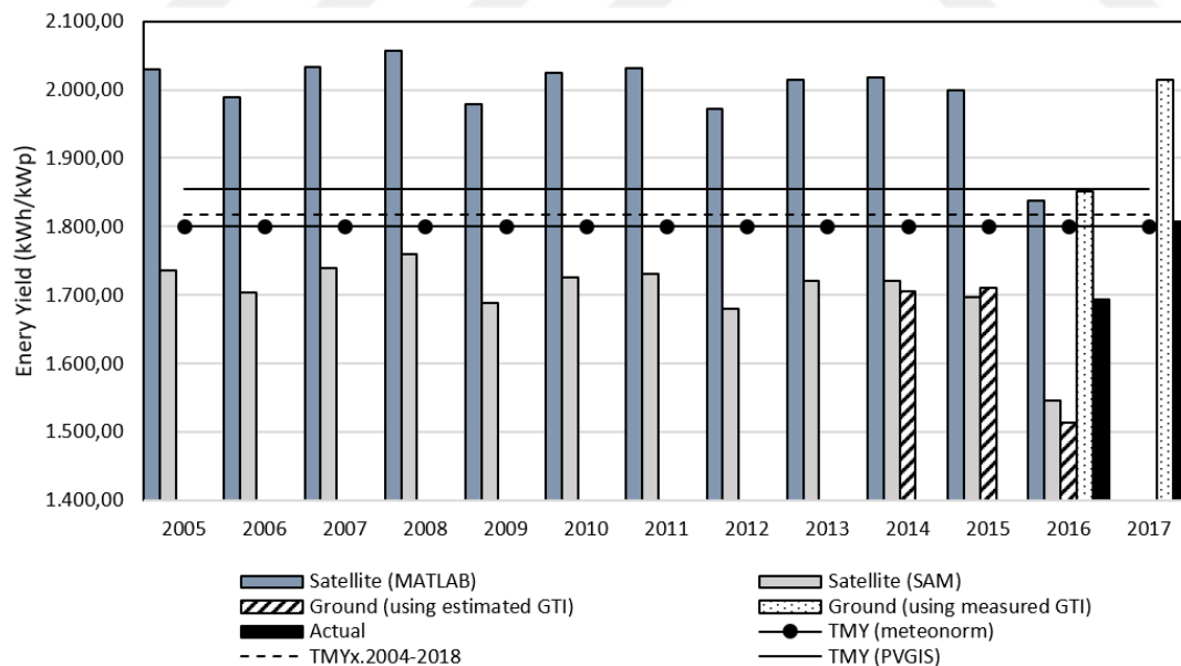
Figure 4.26. A comparison of satellite-based, ground-measured, TMY and actual energy yield results obtained from calculations and SAM simulations using isotropic sky-diffuse model.
