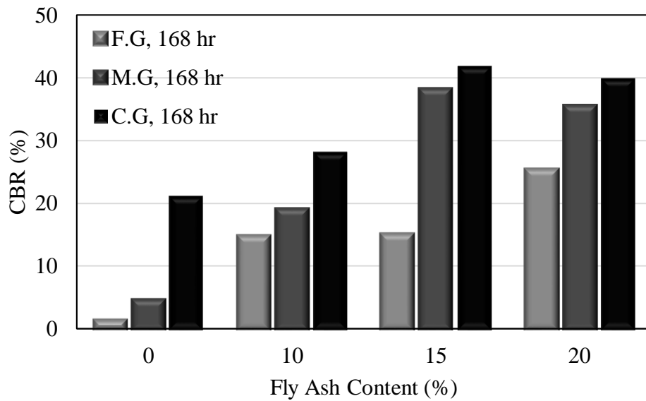
Figure 4.44 The Effect comparison of 10%, 15%, and 20% FA on CBR of F.G, M.G, and C.G soils in 168 hour curing time
