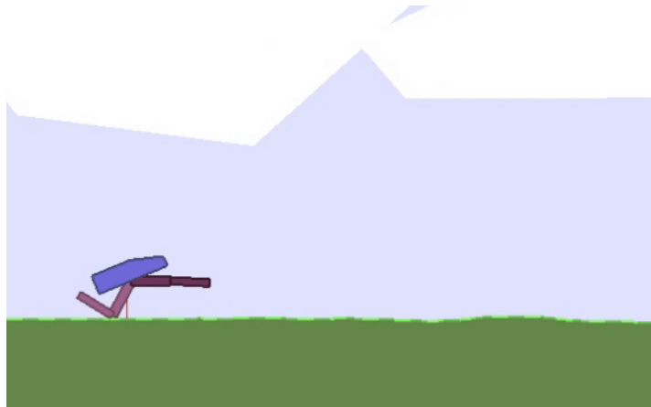
Figure 5.5 : BipedalWalker Environment
