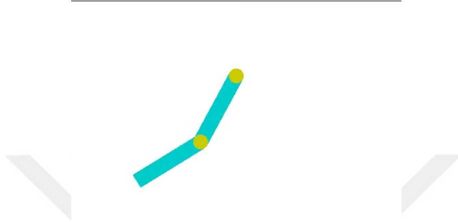
Figure 5.6 : Acrobot Environment
