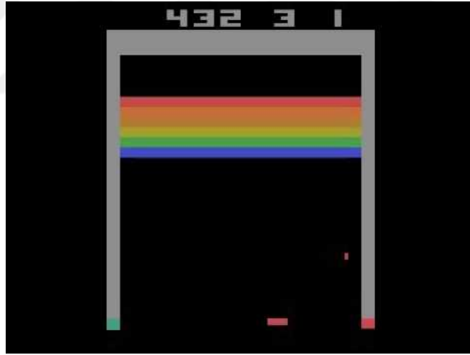
Figure 5.7 : Breakout Environment
