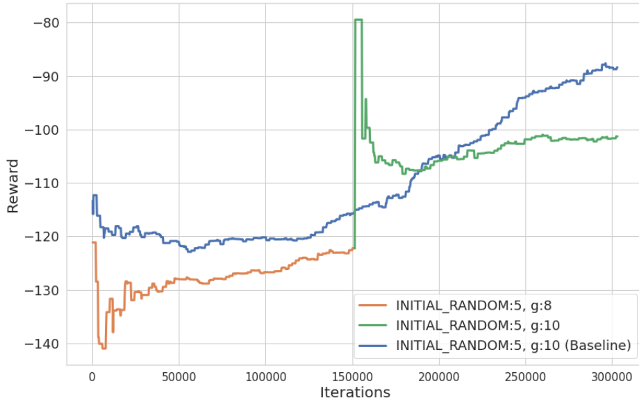
(b) The worst training result on BipedalWalker-v3.
