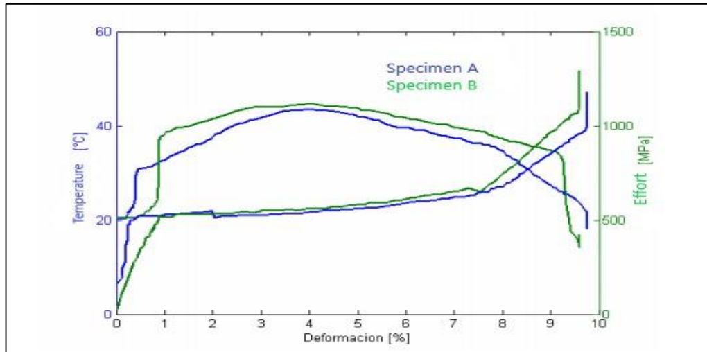
Figure 4.3. Stress vs. deformation and temperature vs. distortion.
