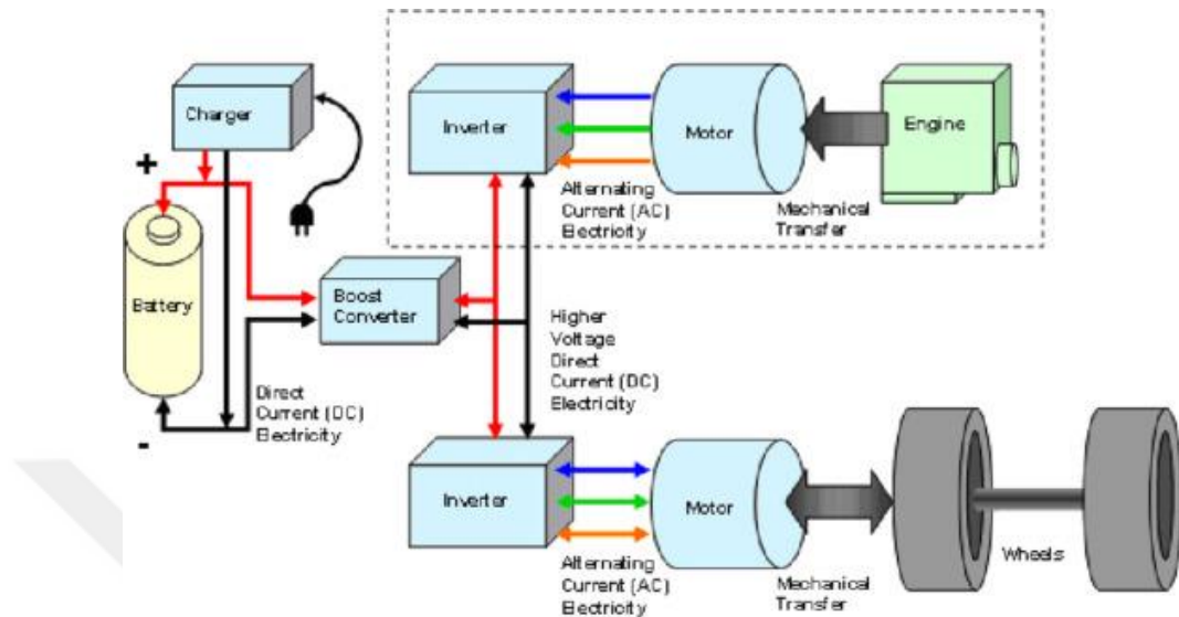
Figure 3.1. Block diagram of EV [53].
