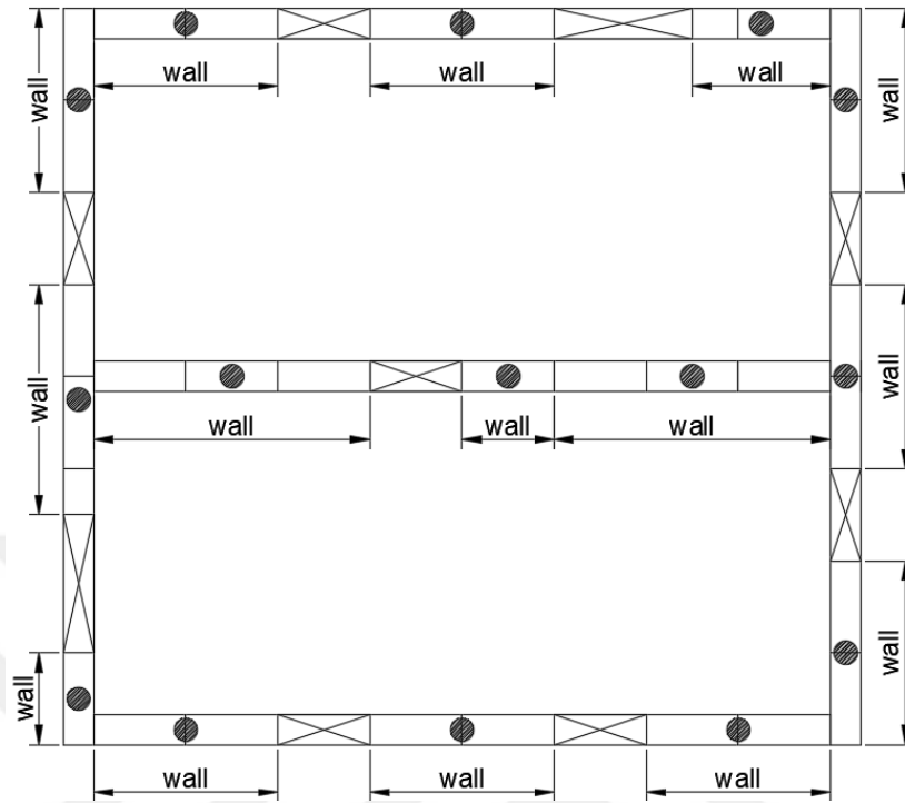
Figure 4.20: Modeling Details of Second Story Walls of the Project Building
