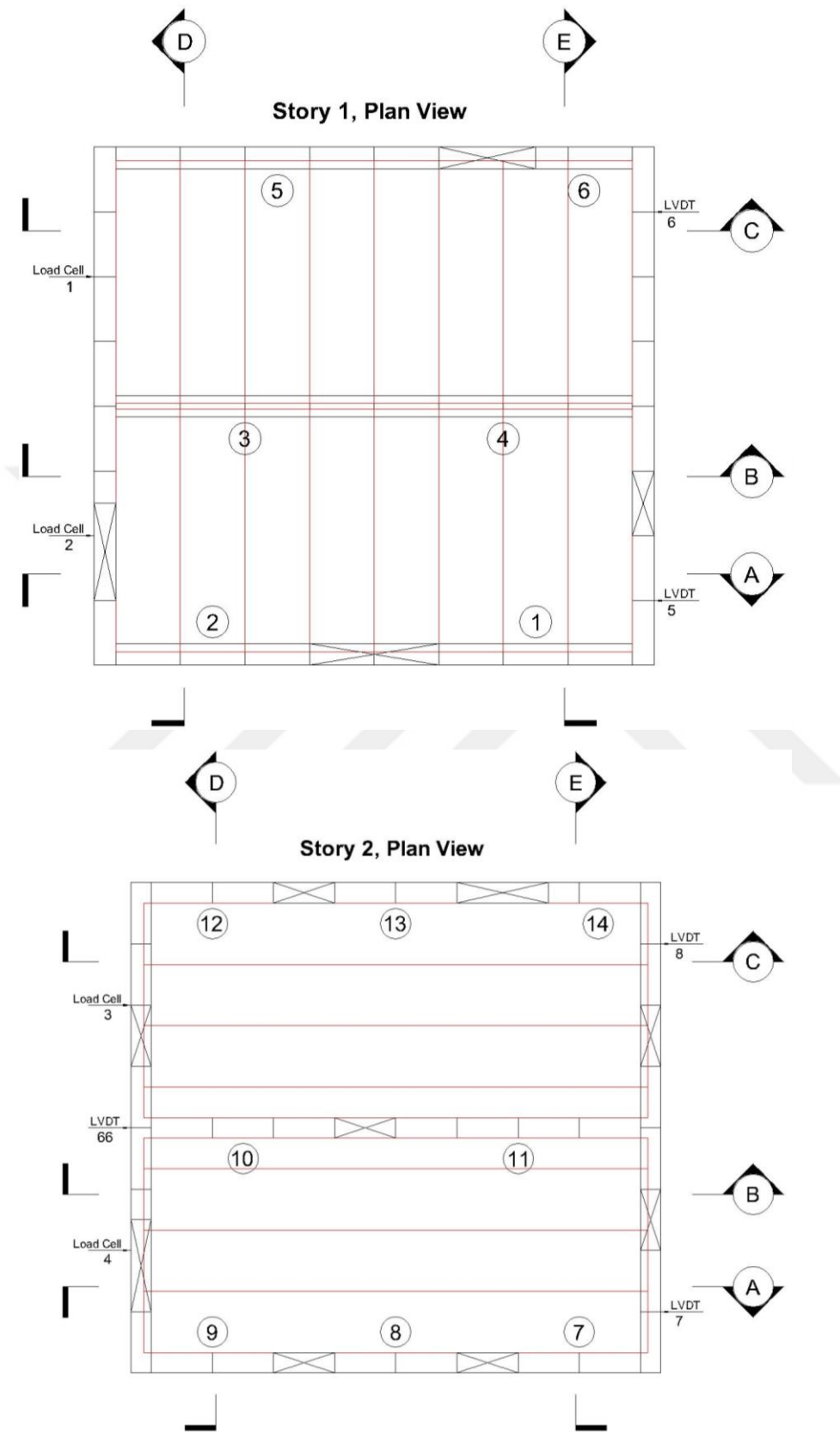
Figure 2.13: Plan Views of the Test Building
