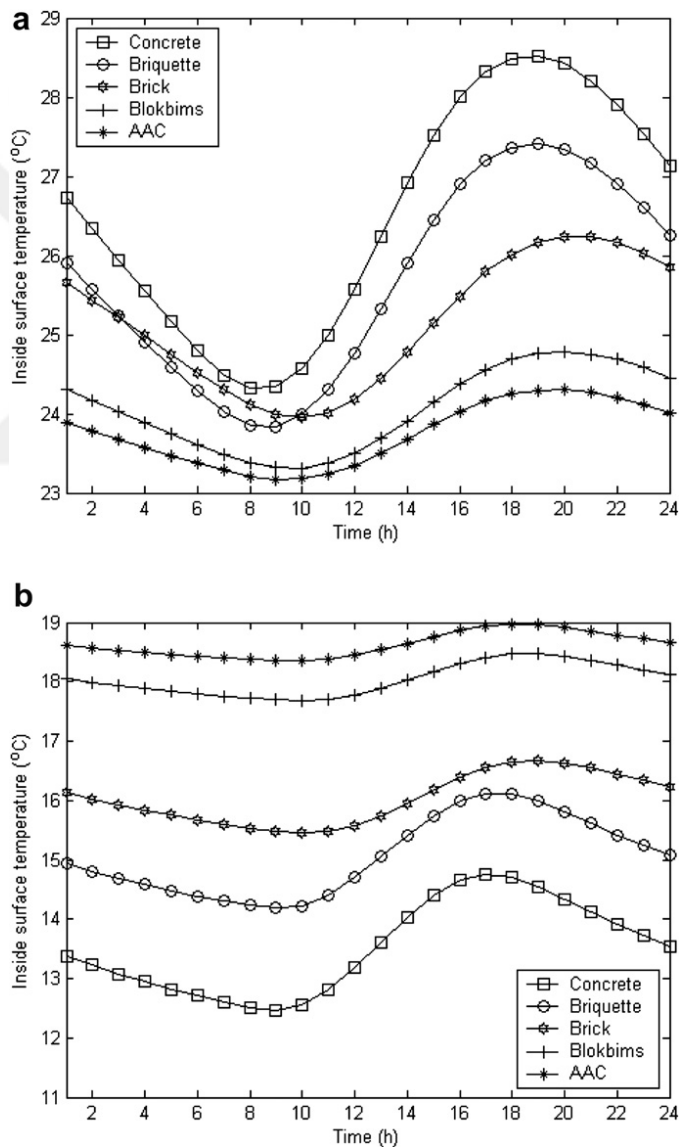
Figure 1.1: Hourly variation of inside surface temperatures of the uninsulated walls: (a) Summer (b) Winter
