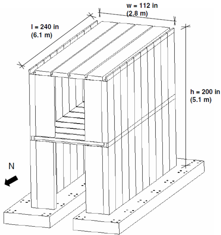
Figure 2.6: 3D view of Two-story Assemblage (Tanner, 2003)
