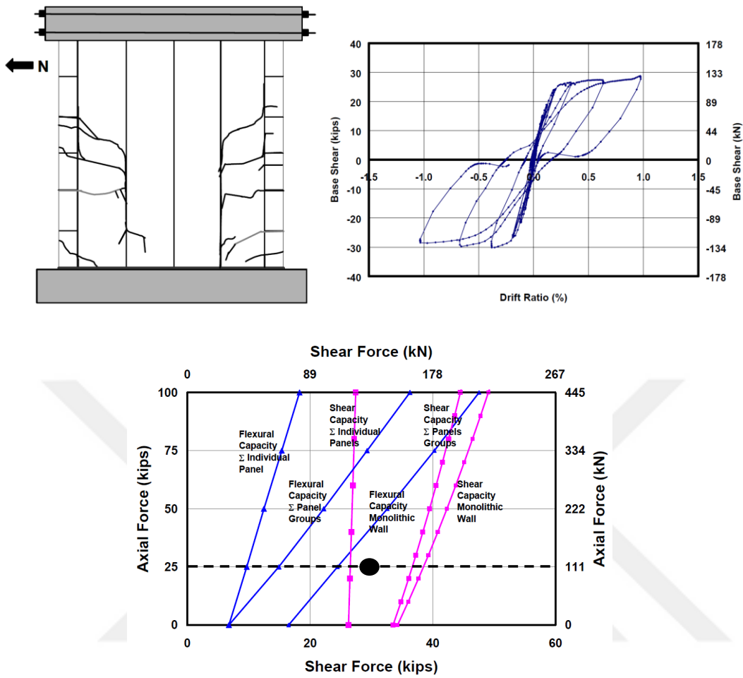
Figure 2.4: Specimen 15 Test Results (top two) & Capacity Curve for specimens 15a, 15b and 16 (bottom) (Tanner, 2003)
