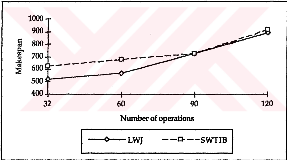
FIGURE 8.5.7. Makespan performances of LWJ and SWTIB in R4.
