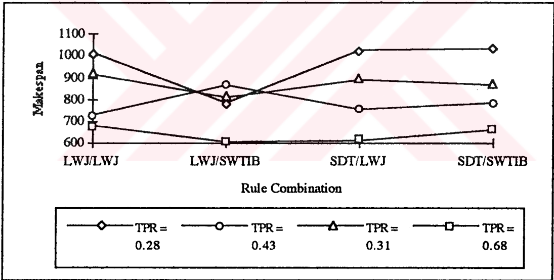
FIGURE 8.5.11. Makespan performances of LWJ/LWJ, LWJ/SWTIB, SDT/LWJ and SDT/SWTIB rule combinations in (R5/R6) while R4 is SWTIB
