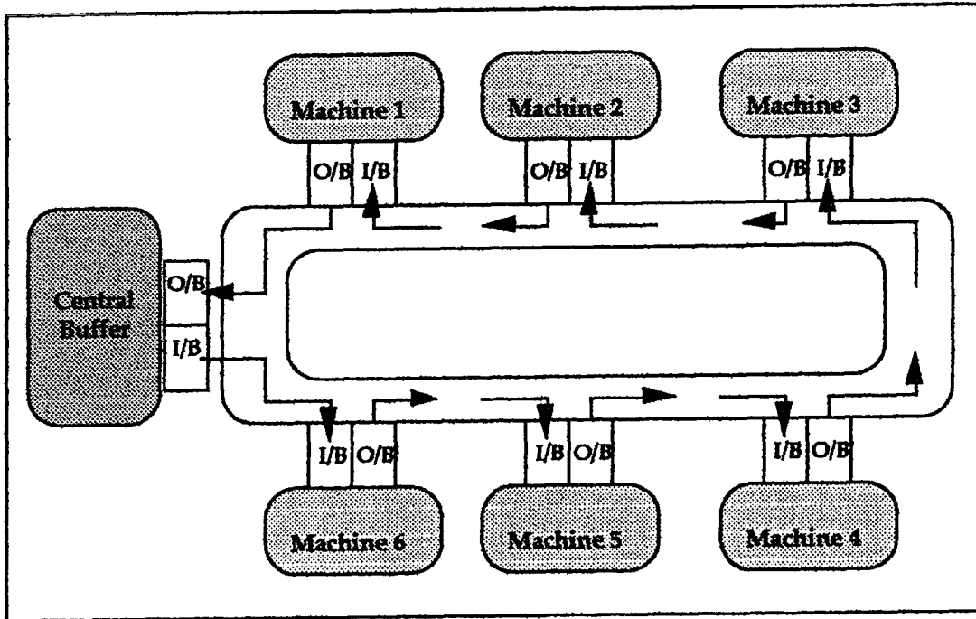
FIGURE 3.3.1. Layout of the hypothetical FMS (6 - machine case)
