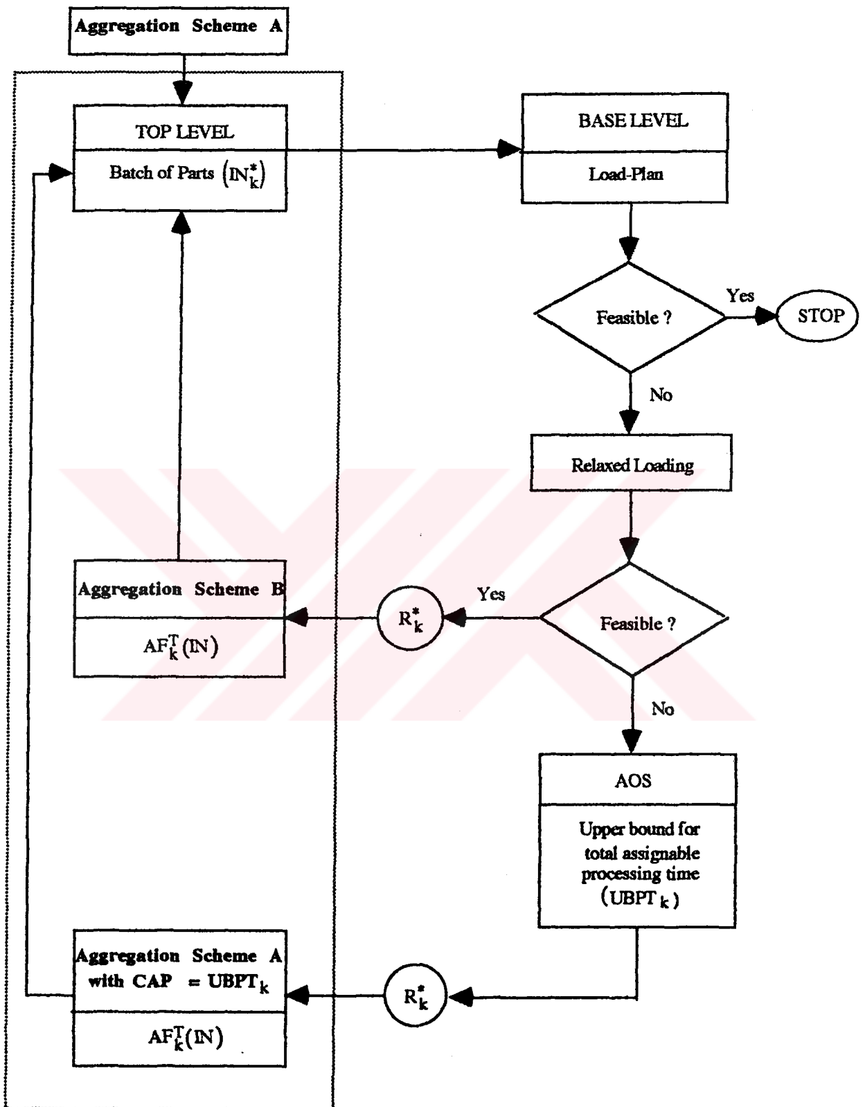
FIGURE 7.3.2.1. The flow-chart of the anticipation process
