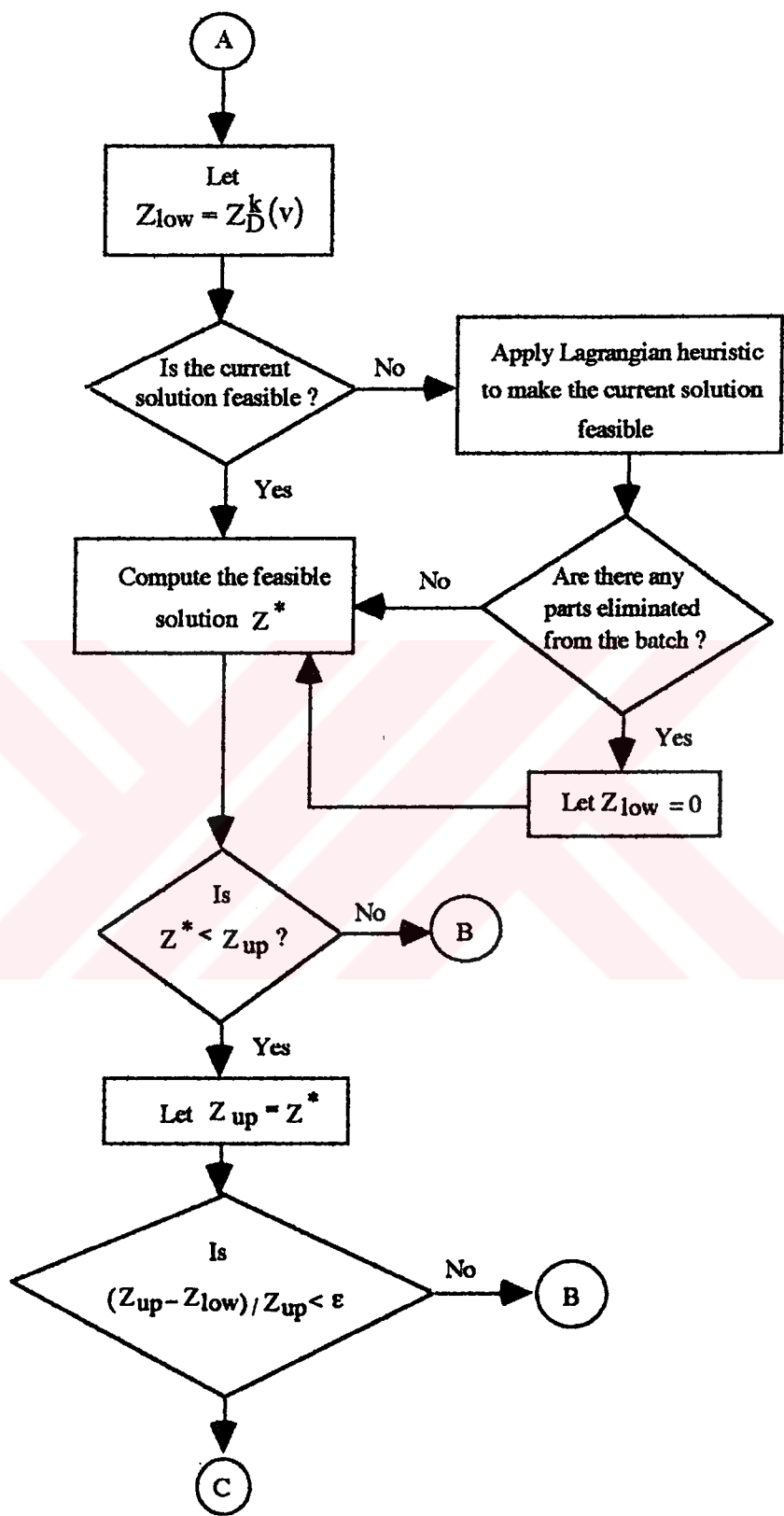
FIGURE 6.2.1. Subgradient optimization procedure to solve (RLM) (continued)
