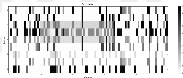
(a) Gibbs sampler.
