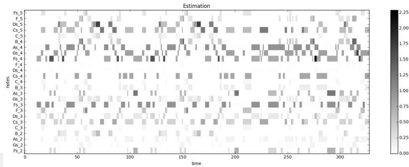
(a) Estimation for X by PF.
