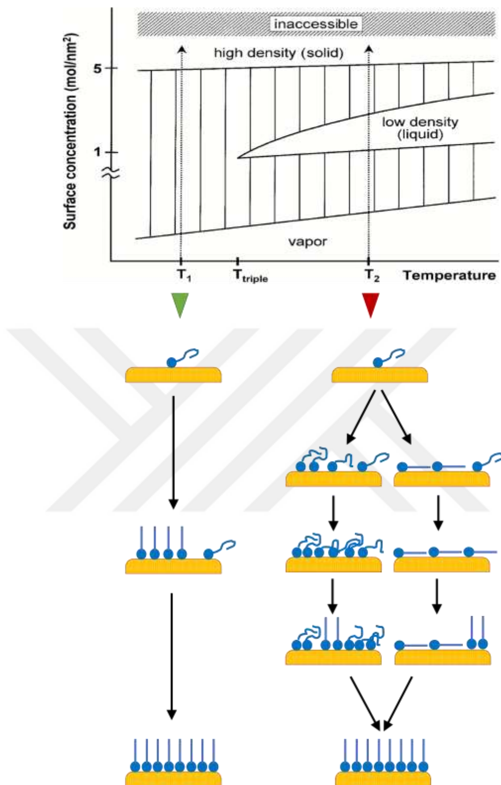
Figure 2-10: Schematic illustration of the differences in growth of a generic SAM system with respect to two hypothetical isothermal paths (at a temperature T_1 or T_2 ) indicated in the quasi-equilibrium phase diagram. Adapted from [147].
