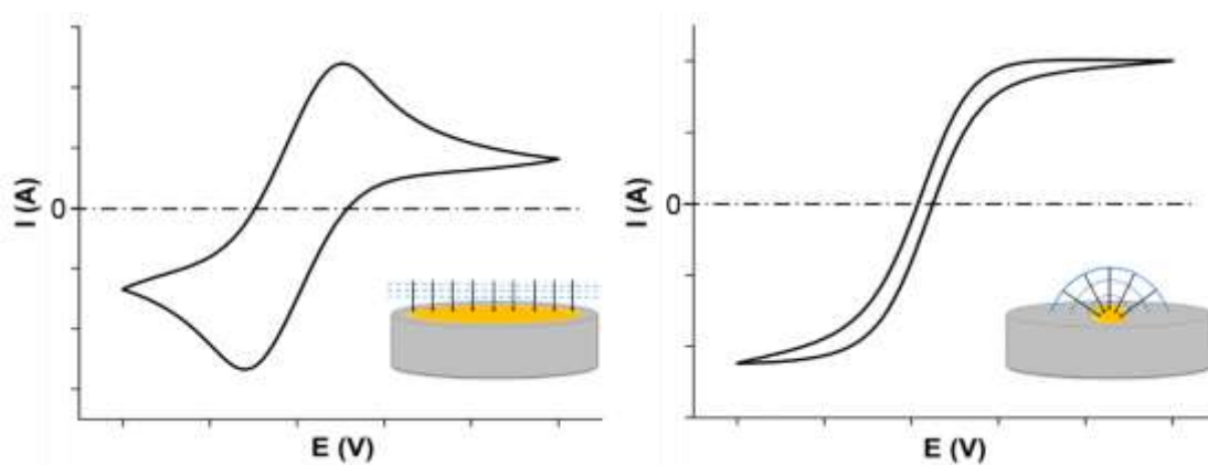
Figure 2-18: Characteristic CV responses of macro- and microelectrodes as a result of linear or hemispherical diffusion.
