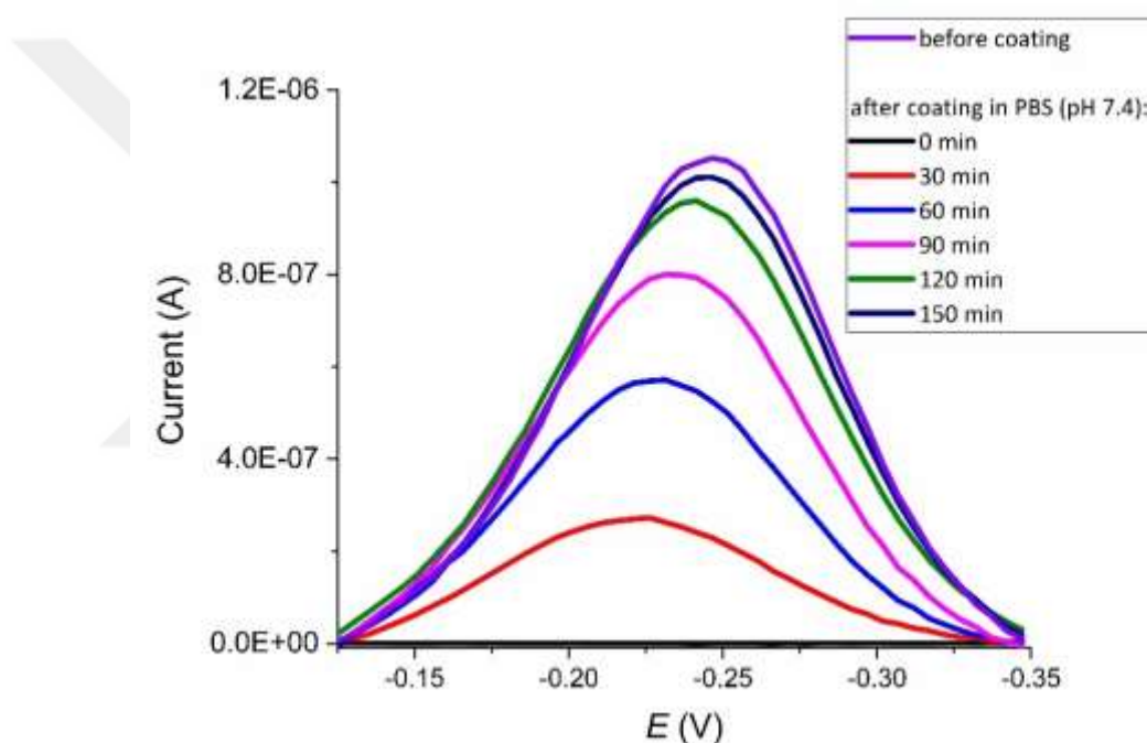
Figure 7-8: SWV curves recorded for an Au SPE modified with the Probe-1 and then coated with a single layer of the 16% Eudragit® followed by its immersion in 1x PBS.
