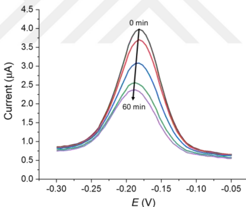
Figure 4-13: Typical background-subtracted SWV curves for a SAM-functionalised probe substrate immobilised onto Au macroelectrode registered for 100 nM trypsin at different incubation times (0, 5, 15, 35 and 60 min) in 1x PBS. Adapted from [7].
