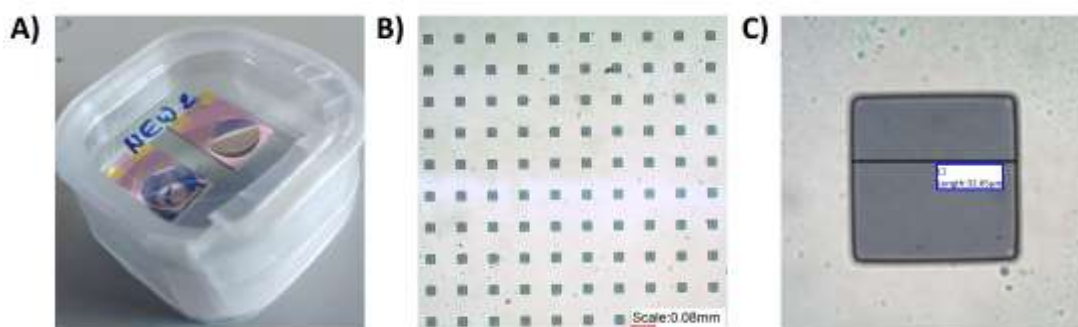
Figure 5-21: A) Macroscopic image of two individual and identical (left: Electrode-1, right: Electrode-2) NanoFlex Microcavity Nanoband Edge Electrode (MNEE) arrays incubated with 40 \mu\text{M} of probe solution by drop-casting. Optical microscope images show B) the array of 10 x 10 electrodes and C) a single microsquare cavity of 30 \mu\text{m} x 30 \mu\text{m} and a 50 nm Pt nanoband at the edge of the cavity.
