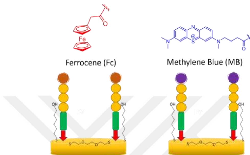
Figure 4-6: Representation of two different probe structures with different redox tags attached, ferrocene (Fc) and methylene blue (MB) as well as their chemical structures.
