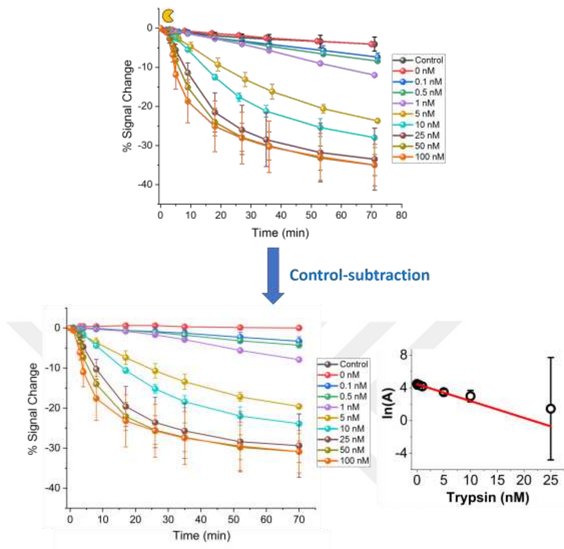
Figure 4-14: Top: Plot of % signal change vs time for SAM-functionalised probe immobilised onto Au macroelectrodes immersed in varying trypsin concentrations in PBS (0, 0.1, 0.5, 1, 5, 10, 25, 50, 100 nM for substrate probe and 100 nM for the negative control probe, containing D-amino acids). All data represent the average (and standard deviations) from (typically) 3 functionalised electrodes. Bottom left: The data recorded for the negative control subtracted from the others. Bottom right: Natural logarithm of A(\%) , after 70 min plotted against the concentration of trypsin. The straight line corresponds to the best linear regression fit ( \ln A = -0.21 [\text{trypsin}/\text{nM}] + 4.46 ; r^2 = 0.87 ). The points of [\text{trypsin}] = 50 and 100 nM were not included in the fit due to that A(t) = 0 and having large replicate error compared to the other concentrations. Adapted from [7].
