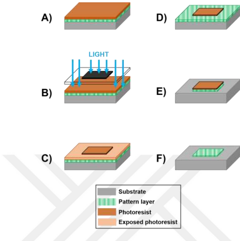
Figure 3-7: The photolithography and etching process. A) Positive photoresist layer is coated on a material to be patterned and B) exposed to UV light through a photomask, leading to C) a patterning of exposed and unexposed photoresist areas and D) the development and thus removal of the exposed photoresist from the substrate. E) Residual pattern of photoresist is used as a protecting layer in the selective etch of the underlying material and then F) removed, leaving the patterned material.
