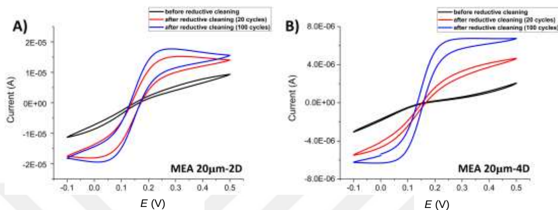
Figure 5-16: Reductive electrochemical removal of SAM-functionalised probes: CVs of a A) MEA 20µm-2D and B) MEA 20µm-4D recorded between -0.1 and +0.5 V at a scan rate of 100 mV.s -1 in an aqueous solution of 1 mM potassium ferri/ferrocyanide and 0.1 M KCl vs Ag/AgCl reference electrode, before reductive cleaning (black line) or after 20 cycles of reductive cleaning (red line) or after 100 cycles of reductive cleaning (blue line).
