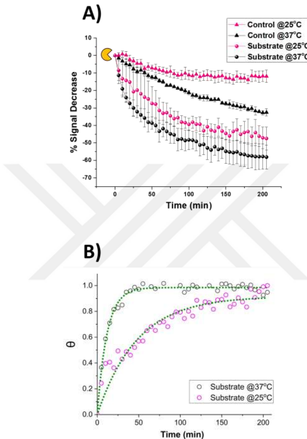
Figure 4-32: (A) Comparative signal decrease vs time curves registered for the miniaturised sensor upon the addition of 100 nM trypsin in 1x PBS at 25 °C (pink) and 37 °C (black) for both control-(triangle) and substrate-modified (circle) microelectrodes. (B) Calculated fractional cleavage, \theta , vs time plots for control-subtracted substrate data from (A). The data points correspond to temperatures of 25 °C (magenta) and 37 °C (black) whilst the green dotted lines show the best iterative fits to equation (1) with k_{\text{eff}} = 0.021 \pm 0.002 \text{ min}^{-1} and 0.082 \pm 0.004 \text{ min}^{-1} respectively.
