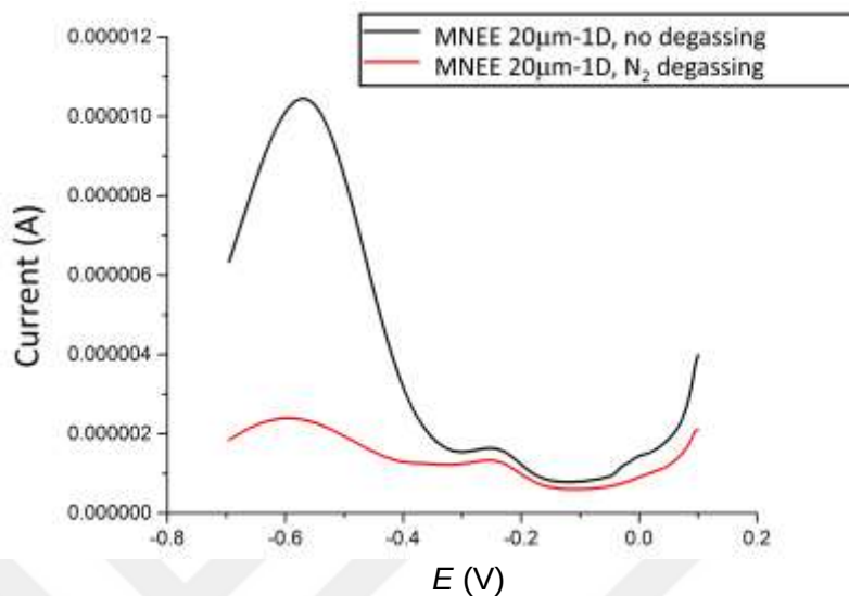
Figure 5-27: Typical SWVs with an extended potential window (-0.7 to +0.1 V) for substrate-modified probe immobilised MNEE 20μm-1D before and after degassing 1x PBS solution with N_2 .
