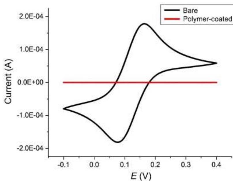
Figure 7-4: CVs of Au SPE recorded in 5 mM potassium ferri/ferrocyanide in 1x PBS, before (black) and after (red) coated with a single layer of 16% Eudragit® S100. CVs were recorded between potentials of -0.1 and +0.4 V at a scan rate of 100 mV/s.
