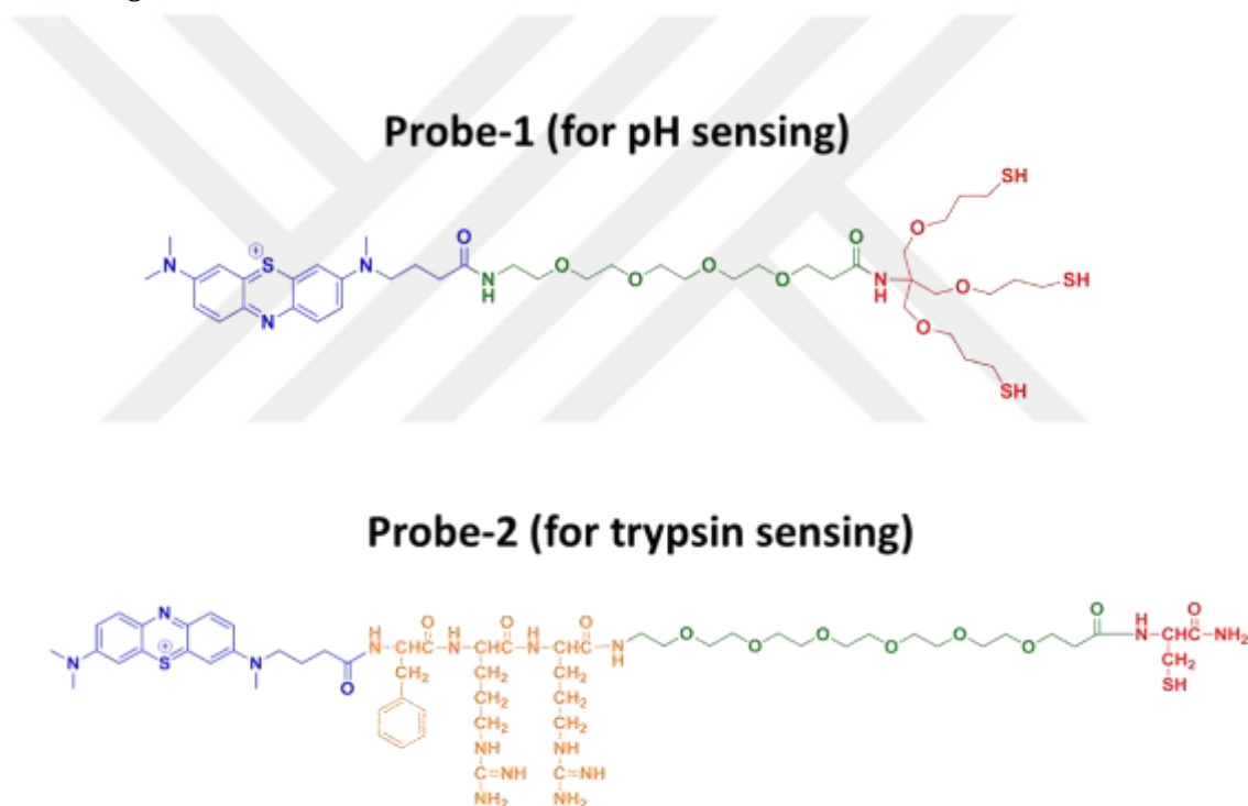
Figure 7-7: Chemical structures of the probes used for pH (Probe-1) and trypsin (Probe-2) sensing. Probe-1 contains methylene blue (blue) as the redox tag, PEG-4 as the spacer and tripod anchor (red) [361]. As detailed in Section 4-2, Probe-2 contains methylene blue (blue) as the redox tag, attached to Phenylalanine-Arginine-Arginine (orange) as the peptide sequence and PEG-6 (green) as the spacer and cysteine (red) as the anchor.
