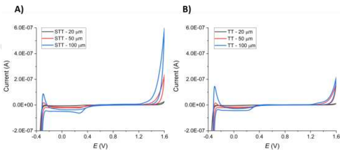
Figure 5-1: CVs of Pt A) superthin track (STT) and B) thin track (TT) microelectrodes of various sizes recorded in 0.1 M \text{H}_2\text{SO}_4 between -0.35 and +1.6 V at a scan rate of 100 \text{ mV}\cdot\text{s}^{-1} . Each scan corresponds to the 20 th cycle of electrochemical cleaning.
