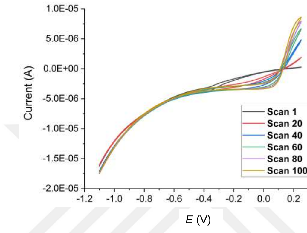
Figure 5-15: Reductive electrochemical removal of SAM-functionalised probes: Typical CVs (1st, 20th, 40th, 60th, 80th and 100th scans) of a MEA 20 \mu m-2D recorded between -1.1 and +0.25 V at a scan rate of 100 mV.s -1 in an aqueous solution of 1 mM potassium ferri/ferrocyanide and 0.1 M KCl.
