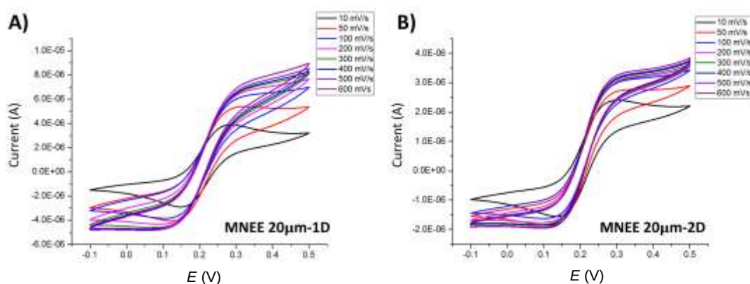
Figure 5-23: A) Typical CVs of in-house built A) MNEE 20 \mu m-1D and B) MNEE 20 \mu m-2D recorded between -0.1 and +0.5 V at varying scan rates (10, 50, 100, 200, 300, 400, 500 and 600 mV.s -1 ) in an aqueous solution of 0.5 mM ferrocene methanol and 0.1 M KCl.
