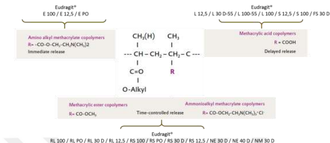
Figure 7-1: Chemical structures of Eudragit® polymers and their enabling of various types of drug release. Adapted from [362].
