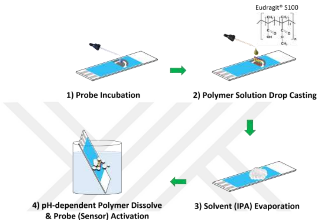
Figure 3-13: Representation of the modification and activation of a probe-modified screen-printed electrode surface with a pH responsive, transient polymeric coating of Eudragit® S 100.
