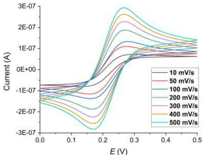
Figure 5-4: CVs of STT 100 \mu\text{m} recorded with varying scan rates (10, 50, 100, 200, 300, 400 and 500 \text{mV.s}^{-1} ) in 5 mM potassium ferri/ferrocyanide in 1x PBS between 0 and +0.5 V.
