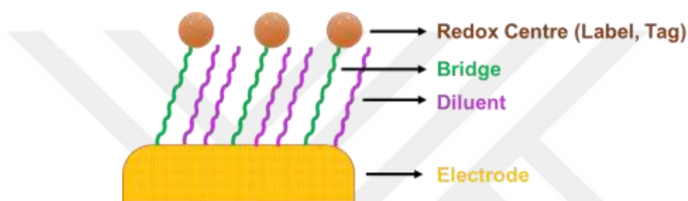
Figure 2-12: The structure of redox-active SAM molecules. Adapted from [176].
