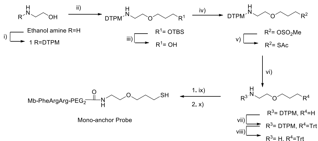
Figure 3-3: Synthesis of mono-anchored redox-labelled peptide probe. Reaction conditions: i) DTPM-NMe 2 , MeOH, overnight; ii) (3-Bromopropoxy)-tert-butyldimethylsilane, NaH, DMF, 24 h; iii) TBAF, THF, overnight; iv) MeSO 2 Cl, Et 3 N, DCM, 3 h; v) KSAc, anhydrous THF, overnight; vi) HCl/MeOH (1/4), 3 h, reflux; vii) triphenyl methanol, TFA, overnight; viii) hydrazine monohydrate, anhydrous THF, 1 h; ix) redox-labelled peptide product (MB-Phe-Arg-Arg-PEG-2-COOH, Figure 3-2), HOBt, EDC, DMF, 24 h; x) TFA/EDT/water/TIS, 30 min [197].
