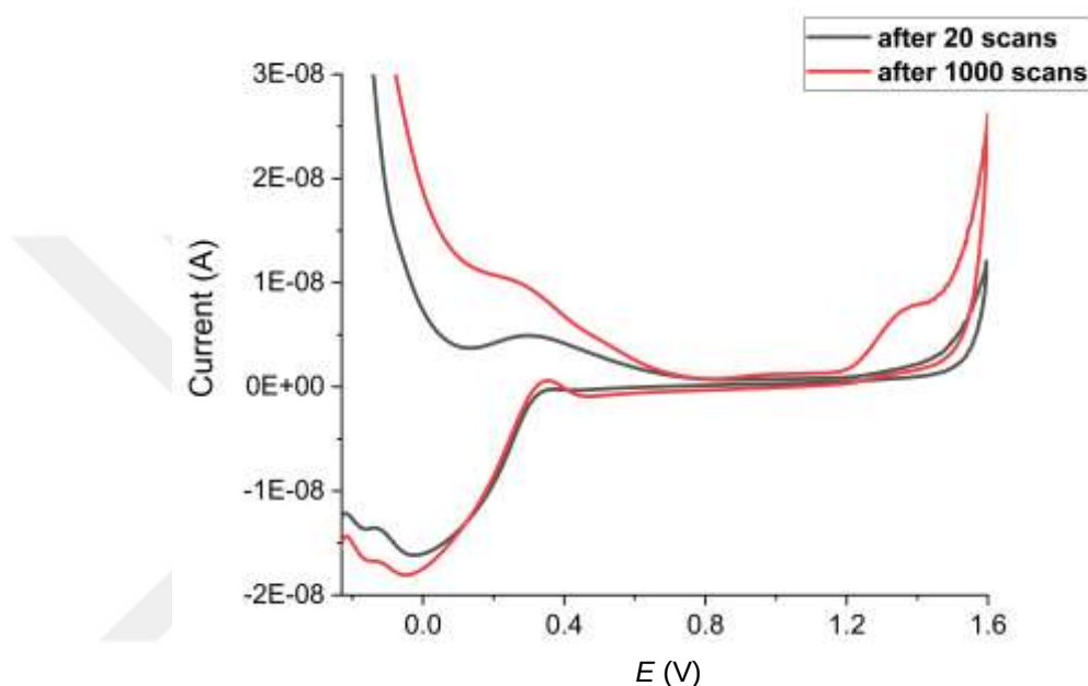
Figure 5-2: Comparative cleaning CVs of Pt TT 20 \mu\text{m} recorded after 20 (black line) or 1000 (red line) scans in 0.1 \text{ M H}_2\text{SO}_4 between -0.35 and +1.6 \text{ V} at a scan rate of 100 \text{ mV.s}^{-1} .
