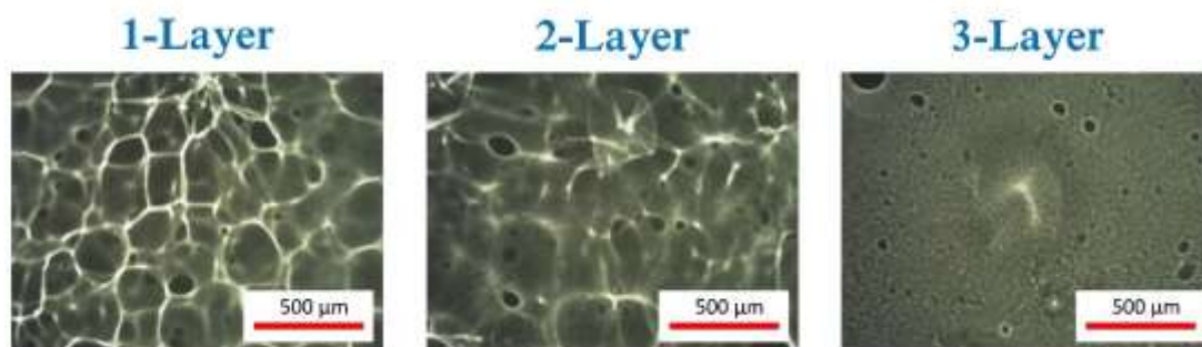
Figure 7-9: Optical microscope images of Au SPEs drop-cast with consecutive layers (1-Layer, 2-Layer and 3-Layer) using 10 \mu\text{L} of 16% (w/v) of the Eudragit® S100 polymeric solution for each layer.
