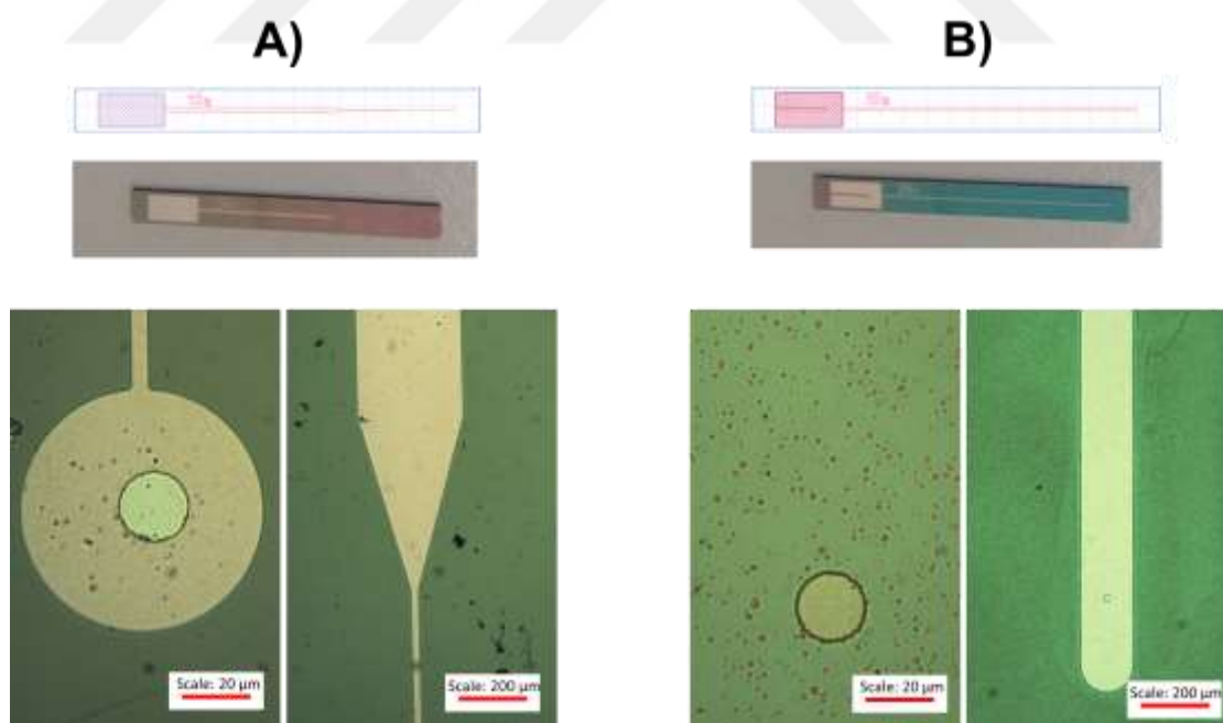
Figure 3-9: Top: mask designs used for photolithography process and photographs of in-house fabricated single disc microelectrodes with 20 \mu\text{m} -diameter; A) superthin track and B) thin track devices. Lower: optical microscopy images of the electrodes and contact tracks.
