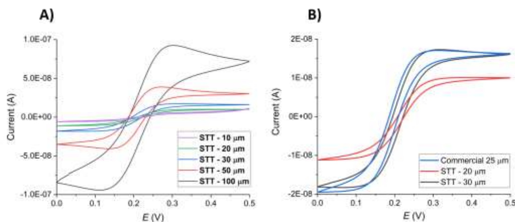
Figure 5-3: CVs of various Pt microelectrodes of different diameters recorded in 5 mM potassium ferri/ferrocyanide in 1x PBS between 0 and +0.5 V at a scan rate of 100 \text{ mV.s}^{-1} : A) STT (10, 20, 30, 50 and 100 \text{ }\mu\text{m} ) and B) commercial ( 25 \text{ }\mu\text{m} ) and STT ( 20 \text{ }\mu\text{m} and 30 \text{ }\mu\text{m} ).
