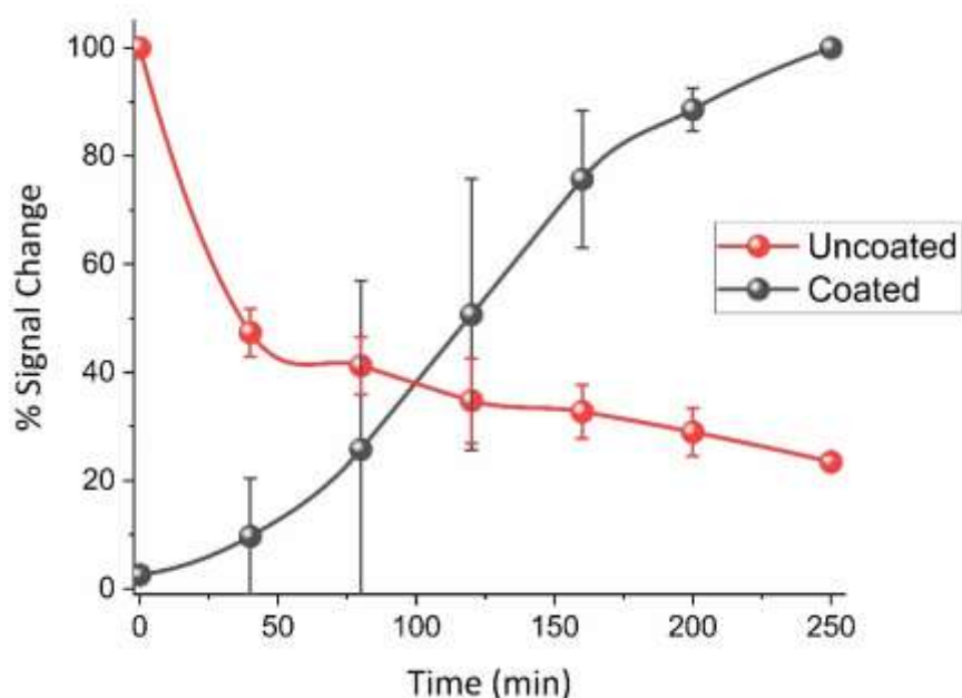
Figure 7-15: % Signal changes registered for the polymer-coated (with a single layer of 16% Eudragit®) and uncoated trypsin sensors (Au SPEs modified with Probe-2) in DMEM inc. 10% FBS.
