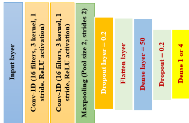
Figure 3.11. The 1D CNN architecture is used in this thesis
