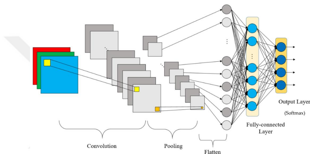
Figure 2.6. CNN Layers
