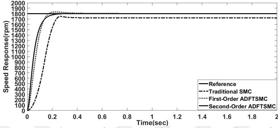
Figure 5.38. Speed responses for the traditional SMC with signum function, first-order ADFTSMC and second-ADFTSMC for set point 1800 rpm, adaptive fault gain \eta = 0.5
