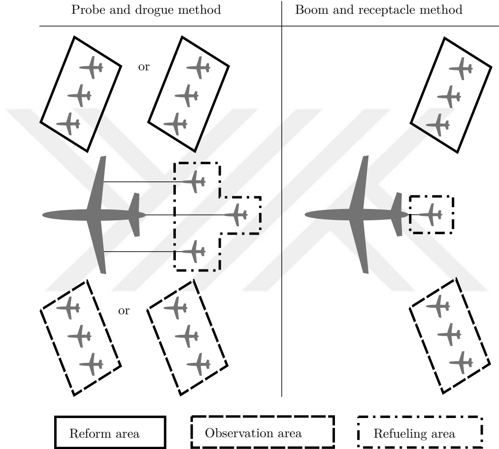
Figure 1.1: Formation flying positions during aerial refueling according to the procedures described by NATO [9]. View from above. For the probe and drogue method, the rear observation and reform areas are used, if there is an observer aircraft behind the tanker-receiver formation.
