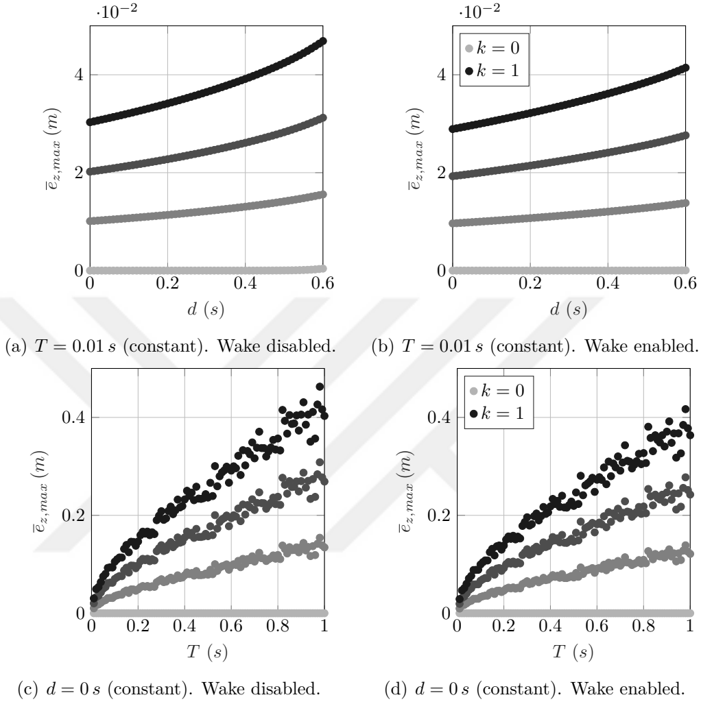
Figure B.10: Variation of \bar{e}_{z,max} with parameters k , d and T on lower-scale aircraft, without and with wake vortex effects. k = \{0, 0.3, 0.6, 1\} . The legend shows only the uppermost and lowermost values from the k -set.
