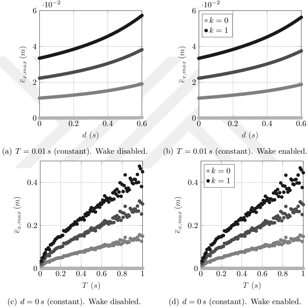
Figure B.9: Variation of \bar{e}_{x,max} with parameters k , d and T on lower-scale aircraft, without and with wake vortex effects. k = \{0, 0.3, 0.6, 1\} . The legend shows only the uppermost and lowermost values from the k -set.
