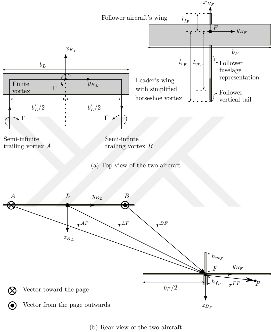
Figure 6.1: Aircraft geometries and reference frames used for vortex effect modeling.
