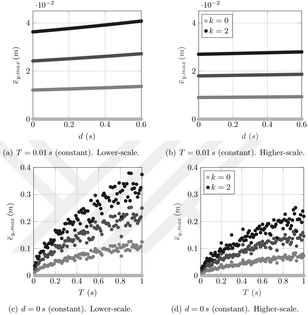
Figure 7.9: Variation of \bar{e}_{y,max} with parameters k , d and T for lower-scale and higher scale aircraft. Results belong to the simulations with disabled wake vortex effects. k = \{0, 0.6, 1.3, 2\} . The legend shows only the uppermost and lowermost values from the k -set.
