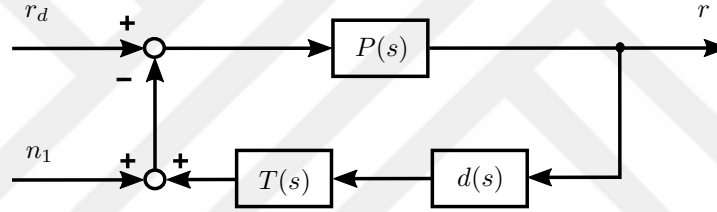
Figure 8.4: Formation flight dynamics as transfer function block diagram, with new error signal n_1 .
