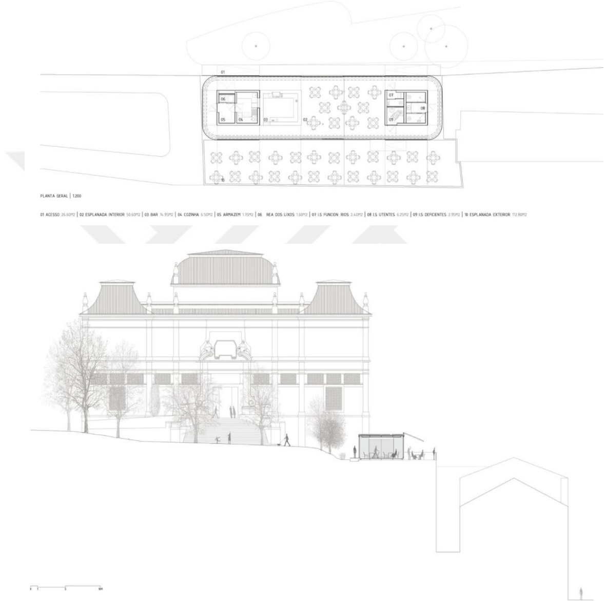
Şekil 4.82. The 9 April Garden'a ait plan ve kesit (ArchDaily, 2011c)
