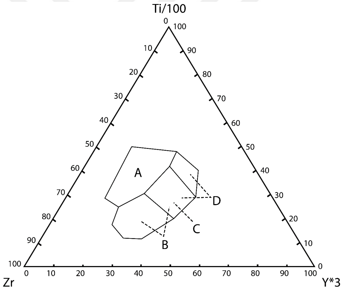
Figure 1.18. Discrimination diagrams of Pearce and Cann (1973) using Ti/100-Zr-Y*3
