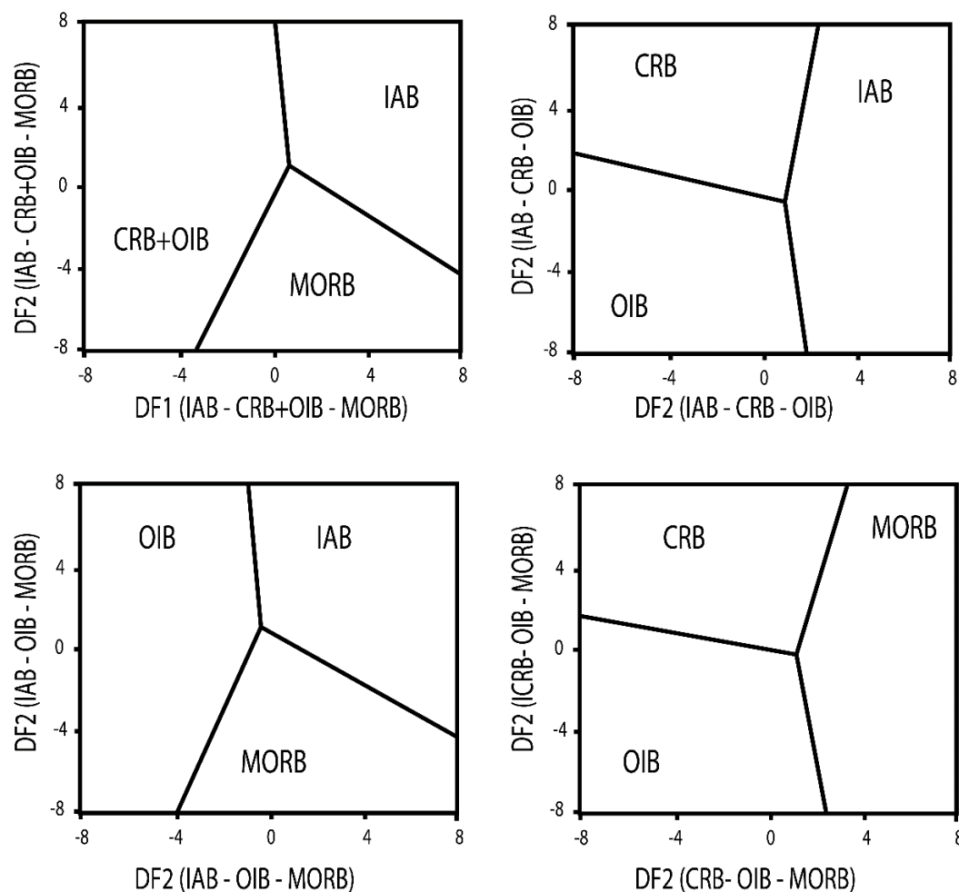
Figure 1.31. Representative discrimination diagrams from Verma and Agrawal et al. (2011)
