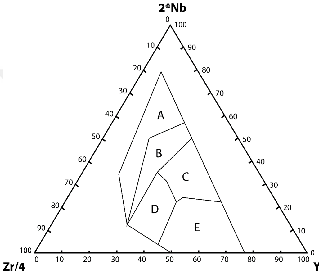
Figure 1.22. Discrimination diagram of Meschede (1986) using 2 \cdot \text{Nb} , \text{Zr}/4 and \text{Y}
