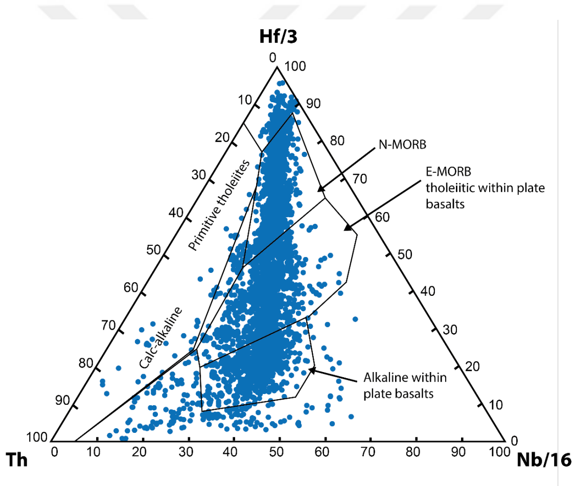
Figure 4.9. Samples of non-subduction settings plotted on Wood (1980) diagram
