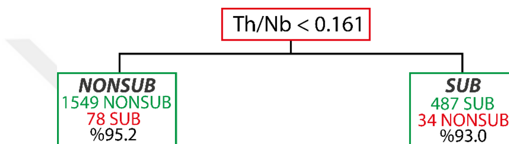
Figure 3.35. Classification results of the decision stump to discriminate between subduction and non-subduction settings
