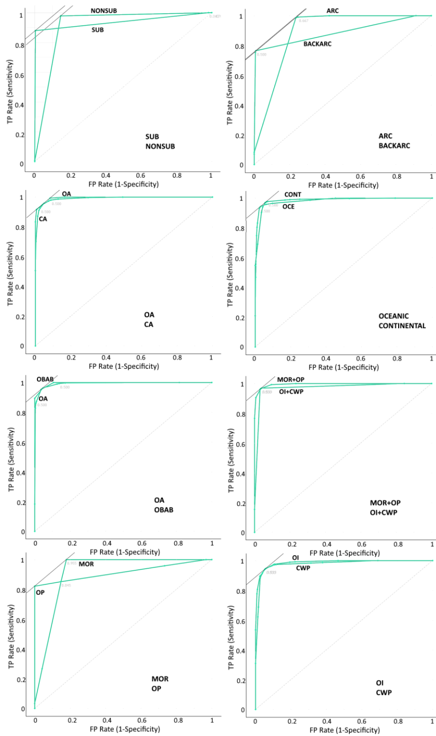
Figure 4.4. ROC for tectonic discriminations
