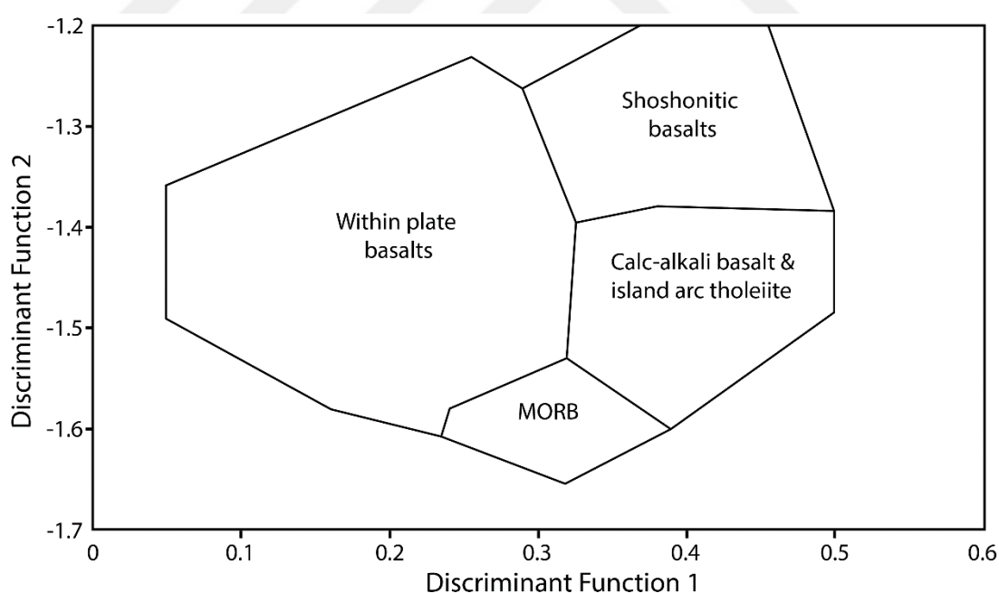
Figure 1.24. Discrimination diagrams of Pearce (1976) using DF1 and DF2
