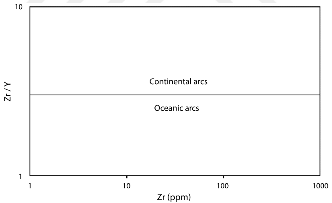
Figure 1.12. Bivariate diagrams by Pearce (1983) using Zr versus Zr/Y
