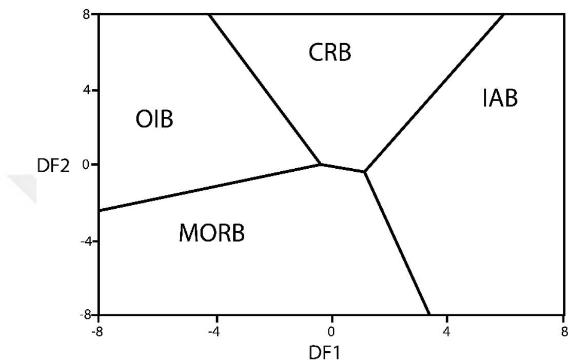
Figure 1.29. Representative discrimination diagram from Verma et al. (2006)
