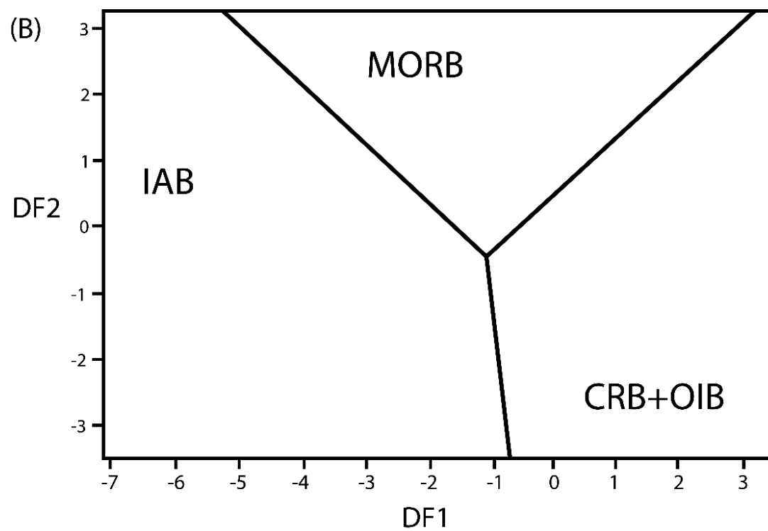
Figure 1.27. Discrimination diagrams of Velikoslavinsky and Kykrylov (2014) using discrimination functions of (A) by major element contents, (B) by inert minor element contents
