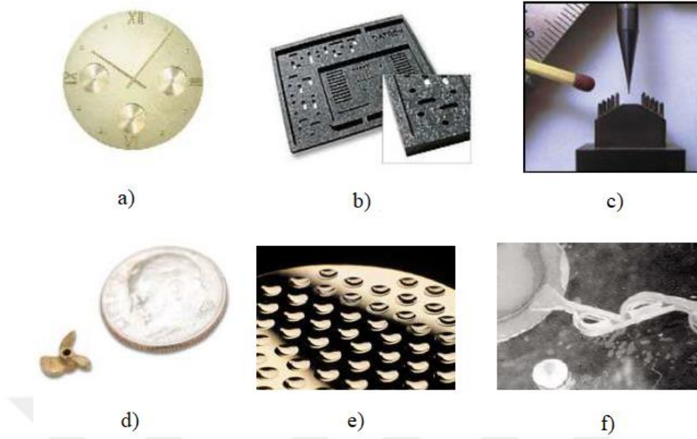
Resim 1. 2 Mikro frezelenmiş ürünlerin örnekleri a) Hassas Kol Saati Kadrani (Wu 2012, İnt. Kyn. 3), b) Lehim Çerçevesi (Wu 2012, İnt. Kyn. 4), c) Mikro Elektrot (Wu 2012, İnt. Kyn. 5), d) Mikro Pervane (Wu 2012, İnt. Kyn. 6), e) Gofret Desenli Optik (Wu 2012, İnt. Kyn. 7), f) Mikro Kapakçık (Wu 2012, İnt. Kyn. 8).
