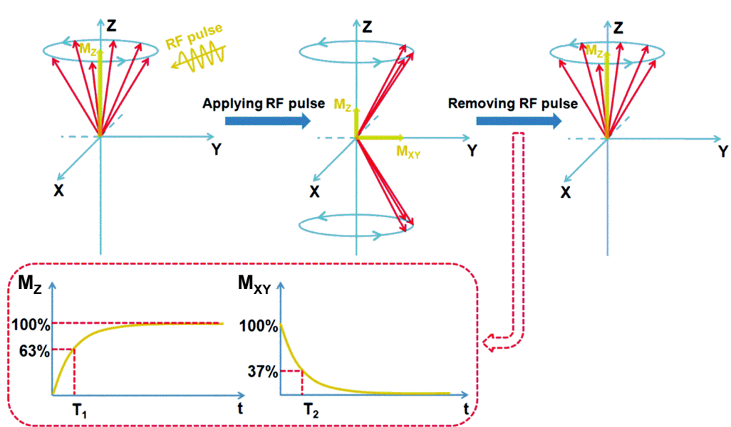
Figure 1.2: NMR relaxation times
