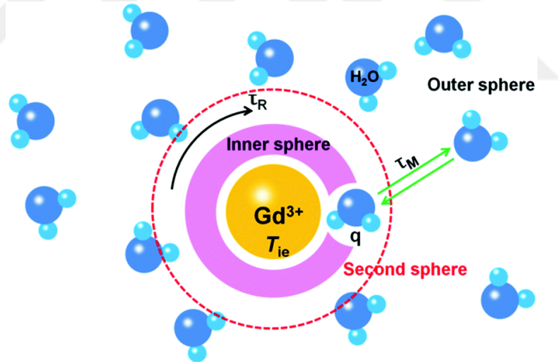
Figure 1.3: Inner and outer sphere effect
