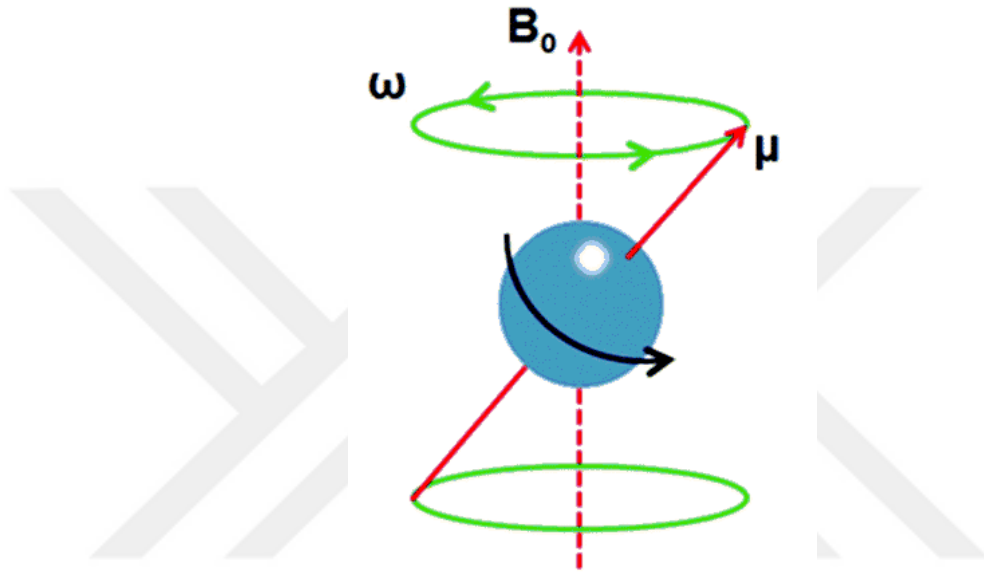
Figure 1.1: NMR spin precession
