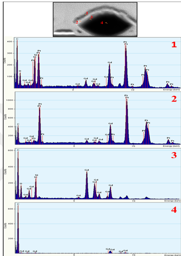
Figure 2.4: Elemental analysis
