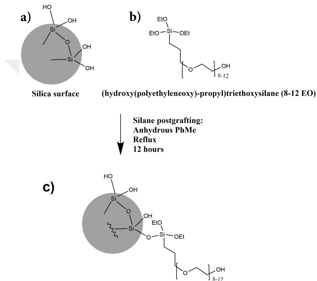
Figure 2.9: PEGylation process
