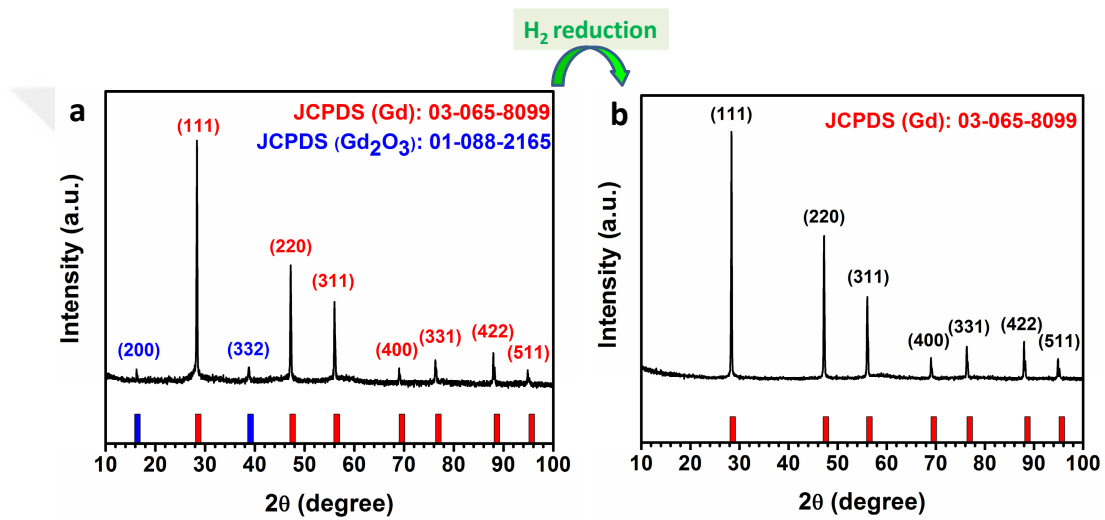
Figure 2.6: Elemental analysis
