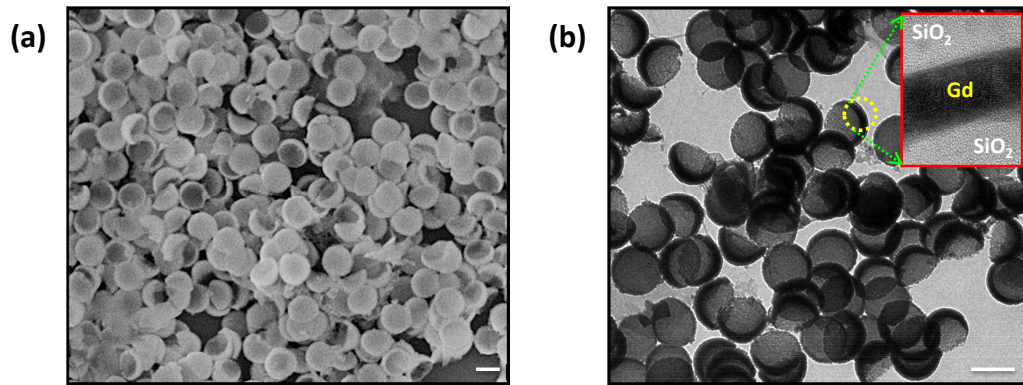
Figure 3.1: SEM and TEM of nanobowls
