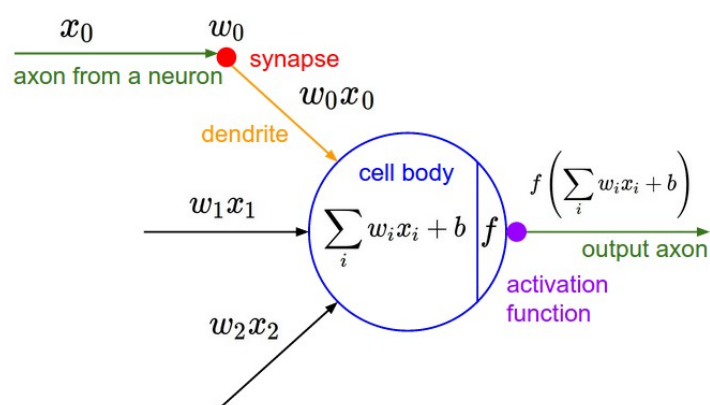
Figure 1.2: Biological inspiration of a perceptron 3
