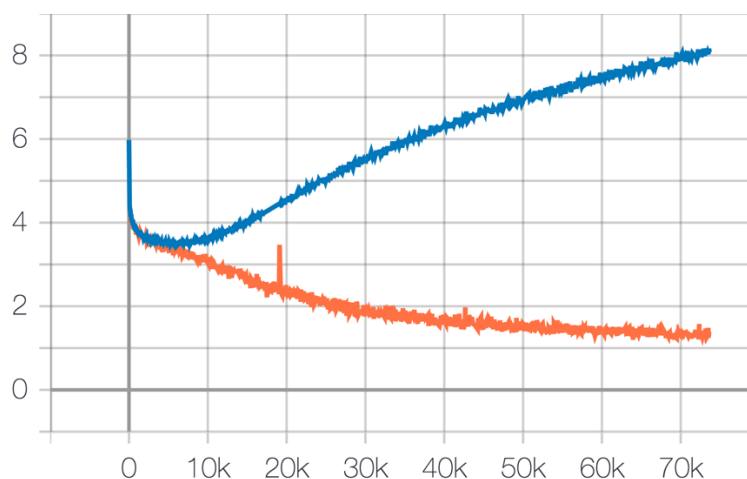
Figure 2.51: Training loss of the training (orange) and validation (blue) set, fourth experiment
