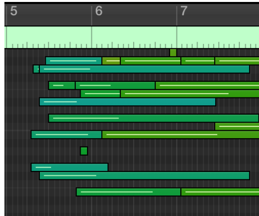
Figure 2.14: Velocity data 19 of figure 2.13
