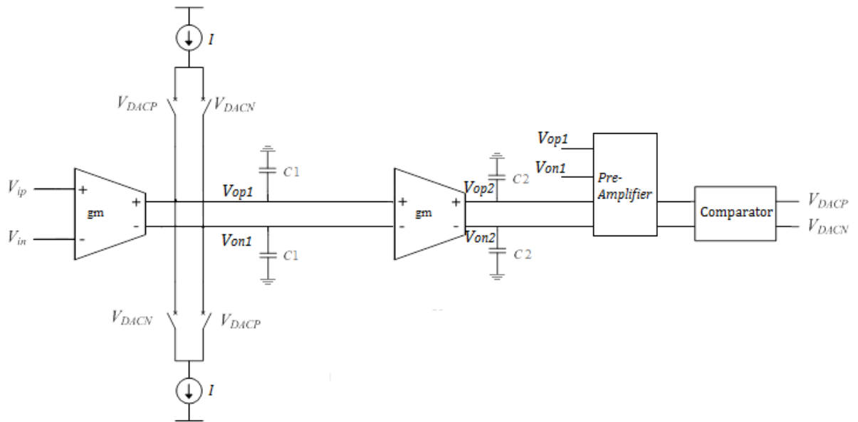
Figure 3.20 Schematic of feedforward configuration of the modulator.
