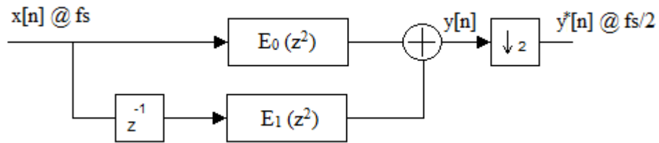
Figure 4.9. Block diagram of FIR filter with coefficients with odd and even indices separated.
