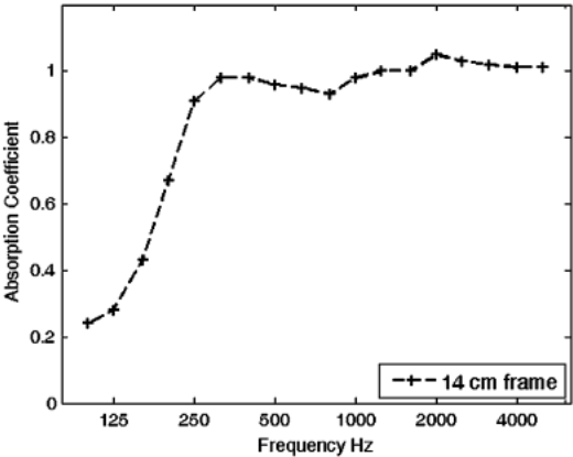
Figure 2.52 Absorption coefficient of end-on reeds of nominal length 14 cm measured in reverberation room (Oldham et al., 2011).
