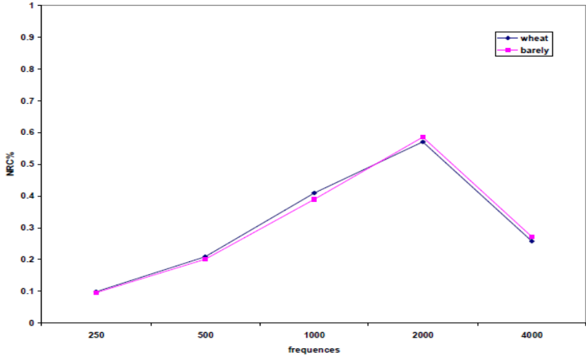
Figure 2.17 Effect of two kinds of straw (Wheat and Barely straws) on NRC %. All points are in the same groups (Saadatnia et al., 2008)
