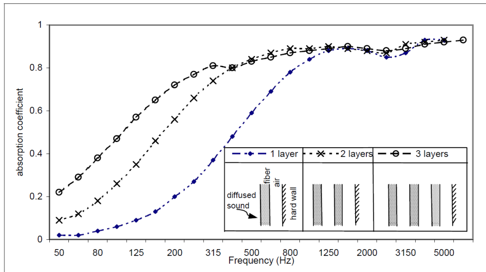
Figure 2.23 Diffused incidence sound absorption coefficients of 20 mm thick coconut coir fiber sample of density 74 \text{ kg/m}^3 backed with airspaces and without micro perforated aluminum plate facing.
