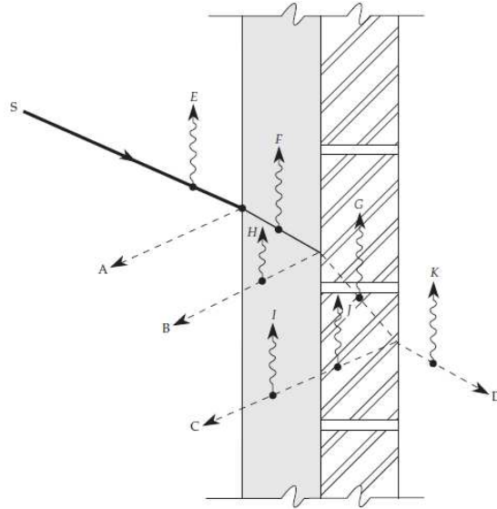
Figure 2.2 Sound absorption of porous material with masonry wall behind (Everest & Pohlmann, 2009, p. 201).
