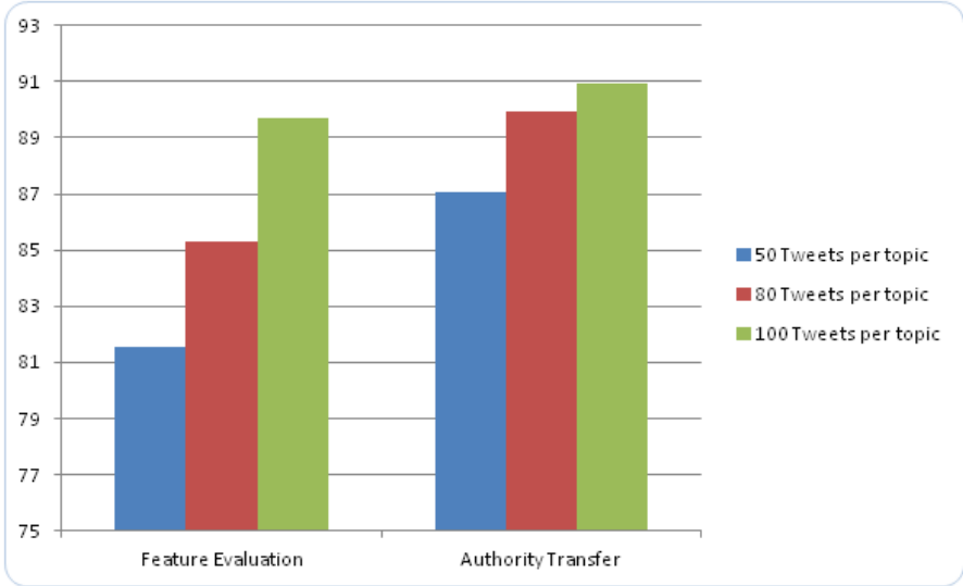
Figure 4.5: Comparison of accuracy rate for different number of tweets per topic
