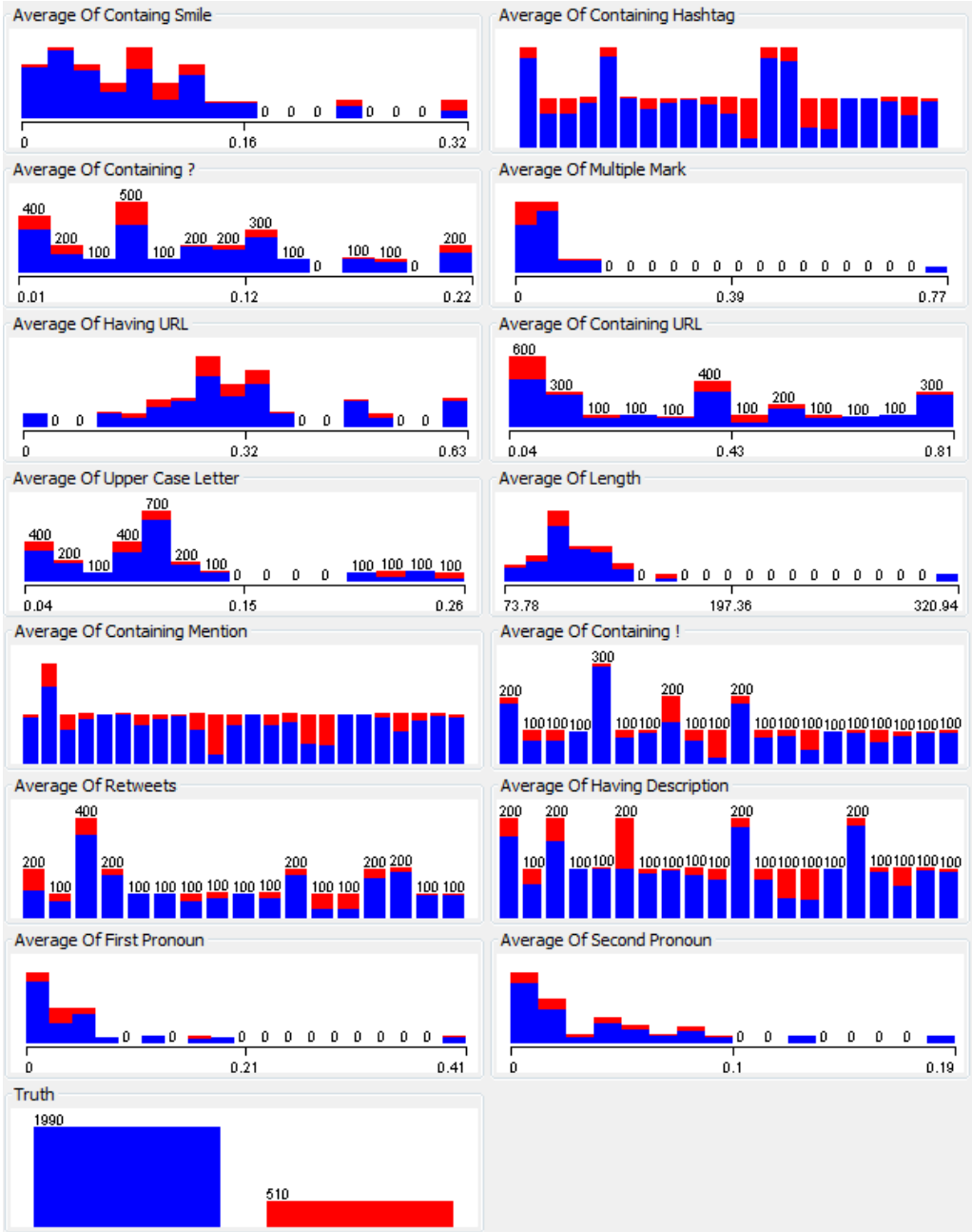
Figure C.3: Histogram of Attributes for Correctness Label - III
