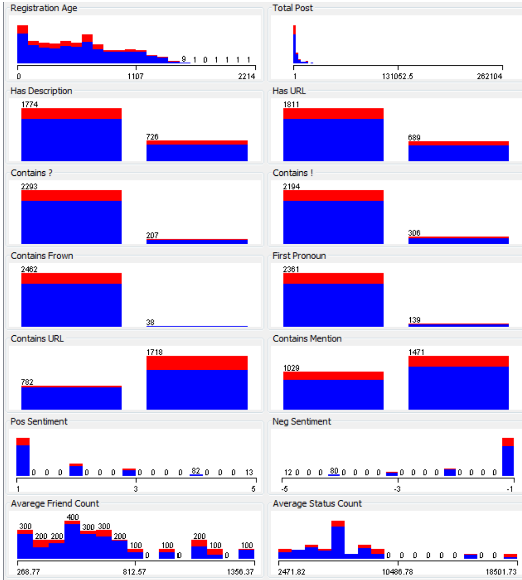
Figure C.1: Histogram of Attributes for Correctness Label - I
