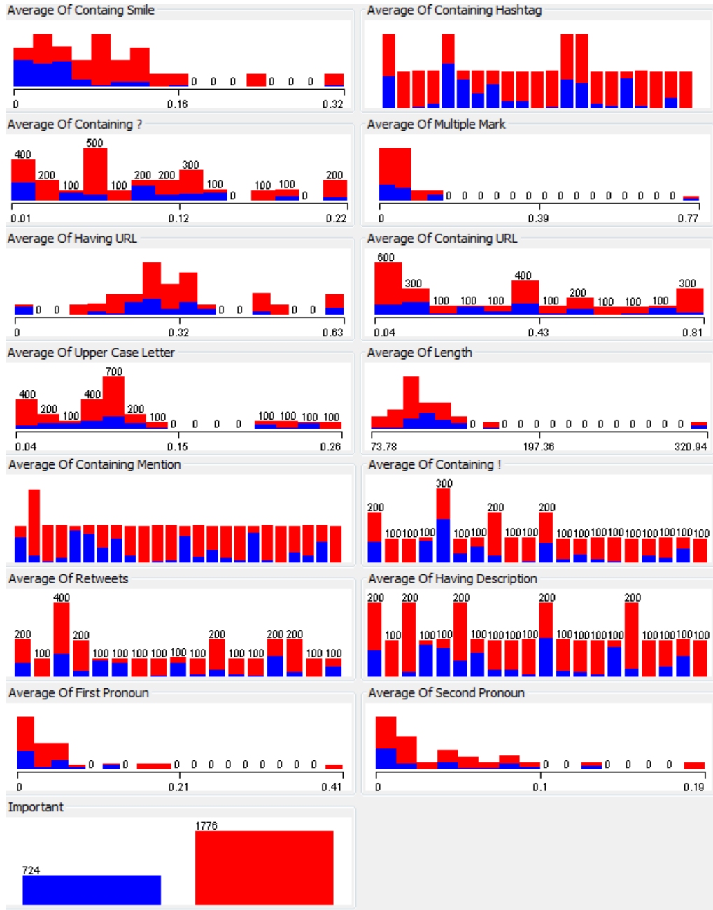
Figure B.3: Histogram of Attibutes for Importance Label - III
