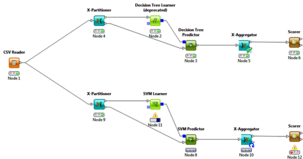
Figure 3.9: Learning Schemes for Knime Tool
