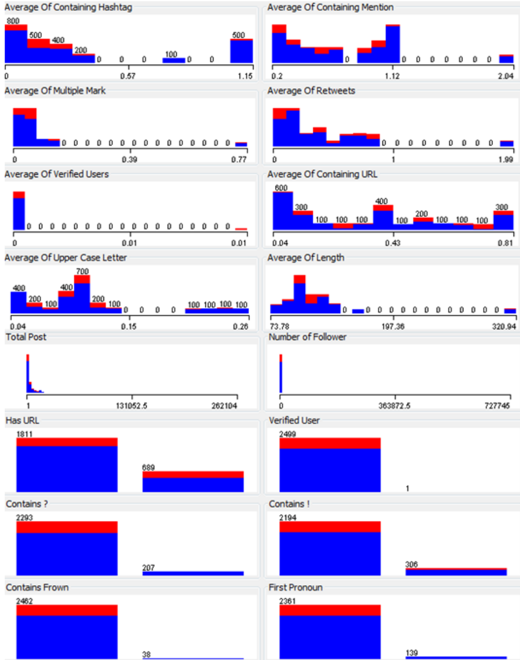
Figure A.2: Histogram of Attitubes for Newsworthiness Label - II
