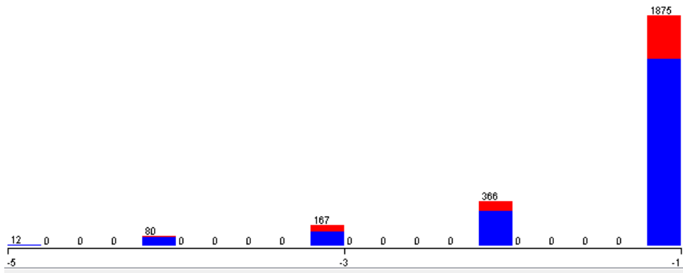
Figure 3.4: Histogram Detail of Feature - Negative Sentiment Score
