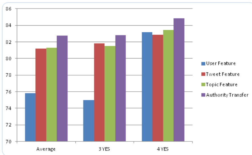
Figure 4.7: Importance label accuracy rate when training features separately
