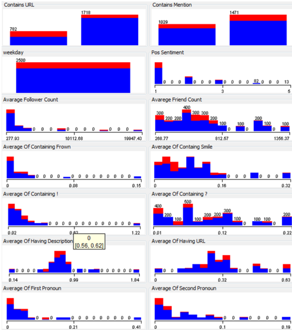
Figure A.3: Histogram of Attibutes for Newsworthiness Label - III
