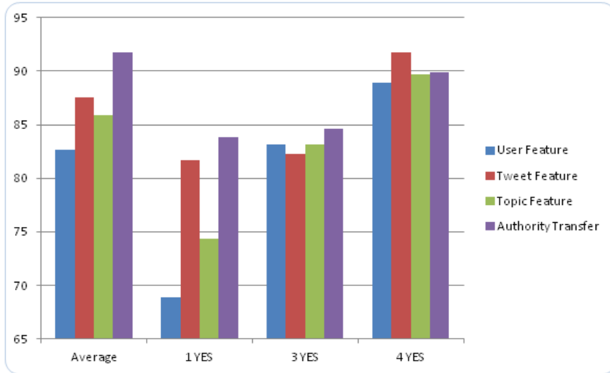
Figure 4.3: Newsworthiness label accuracy rate when training features separately
