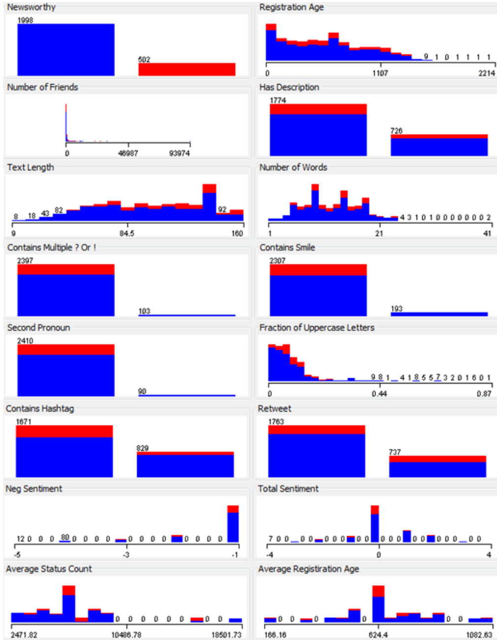
Figure A.1: Histogram of Attributes for Newsworthiness Label - I
