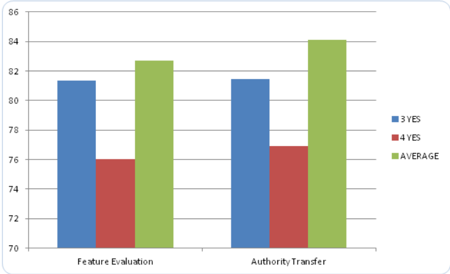
Figure 4.8: Correctness label accuracy rate when training all features together
