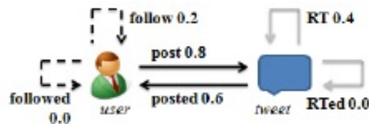
Figure 2.1: Sample Graph Used in TURank. Retrieved from [38]
