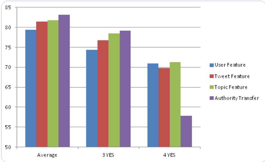
Figure 4.9: Correctness label accuracy rate when training features separately
