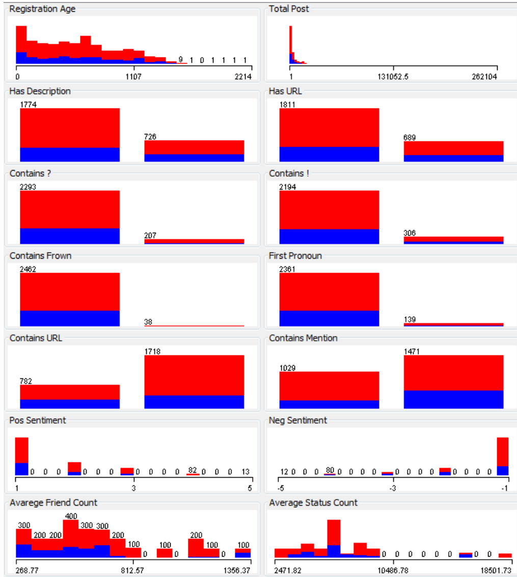
Figure B.1: Histogram of Attributes for Importance Label - I
