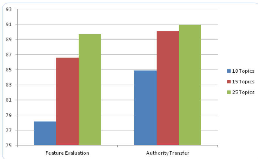
Figure 4.4: Comparison of accuracy rate for different number of topics
