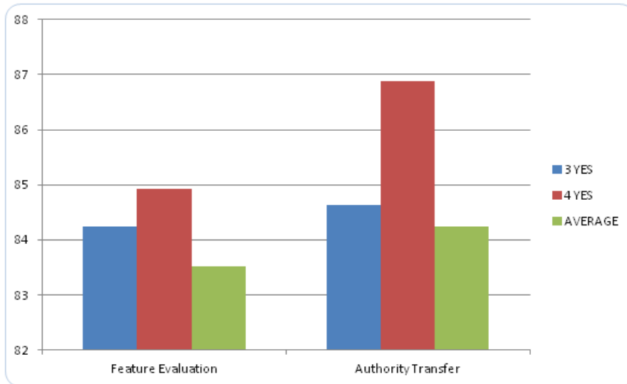
Figure 4.6: Importance label accuracy rate when training all features together
