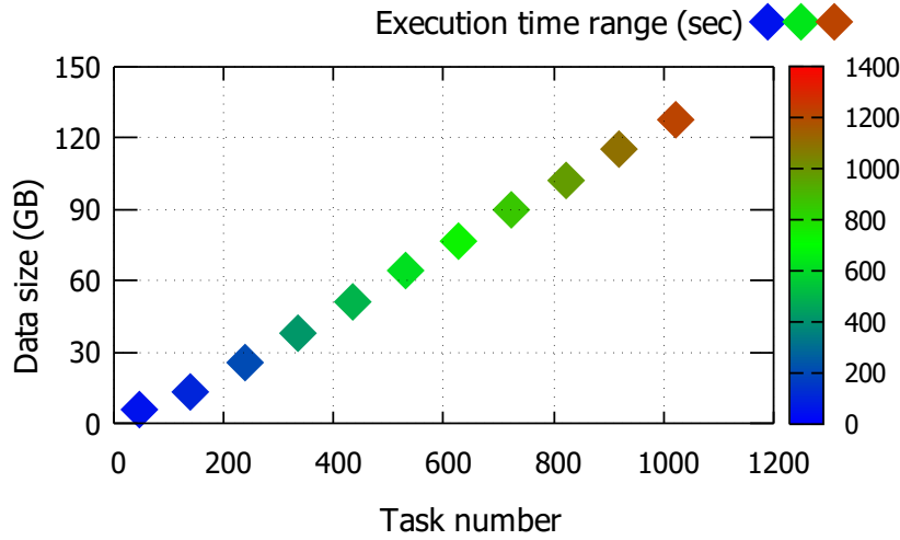
Figure 3.11: K-means execution time on different data size
