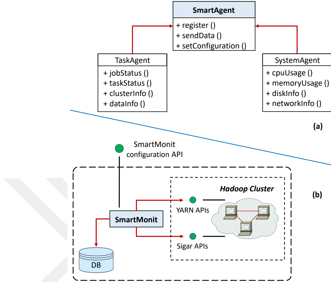
Figure 3.2: Monitoring agents model (a); Implementation of SmartMonit mechanism in a Hadoop cluster (b).
