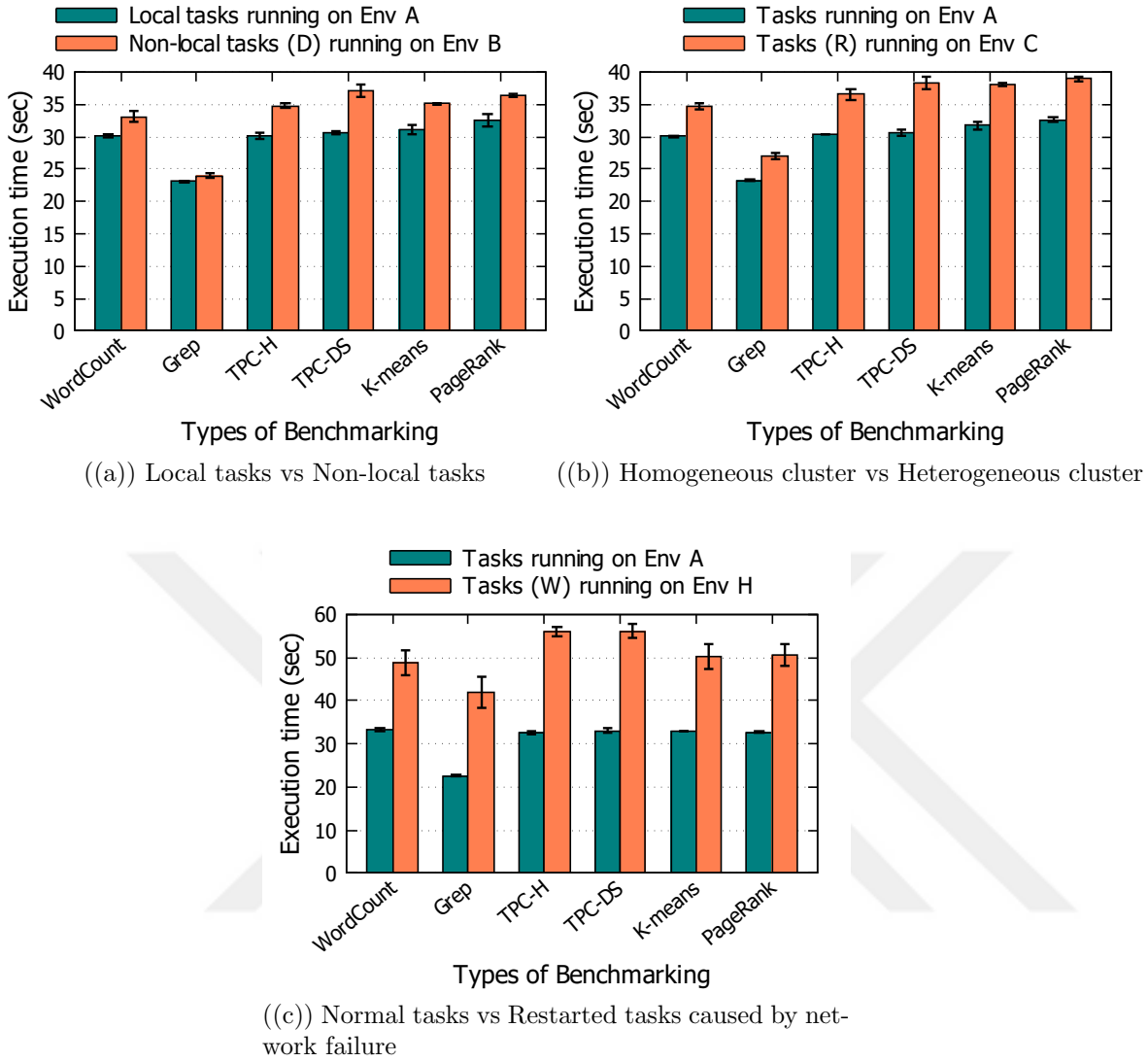
Figure 4.5: Comparison of execution time of the tasks
