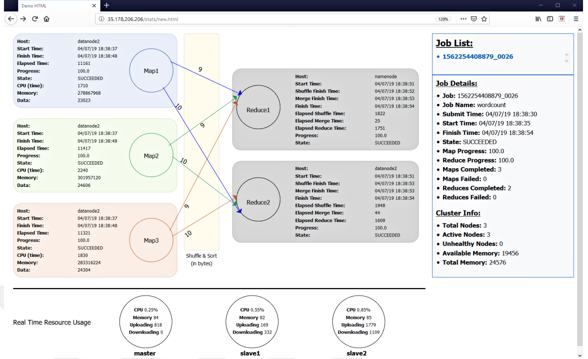
Figure 3.14: Execution graph in a real-time monitoring system.
