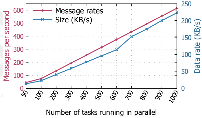
((b)) The message rates and network overhead
