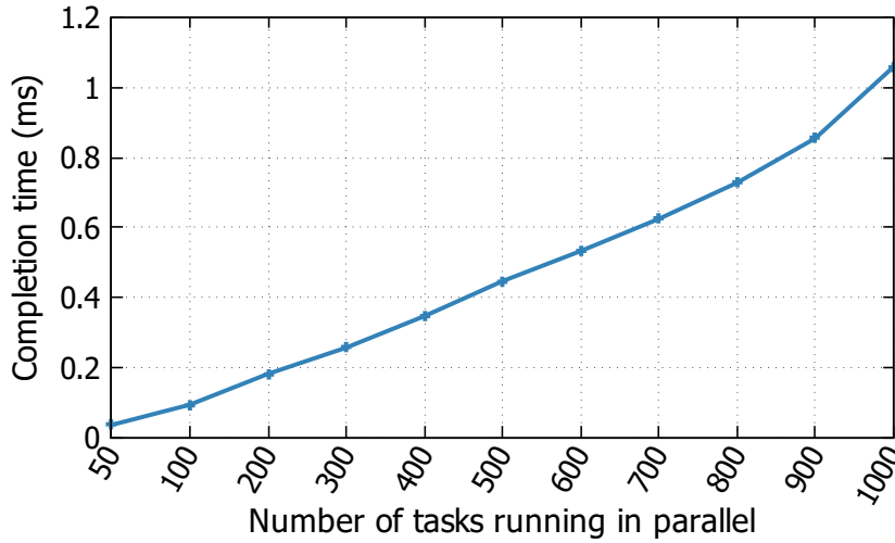
Figure 3.4: Metrics collection completion time
