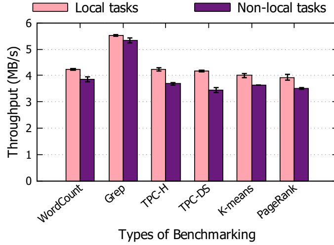
Figure 4.6: The throughput of AutoDiagn
