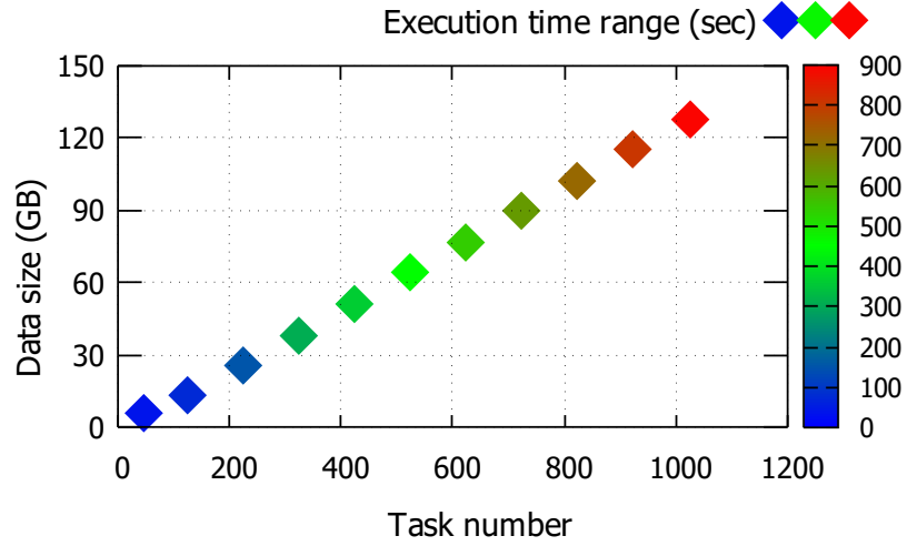
Figure 3.8: Grep execution time on different data size
