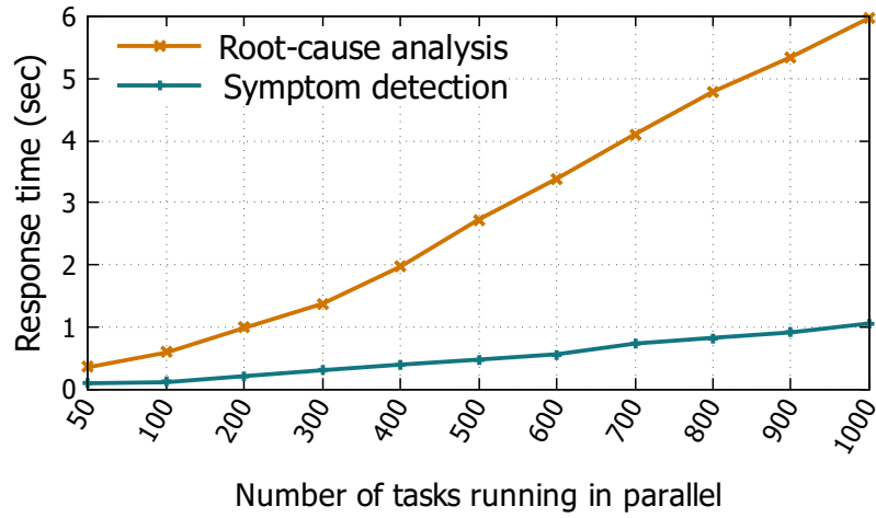
((a)) The end-to-end response time of AutoDiagn diagnosis system
