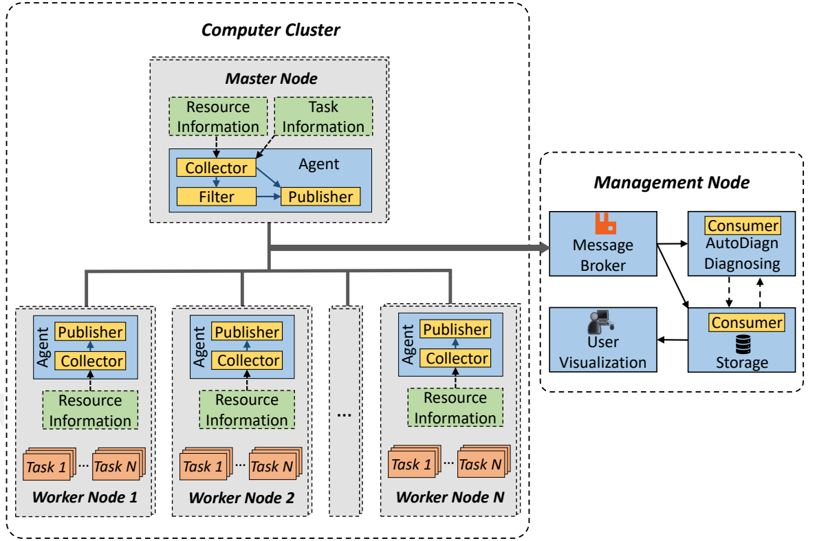
Figure 4.3: The high-level architecture of the monitoring framework
