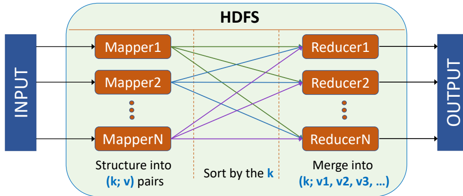
Figure 2.5: MapReduce working principle
