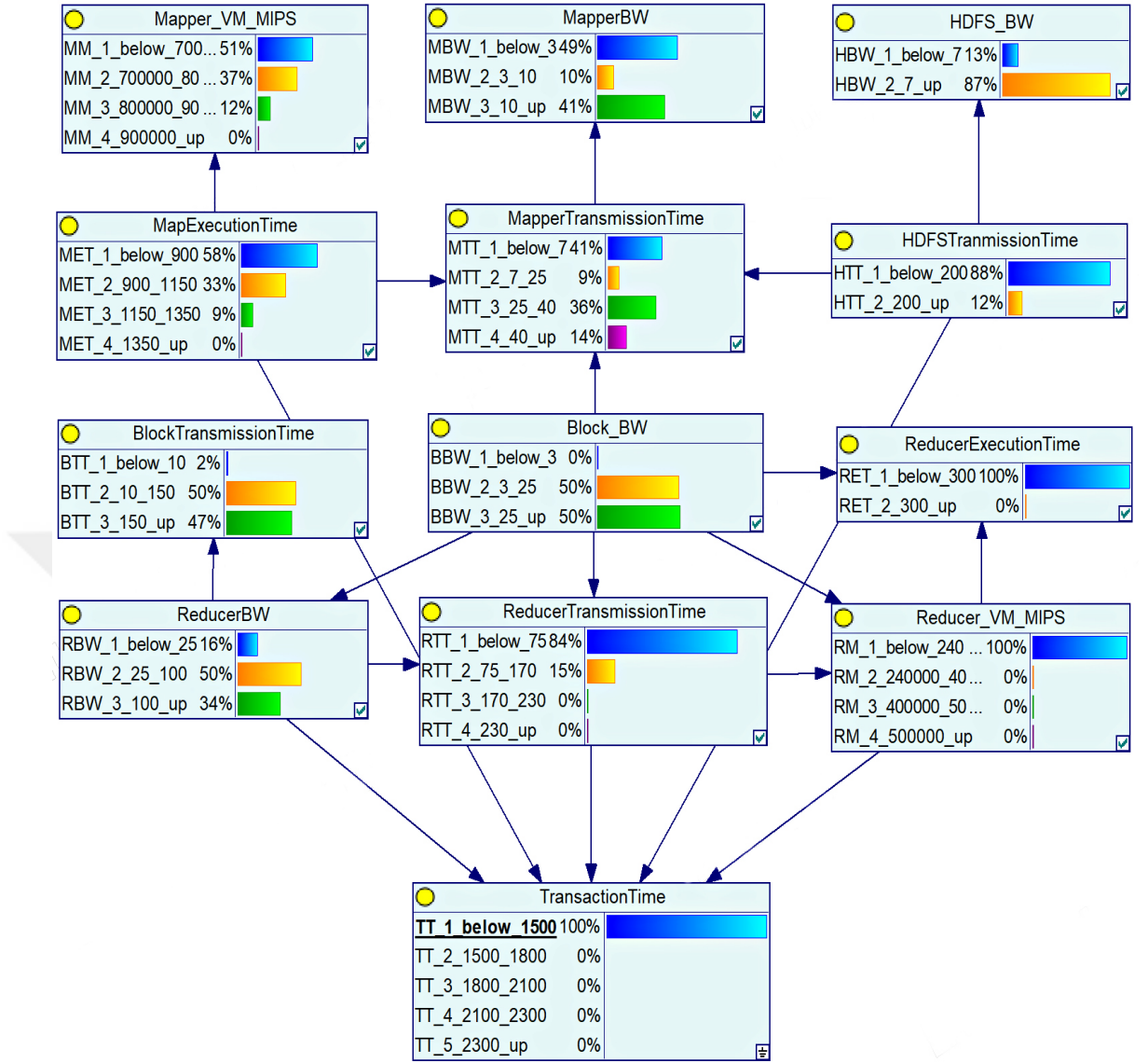
Figure 5.5: Screenshot of Bayesian Network implementation in GeNIe platform.
