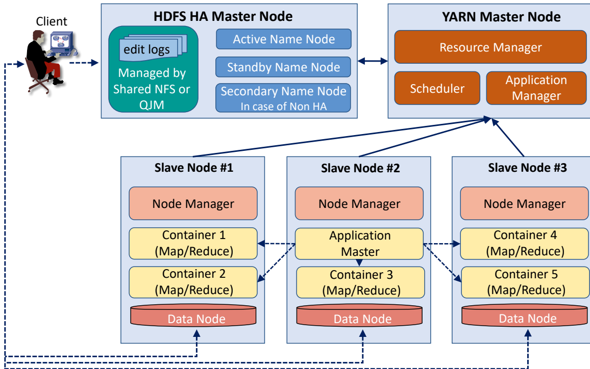
Figure 2.2: A typical Hadoop architecture
