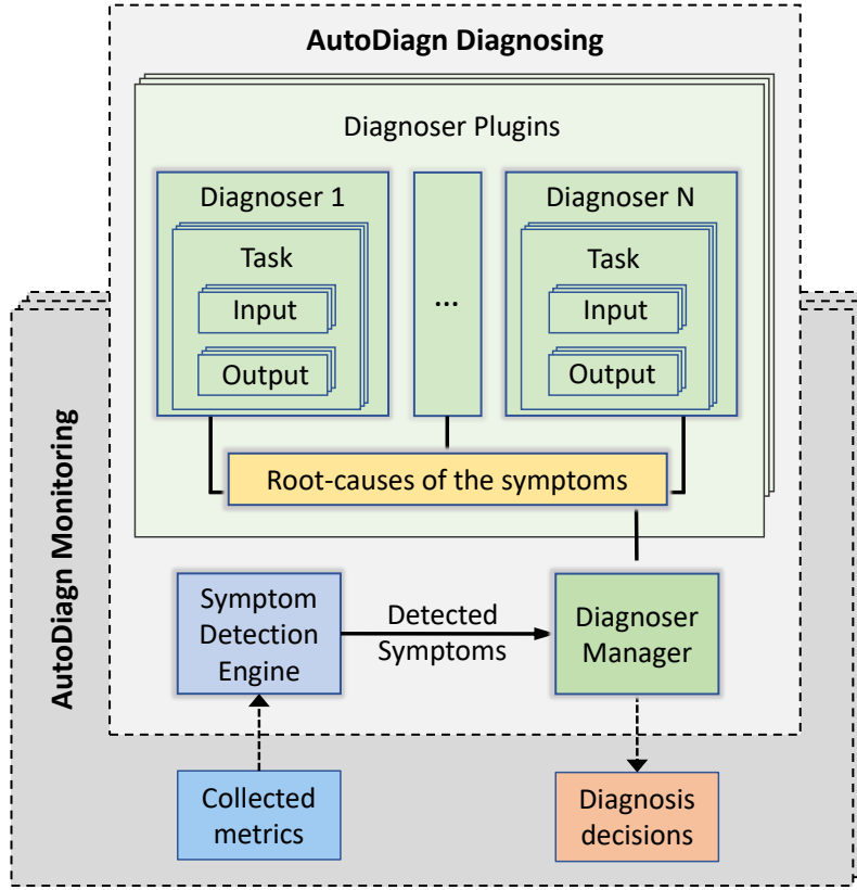
Figure 4.2: The high-level architecture of the AutoDiagn system
