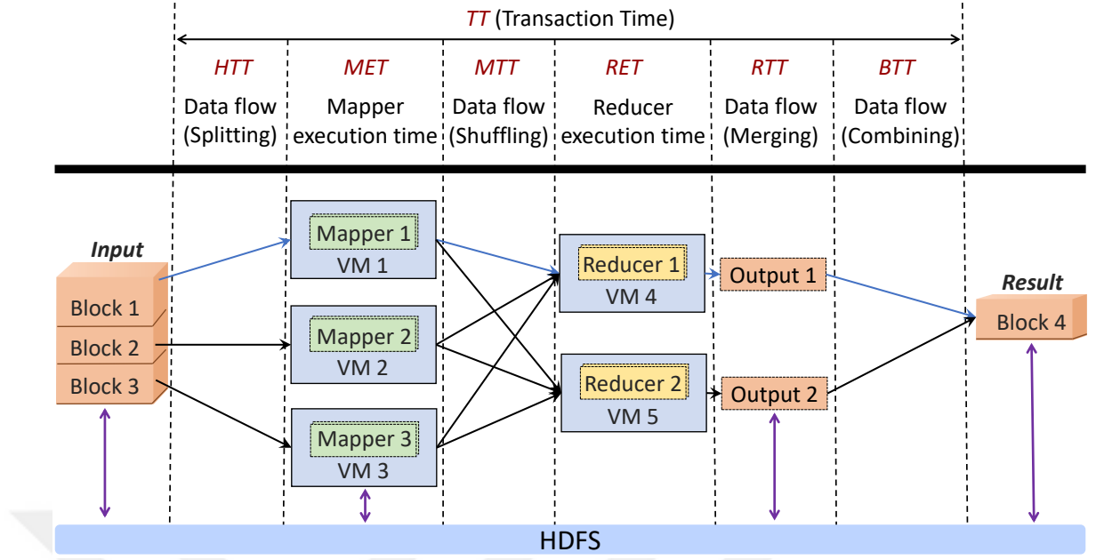
Figure 5.1: End-to-end Transaction time of a task
