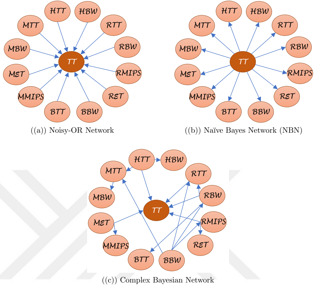
Figure 5.3: Bayesian Networks for Big Data QoS diagnosis and prediction
