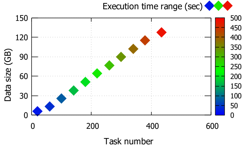
Figure 3.9: TPC-H execution time on different data size
