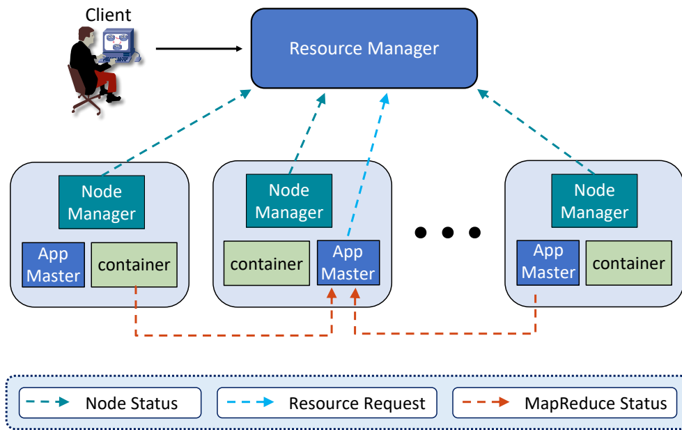
Figure 2.3: YARN architecture and its components
