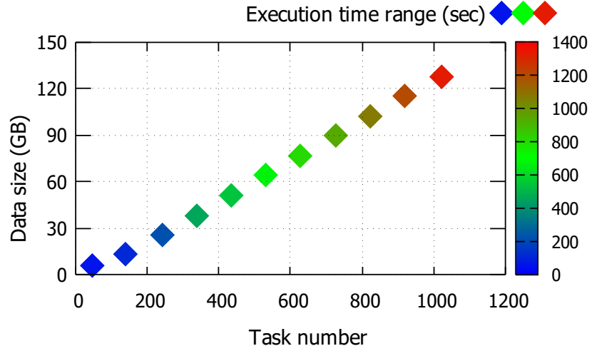
Figure 3.12: PageRank execution time on different data size
