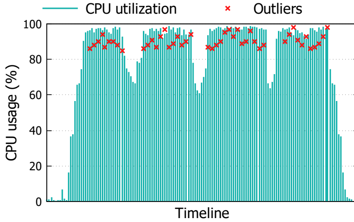
((a)) CPU utilization of less powerful hosts and outliers
