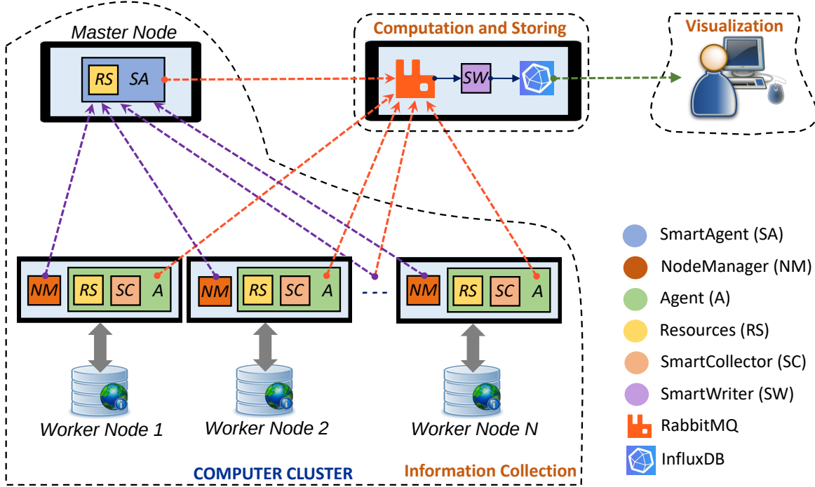
Figure 3.3: The framework of SmartMonit.
