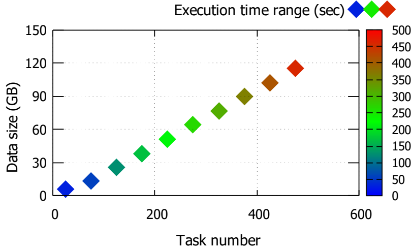
Figure 3.10: TPC-DS execution time on different data size
