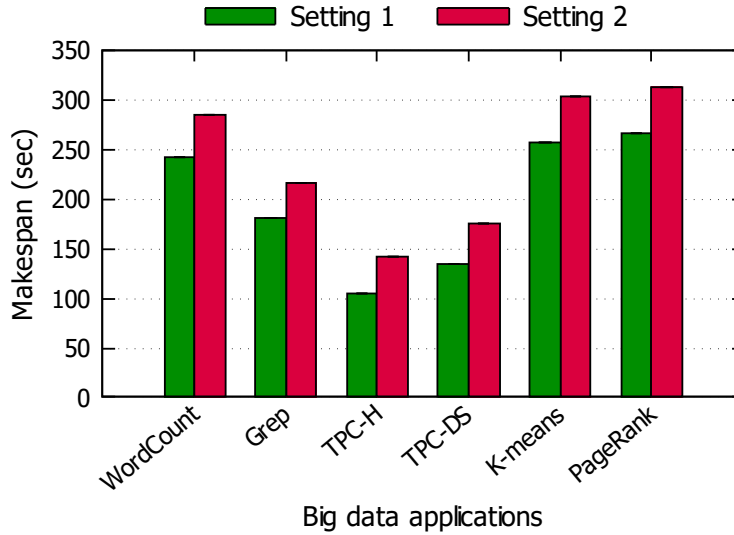
Figure 1.1: Six big data applications are executed in a cloud-based Hadoop cluster with two settings: 1) the input data and jobs are allocated in the same node; 2) the input data and jobs are allocated in different nodes. In Setting 2, the execution time of each application is delayed by transmitting data across nodes.
