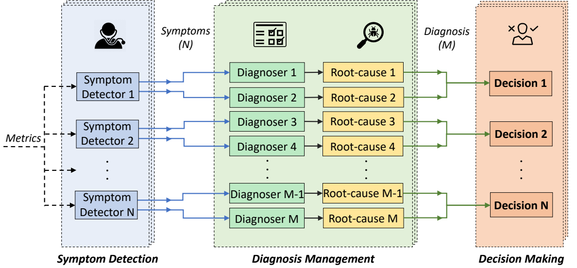
Figure 4.1: The key design idea of root-cause analysis for big data processing systems
