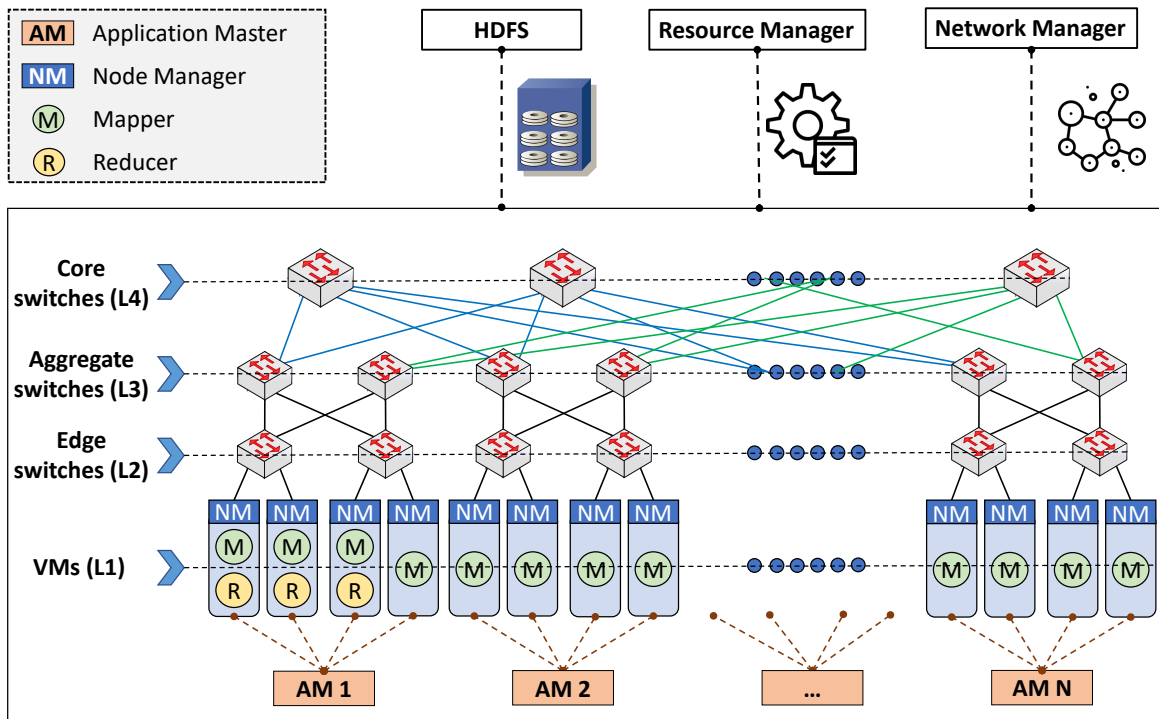
Figure 5.4: Fat-tree topology used in the simulated use-case experiments.
