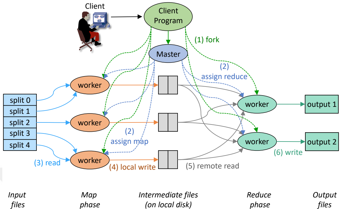
Figure 2.6: High-level MapReduce processing pattern
