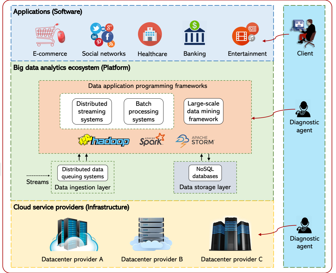
Figure 1.2: Performance diagnosis of big data systems in cloud datacenters
