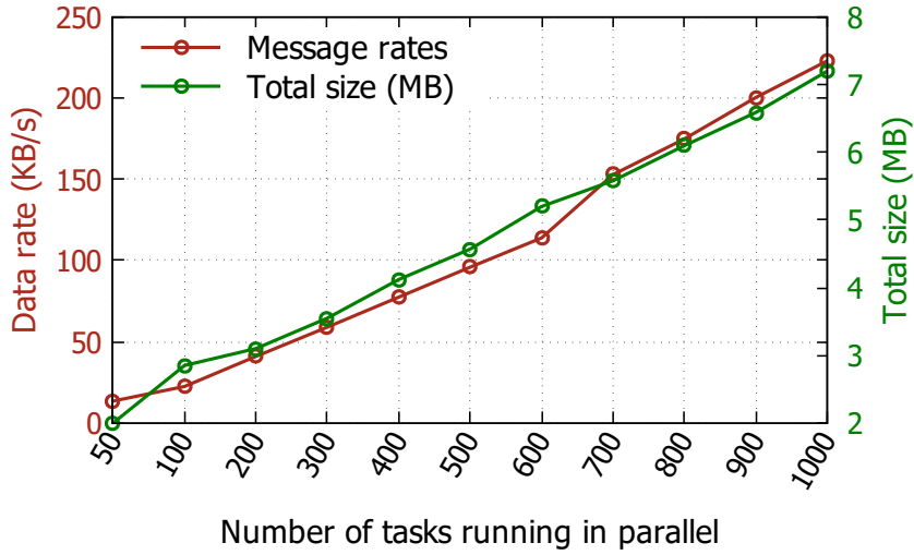
Figure 3.6: The network and storage overheads of SmartMonit
