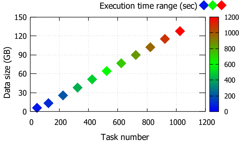
Figure 3.7: WordCount execution time on different data size
