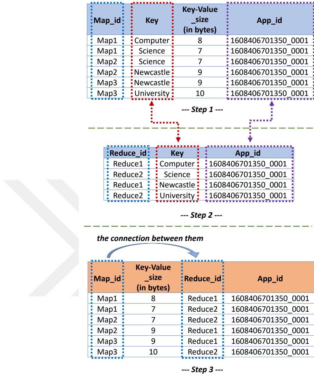
Figure 3.13: The algorithm of SmartWriter.
