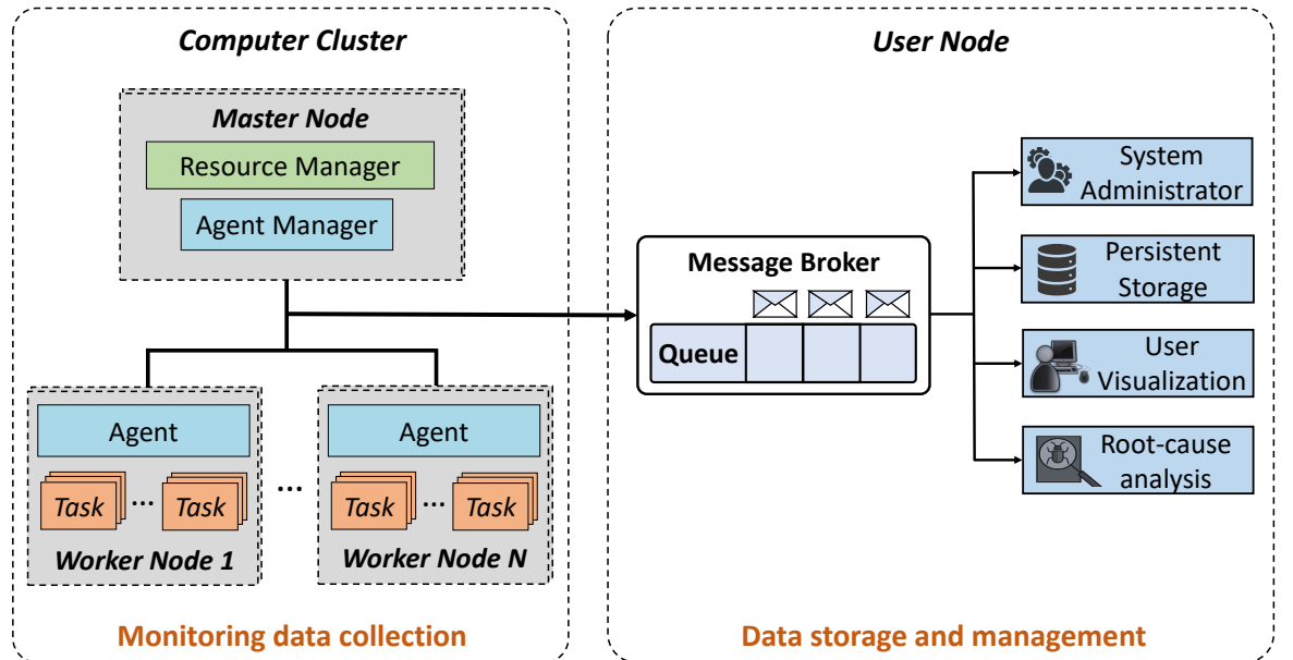
Figure 3.1: Example scenario for monitoring big data systems
