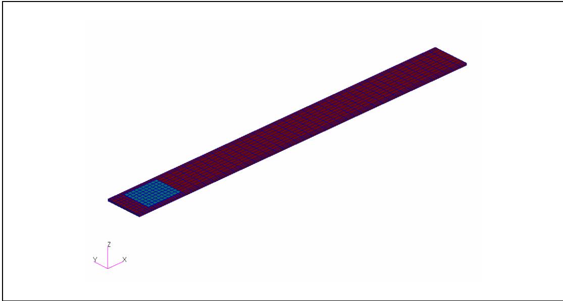
Figure 3.3 Solid-solid finite element model of the smart beam with 1628 nodes and 808 CHEXA elements
