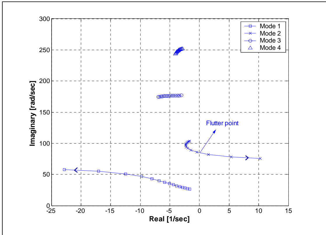
Figure 4.9 Root-locus of the state-space model of the aft-swept wing as a function of the flight speed ( \rho = 1.1507 \text{ kg/m}^3 )
