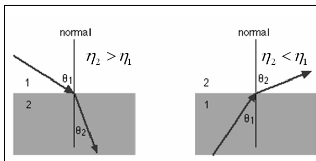
Figure 3.1.2. Light traveling between two mediums with different index of refraction
