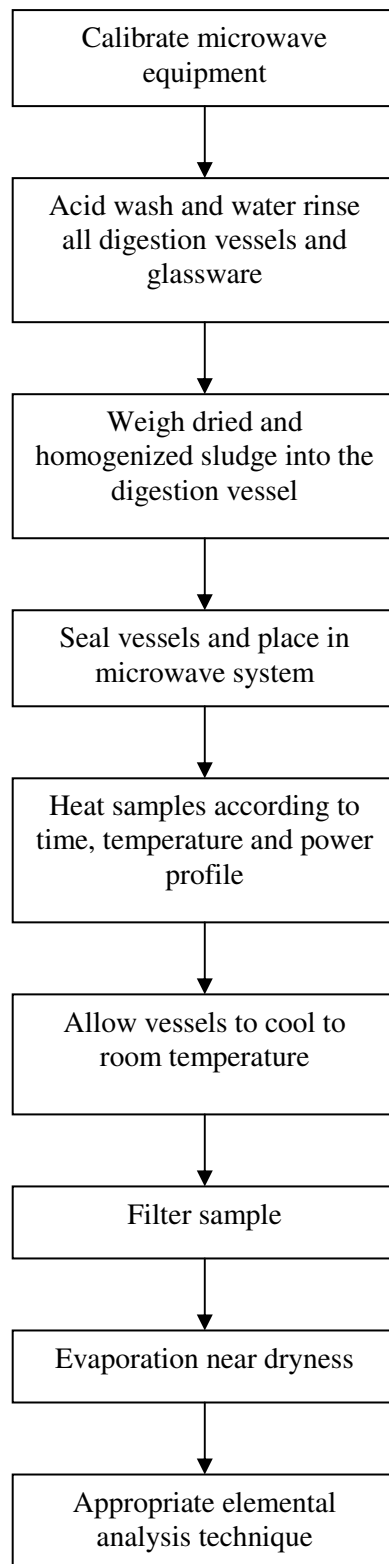
Figure 1. Overall digestion procedure
