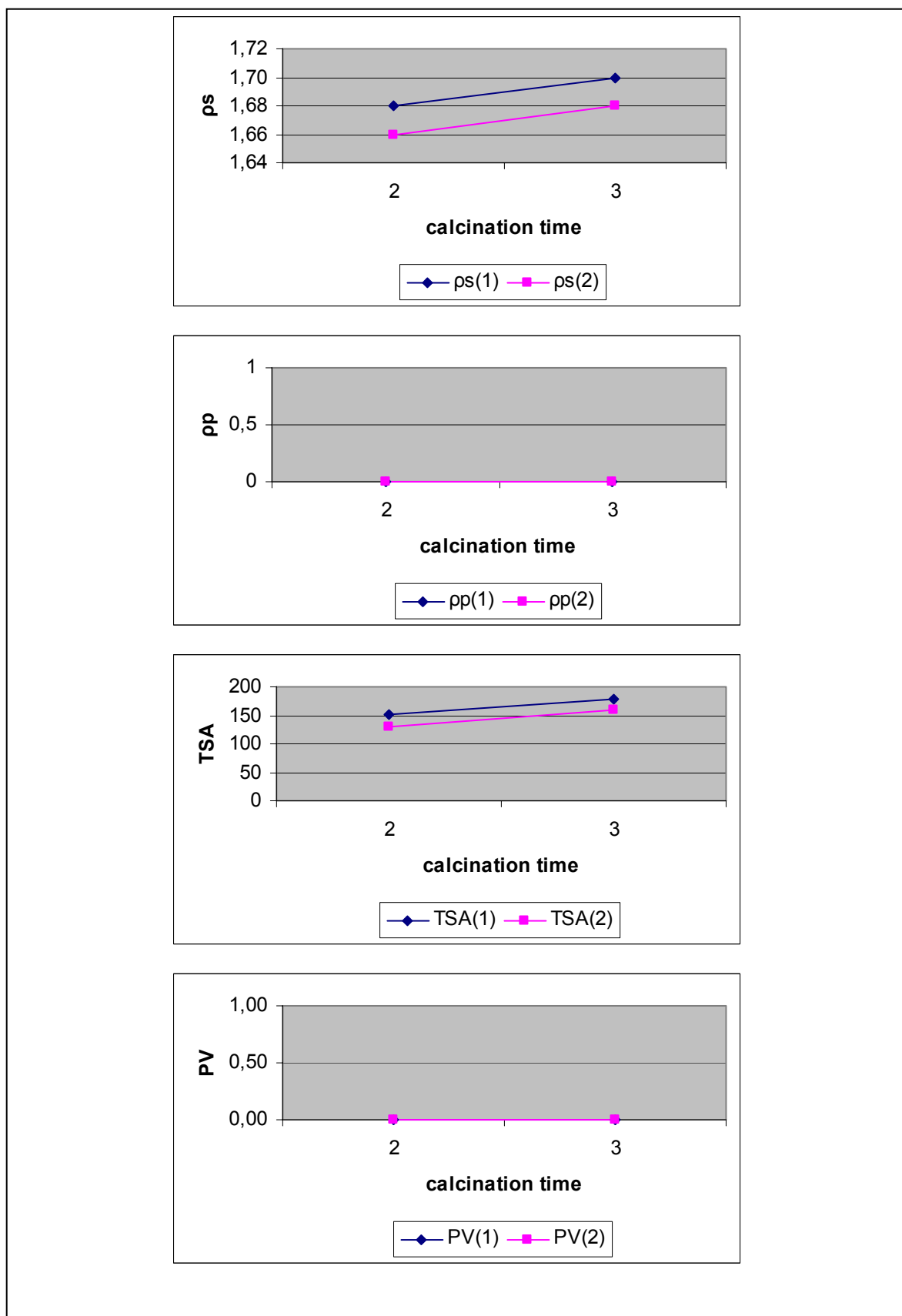
Figure 4.4. Effect of calcination time on physical properties of 1.4%Pt-2.5%Co-2.5%Ce/Al 2 O 3 ; (1) and (2) indicate calcination conditions in Tables 4.7 and 4.8, respectively.
