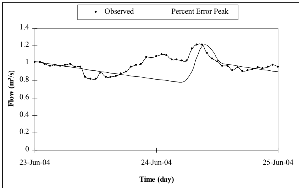
Figure B.31. Serindere Subbasin Event 39 Flow Hydrographs
