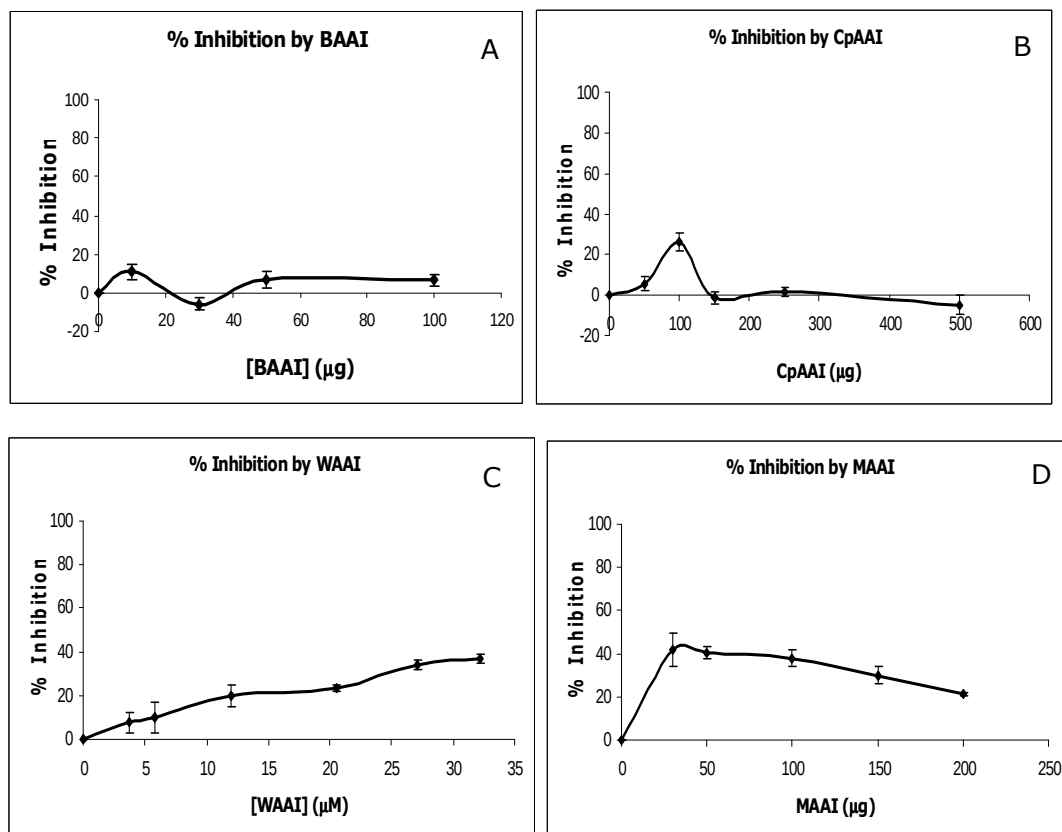
Figure 3.4 Percent inhibition of sunn pest midgut \alpha -amylase activity by different concentrations of \alpha -amylase inhibitors. A) bean \alpha -amylase inhibitor (BAAI), B) chickpea \alpha -amylase inhibitor (CpAAI), C) wheat \alpha -amylase inhibitor (WAAI) and D) maize \alpha -amylase inhibitor (MAAI). Values in x-axis indicates the amount of inhibitor included per assay
