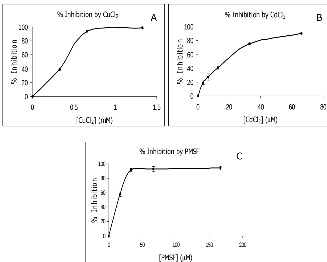
Figure 3.18 Inhibition of H. armigera midgut leucine aminopeptidase-like activity by different concentrations of protease inhibitors. A) \text{CuCl}_2 B) \text{CdCl}_2 and C) PMSF.
