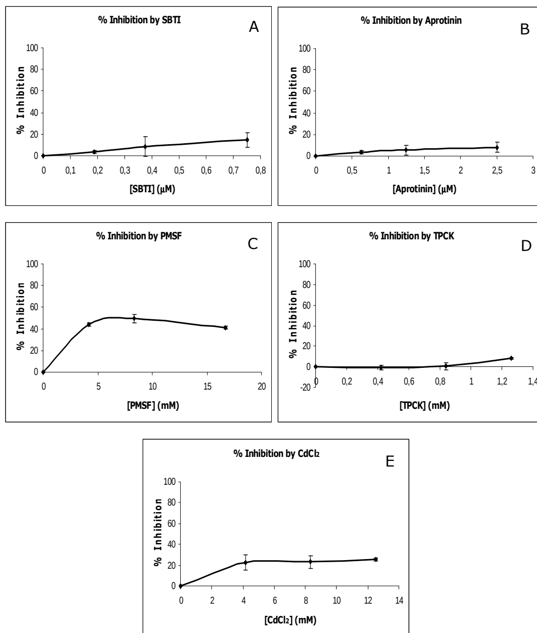
Figure 3.8 Inhibition of sunn pest midgut total protease (azoalbumin hydrolyzing) activity by different concentrations of protease inhibitors. A) soybean trypsin inhibitor (SBTI), B) aprotinin, C) PMSF D) TPCK and E) CdCl 2 .
