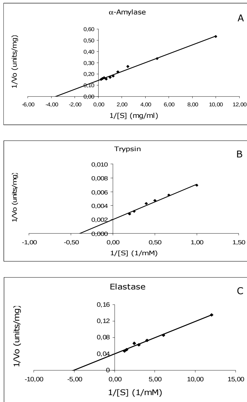
Figure 3.11 Lineweaver-Burk Plots for Helicoverpa armigera midgut hydrolytic enzymes. A) α-amylase, B) trypsin and C) elastase.
