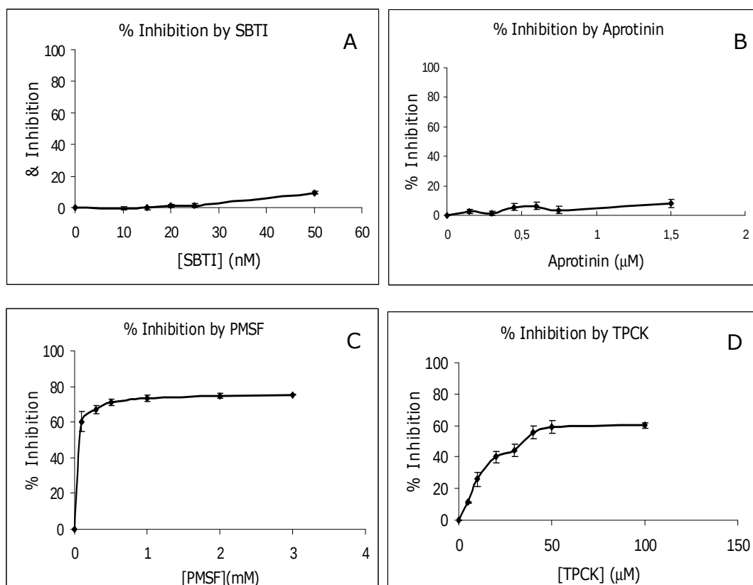
Figure 3.16 Inhibition of H. armigera midgut elastase activity by different concentrations of protease inhibitors. A) soybean trypsin inhibitor (SBTI), B) aprotinin C) PMSF and D) TPCK.
