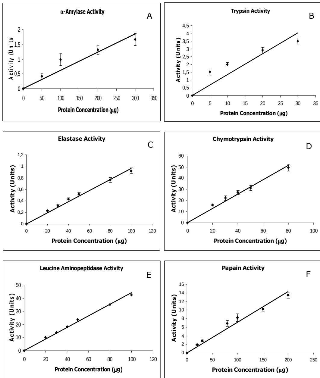
Figure 3.9 Hydrolytic enzymes from cotton bollworm midgut. A) \alpha -Amylase activity (1 Unit activity = mmoles maltose produced/10 min); B) Trypsin activity; C) Elastase activity; D) Chymotrypsin Activity E) Leucine aminopeptidase activity (1 Unit activity = \mu moles p -nitroanilide produced /min); F) Papain Activity (1 Unit activity = 0.001 units change in OD 440 /min).
