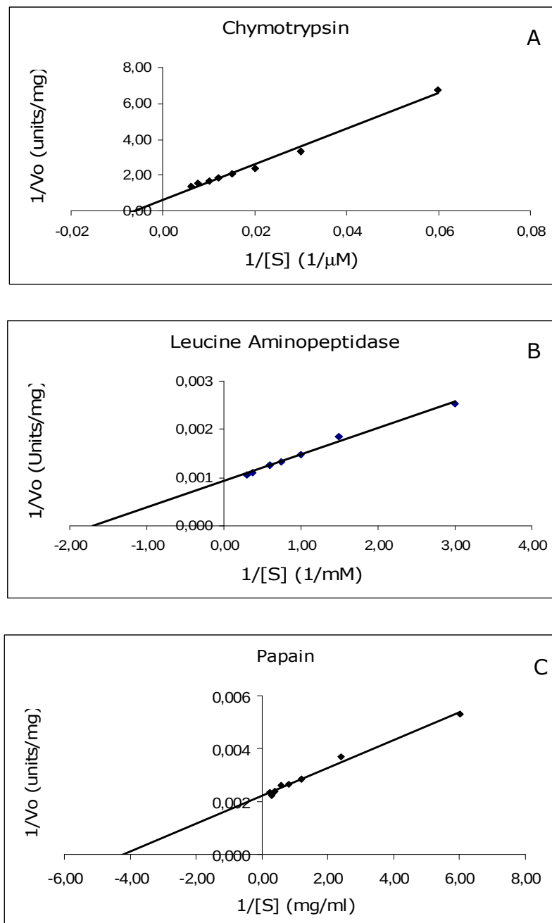
Figure 3.12 Lineweaver-Burk Plots for Helicoverpa armigera midgut hydrolytic enzymes. A) Chymotrypsin, B) leucine aminopeptidase and C) papain.
