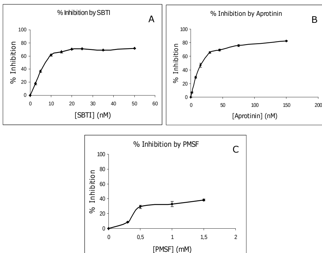
Figure 3.15 Inhibition of H. armigera midgut trypsin activity by different concentrations of protease inhibitors. A) soybean trypsin inhibitor (SBTI), B) aprotinin and C) PMSF.
