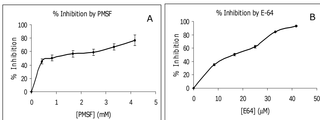
Figure 3.19 Inhibition of H. armigera midgut papain activity by different concentrations of protease inhibitors. A) PMSF and B) E-64.
