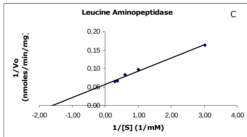
Figure 3.3 Lineweaver-Burk Plot for sunn pest midgut hydrolytic enzymes. A) \alpha -amylase, B) trypsin and C) leucine aminopeptidase.
