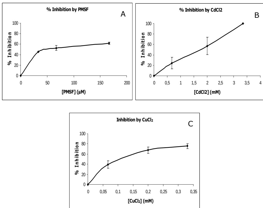
Figure 3.7 Inhibition of sunn pest midgut leucine aminopeptidase activity by different concentrations of protease inhibitors. A) PMSF, B) CdCl 2 and C) CuCl 2 .
