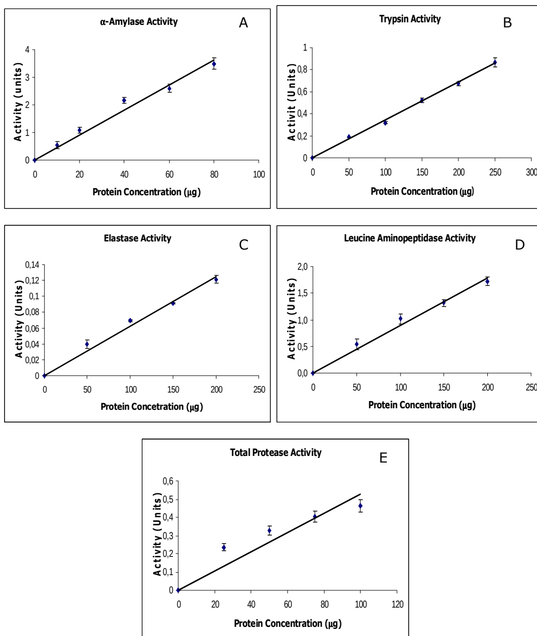
Figure 3.1 Hydrolytic enzymes from Sunn Pest midgut. A) \alpha -Amylase activity (1 Unit activity = mmoles maltose produced/10 min); B) Trypsin activity; C) Elastase activity; D) Leucine aminopeptidase activity (1 Unit activity = \mu moles p -nitroanilide produced /min); E) Total protease activity (1 Unit activity = 0.001 units change in OD 335 /min).
