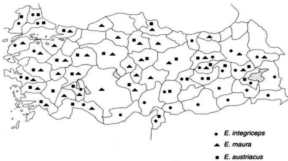
Figure 1.2 Distribution of Eurygaster species in Turkey.
