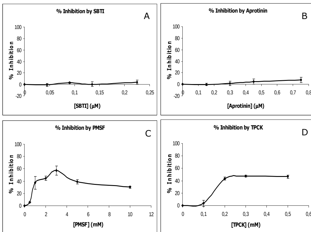
Figure 3.6 Inhibition of sunn pest midgut elastase activity by different concentrations of protease inhibitors. A) soybean trypsin inhibitor (SBTI), B) aprotinin, C) PMSF and D) TPCK.
