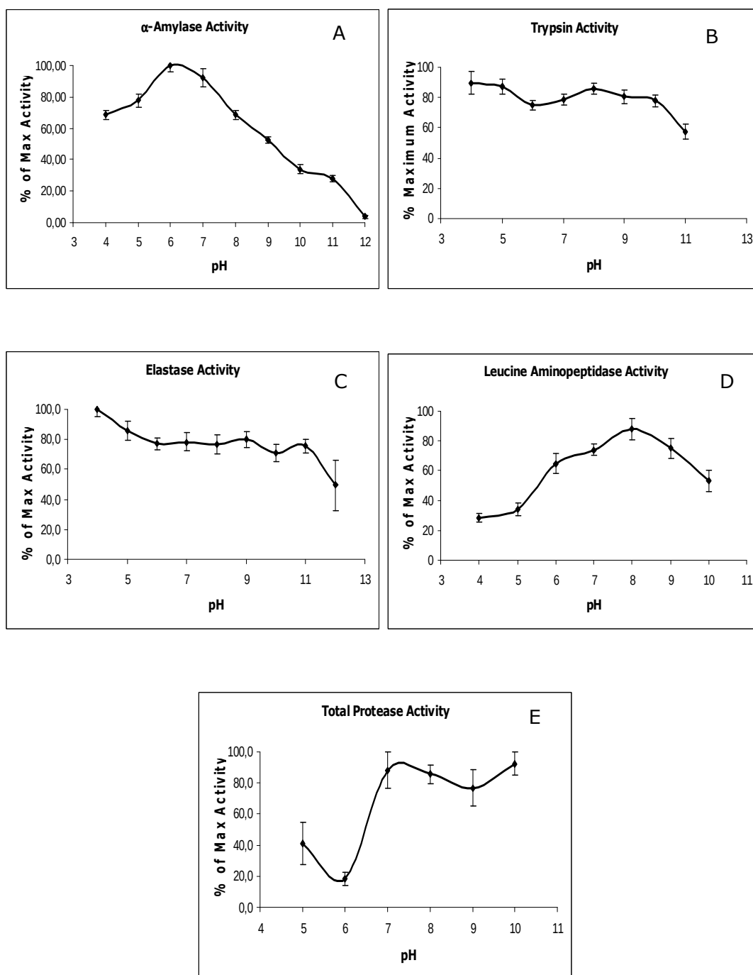
Figure 3.2 Effect of pH on hydrolytic enzymes of sunn pest. A) \alpha -Amylase, B) Trypsin, C) Elastase, D) Leucine aminopeptidase and E) Total protease.
