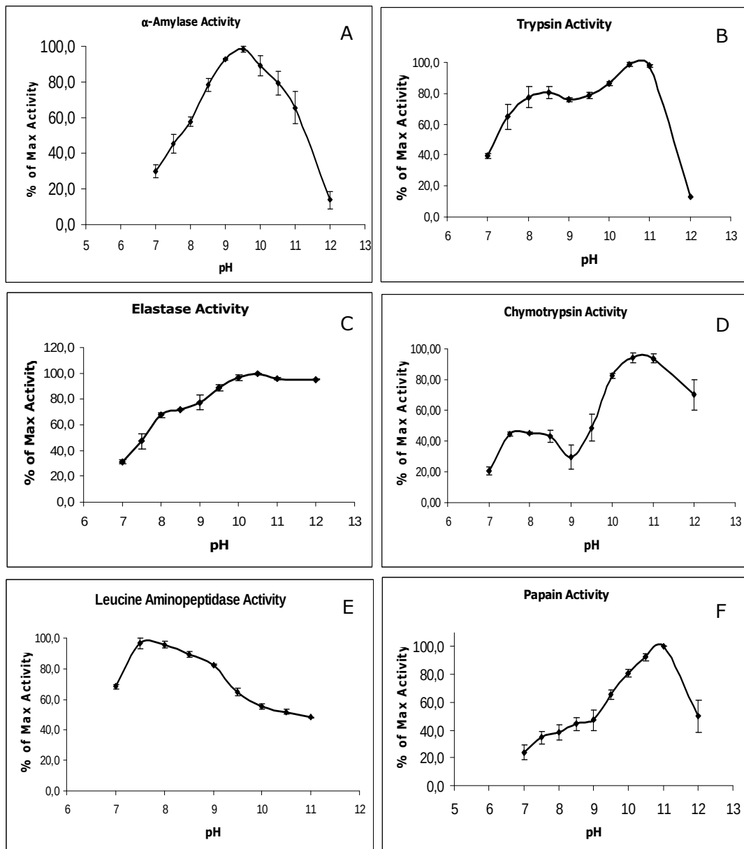
Figure 3.10 Effect of pH on H. armigera midgut hydrolytic enzymes. A) \alpha -Amylase, B) Trypsin, C) Elastase, D) Chymotrypsin E) Leucine aminopeptidase and F) Papain.
