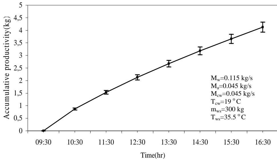
Figure F.1 Accumulative productivity of the system (with error bars).
