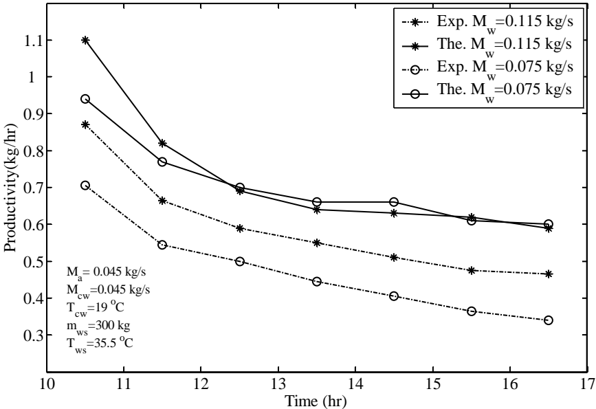
Figure 5.14 Comparison between experimental and theoretical results at different values of the feed water mass flow rate.
