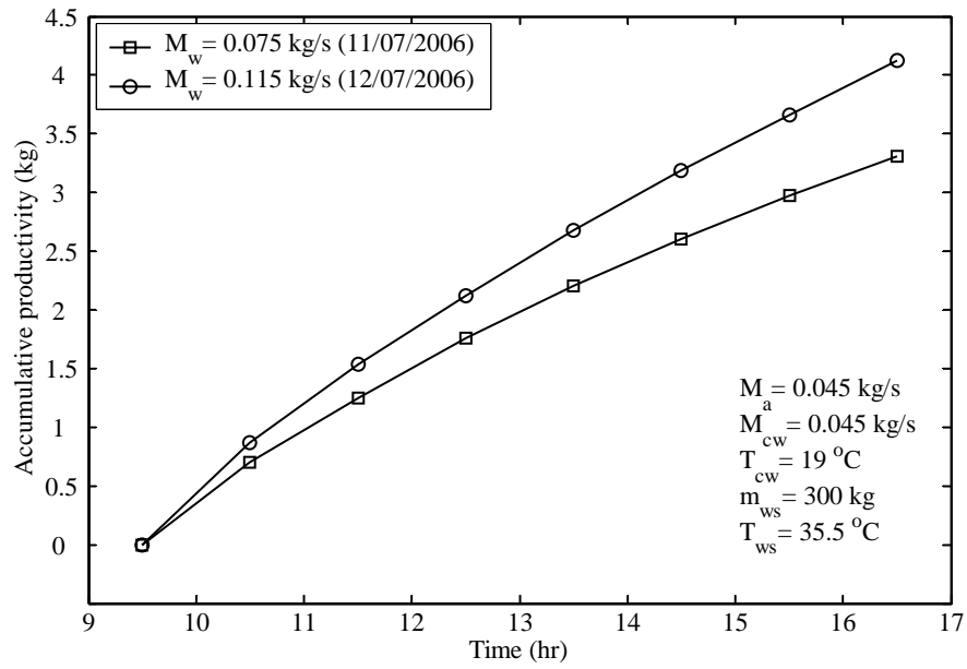
Figure 5.2 Effect of feed water mass flow rate on the system productivity.
