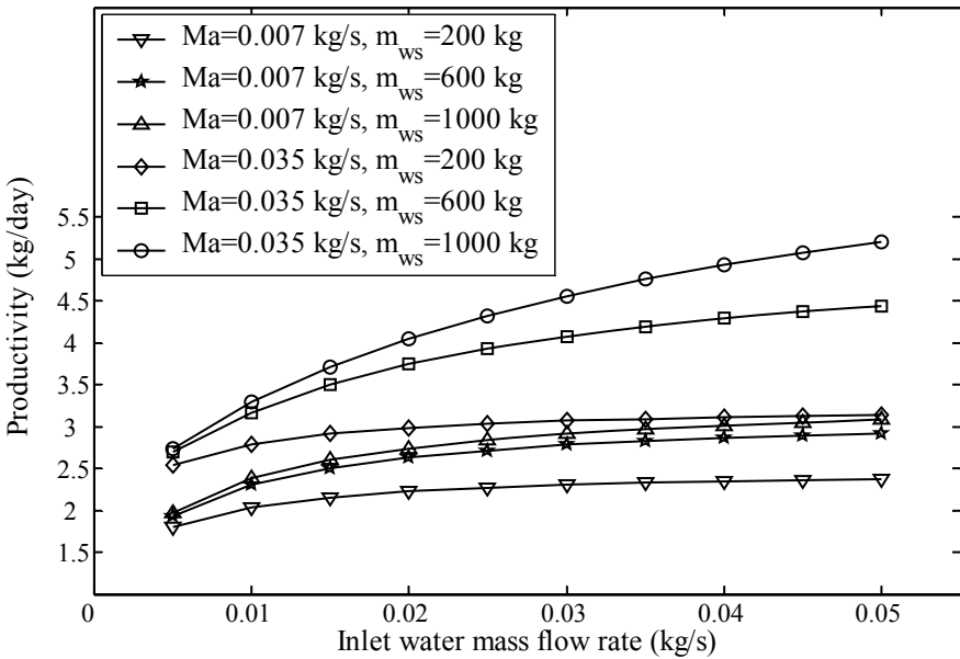
Figure 3.15 The effect of the initial water mass in the storage tank on the system productivity.
