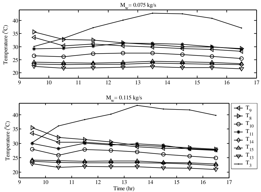
Figure 5.3 Variation of the process air, feed water and cooling water temperatures with time in the system at different water mass flow rates.
