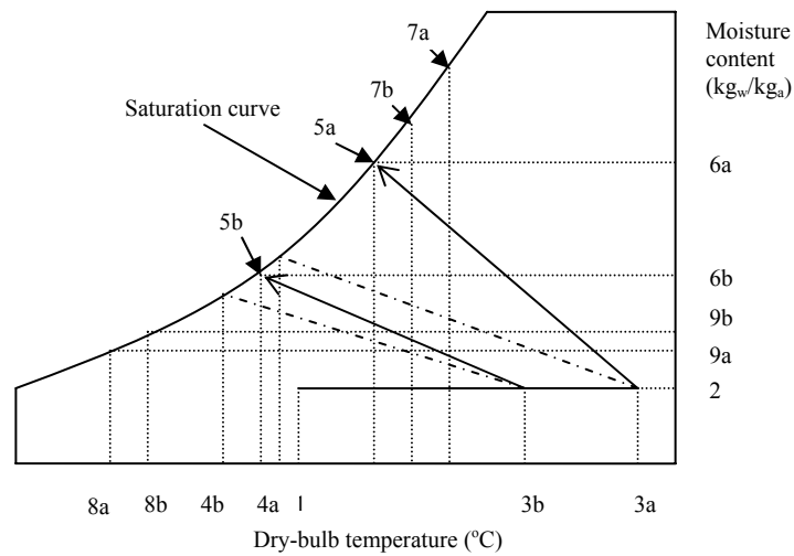
Figure 3.14 Change of state of process air through the system at different air mass flow rates. (1 & 2, represent the state of the air at the inlet of the solar air heater; 3 & 4, represent the state of the air at the inlet of the humidifier; 5 & 6, represent the state of the air leaving the humidifier; 7, represents the inlet water temperature to the humidifier; 8 & 9, represent the state of the air leaving the dehumidifier; a & b, represent the different air mass flow rates ( b > a )).
