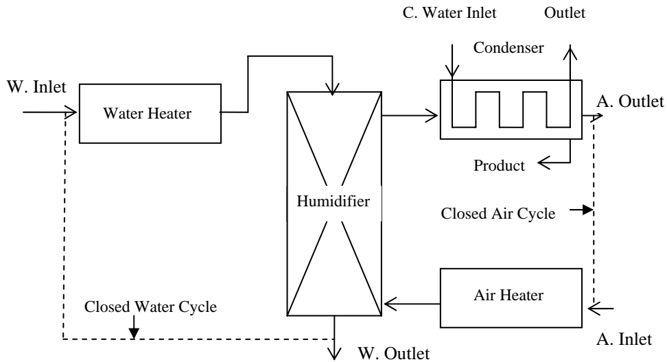
Figure 1.2 A schematic view of a solar water desalination system using humidification-dehumidification technique.
