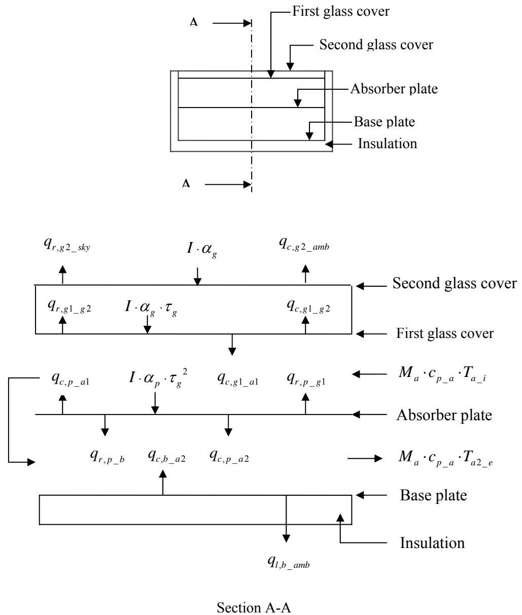
Figure 3.2 Energy balance of the double-pass flat plate solar air heater.
