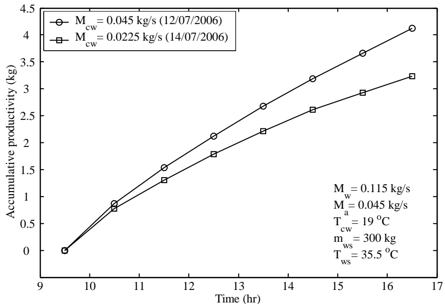
Figure 5.6 Effect of cooling water mass flow rate on the system productivity.
