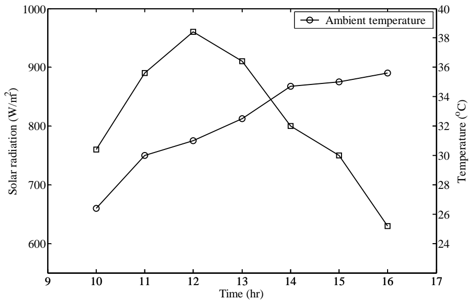
Figure 5.1 Variation of the average solar radiation and ambient temperature with time during the period of 11-16 July 2006.
