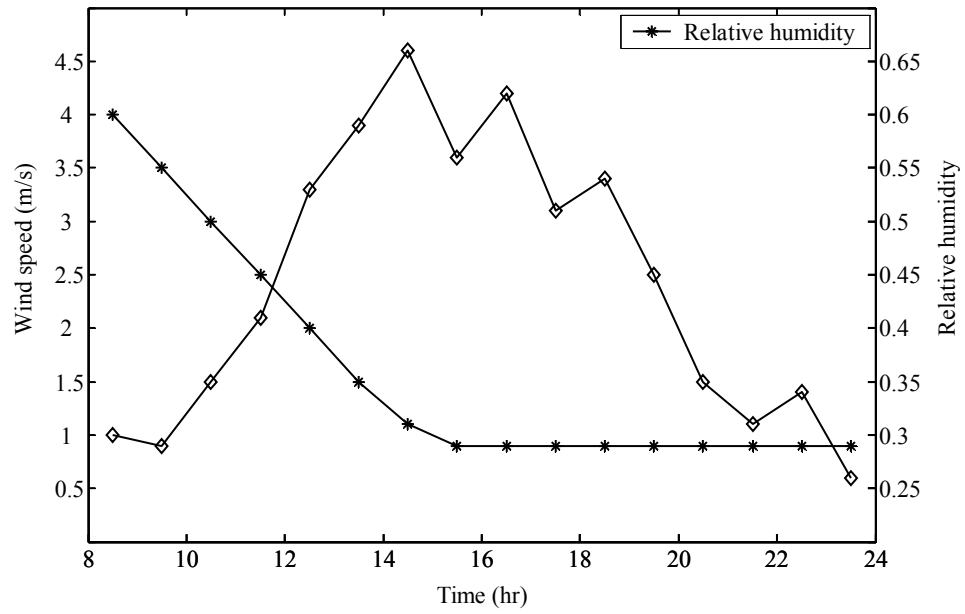
Figure 3.5 Variation of wind speed and relative humidity of the ambient air during the average day of August in Ankara, Turkey.
