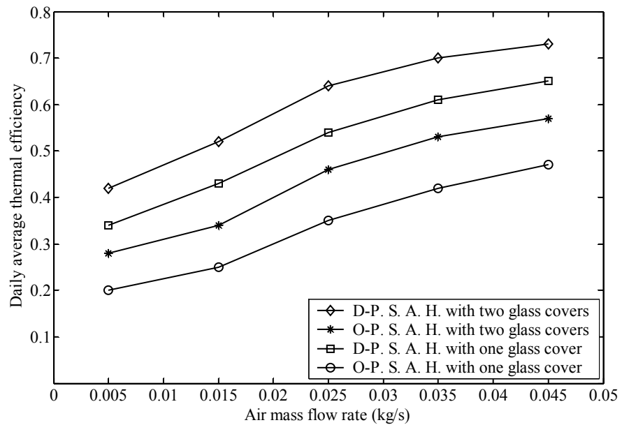
Figure 3.6 Effect of the air mass flow rate on the daily average thermal efficiency of the flat plate solar air heaters.
