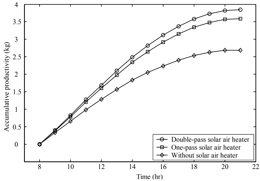
Figure 3.9 The influence of the inclusion of solar air heater and its different configurations on the system productivity.
