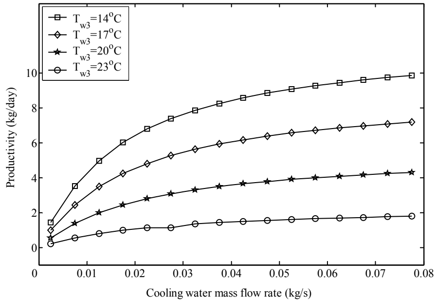
Figure 3.17 The effect of the cooling water mass flow rate on the system productivity.
