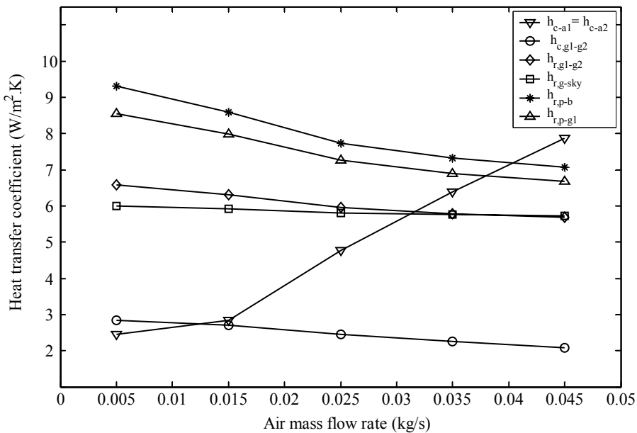
Figure 3.7 Variation of the convective and radiative heat transfer coefficients with air mass flow rate (at 11:30 a.m.)
