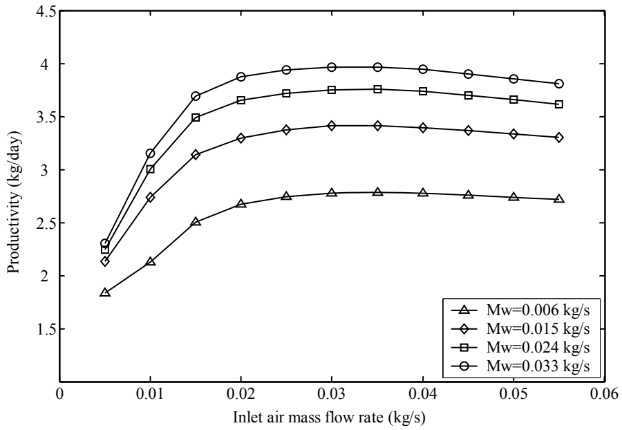
Figure 3.13 The effect of the inlet air mass flow rate on the system productivity.
