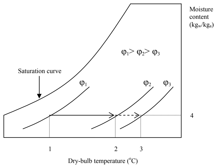
Figure 3.10 Change of state of process air through both the double-pass and single-pass air heater cases. (1, represents the dry-bulb temperature of the air at the inlet of the solar air heater (single and double-pass); 2, represents the dry-bulb temperature of the air leaving the single-pass solar air heater; 3, represents the dry-bulb temperature of the air leaving the double-pass solar air heater; 4, represents the moisture content of the air).
