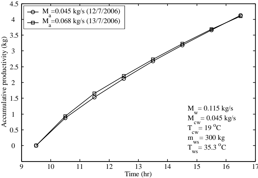
Figure 5.4 Effect of process air mass flow rate on the system productivity.
