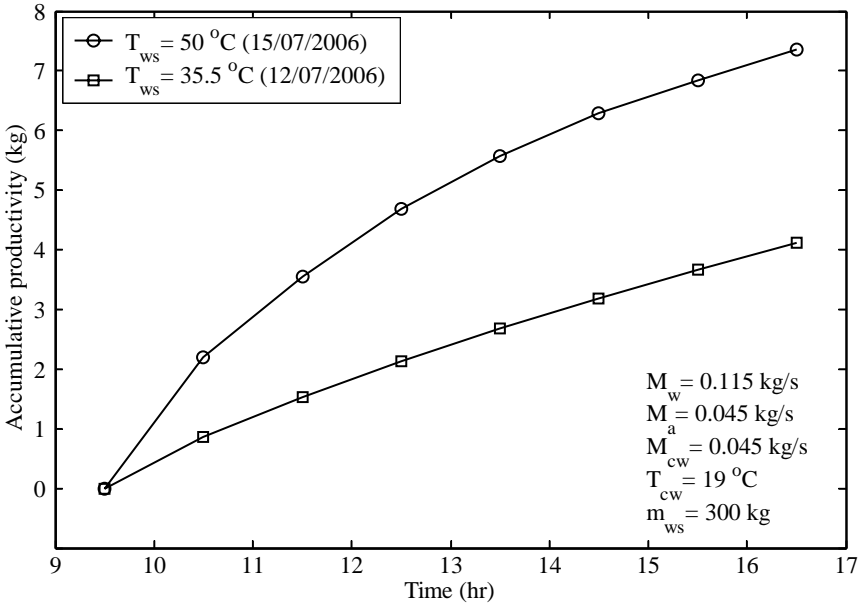
Figure 5.8 Effect of initial water temperature inside the tank on the system productivity.
