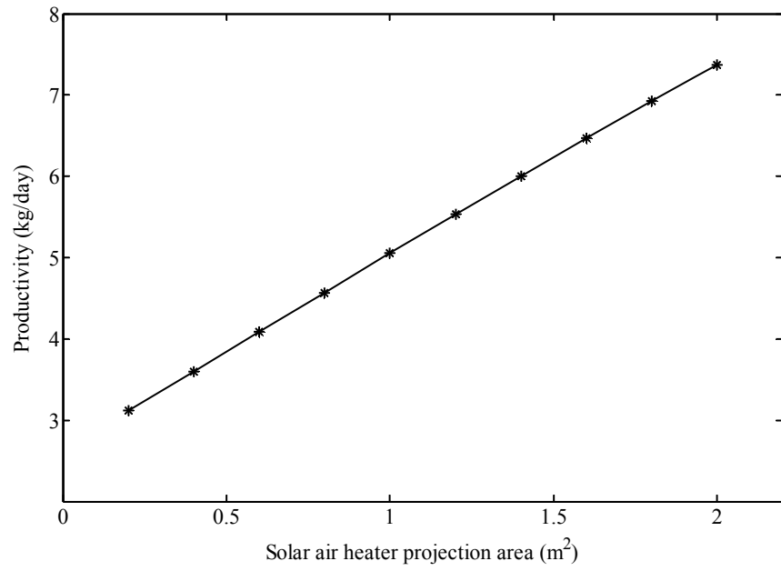
Figure 3.20 The effect of the solar air heater area on the system productivity.
