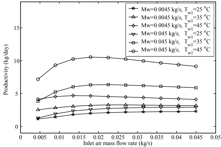
Figure 3.16 The effect of the initial water temperature in the storage tank on the system productivity.
