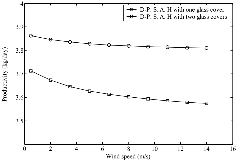
Figure 3.18 The effect of the wind speed on the system productivity.
