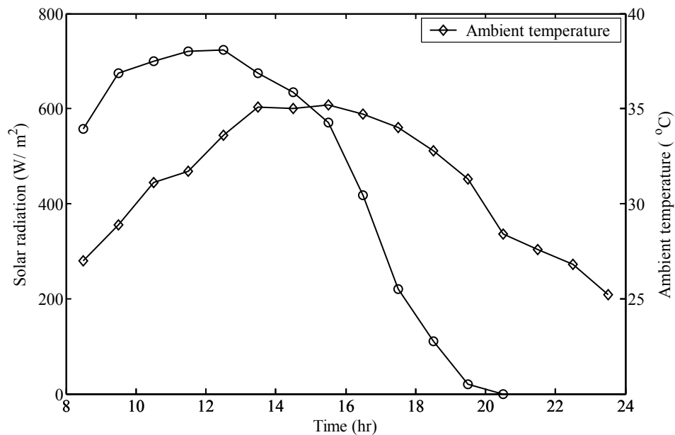
Figure 3.4 Variation of global solar radiation and ambient temperature during the average day of August in Ankara, Turkey.
