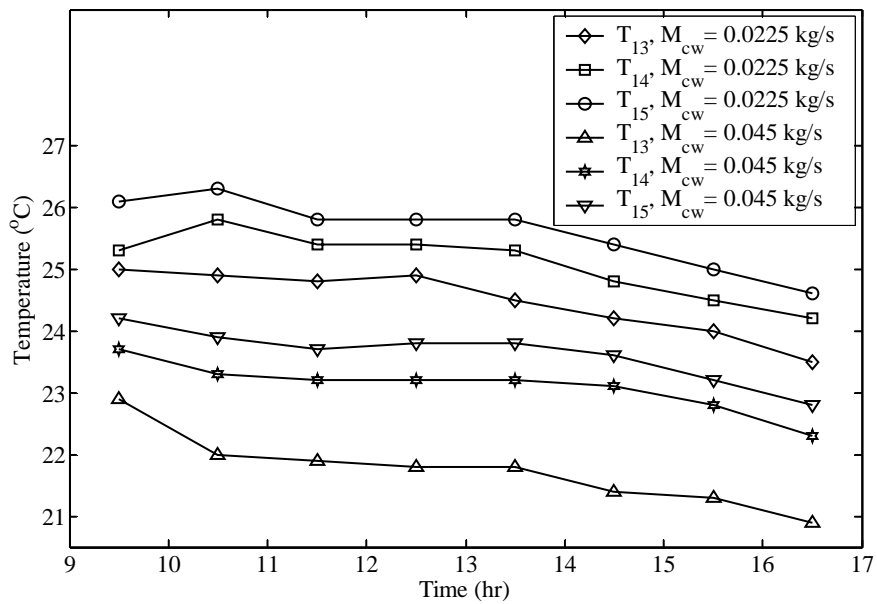
Figure 5.7 Variation of the process air and cooling water temperatures with time at the exit of the dehumidifier at different cooling water mass flow rates.
