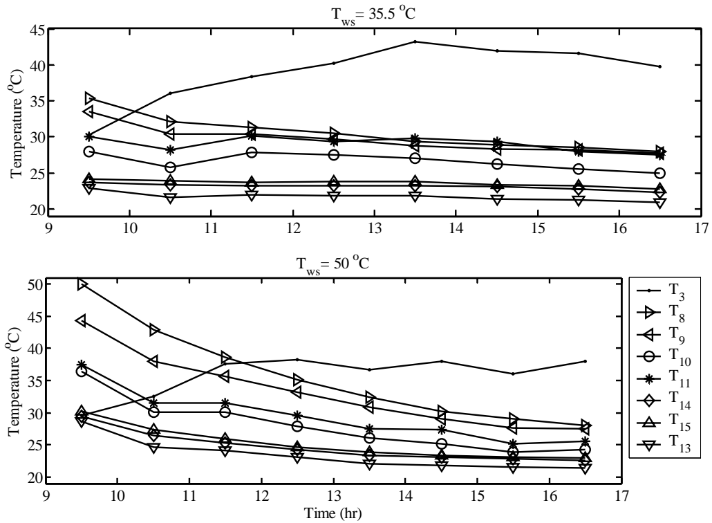
Figure 5.9 Variation of the process air, feed water and cooling water temperatures with time in the system at different initial water temperatures inside the tank.
