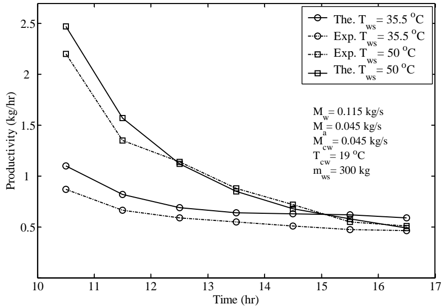
Figure 5.18 Comparison between experimental and theoretical results at different values of the initial water mass inside tank.
