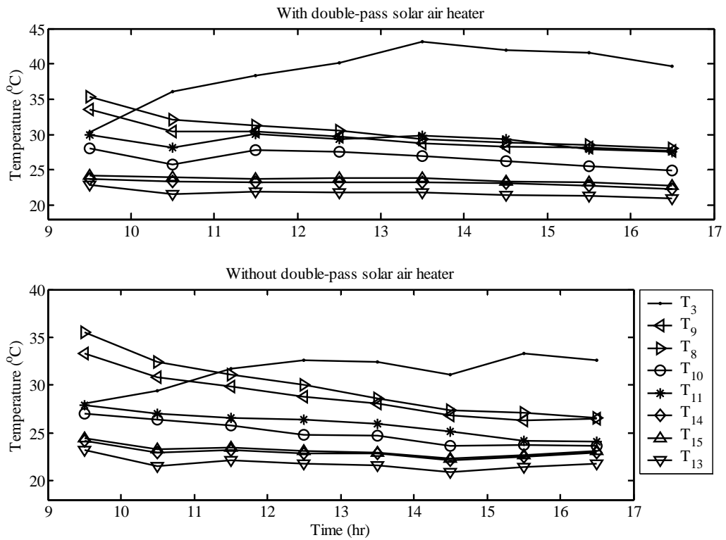
Figure 5.13 Variation of the process air, feed water and cooling water temperatures with time in the system with and without solar air heater.
