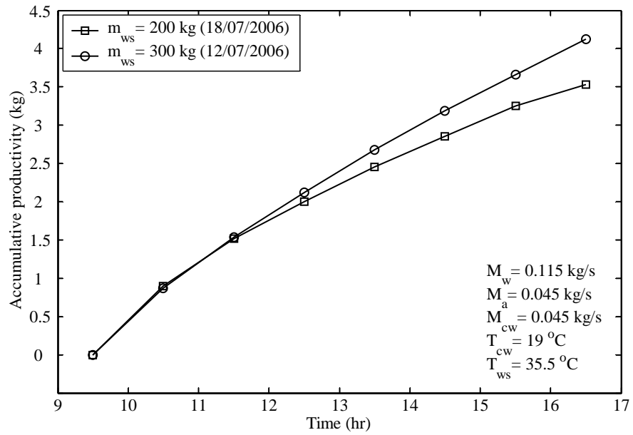
Figure 5.10 Effect of initial water mass inside the tank on the system productivity.
