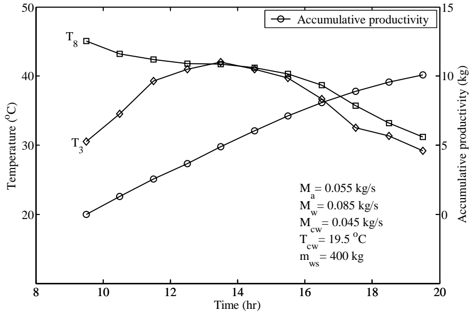
Figure 5.20 The performance of the system integrated with an evacuated tubular solar water heater unit.
