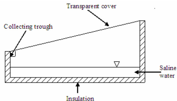
Figure 1.1 A schematic drawing of the simple basin type solar still.
