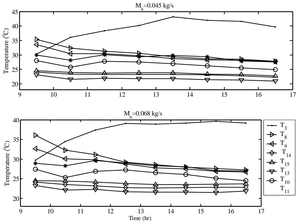
Figure 5.5 Variation of the process air, feed water and cooling water temperatures with time in the system at different air mass flow rates.
