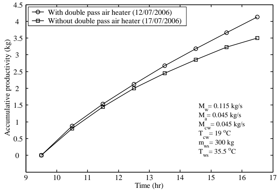
Figure 5.12 Effect of double-pass solar air heater on the system productivity.
