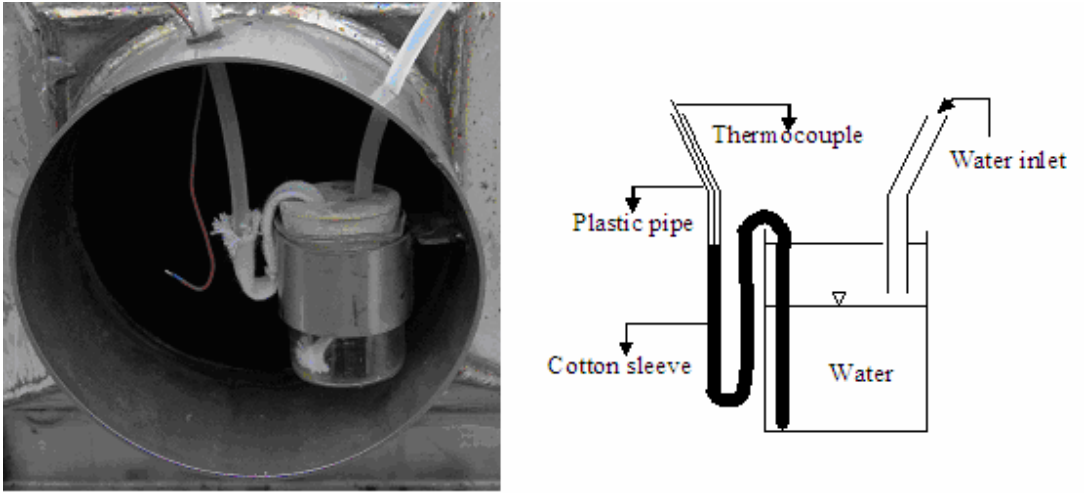
Figure 4.8 Wet-bulb temperature measurement of the air.
