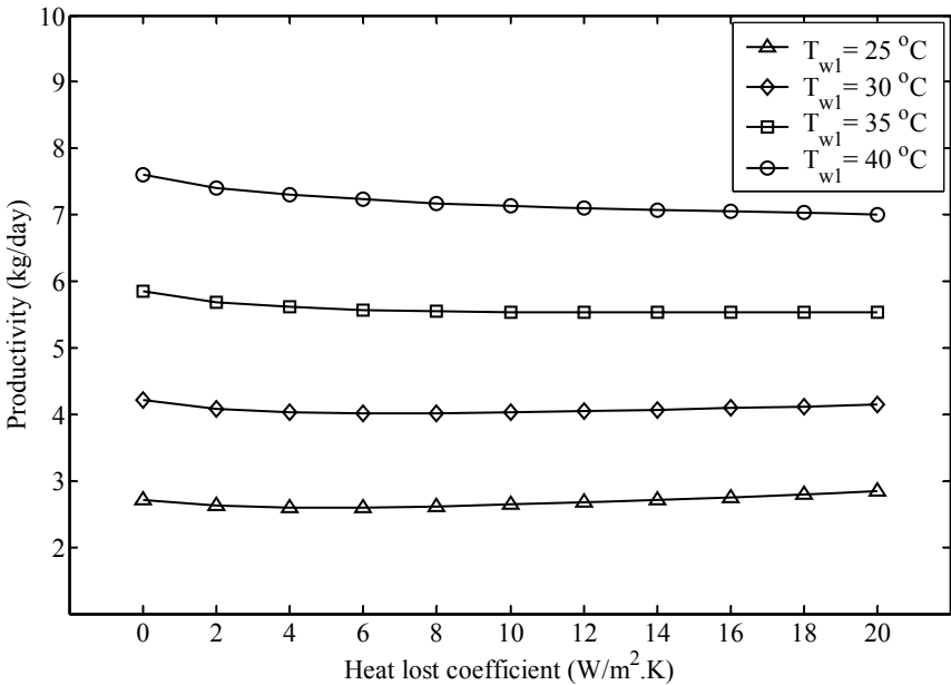
Figure 3.19 The effect of the bottom heat loss coefficients of the solar air heater and the water storage tank on the system productivity.
