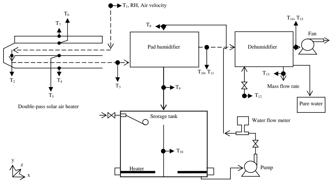
Figure 4.14 Schematic drawing of the set-up and the thermocouple locations.
