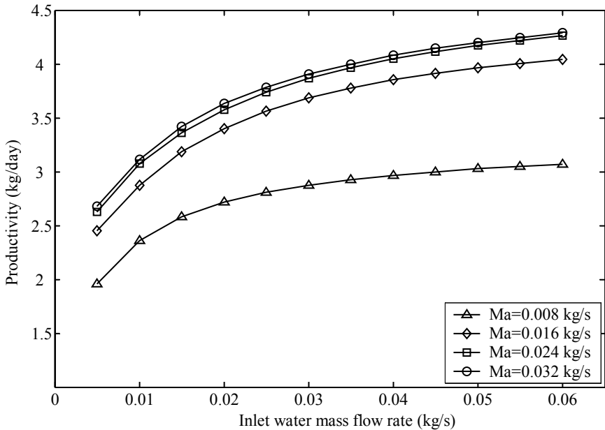
Figure 3.11 The effect of the humidifier inlet water mass flow rate on the system productivity.
