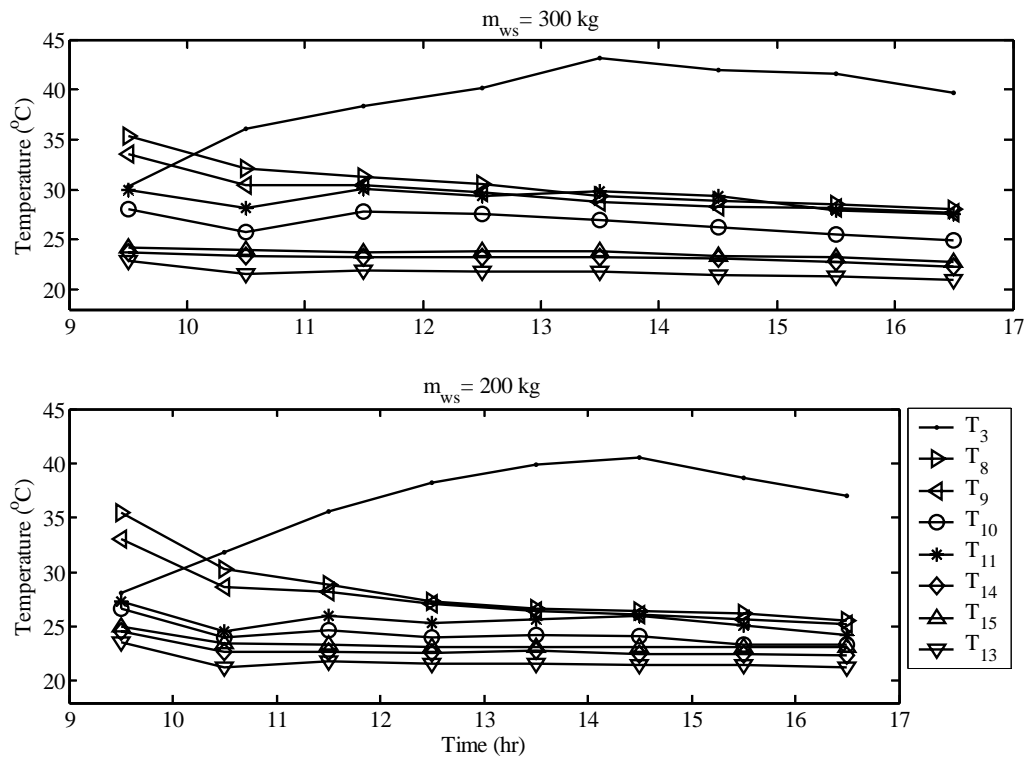
Figure 5.11 Variation of the process air, feed water and cooling water temperatures with time in the system at different initial water mass inside the tank.
