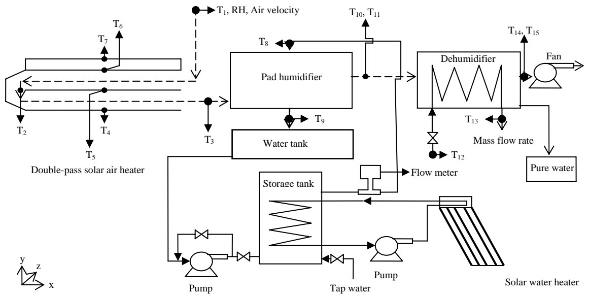
Figure E.2 Schematic drawing of the set-up integrated with an evacuated tubular solar water heater system and the thermocouple locations.
