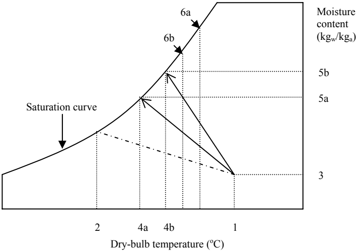
Figure 3.12 Change of state of process air through the humidifier at different water mass flow rates. (1, 2 & 3, represent the state of the air at the inlet of the humidifier; 4 & 5, represent the state of the air leaving the humidifier; 6, represents the inlet water temperature to the humidifier; a & b, represent the different water mass flow rates ( b > a )).
