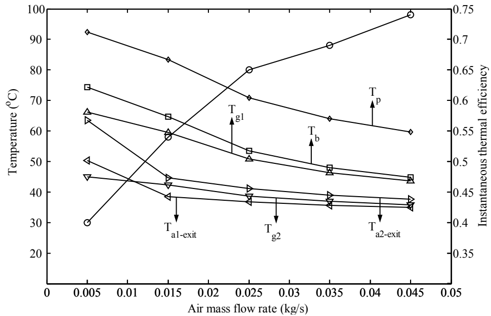
Figure 3.8 Effect of the air mass flow rate on the instantaneous thermal efficiency, temperature of the process air and different air heater components (at 11:30 a.m.).
