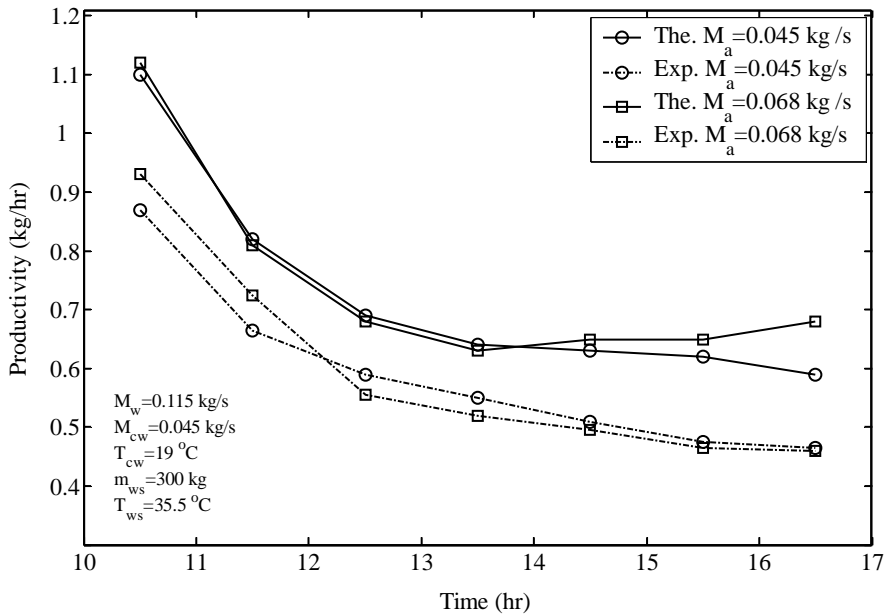
Figure 5.16 Comparison between experimental and theoretical results at different values of the air mass flow rate.
