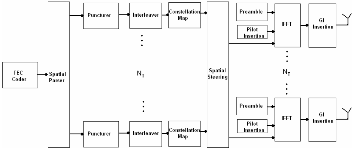
Figure 2.9 MIMO-OFDM Transmitter.
