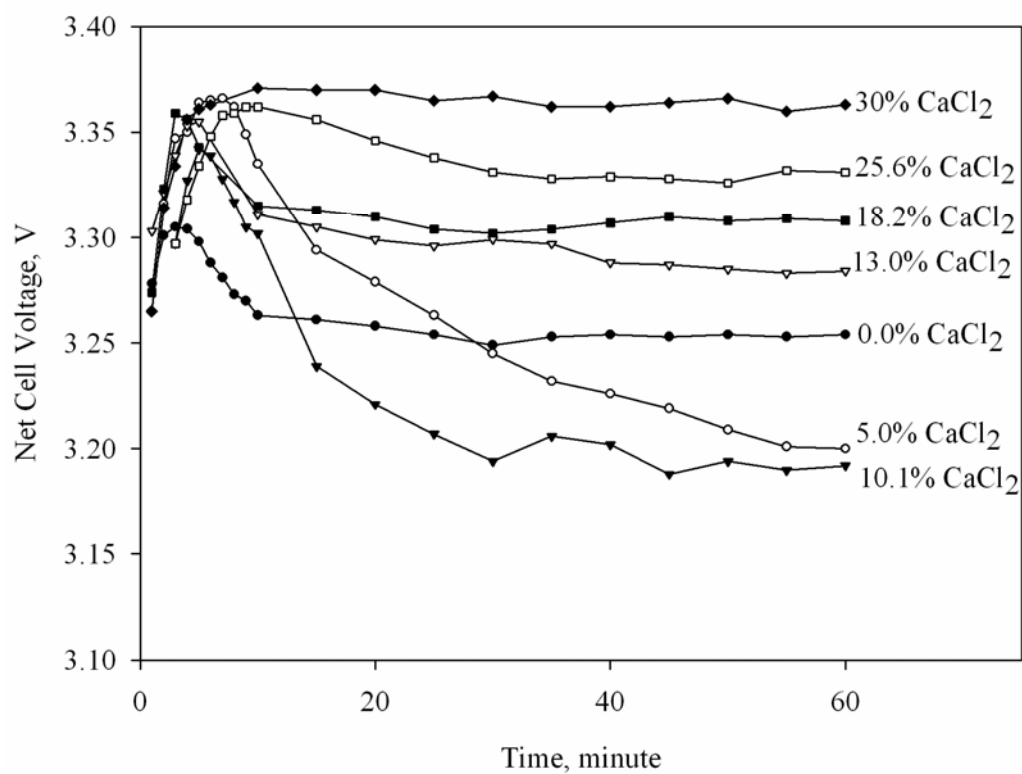
Figure 58 Net cell voltage vs. time at 13 mm ACD for experiments involving the effect of \text{CaCl}_2 .
