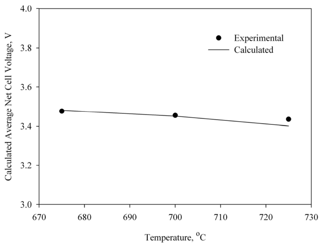
Figure 43 Calculated average net cell voltages for the experiments involving the effect of temperature.
