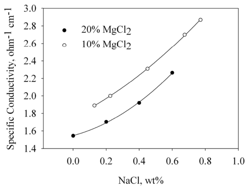
Figure 50 Specific conductivity of the \text{MgCl}_2 - \text{NaCl} - \text{KCl} electrolyte.
