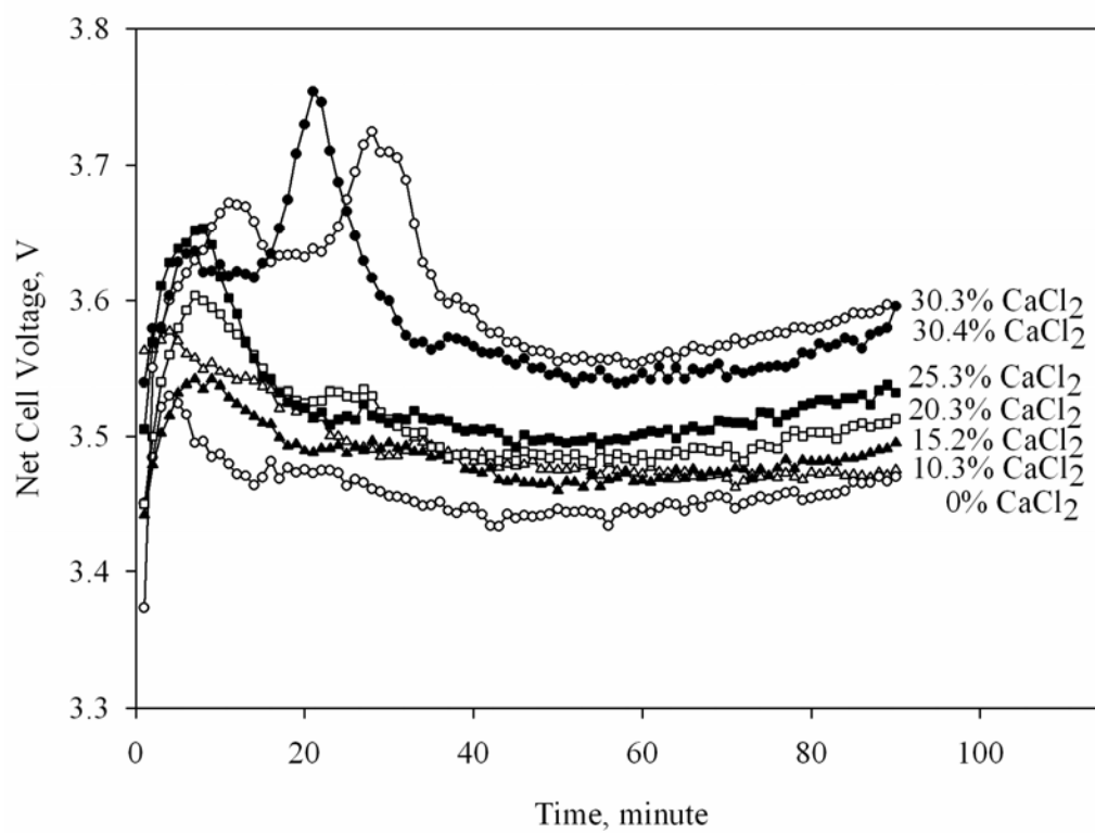
Figure 59 Net cell voltage vs. time at 20 mm ACD for the experiments involving the effect of \text{CaCl}_2 .
