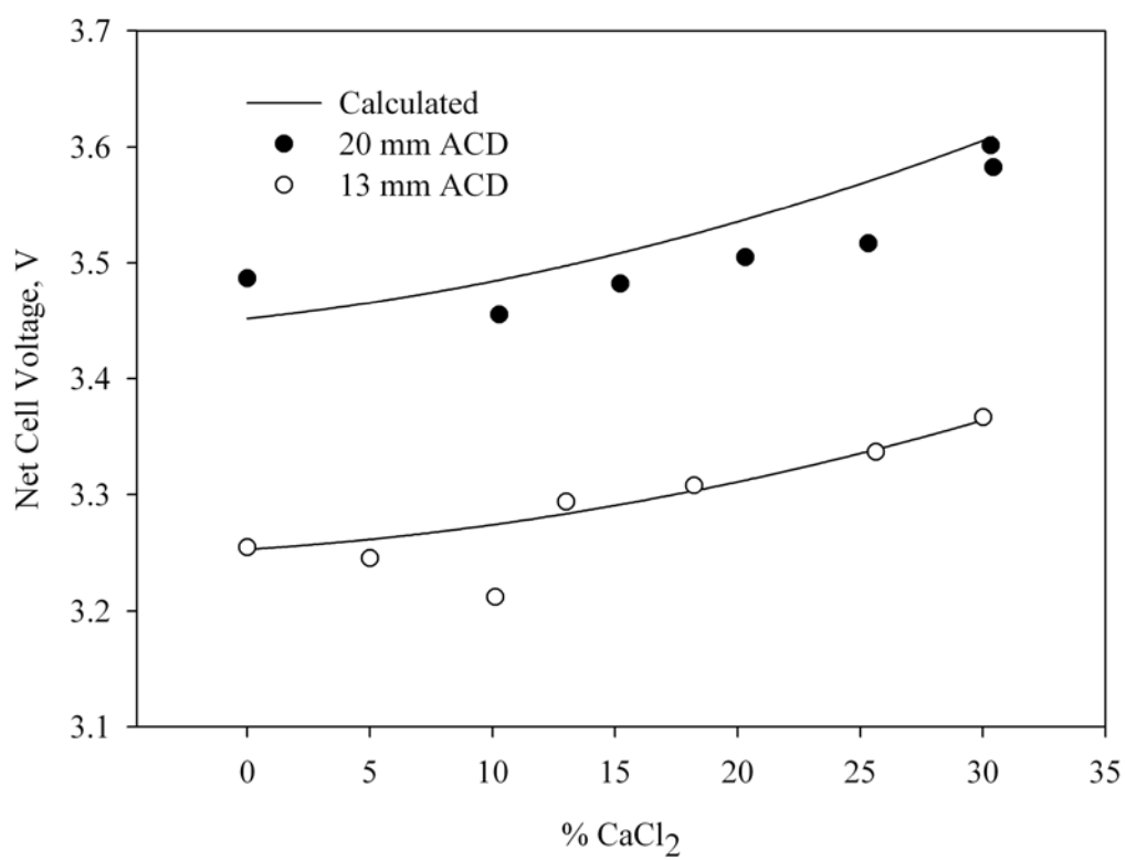
Figure 65 Calculated and experimental cell voltages for the experiments involving the effect of \text{CaCl}_2 .
