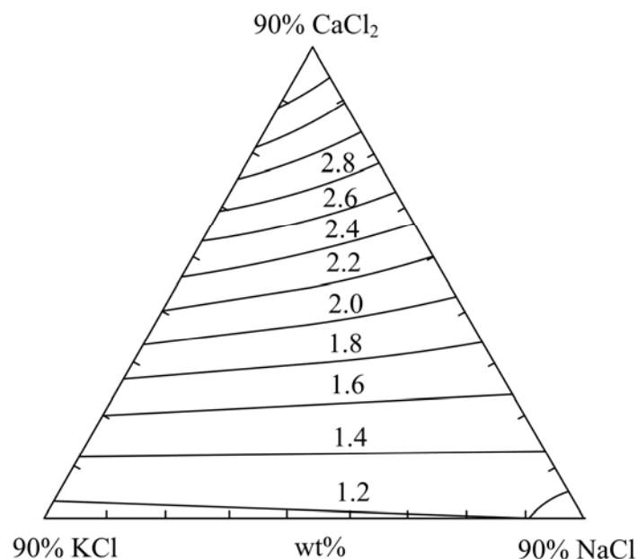
Figure 7 Densities, \text{g}\cdot\text{cm}^{-3} , for 10% \text{MgCl}_2 -KCl-NaCl- \text{CaCl}_2 system at 750°C [28].
