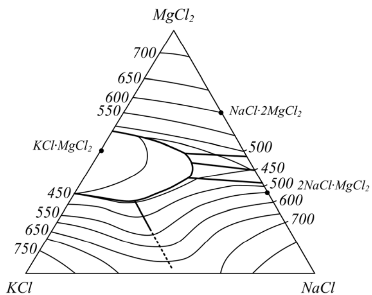
Figure 2 Liquidus surface of the system \text{MgCl}_2 -KCl-NaCl [23].
