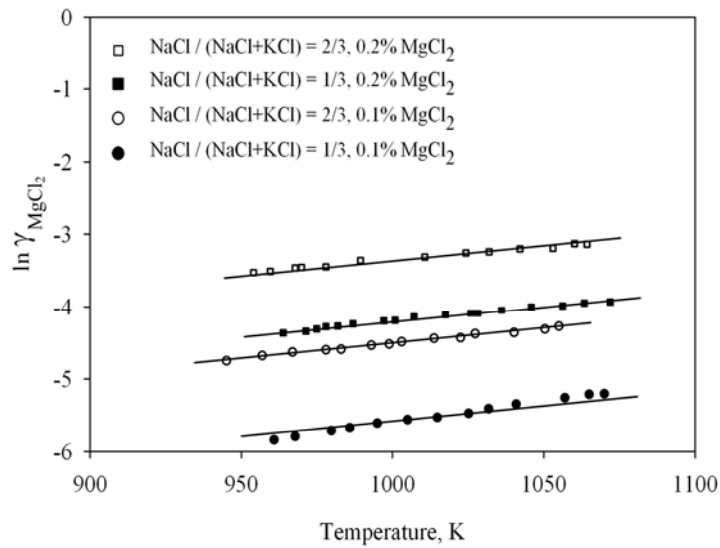
Figure 38 The change in \text{MgCl}_2 activity coefficient with temperature [57].
