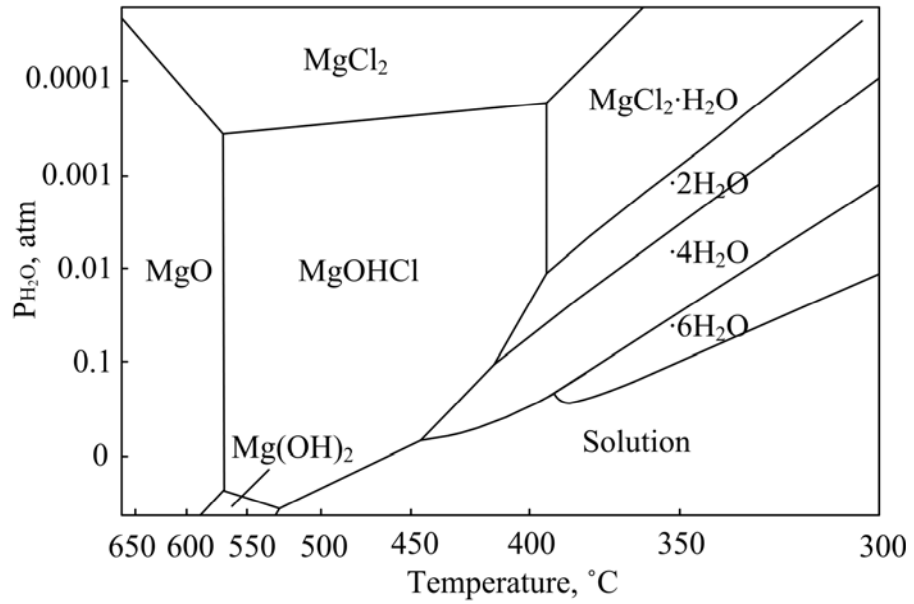
Figure 12 Stability regions of magnesium chloride hydrates under \text{H}_2\text{O} pressure, P_{\text{HCl}} = 0.001 \text{ atm} [29].
