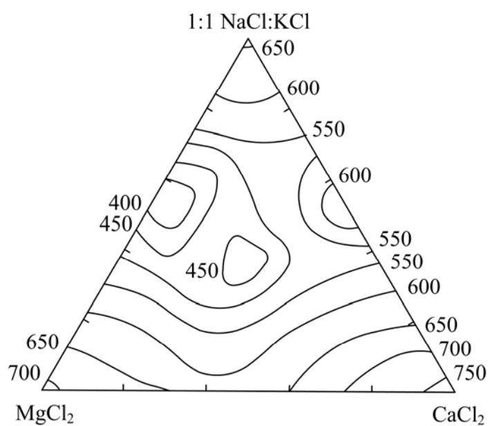
Figure 3 Liquidus surface of the system \text{MgCl}_2 - \text{CaCl}_2 -1:1 (KCl:NaCl) showing some of the isotherms [24].
