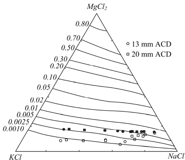
Figure 49 \text{MgCl}_2 isoactivity lines in \text{MgCl}_2 - \text{NaCl} - \text{KCl} ternary [50].
