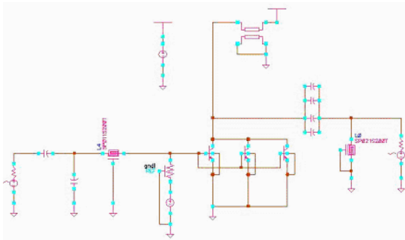
Figure 4.23: Cadence test setup for testing the CPW structure
