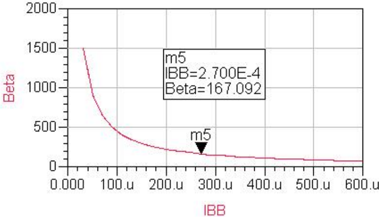
Figure 3.4: Beta versus IBB at ICE which is specified by the marker m1
