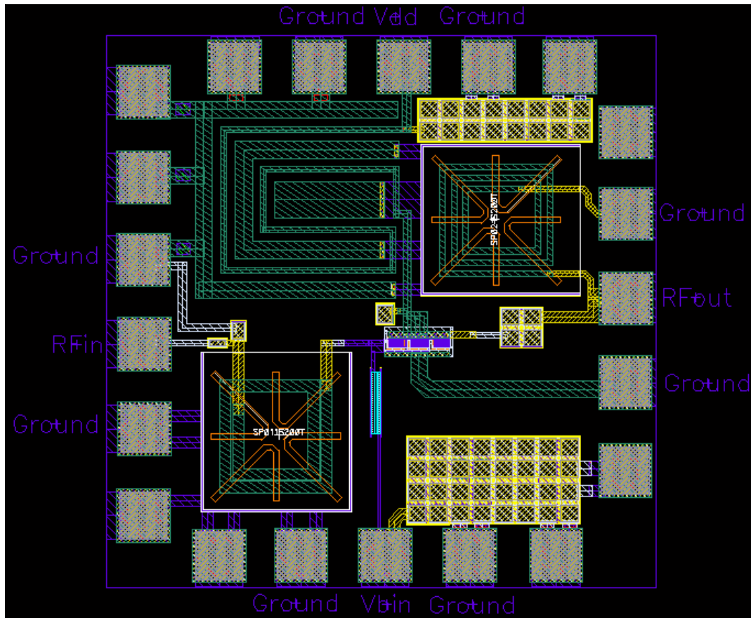
Figure 4.34: Layout of the single stage PA with the CPW Structure in Figure 4.35
