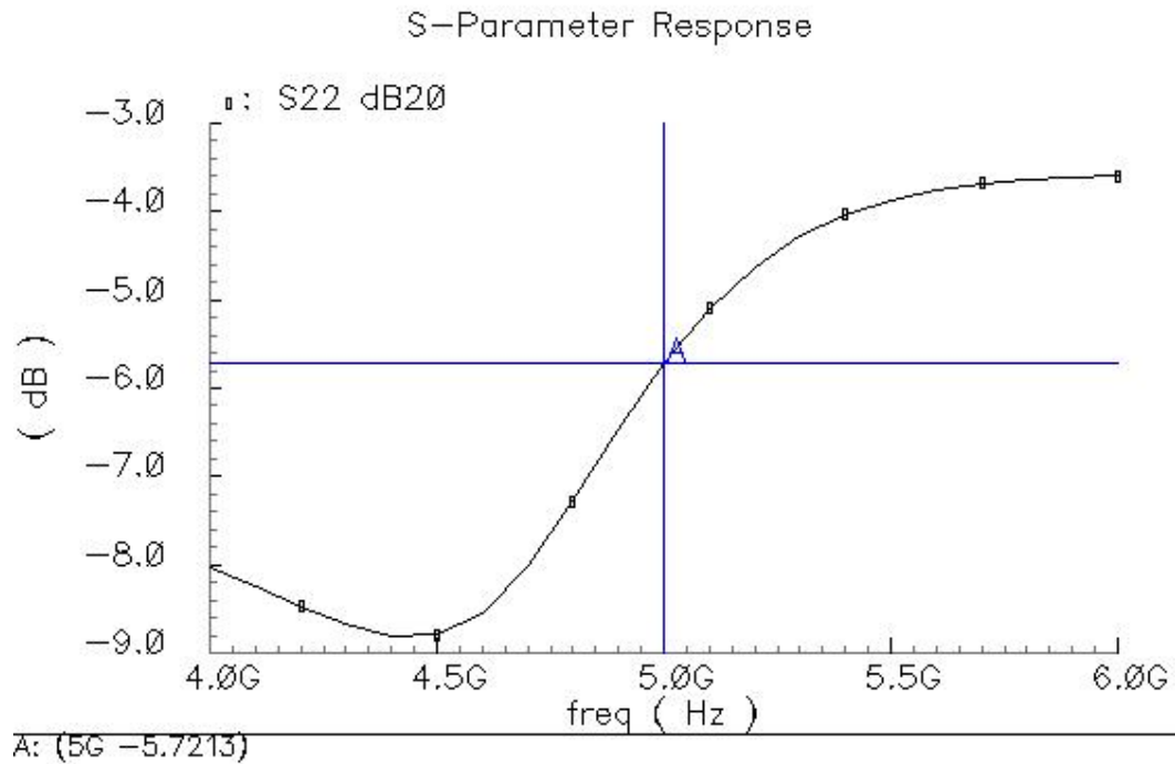
Figure 4.5: s_{22} response
