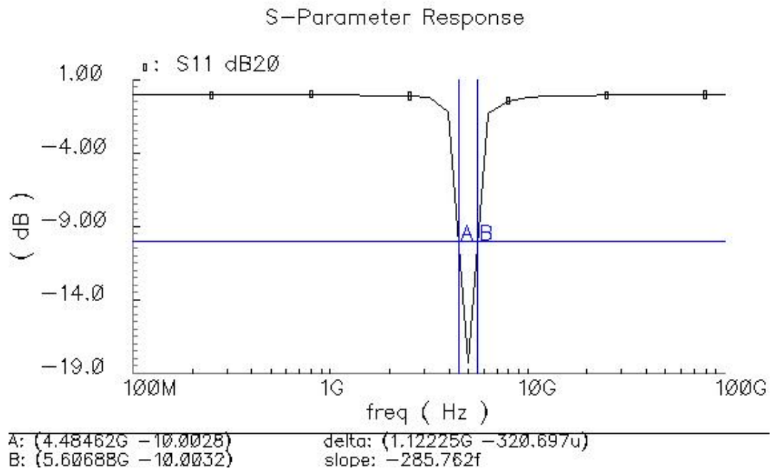
Figure 4.4: (a) s_{11} response (b) frequency bandwidth in which s_{11} drops below -10 dB
