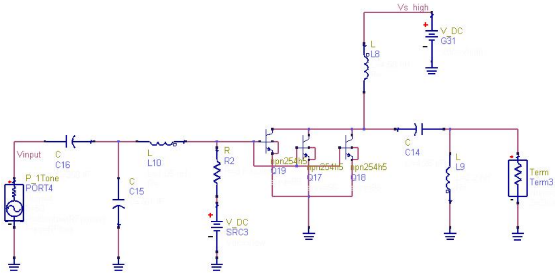
Figure 3.12: Class A PA schematic with ideal elements in ADS
