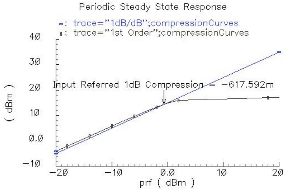
Figure 4.2: Input referred 1 dB compression point (Gain=14.95 dB at 1 dB compression point)
