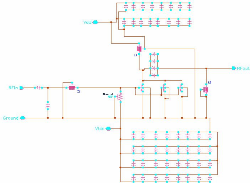
Figure 4.8: Final schematic of single stage PA
