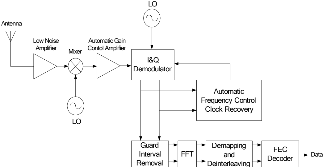
Figure 2.4: Block diagram of an IEEE 802.11a receiver
