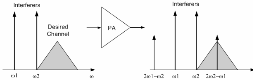
Figure 2.8: Corruption of the desired signal due to nearby interferers
