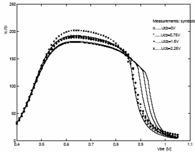
Figure A.3: Beta plots of a bipolar transistor (npn254h5; 24µm emitter length) for a typical wafer
