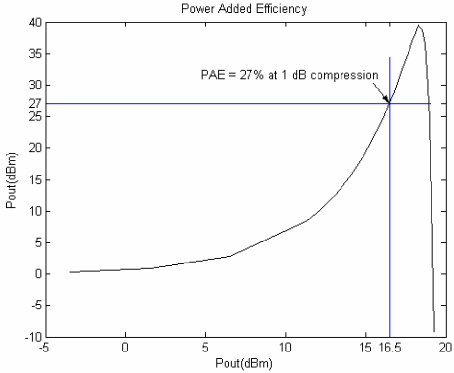
Figure 4.26: Power added efficiency
