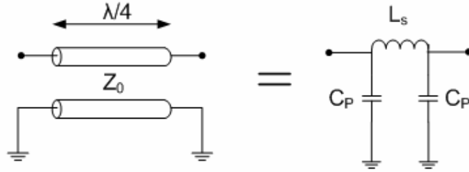
Figure 3.17: “Pi” LC network model of a quarter wavelength transmission line
