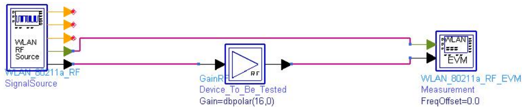
Figure 4.16: ADS setup for the IEEE 802.11a PA EVM measurements
