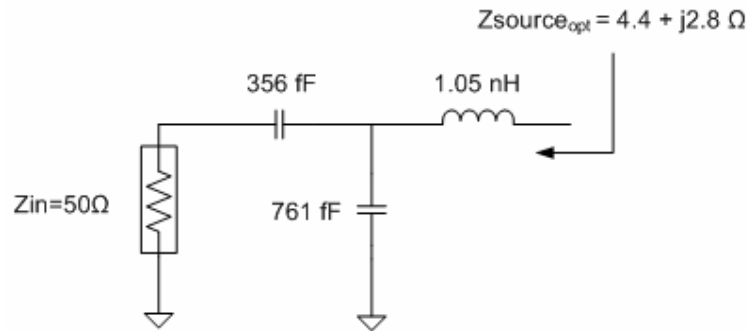
Figure 3.11: Input matching network
