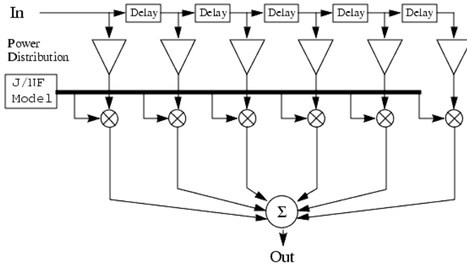
Figure A.1: Delay and Doppler Spread and Carrier Phase Shift
