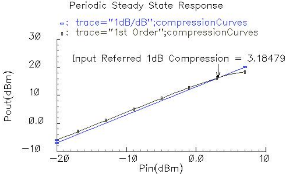
Figure 4.19: Input referred 1 dB compression point (Gain=13 dB at 1 dB compression point)
