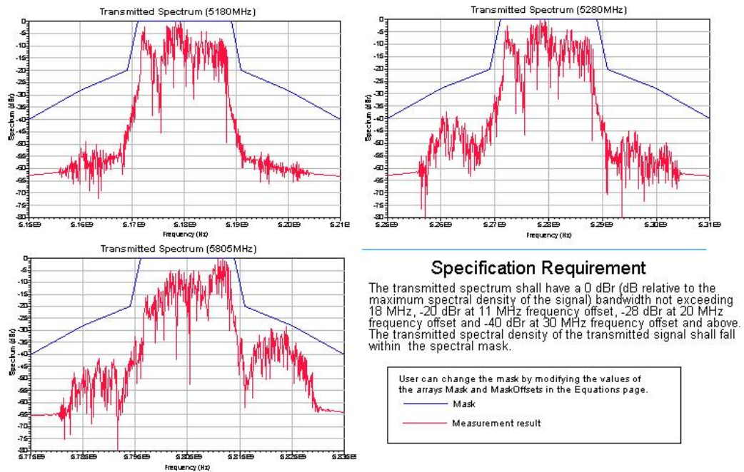
Figure 4.15: 802.11a transmit spectrum mask measurement results in the presence of WLAN channel model A
