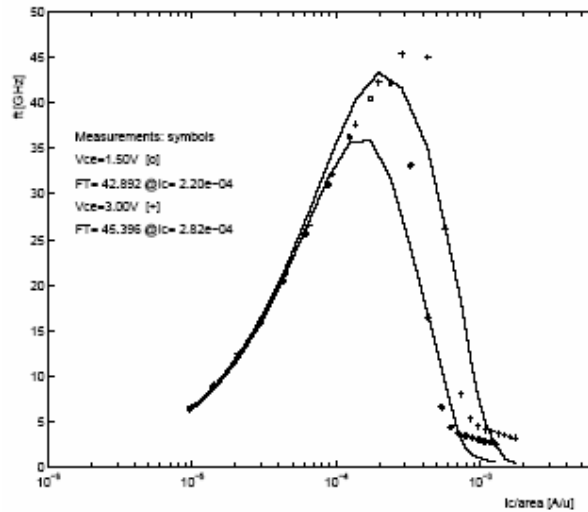
Figure A.4: Ft plots of a bipolar transistor (npn254h5; 12µm emitter length) for a typical wafer
