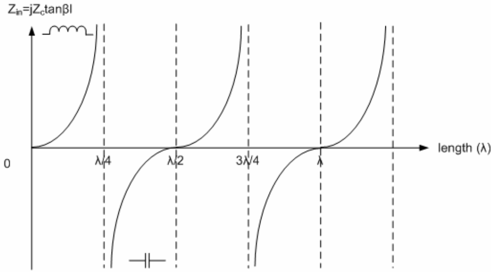
Figure 3.21: Input impedance versus length
