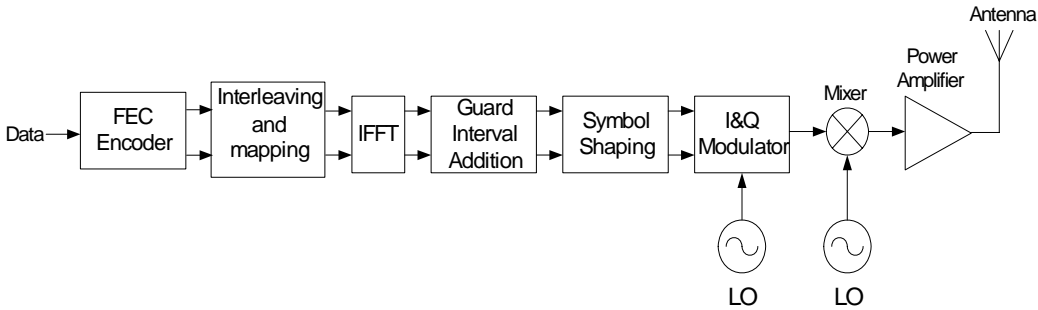
Figure 2.3: Block diagram of an IEEE 802.11a transmitter
