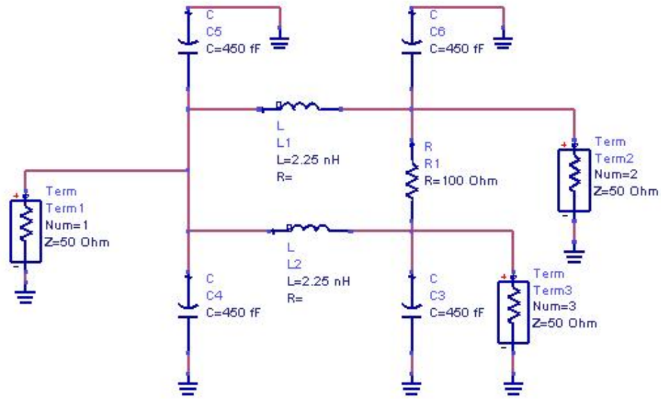
Figure 3.18: Lumped element Equal split Wilkinson power divider at 5GHz center frequency
