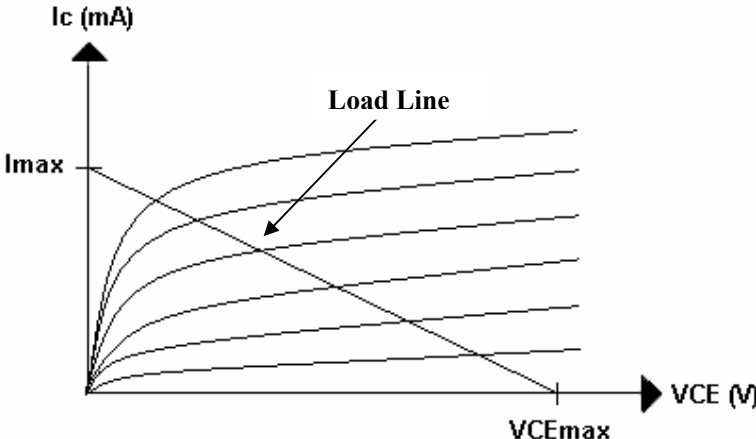
Figure 2.12: I-V characteristics of a transistor
