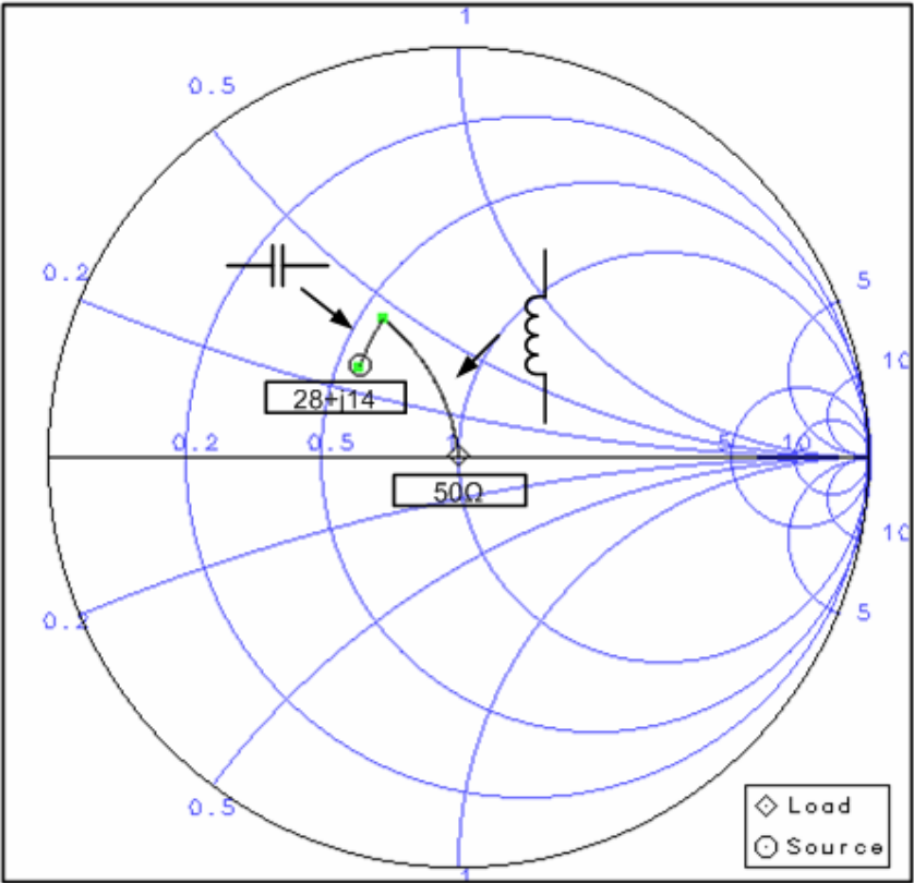
Figure 3.8: Output matching network design using ADS Smith Chart utility
