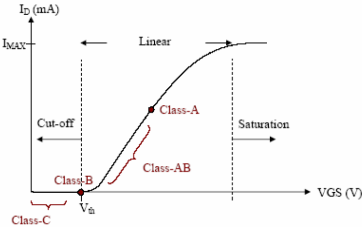
Figure 2.14: Q point of Class A, AB, B and C PAs
