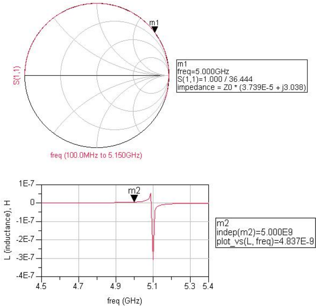
Figure 3.25: Inductance of capacitively loaded coplanar waveguide model
