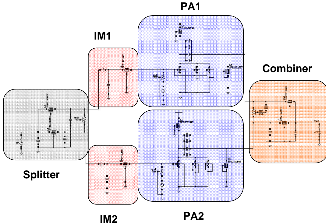
Figure 4.18: Combined power amplifier
