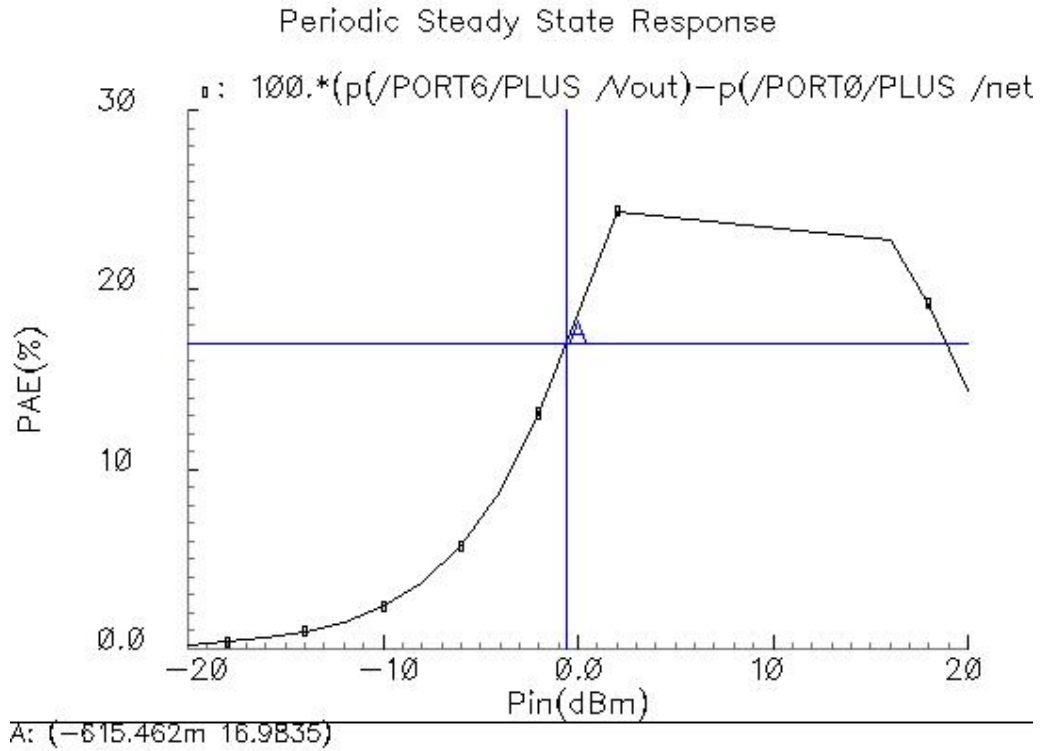
Figure 4.3: Power Added Efficiency (PAE)
