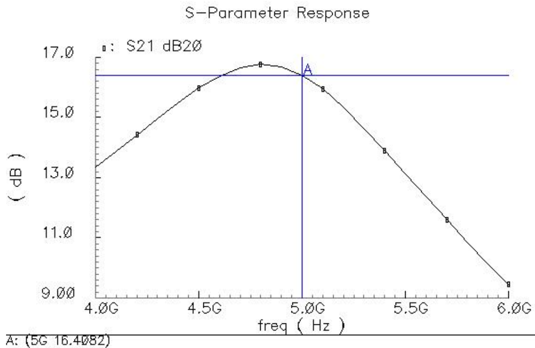
Figure 4.6: Power gain
