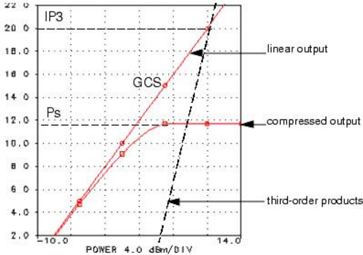
Figure 4.12: Important PA metrics
