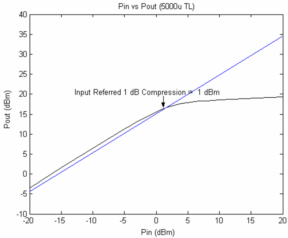
Figure 4.25: Input referred 1 dB compression point (Gain=15.5 dB at 1 dB compression point)
