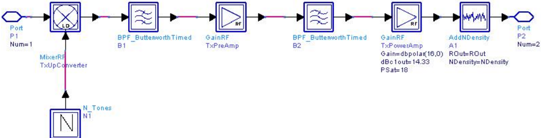
Figure 4.11: WLAN 802.11a transmitter
