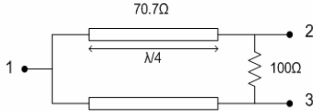
Figure 3.16: Microstrip Wilkinson combiner
