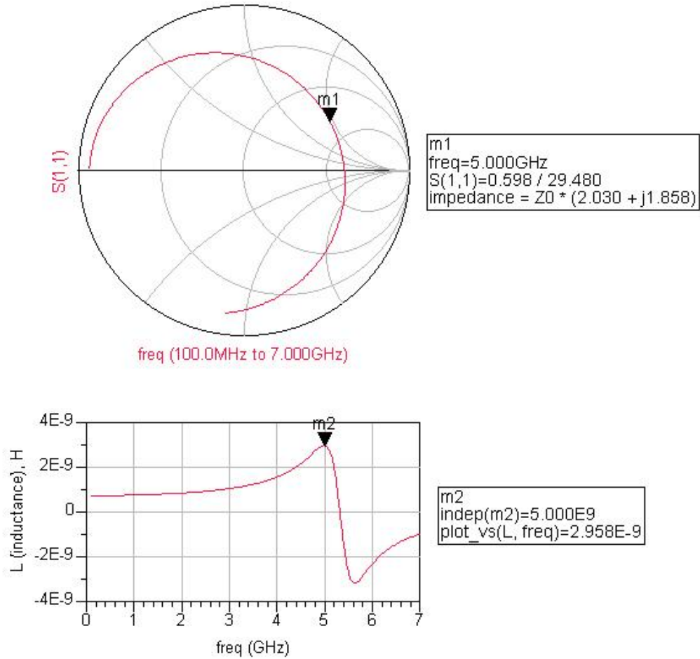
Figure 4.31: Inductance of the CPW structure in Figure 4.33
