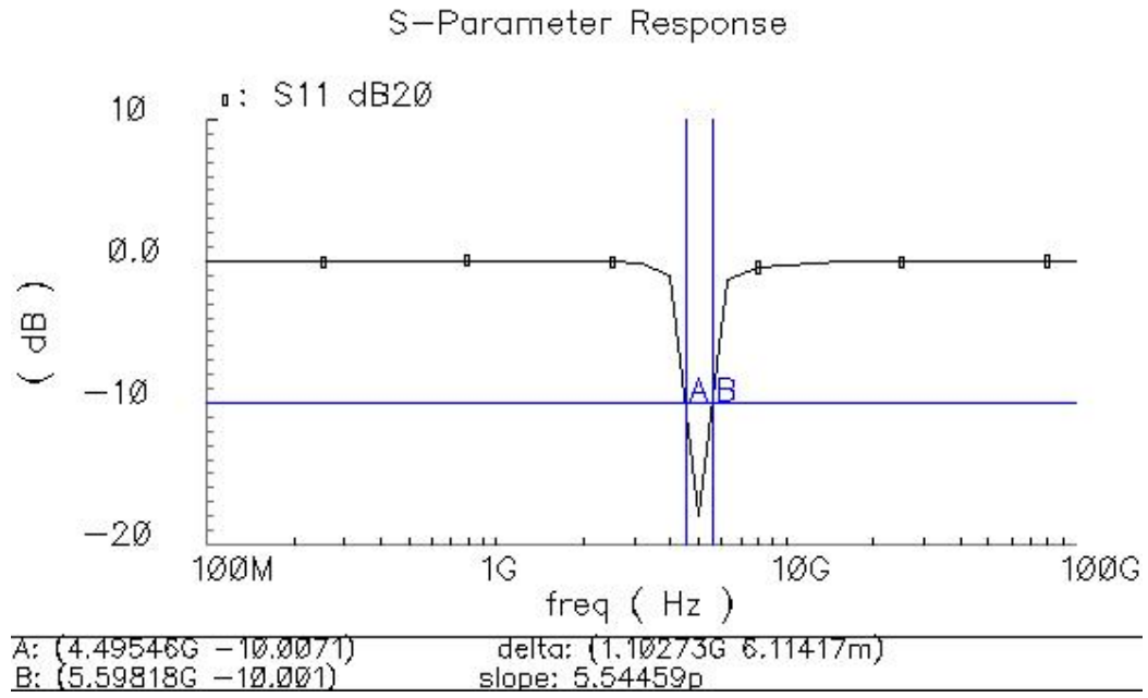
Figure 4.27: (a) s_{11} response (b) s_{11} in a logarithmic scale ( s_{11} is below -10 dB from 4.5 GHz to 5.6 GHz)
