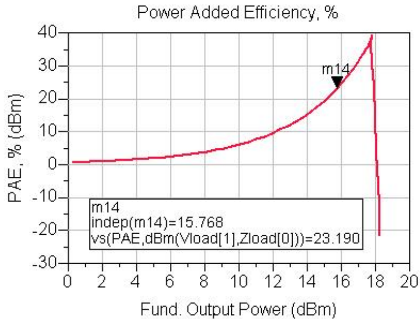
Figure 3.14: Single stage Class A PAE curve
