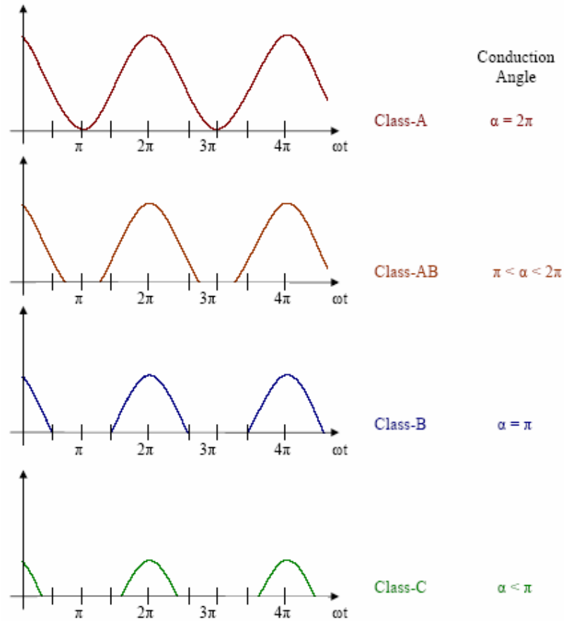
Figure 2.15: Summary of Class A, AB, B and C conduction angles
