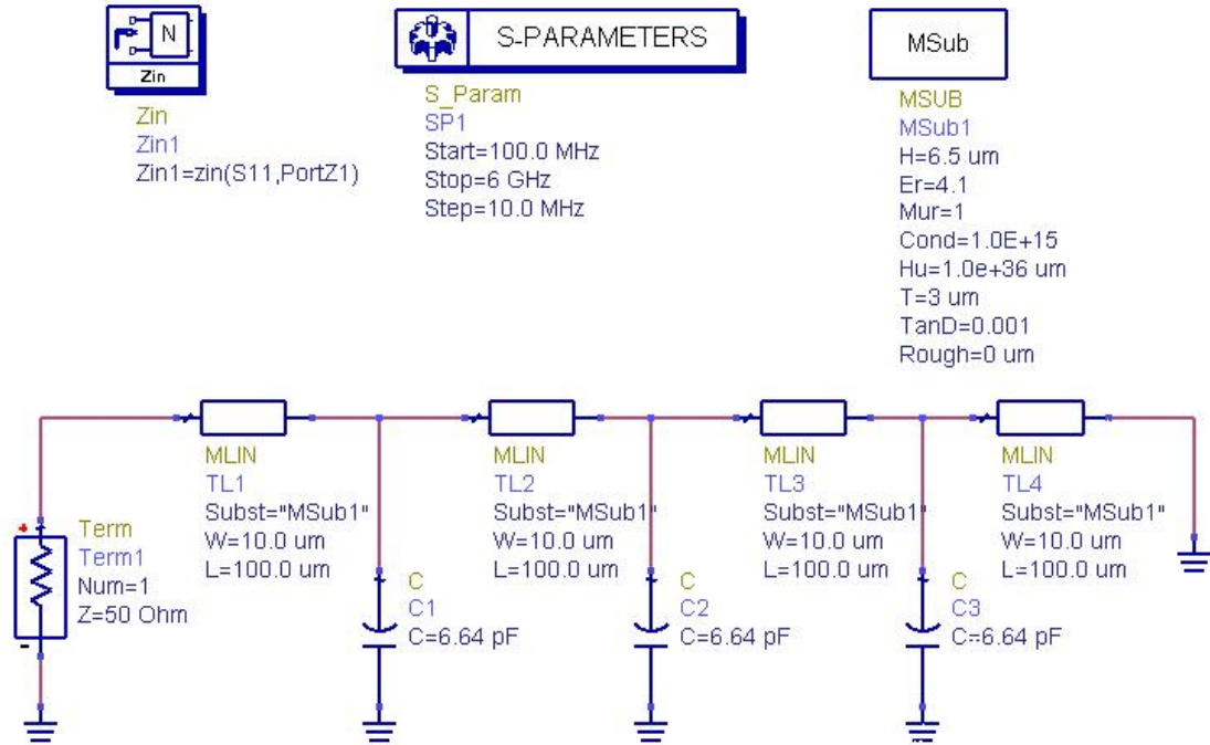
Figure 3.22: Capacitively loaded microstrip line model
