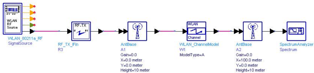
Figure 4.14: ADS setup for the IEEE 802.11a transmit RF spectrum measurements in the presence of WLAN channel model A
