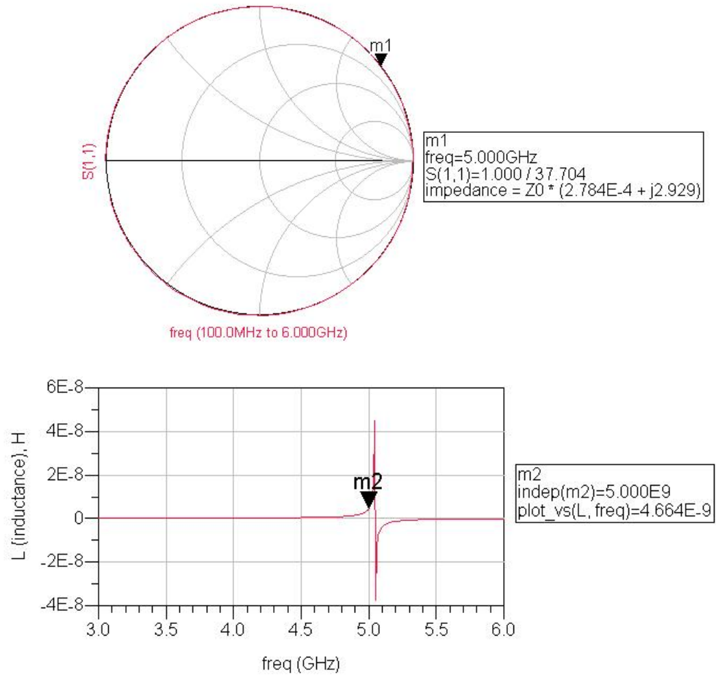
Figure 3.23: Inductance of capacitively loaded microstrip line model
