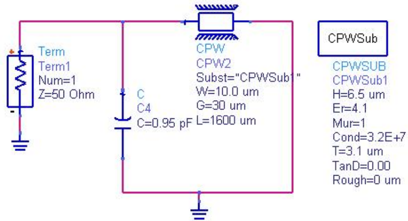
Figure 4.32: CPW structure
