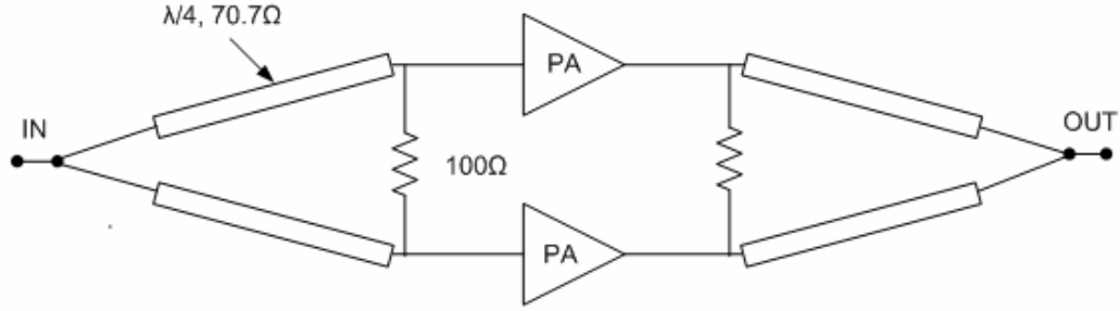
Figure 3.15: In-phase power combining using Wilkinson power combiners
