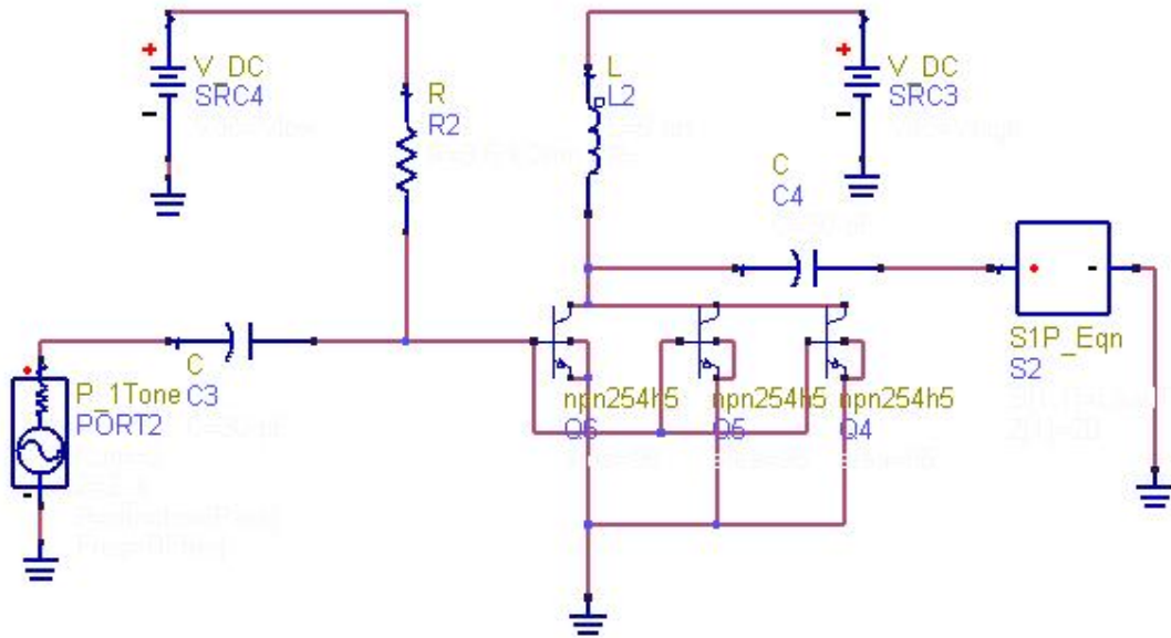
Figure 3.5: Load Pull Setup in ADS
