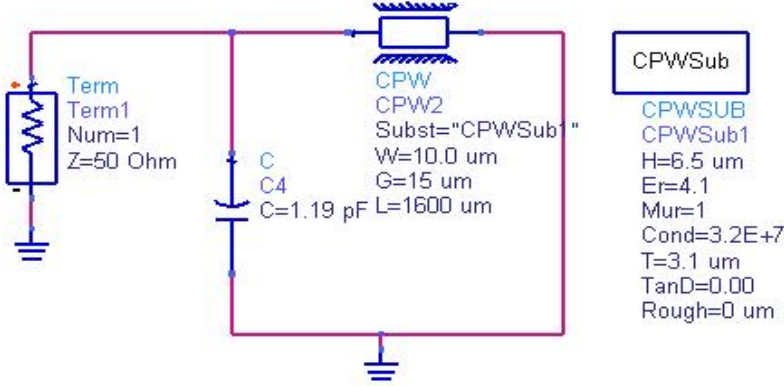
Figure 4.30: Modified CPW structure
