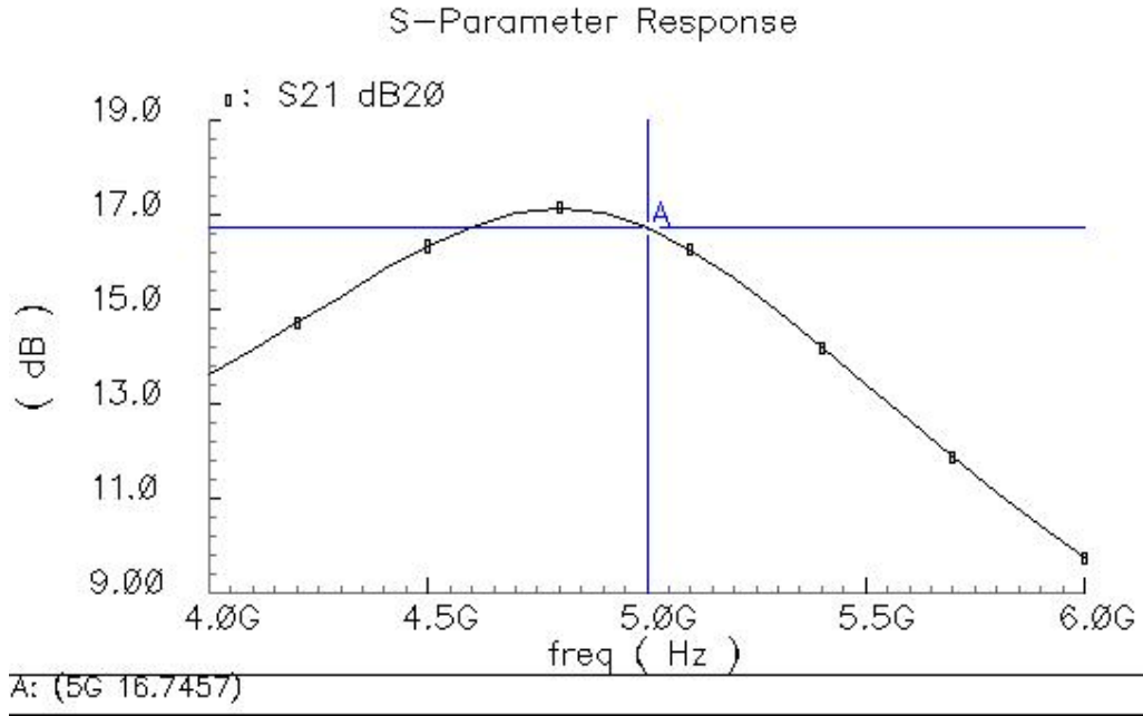
Figure 4.29: Power Gain ( S_{21} )
