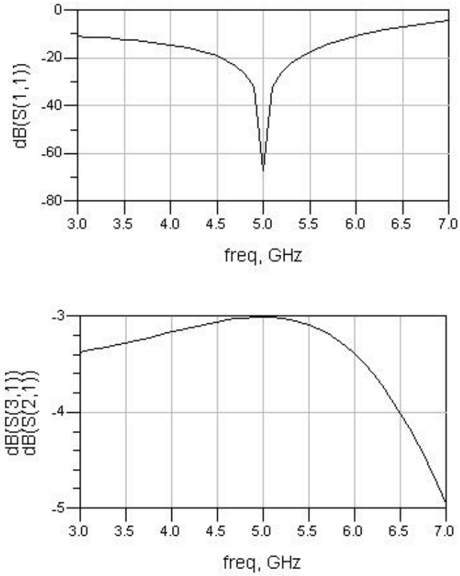
Figure 3.19: Simulated s_{11} , s_{21} and s_{31} parameters of lumped element Wilkinson power splitter model
