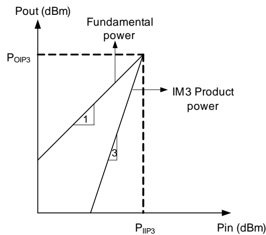
Figure 2.9: Third Order Intercept Point
