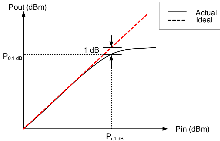
Figure 2.7: 1 dB compression characteristics
