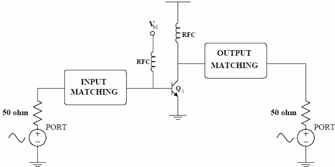
Figure 2.6: Basic topology of a power amplifier
