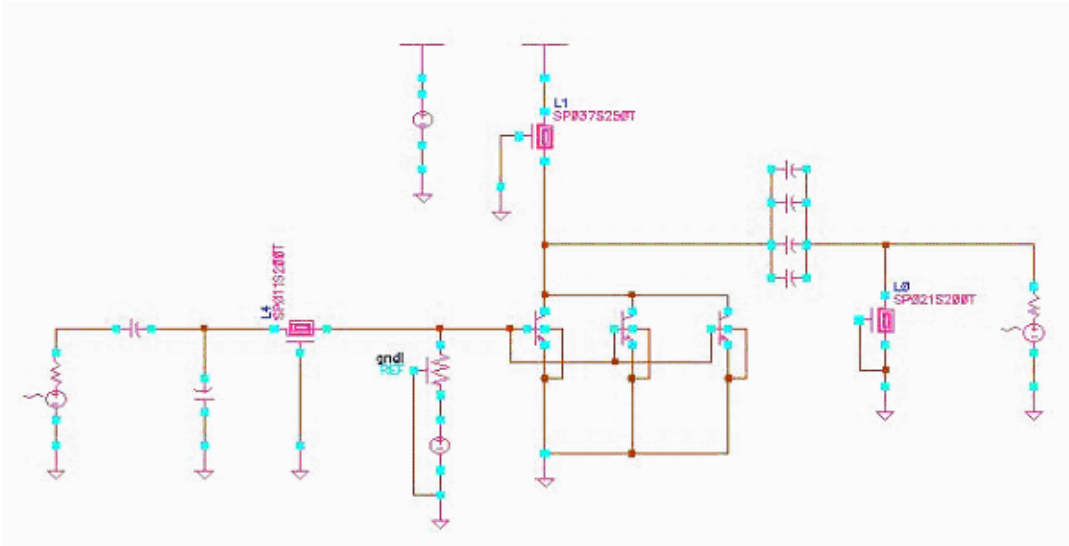
Figure 4.1: Simulation setup of single stage PA circuit
