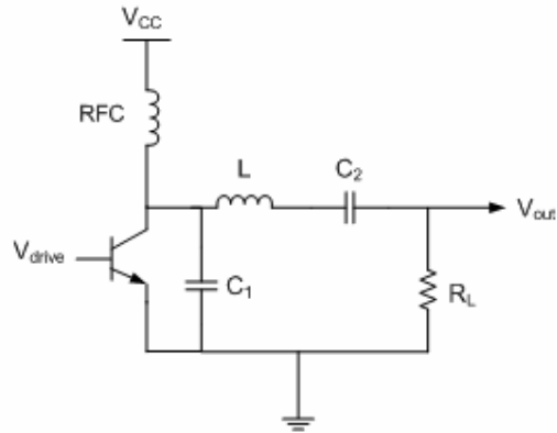
Figure 2.17: Class E amplifier
