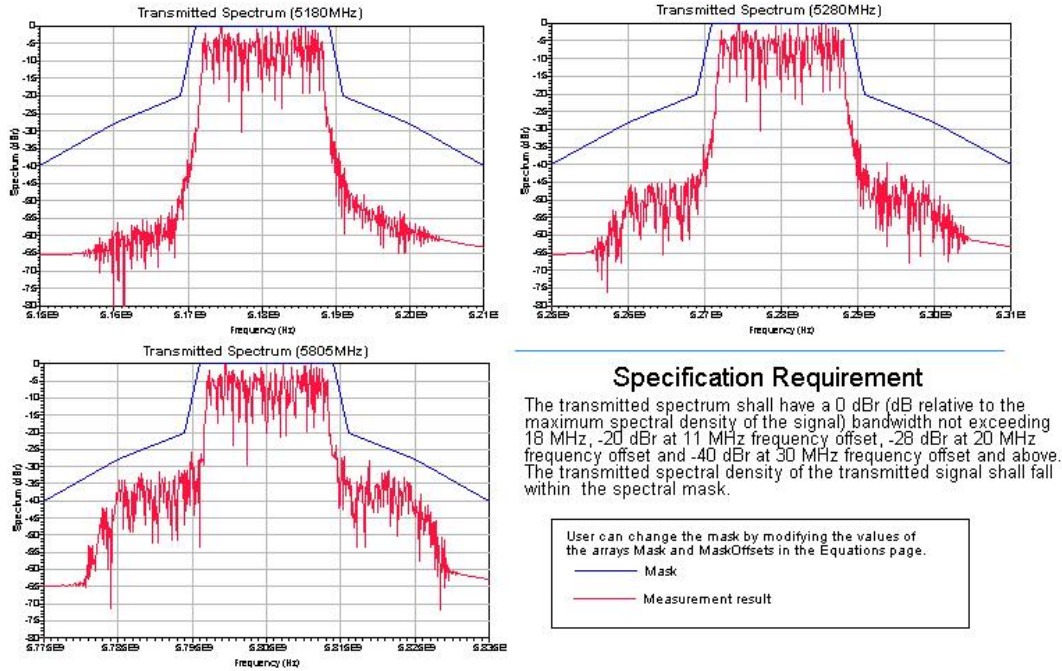
Figure 4.13: 802.11a transmit spectrum mask measurement results for three different frequency bands of 802.11a standard
