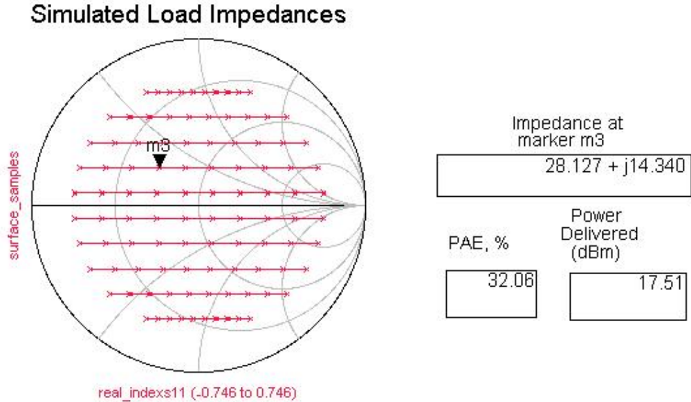
Figure 3.7: Simulated load impedances
