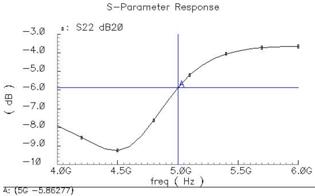
Figure 4.28: s_{22} response
