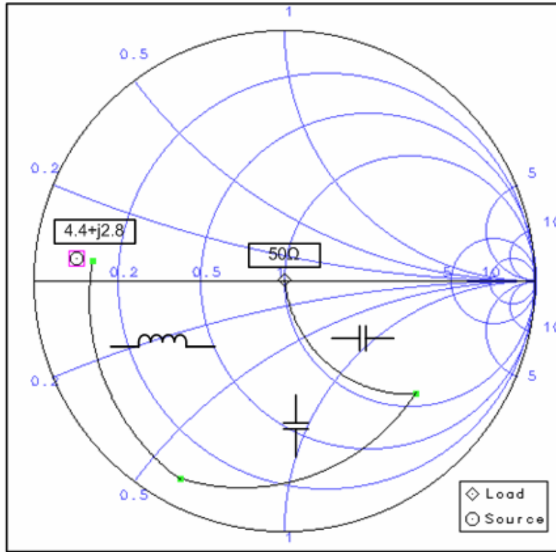
Figure 3.10: Input matching network design using ADS Smith Chart utility
