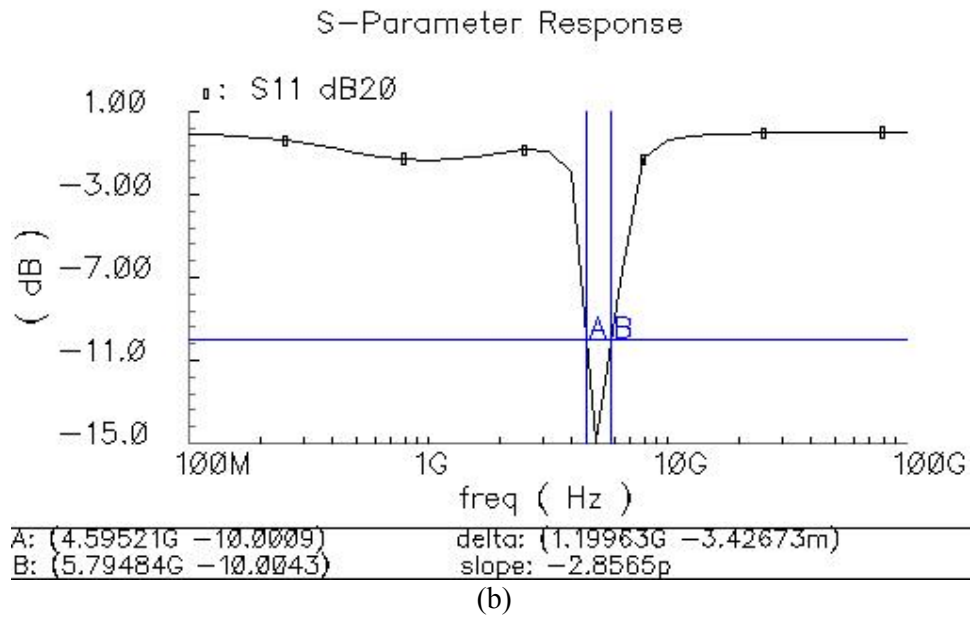
Figure 4.20: (a) s_{11} response (b) s_{11} in a logarithmic scale ( s_{11} is below -10 between 4.59 - 5.79 GHz bandwidth)
