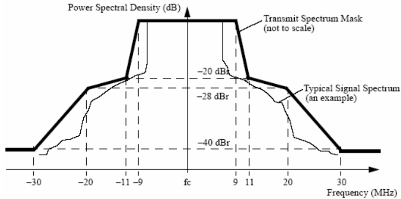
Figure 2.2: Transmit spectrum mask
