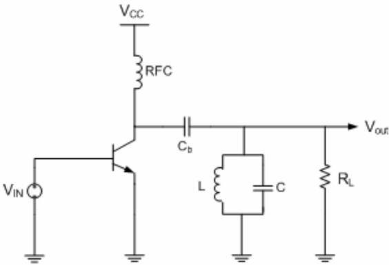
Figure 2.11: General linear power amplifier model
