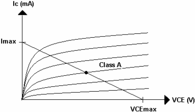
Figure 2.13: Class A Optimal Bias Point
