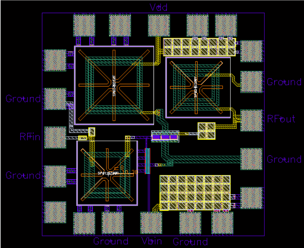
Figure 4.9: Layout of the single stage PA
