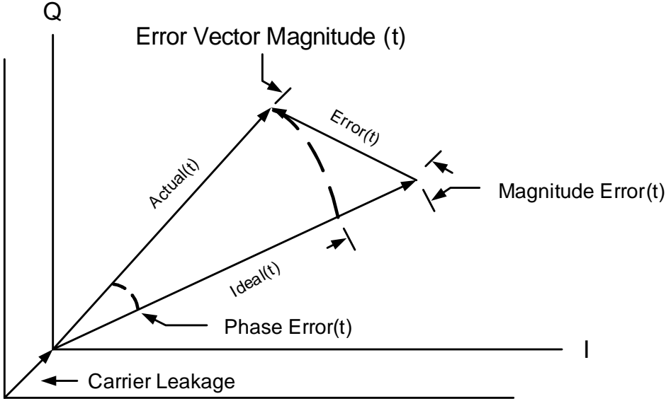
Figure 2.10: Error Vector Magnitude representation
