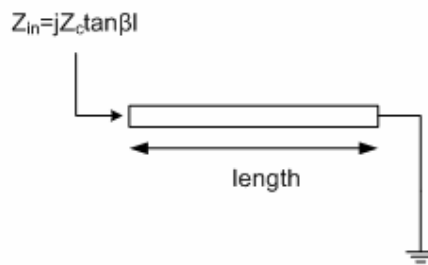
Figure 3.20: Short circuited transmission line
