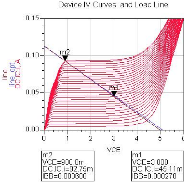
Figure 3.3: Transistor I-V curves
