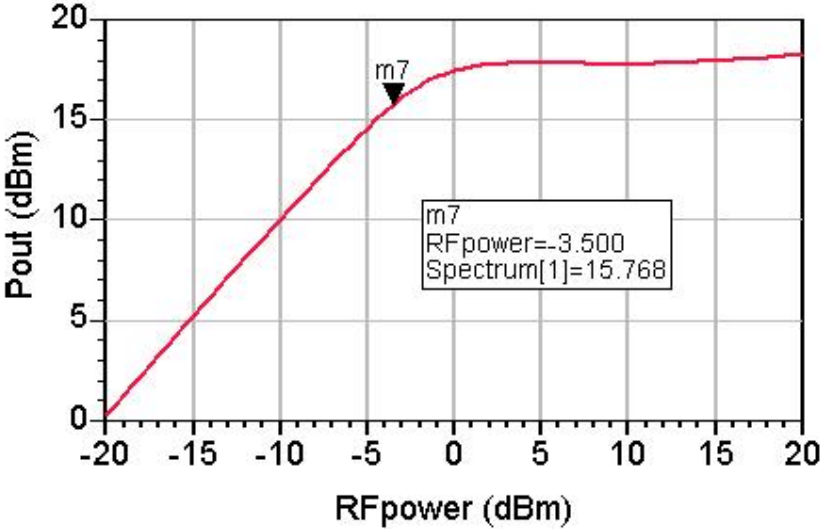
Figure 3.13: Single stage Class A output power and 1 dB compression point
