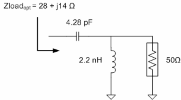
Figure 3.9: Output matching network
