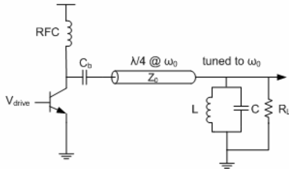
Figure 2.18: Class F amplifier
