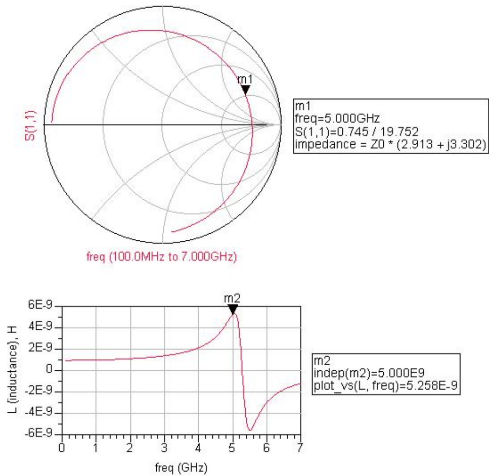
Figure 4.33: Inductance of the CPW Structure in Figure 4.35
