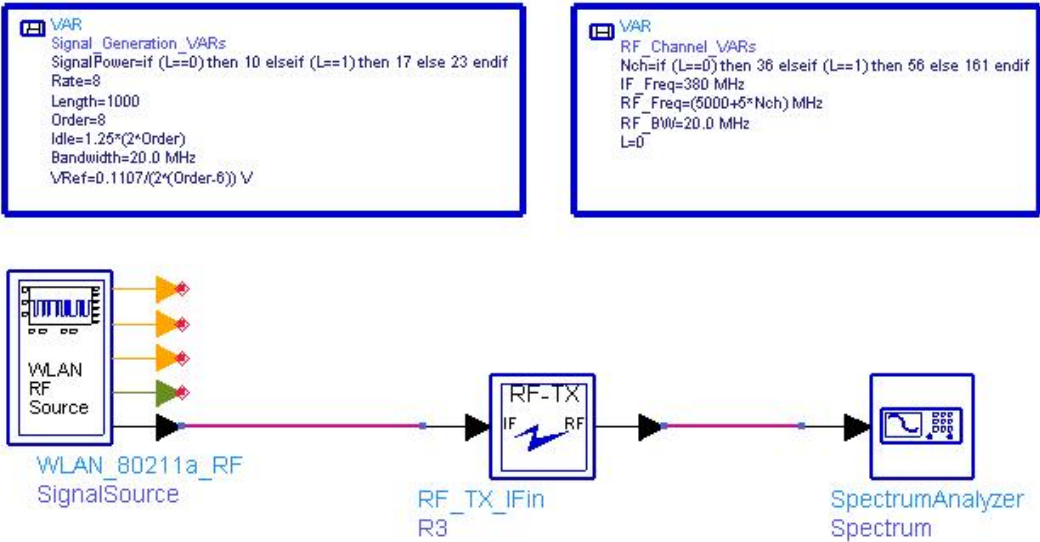
Figure 4.10: WLAN 802.11a spectrum measurement setup
