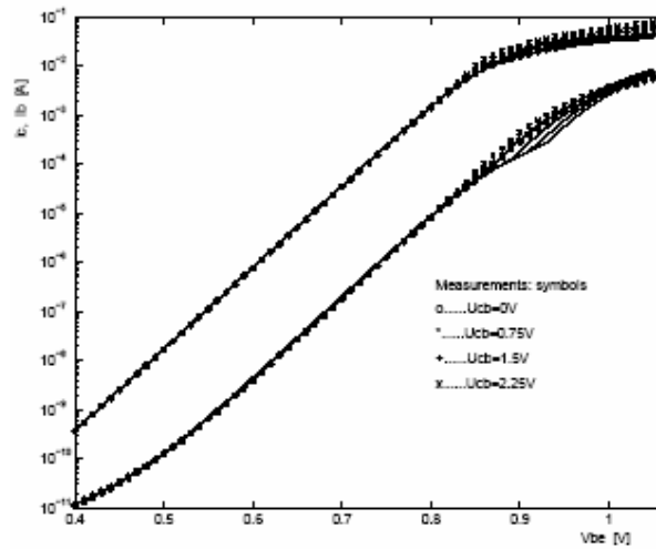
Figure A.2: Gummel Plots of a bipolar transistor (npn254h5; 24µm emitter length)
