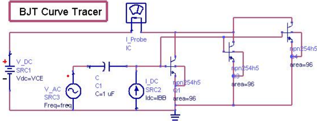
Figure 3.2: This circuit generates I-V curves and computes optimal bias for Class A operation
