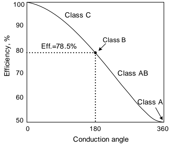
Figure 2.16: Maximum theoretical efficiency of an ideal amplifier as a function of conduction angle
