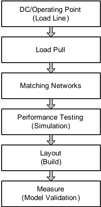
Figure 3.1: PA design roadmap
