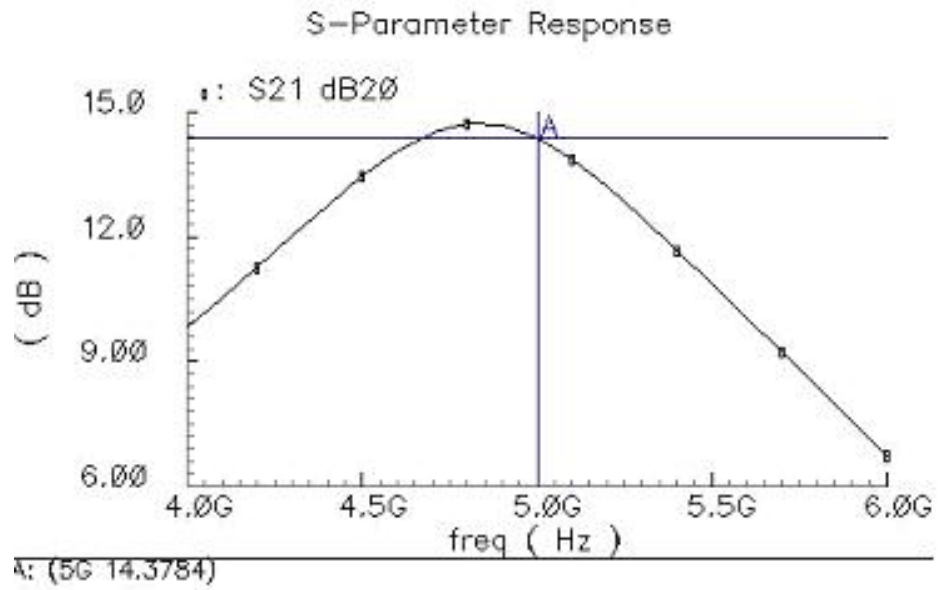
Figure 4.22: Power Gain ( s_{21} )
