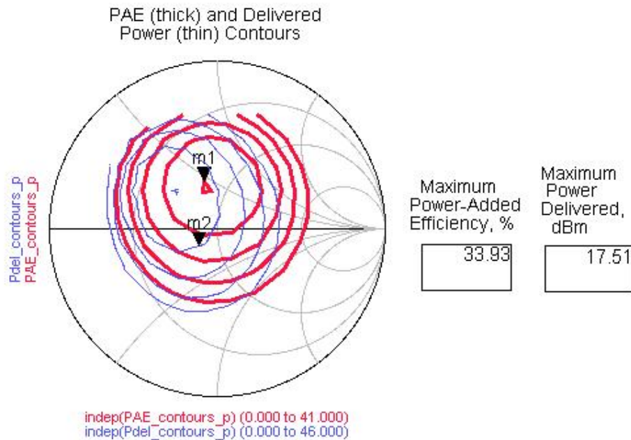
Figure 3.6: Maximum PAE and Pout circles on the Smith Chart
