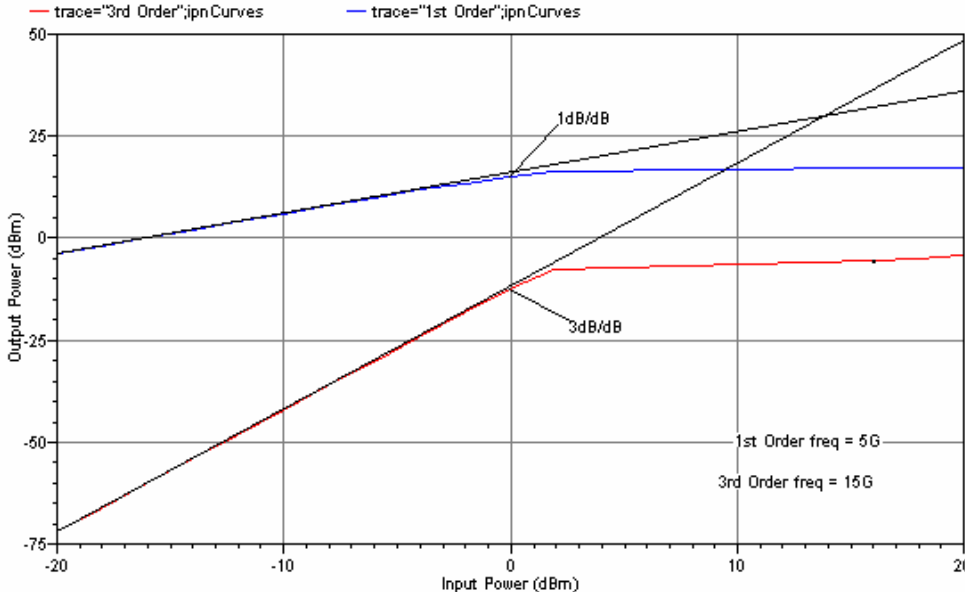
Figure 4.7: Third Order Intercept point
