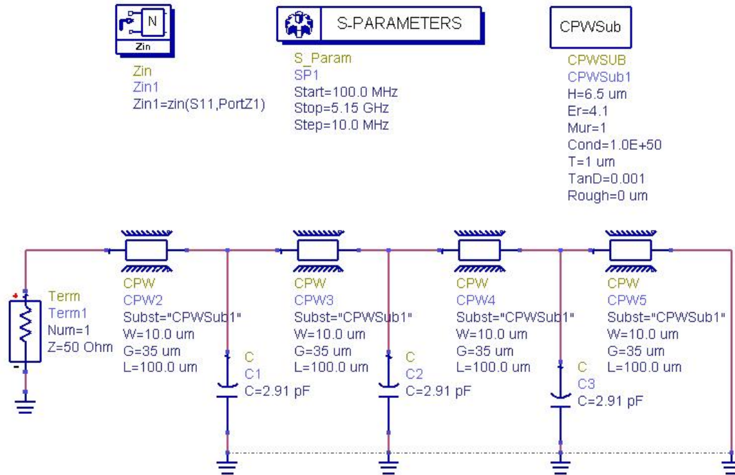
Figure 3.24: Capacitively loaded coplanar waveguide model
