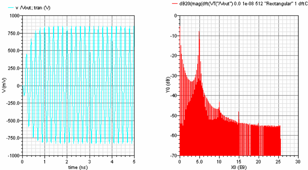
Figure 4.24: Output voltage waveform and power spectrum at -10 dBm input power
