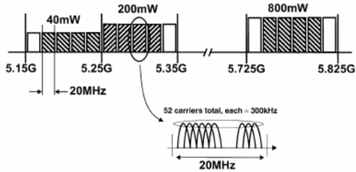
Figure 2.1: OFDM PHY frequency channel plan for the United States
