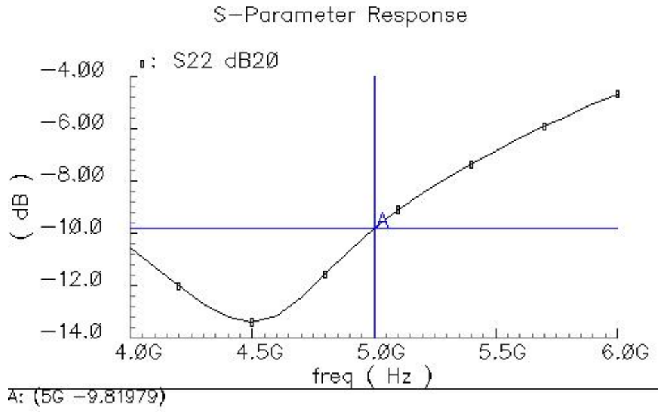
Figure 4.21: s_{22} response
