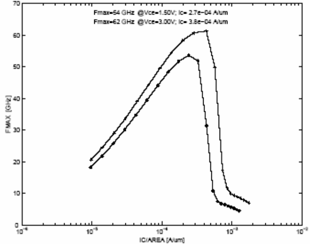
Figure A.5: Fmax plots of a bipolar transistor (npn254h5; 12µm emitter length) for a typical wafer
