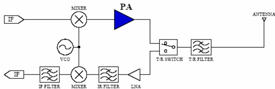
Figure 2.5: Block diagram of an RF transceiver
