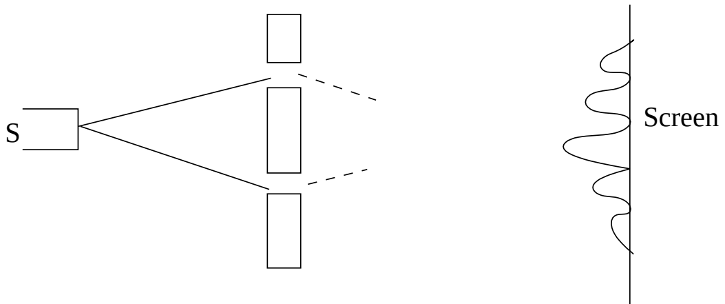
Figure 1.3. Double-Slit
