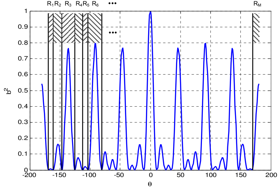
Figure 3-6 Partitioning of b^2
