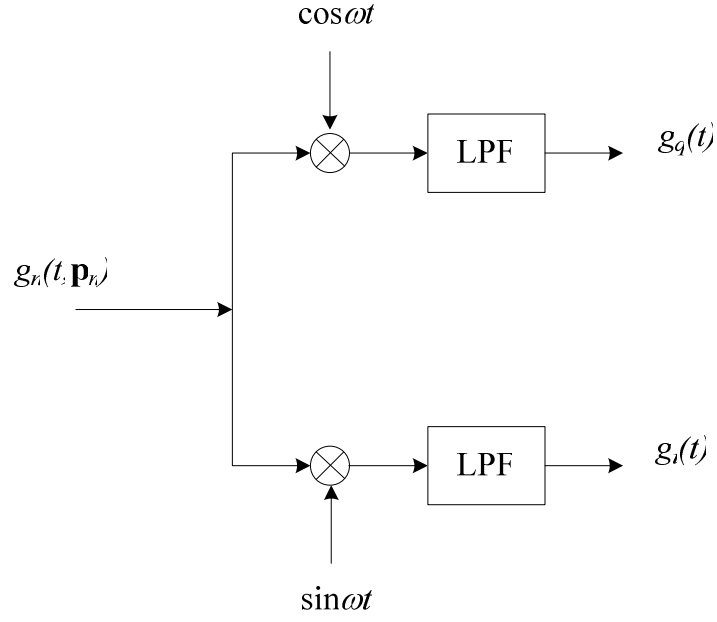
Figure 2-3 Quadrature demodulation
