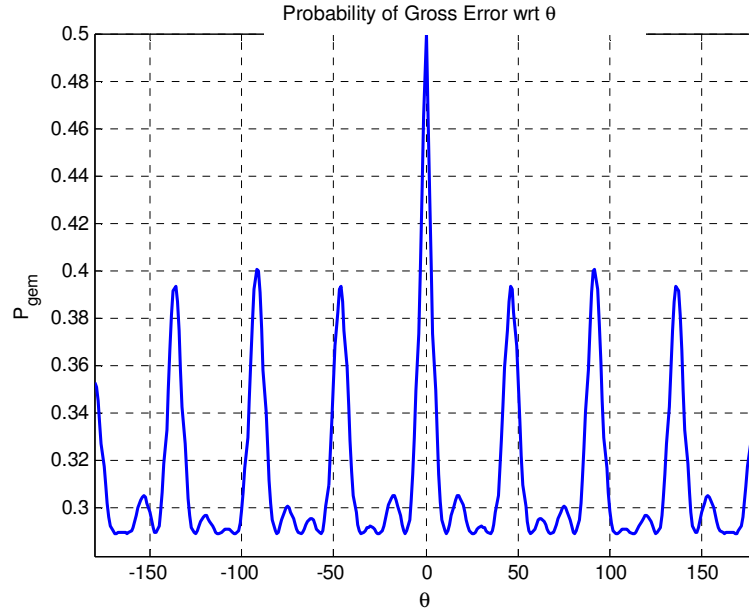
Figure 3-7 Calculated probability of gross error for the UCA when SNR = -20 \text{ dB}
