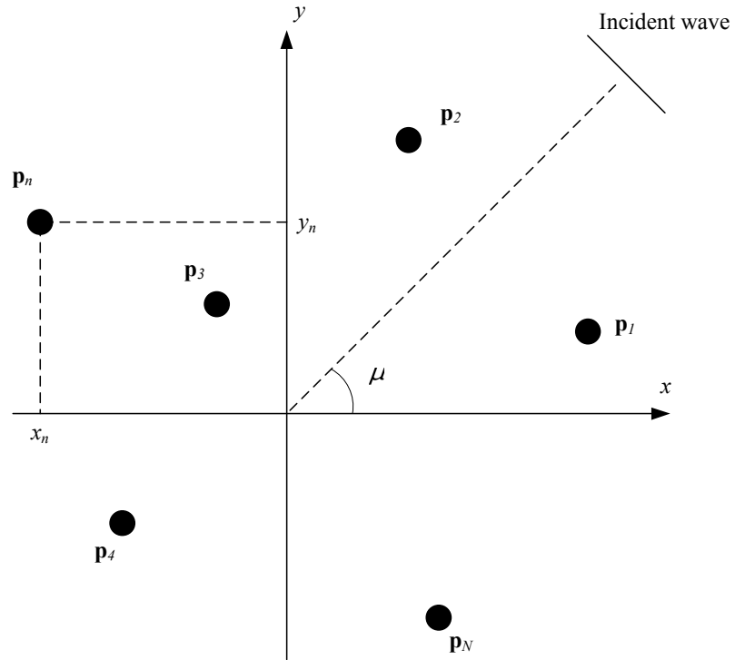
Figure 2-2 Planar array geometry
