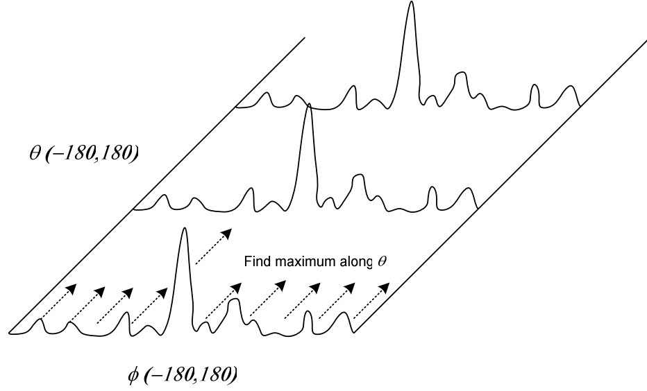
Figure 4-4 Procedure of forming M(\phi)
