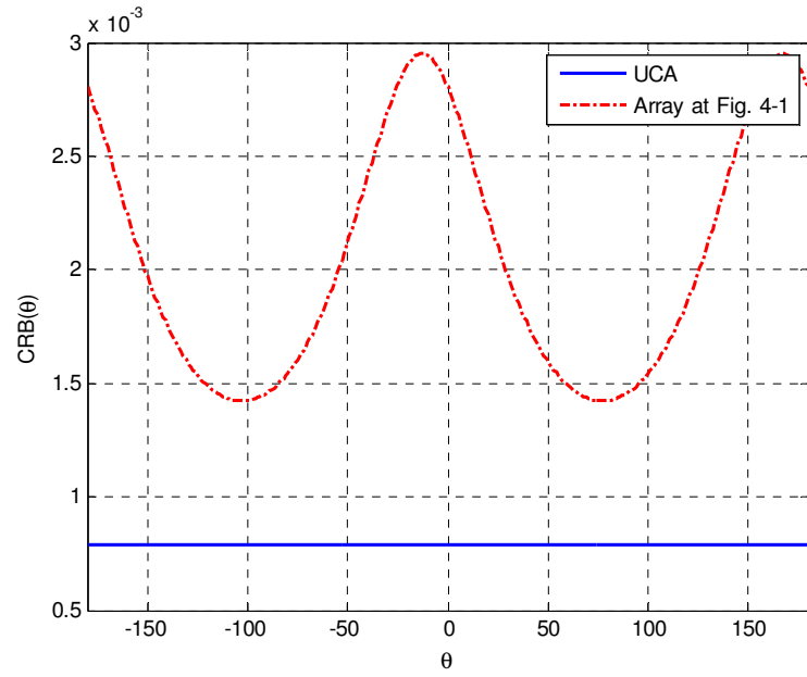
Figure 4-9 Comparison of the CRB of both arrays
