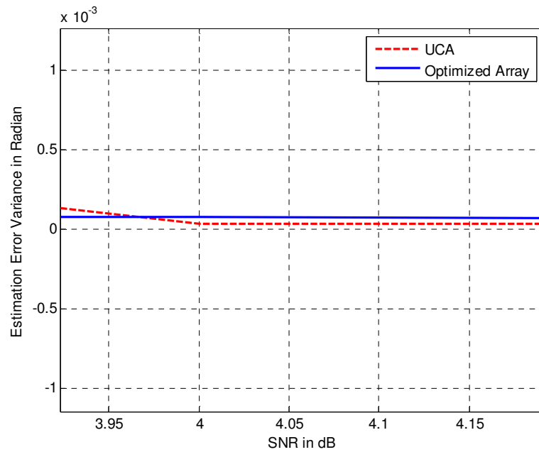
Figure 5-15 Effect of the main lobe expansion to the error variances
