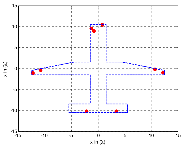
Figure 5-44 The optimized array of 9 elements when the threshold is 8.6
