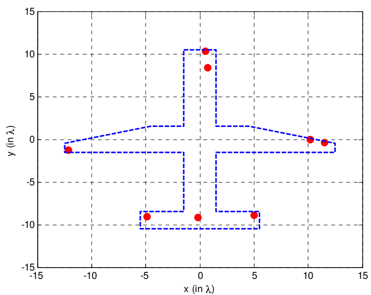
Figure 5-42 The optimized array of 8 elements when the threshold is 7.7
