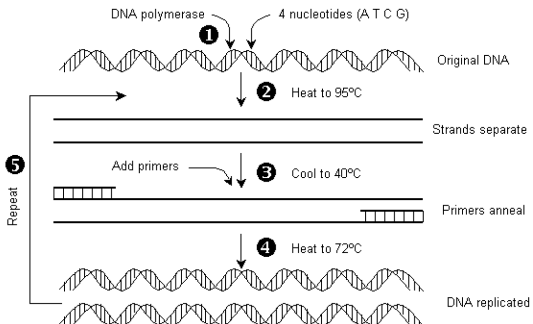
Figure 2.2 The Polymerase Chain Reaction ( http://www.biologymad.com )
