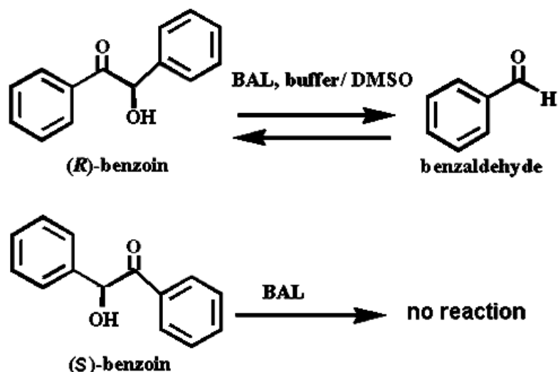
Figure 1.2 Conversion reaction of (R)- and (S)- enantiomers of benzoin molecule.
