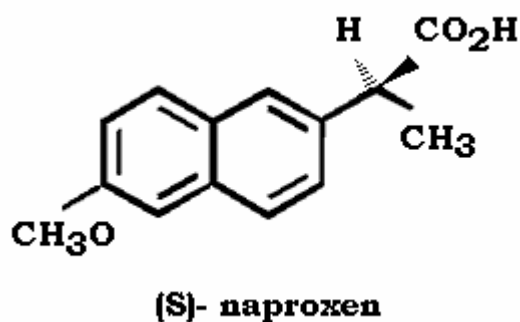
Figure 1.1 S- enantiomers of naproxen molecule.
